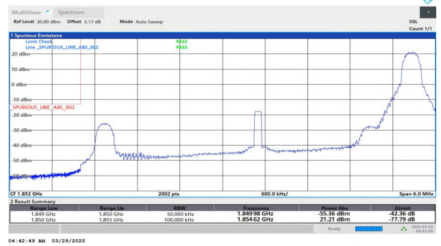
Band25-5MHz-QPSK-26065-1RB#24-PASS
