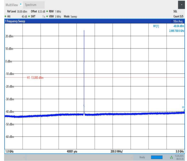
Band25-1.4MHz-QPSK-26365-1RB#0-1000~3000-PASS
