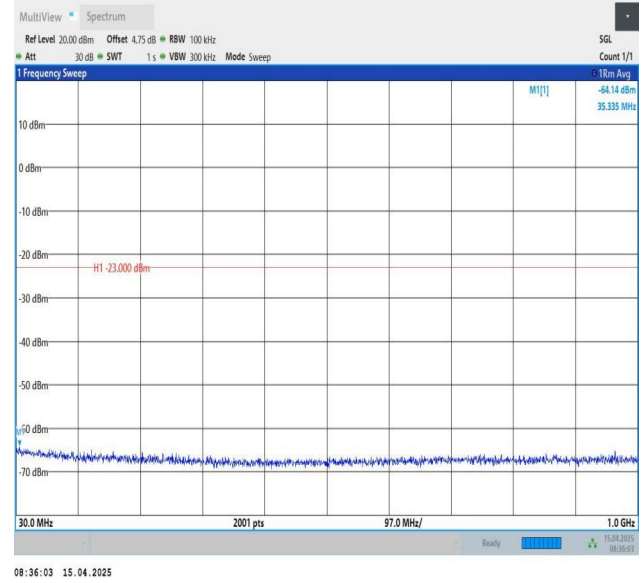
Band25-1.4MHz-QPSK-26365-1RB#5-30~1000-PASS
