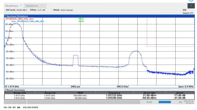
Band25-3MHz-QPSK-26675-1RB#0-PASS
