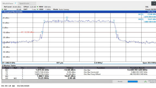
Band25-15MHz-QPSK-26365-75RB#0-PASS
