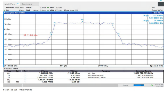
Band25-1.4MHz-16QAM-26365-6RB#0-PASS
