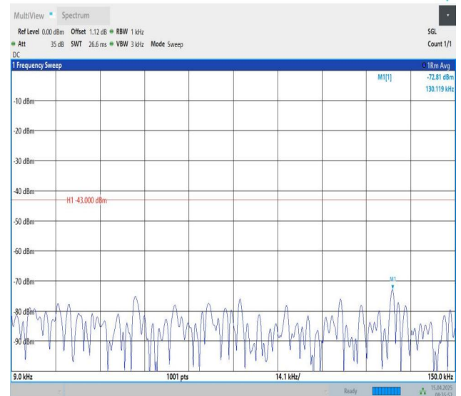
Band25-1.4MHz-QPSK-26365-1RB#5-0.009~0.15-PASS
