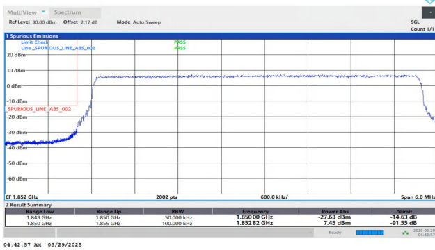
Band25-5MHz-QPSK-26065-25RB#0-PASS
