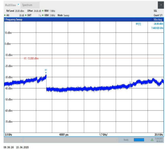
Band25-1.4MHz-QPSK-26365-1RB#5-3000~20000-PASS
