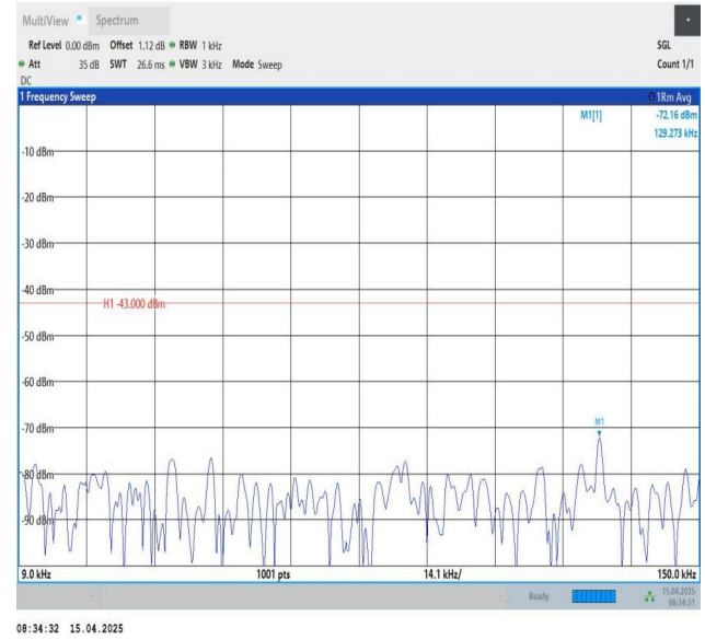
Band25-1.4MHz-QPSK-26047-1RB#5-0.009~0.15-PASS
