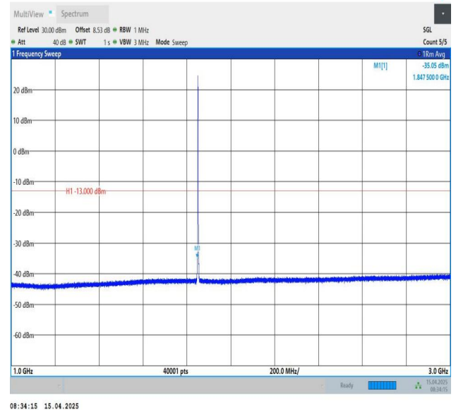
Band25-1.4MHz-QPSK-26047-1RB#0-1000~3000-PASS
