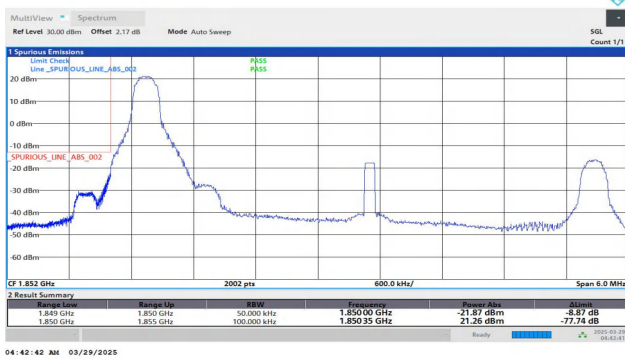
Band25-5MHz-QPSK-26065-1RB#0-PASS
