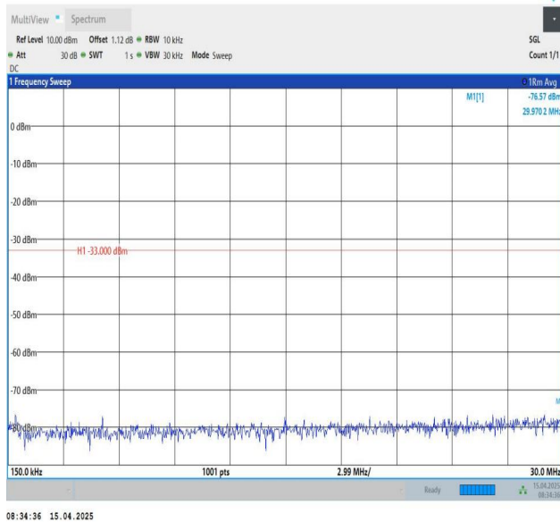
Band25-1.4MHz-QPSK-26047-1RB#5-0.15~30-PASS
