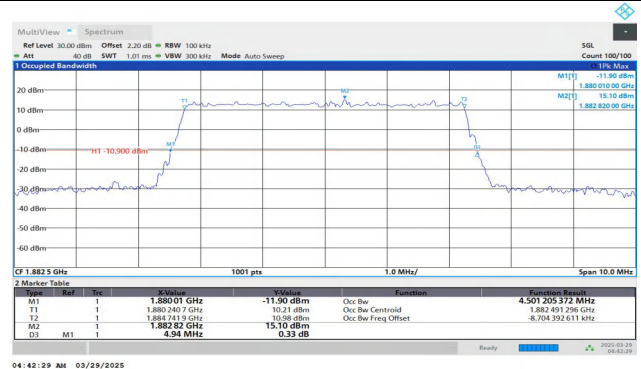
Band25-5MHz-16QAM-26365-25RB#0-PASS
