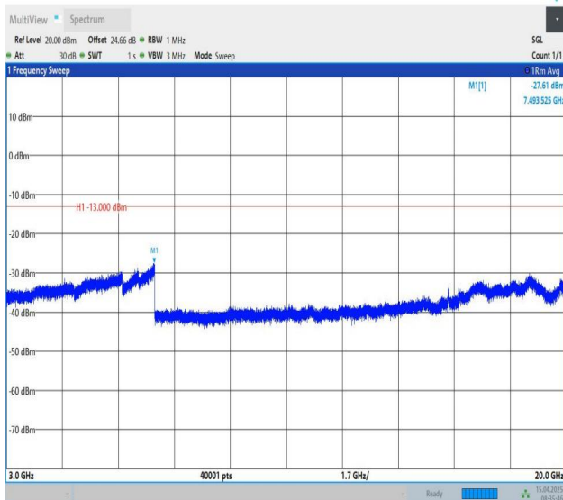
Band25-1.4MHz-QPSK-26365-1RB#0-3000~20000-PASS
