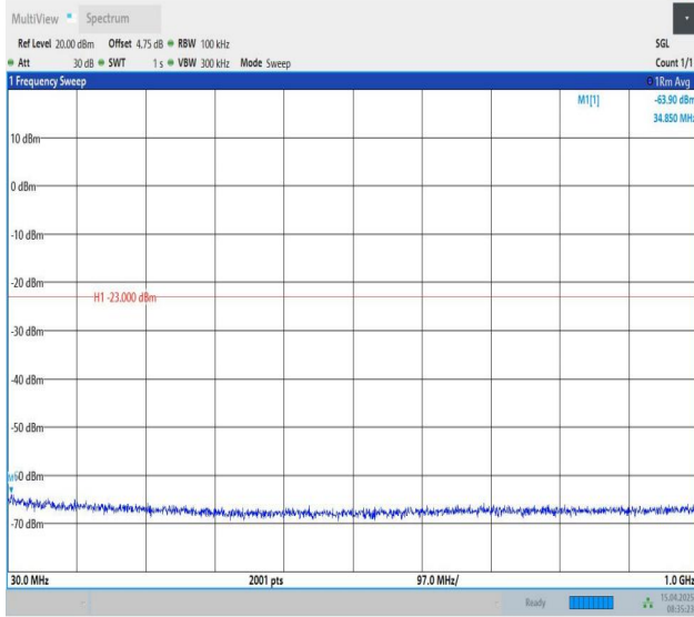
Band25-1.4MHz-QPSK-26365-1RB#0-30~1000-PASS
