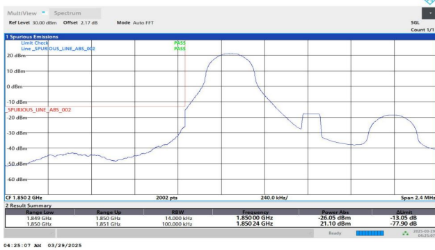
Band25-1.4MHz-QPSK-26047-1RB#0-PASS
