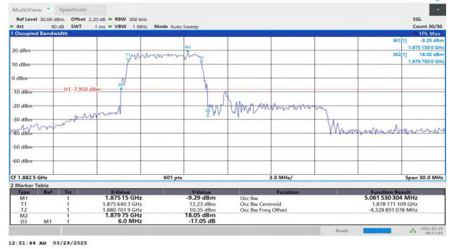
Band25-15MHz-16QAM-26365-27RB#0-PASS
