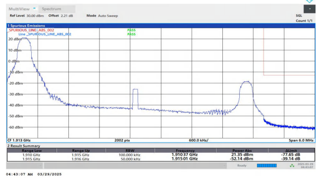
Band25-5MHz-QPSK-26665-1RB#0-PASS
