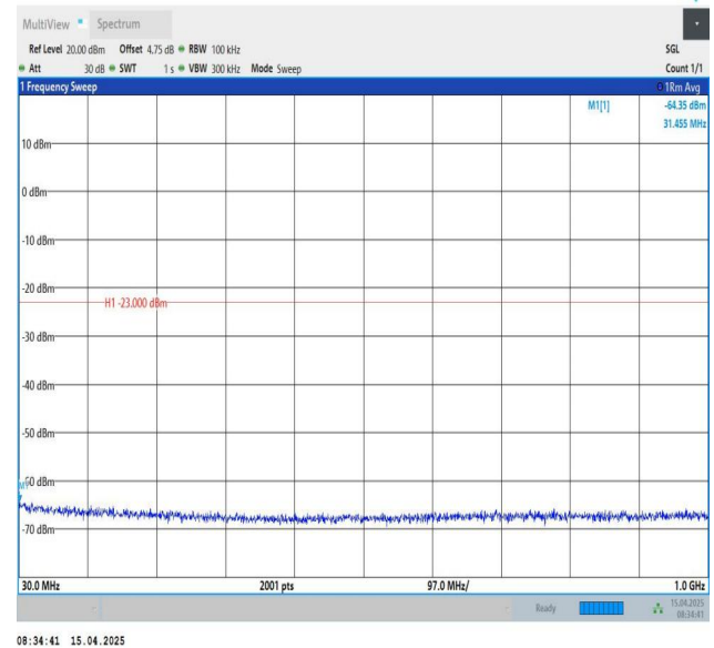
Band25-1.4MHz-QPSK-26047-1RB#5-30~1000-PASS
