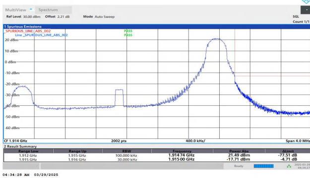
Band25-3MHz-QPSK-26675-1RB#14-PASS
