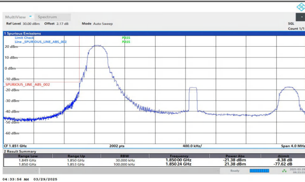
Band25-1.4MHz-QPSK-26683-1RB#5-PASS
