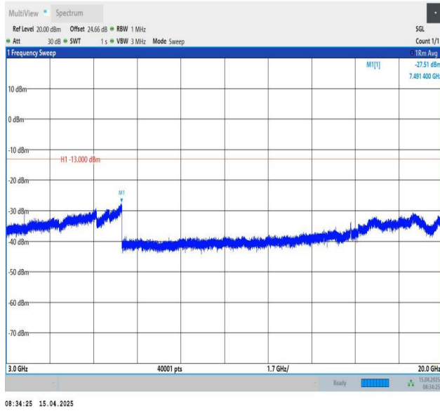
Band25-1.4MHz-QPSK-26047-1RB#0-3000~20000-PASS
