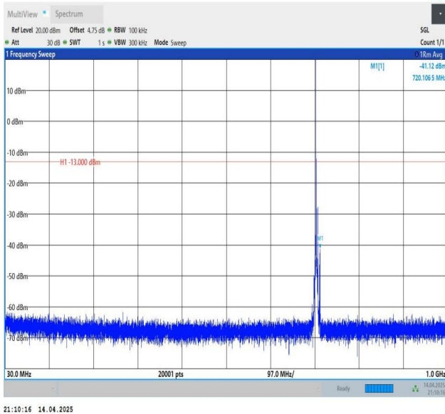
Band12-5MHz-QPSK-23155-1RB#0-30~1000-PASS
