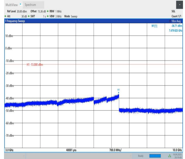
Band12-10MHz-QPSK-23095-1RB#49-3000~10000-PASS
