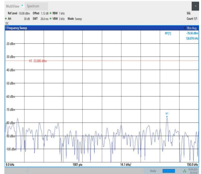
Band12-5MHz-QPSK-23095-1RB#24-0.009~0.15-PASS
