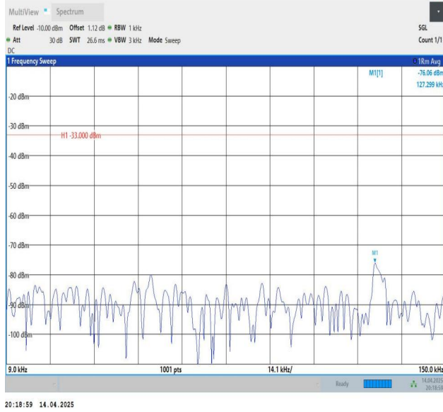
Band12-10MHz-QPSK-23095-1RB#0-0.009~0.15-PASS
