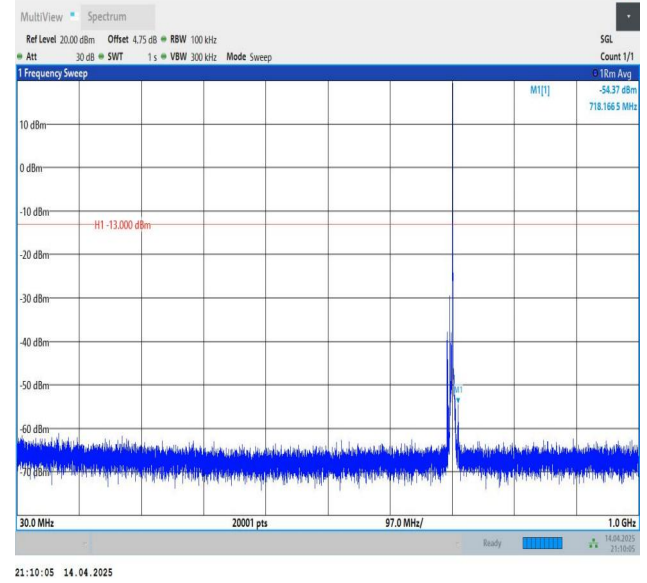
Band12-5MHz-QPSK-23095-1RB#24-30~1000-PASS
