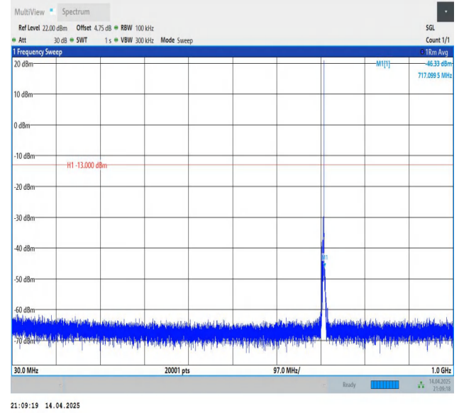
Band12-3MHz-QPSK-23165-1RB#14-30~1000-PASS
