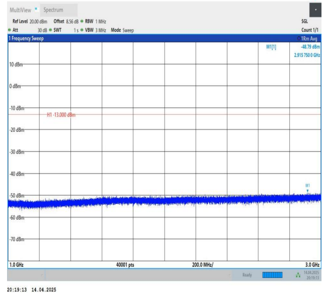
Band12-10MHz-QPSK-23095-1RB#0-1000~3000-PASS
