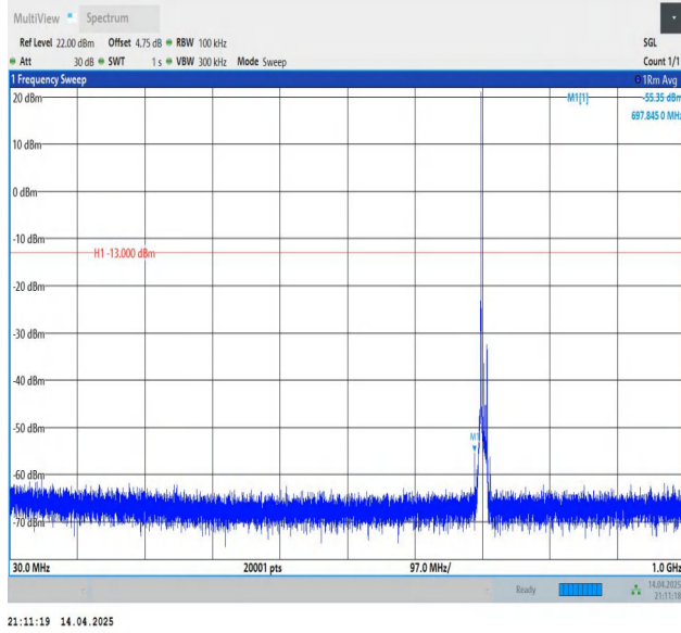
Band12-10MHz-QPSK-23130-1RB#0-30~1000-PASS
