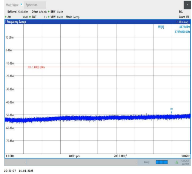
Band12-10MHz-QPSK-23130-1RB#0-1000~3000-PASS
