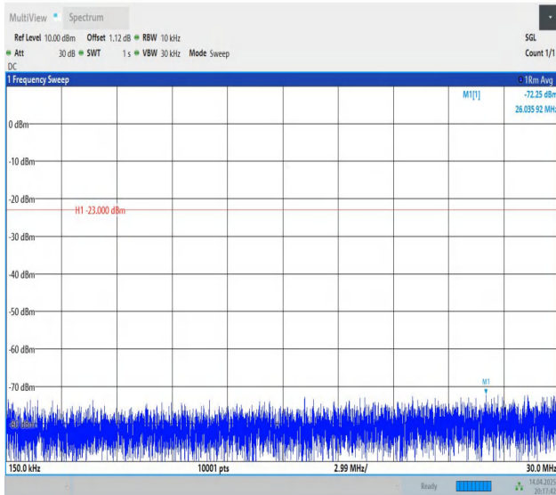
Band12-5MHz-QPSK-23155-1RB#24-0.15~30-PASS
