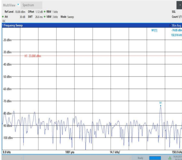
Band12-3MHz-QPSK-23165-1RB#0-0.009~0.15-PASS
