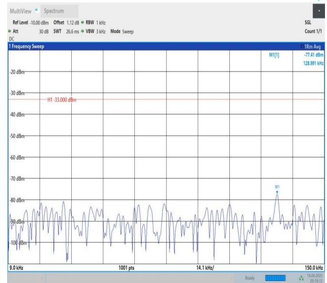
Band12-10MHz-QPSK-23060-1RB#49-0.009~0.15-PASS
