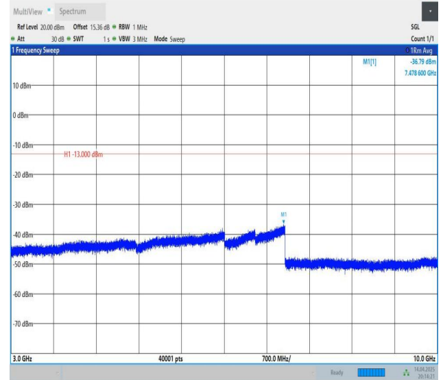
Band12-3MHz-QPSK-23095-1RB#14-3000~10000-PASS
