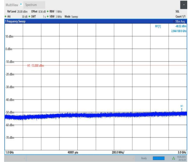
Band12-5MHz-QPSK-23095-1RB#0-1000~3000-PASS
