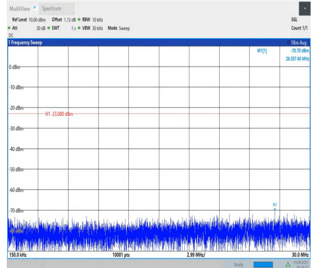
Band12-3MHz-QPSK-23165-1RB#0-0.15~30-PASS
