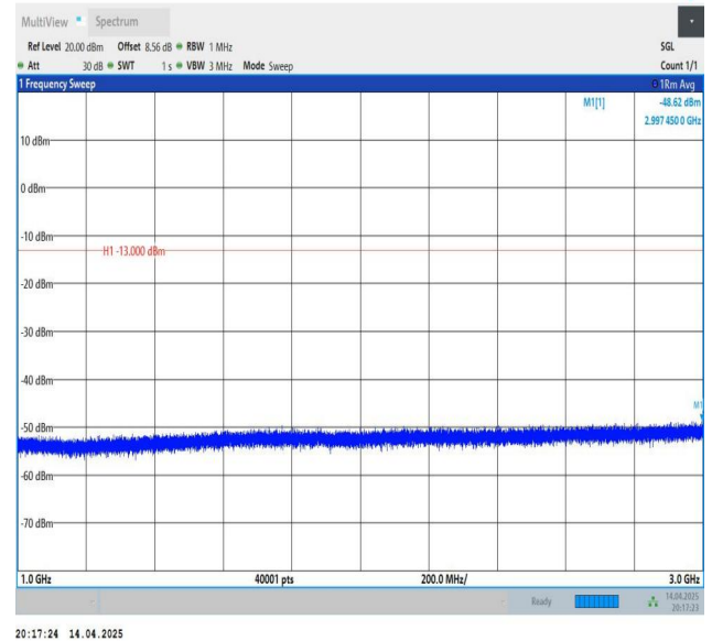
Band12-5MHz-QPSK-23155-1RB#0-1000~3000-PASS
