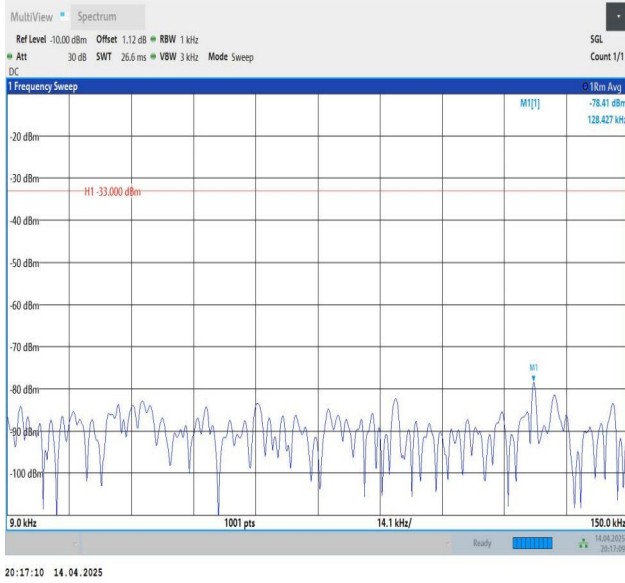
Band12-5MHz-QPSK-23155-1RB#0-0.009~0.15-PASS
