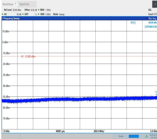
Band12-10MHz-QPSK-23095-1RB#49-1000~3000-PASS
