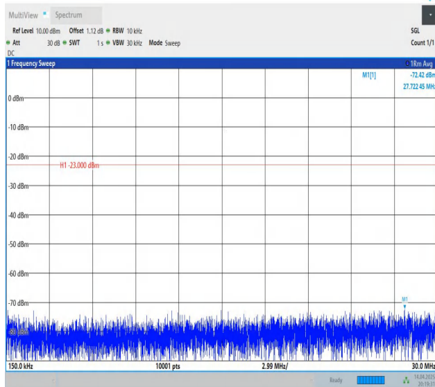
Band12-10MHz-QPSK-23095-1RB#49-0.15~30-PASS
