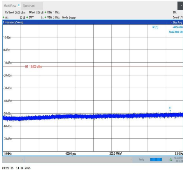
Band12-10MHz-QPSK-23130-1RB#49-1000~3000-PASS
