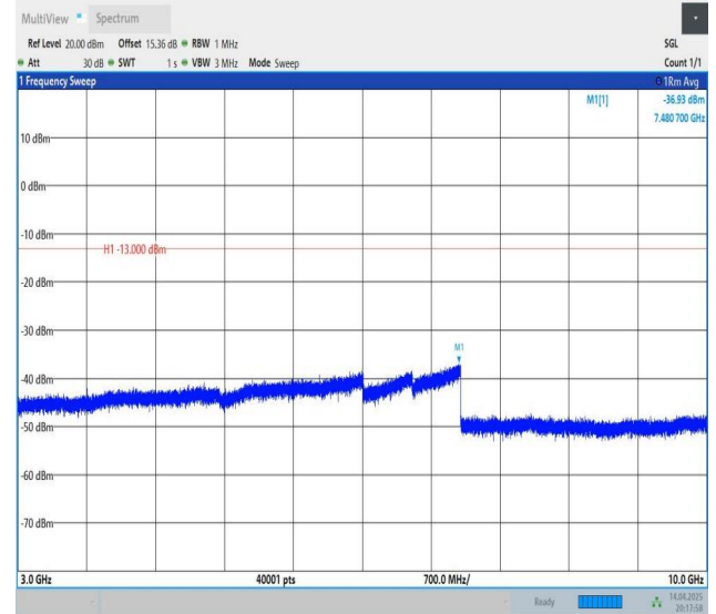
Band12-5MHz-QPSK-23155-1RB#24-3000~10000-PASS
