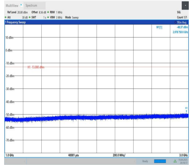
Band12-10MHz-QPSK-23060-1RB#0-1000~3000-PASS
