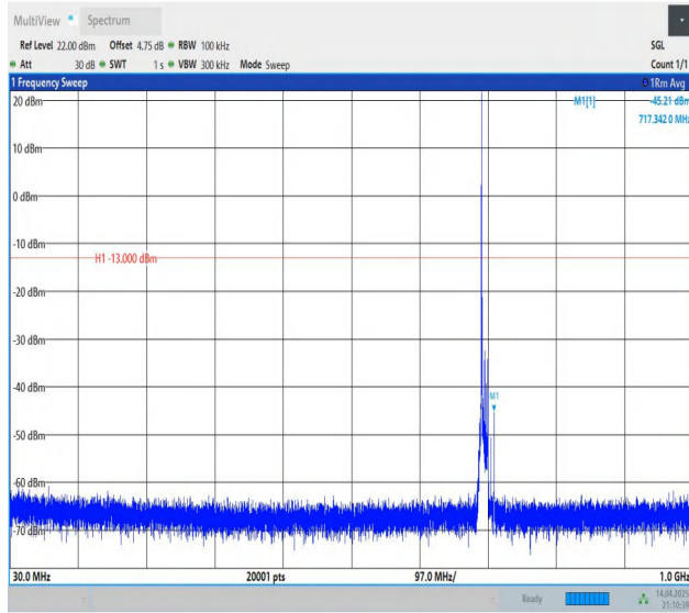
Band12-10MHz-QPSK-23060-1RB#0-30~1000-PASS
