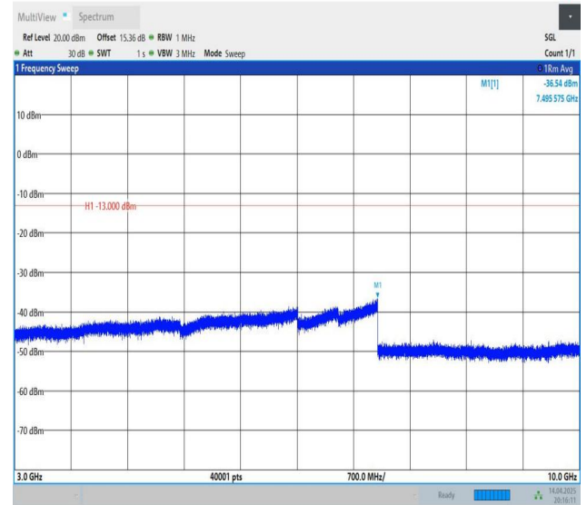
Band12-5MHz-QPSK-23035-1RB#24-3000~10000-PASS
