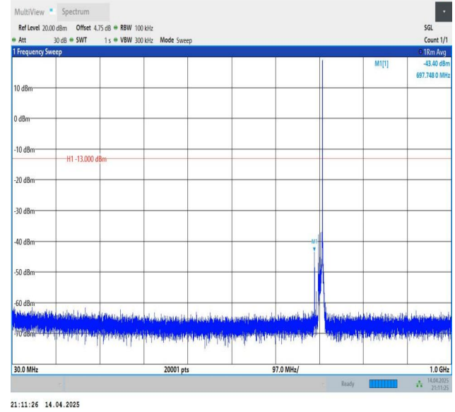
Band12-10MHz-QPSK-23130-1RB#49-30~1000-PASS
