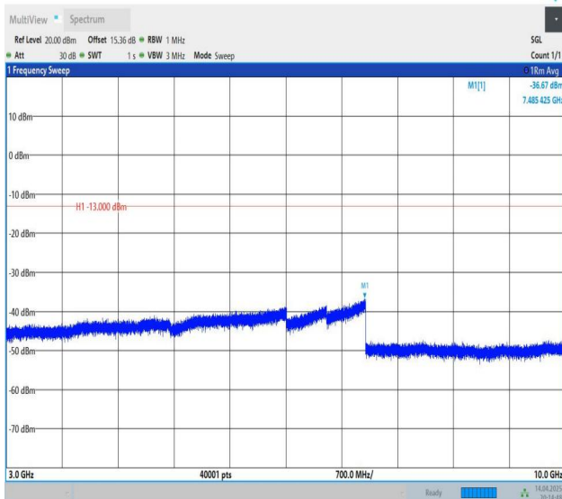
Band12-3MHz-QPSK-23165-1RB#0-3000~10000-PASS
