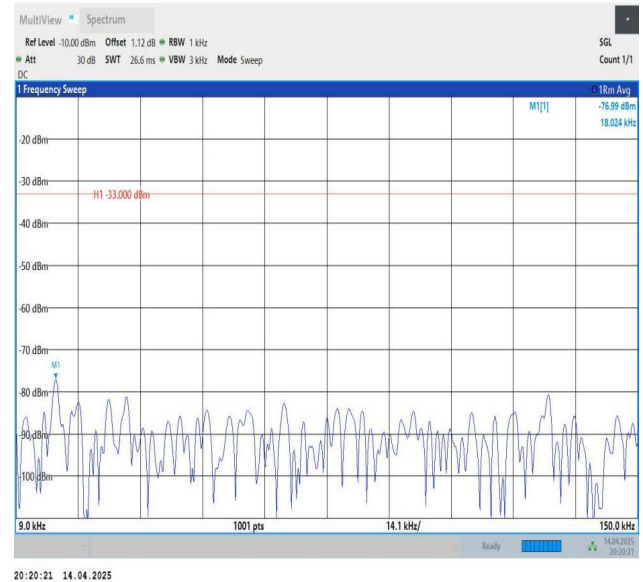
Band12-10MHz-QPSK-23130-1RB#49-0.009~0.15-PASS
