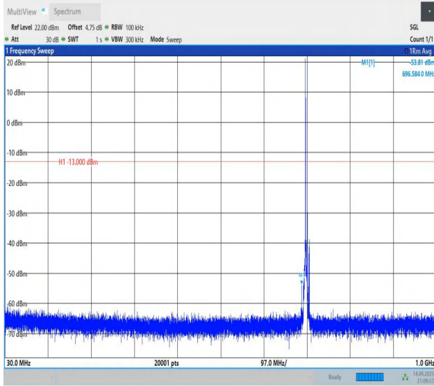
Band12-5MHz-QPSK-23095-1RB#0-30~1000-PASS
