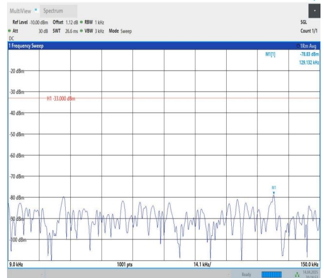
Band12-3MHz-QPSK-23165-1RB#14-0.009~0.15-PASS
