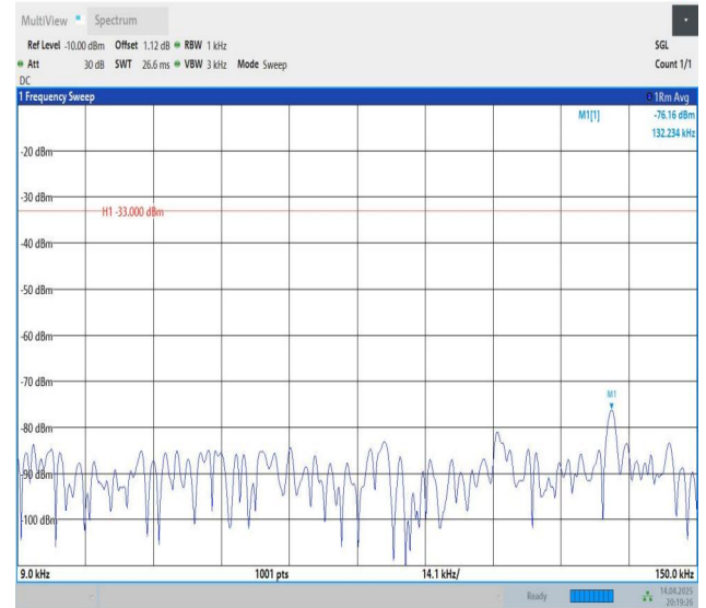
Band12-10MHz-QPSK-23095-1RB#49-0.009~0.15-PASS
