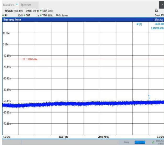
Band12-5MHz-QPSK-23035-1RB#24-1000~3000-PASS
