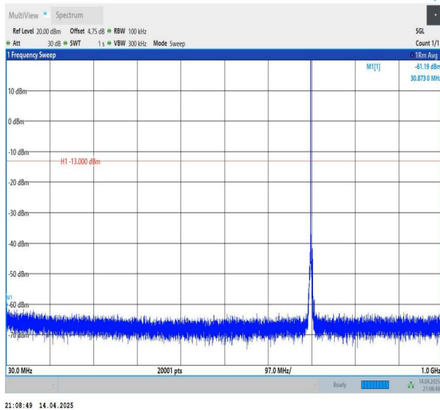
Band12-3MHz-QPSK-23095-1RB#0-30~1000-PASS
