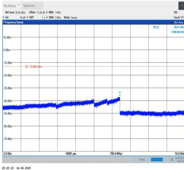
Band12-10MHz-QPSK-23130-1RB#0-3000~10000-PASS
