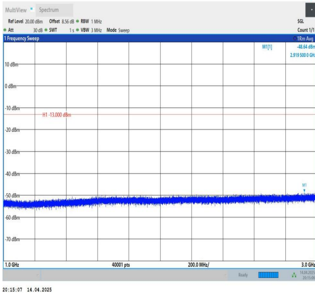
Band12-3MHz-QPSK-23165-1RB#14-1000~3000-PASS
