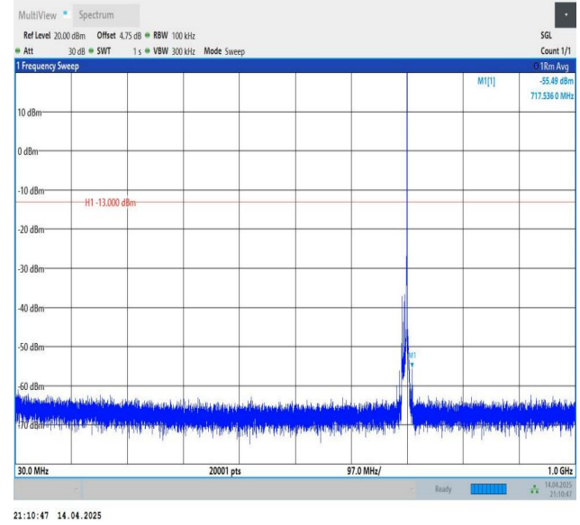
Band12-10MHz-QPSK-23060-1RB#49-30~1000-PASS
