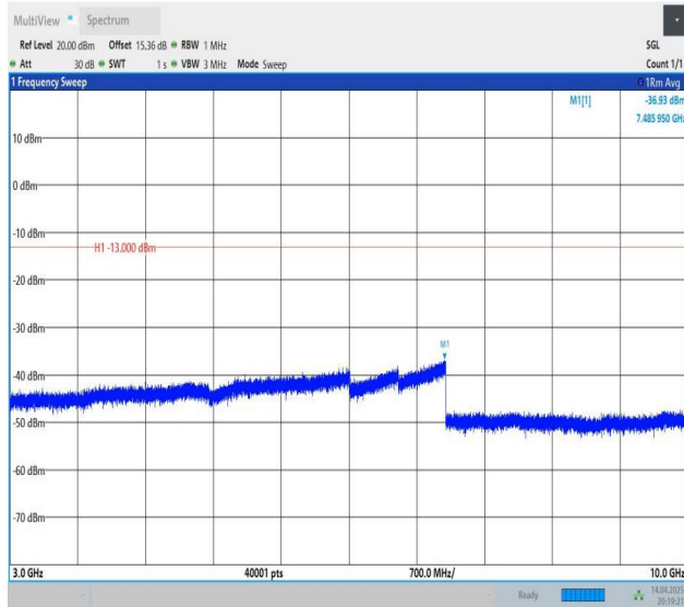
Band12-10MHz-QPSK-23095-1RB#0-3000~10000-PASS
