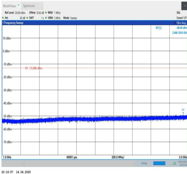
Band12-5MHz-QPSK-23095-1RB#24-1000~3000-PASS
