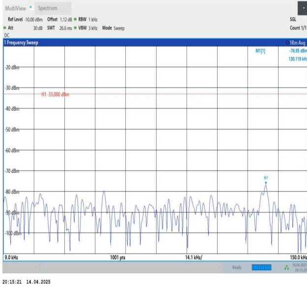
Band12-5MHz-QPSK-23035-1RB#0-0.009~0.15-PASS
