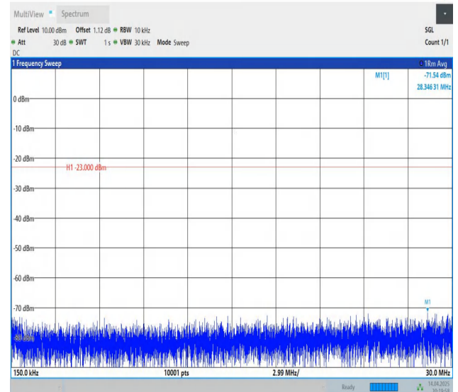
Band12-10MHz-QPSK-23130-1RB#0-0.15~30-PASS
