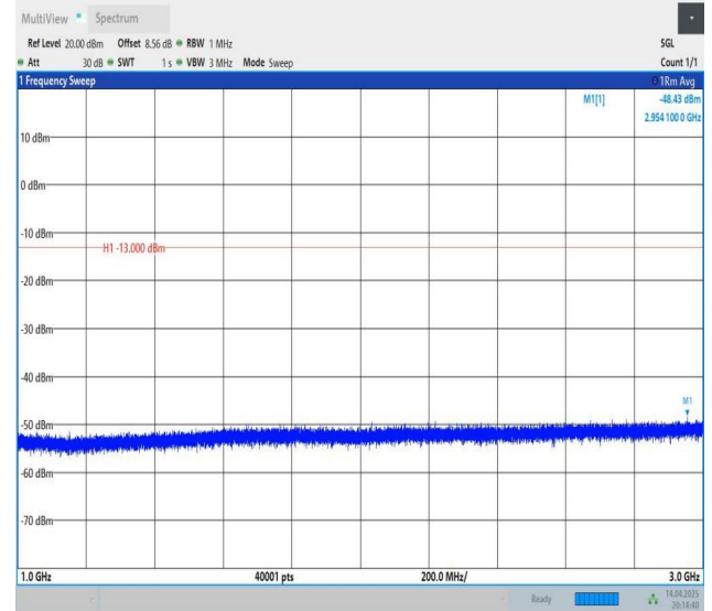
Band12-3MHz-QPSK-23165-1RB#0-1000~3000-PASS
