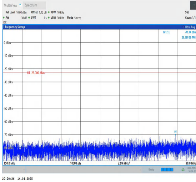
Band12-10MHz-QPSK-23130-1RB#49-0.15~30-PASS
