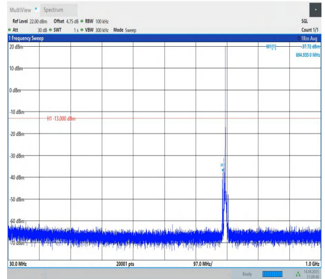
Band12-5MHz-QPSK-23035-1RB#24-30~1000-PASS
