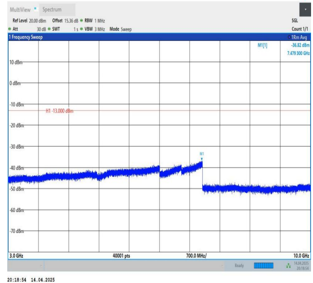
Band12-10MHz-QPSK-23060-1RB#49-3000~10000-PASS
