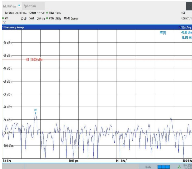
Band12-10MHz-QPSK-23130-1RB#0-0.009~0.15-PASS
