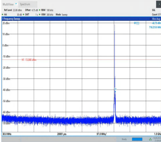
Band12-3MHz-QPSK-23165-1RB#0-30~1000-PASS
