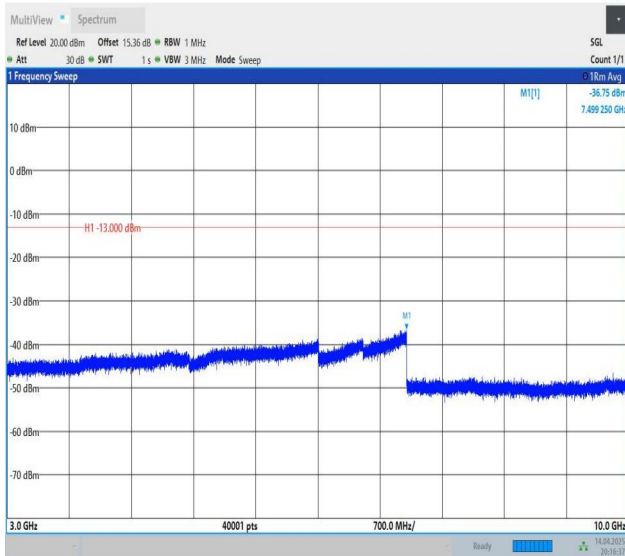
Band12-5MHz-QPSK-23095-1RB#0-3000~10000-PASS
