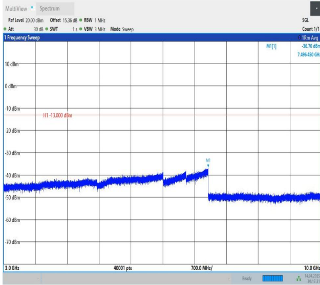
Band12-5MHz-QPSK-23155-1RB#0-3000~10000-PASS
