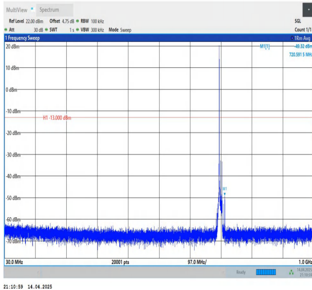
Band12-10MHz-QPSK-23095-1RB#0-30~1000-PASS
