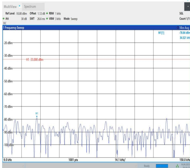
Band12-5MHz-QPSK-23095-1RB#0-0.009~0.15-PASS
