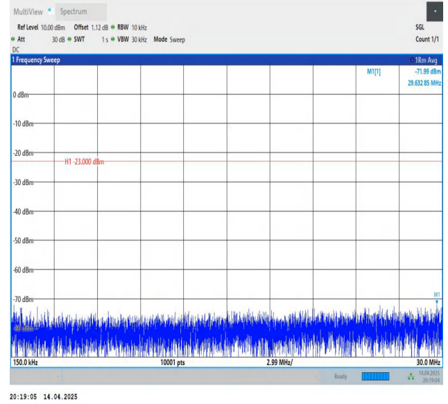
Band12-10MHz-QPSK-23095-1RB#0-0.15~30-PASS
