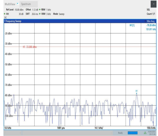
Band12-5MHz-QPSK-23155-1RB#24-0.009~0.15-PASS
