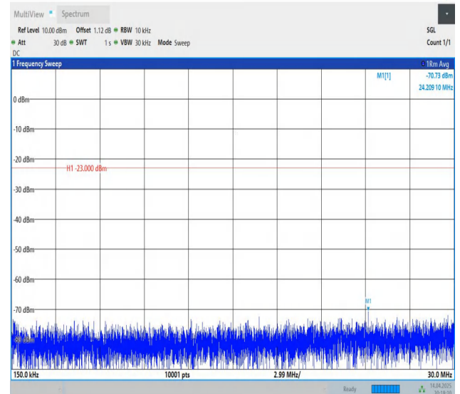
Band12-10MHz-QPSK-23060-1RB#0-0.15~30-PASS
