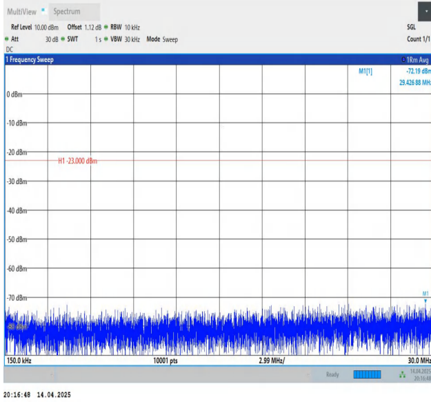
Band12-5MHz-QPSK-23095-1RB#24-0.15~30-PASS
