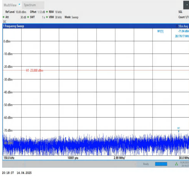
Band12-10MHz-QPSK-23060-1RB#49-0.15~30-PASS
