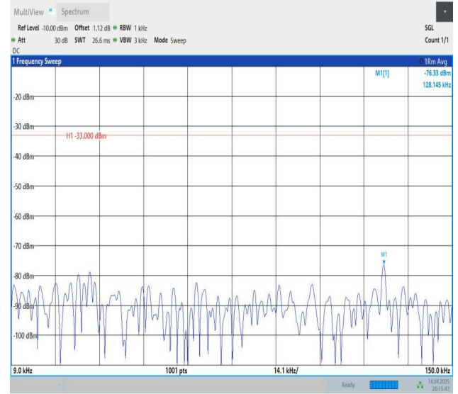
Band12-5MHz-QPSK-23035-1RB#24-0.009~0.15-PASS
