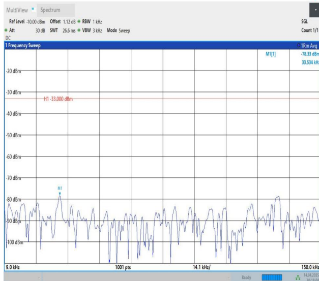
Band12-10MHz-QPSK-23060-1RB#0-0.009~0.15-PASS
