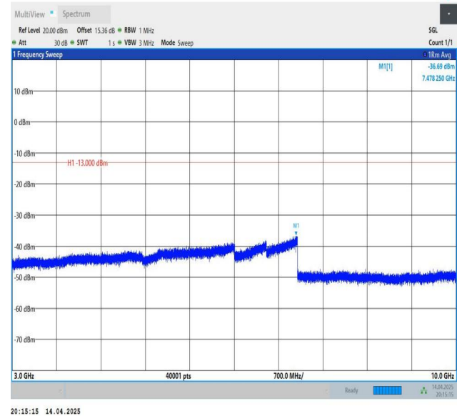
Band12-3MHz-QPSK-23165-1RB#14-3000~10000-PASS
