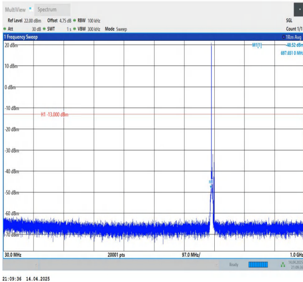
Band12-5MHz-QPSK-23035-1RB#0-30~1000-PASS
