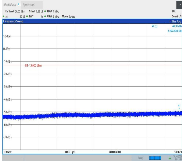
Band12-5MHz-QPSK-23155-1RB#24-1000~3000-PASS
