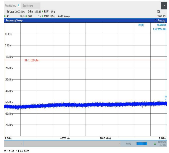
Band12-3MHz-QPSK-23095-1RB#0-1000~3000-PASS
