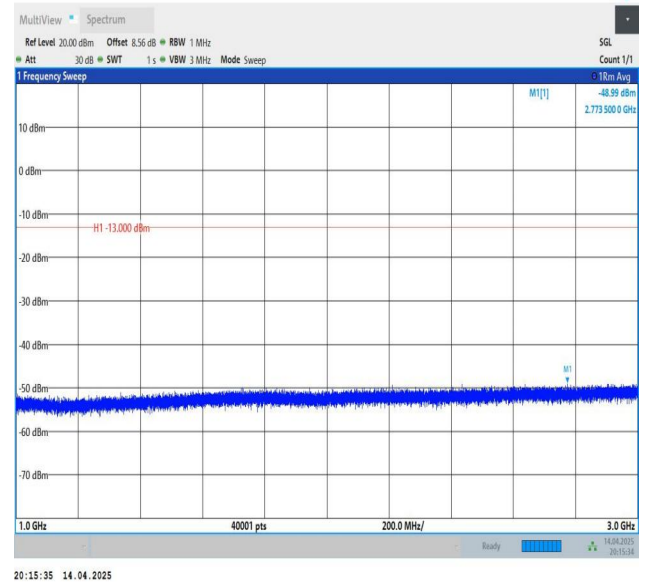
Band12-5MHz-QPSK-23035-1RB#0-1000~3000-PASS
