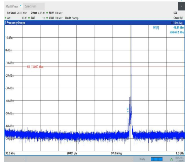
Band12-10MHz-QPSK-23095-1RB#49-30~1000-PASS
