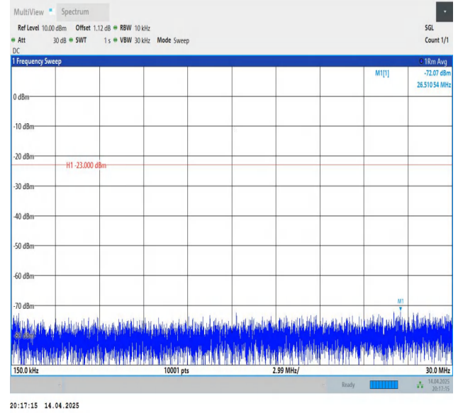
Band12-5MHz-QPSK-23155-1RB#0-0.15~30-PASS
