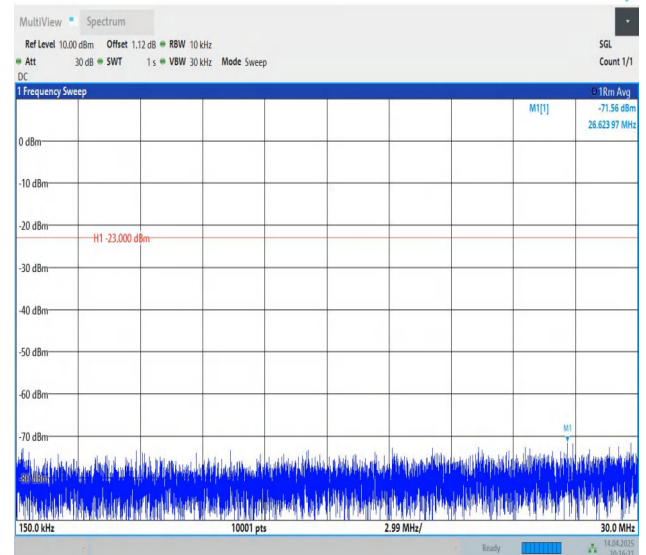
Band12-5MHz-QPSK-23095-1RB#0-0.15~30-PASS
