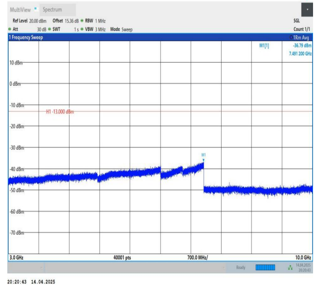
Band12-10MHz-QPSK-23130-1RB#49-3000~10000-PASS
