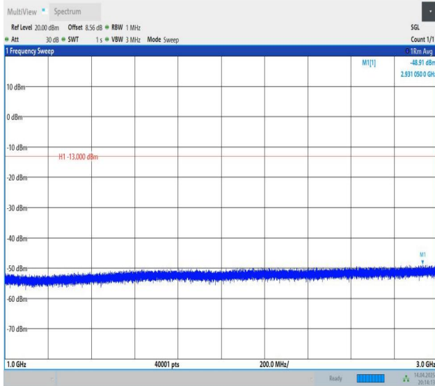
Band12-3MHz-QPSK-23095-1RB#14-1000~3000-PASS
