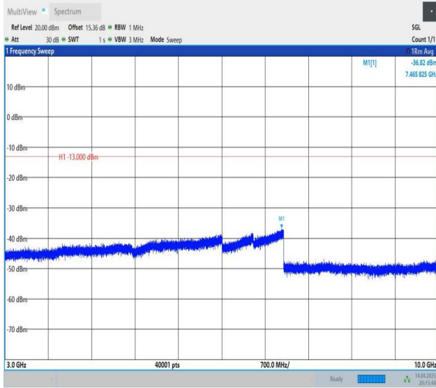
Band12-5MHz-QPSK-23035-1RB#0-3000~10000-PASS
