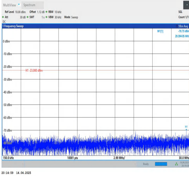
Band12-3MHz-QPSK-23165-1RB#14-0.15~30-PASS
