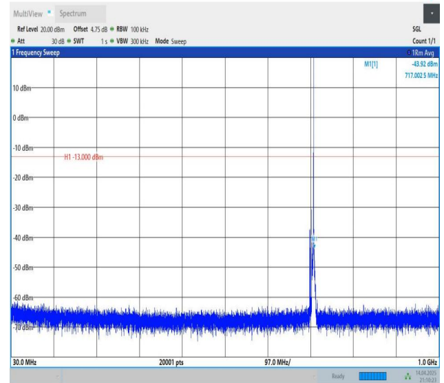
Band12-5MHz-QPSK-23155-1RB#24-30~1000-PASS
