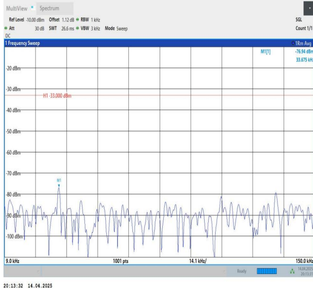
Band12-3MHz-QPSK-23095-1RB#0-0.009~0.15-PASS
