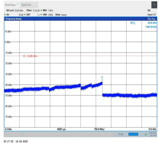
Band12-5MHz-QPSK-23095-1RB#24-3000~10000-PASS
