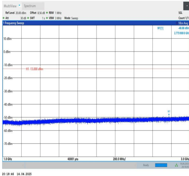
Band12-10MHz-QPSK-23060-1RB#49-1000~3000-PASS
