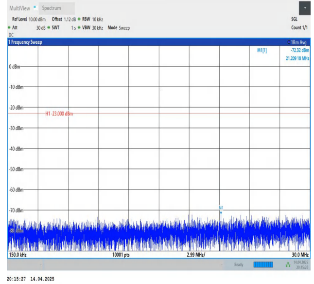
Band12-5MHz-QPSK-23035-1RB#0-0.15~30-PASS
