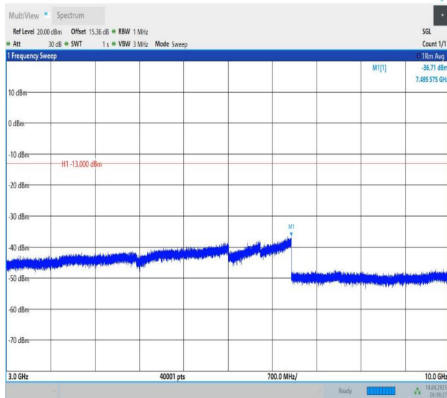
Band12-10MHz-QPSK-23060-1RB#0-3000~10000-PASS
