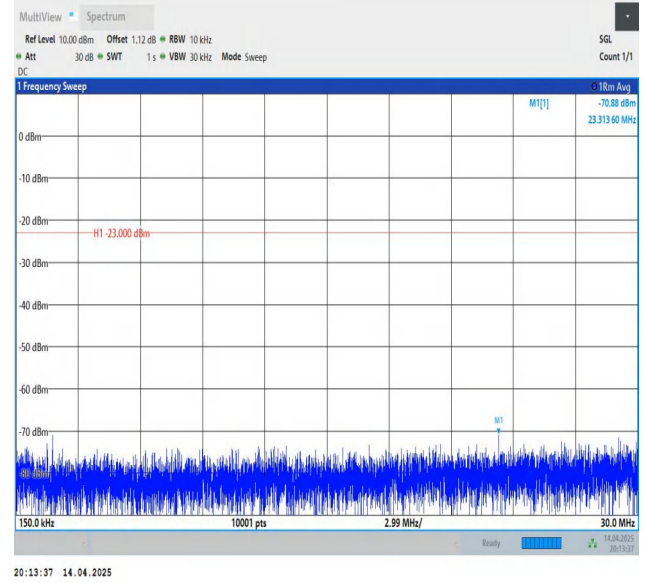
Band12-3MHz-QPSK-23095-1RB#0-0.15~30-PASS
