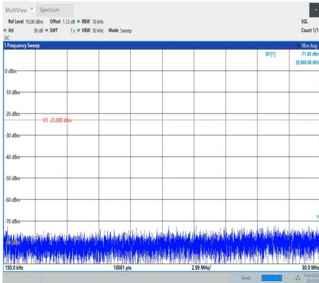
Band12-5MHz-QPSK-23035-1RB#24-0.15~30-PASS
