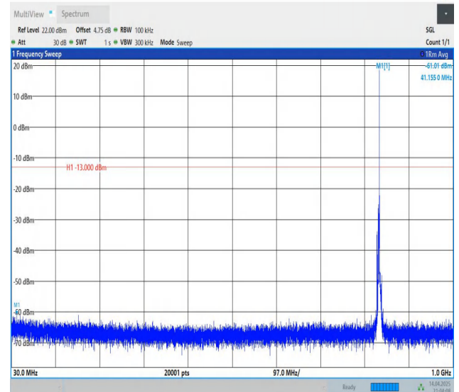
Band5-3MHz-QPSK-20525-1RB#14-30~1000-PASS
