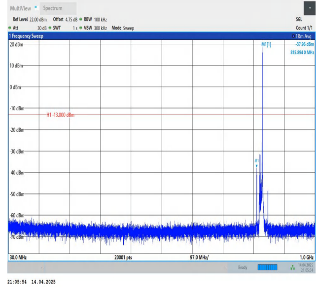
Band5-10MHz-QPSK-20450-1RB#49-30~1000-PASS
