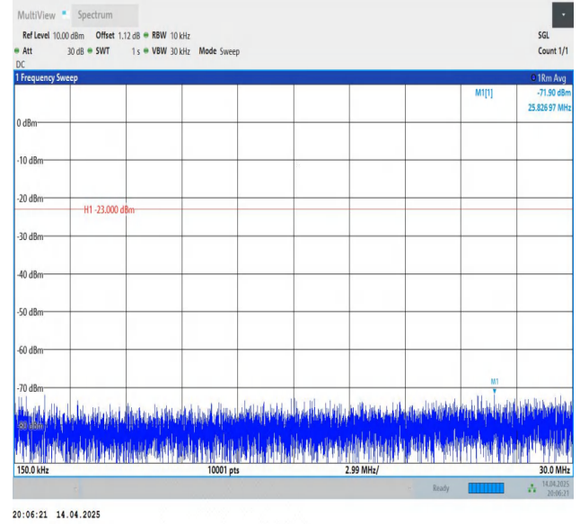
Band5-5MHz-QPSK-20625-1RB#0-0.15~30-PASS
