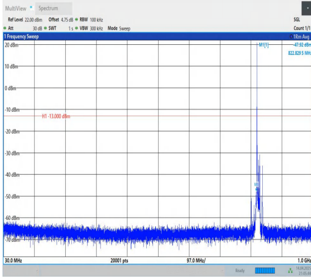
Band5-10MHz-QPSK-20450-1RB#0-30~1000-PASS
