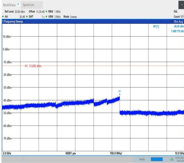
Band5-3MHz-QPSK-20525-1RB#0-3000~10000-PASS
