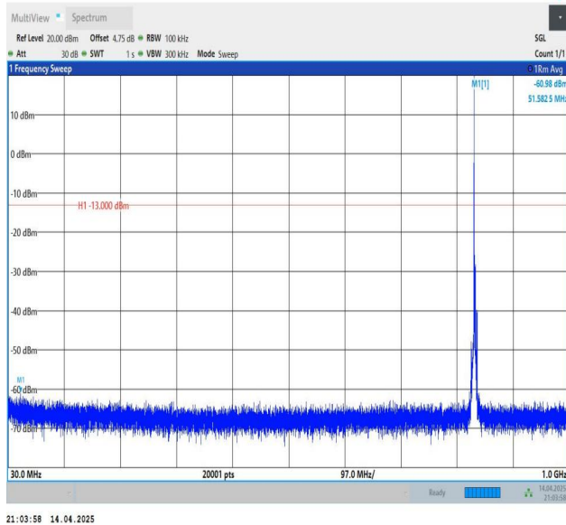
Band5-3MHz-QPSK-20525-1RB#0-30~1000-PASS
