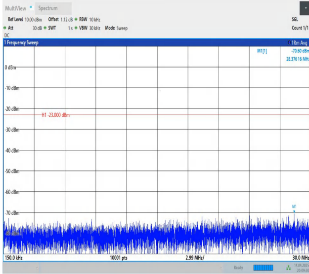
Band5-10MHz-QPSK-20600-1RB#49-0.15~30-PASS
