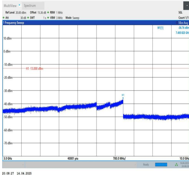
Band5-10MHz-QPSK-20525-1RB#0-3000~10000-PASS
