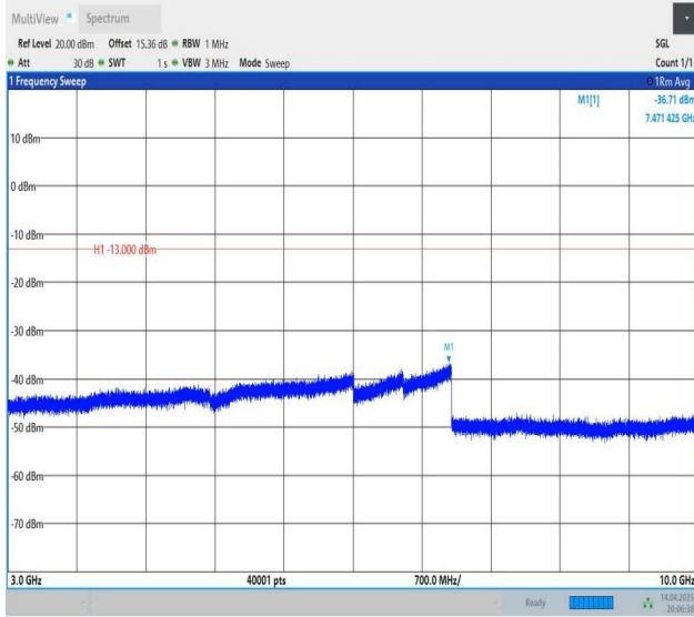
Band5-5MHz-QPSK-20625-1RB#0-3000~10000-PASS
