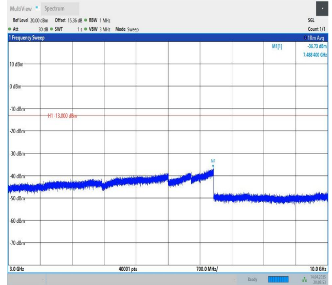
Band5-10MHz-QPSK-20525-1RB#49-3000~10000-PASS
