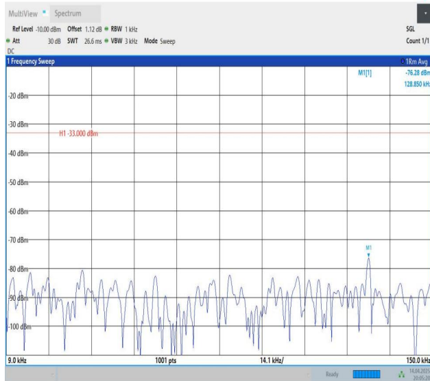
Band5-5MHz-QPSK-20525-1RB#0-0.009~0.15-PASS
