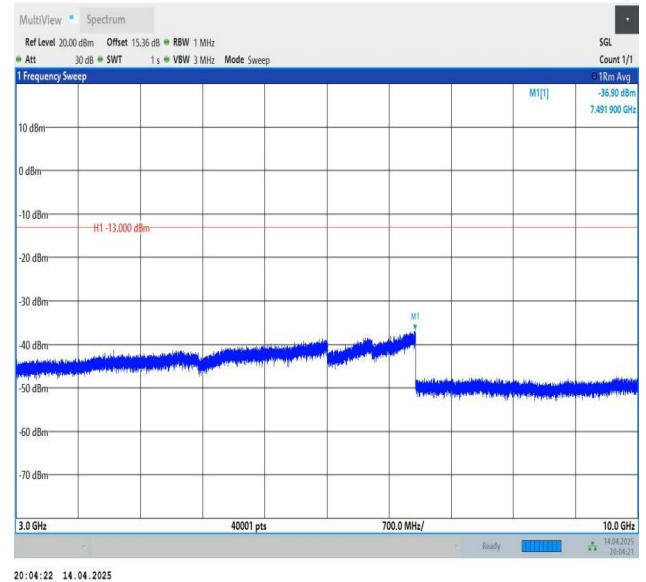
Band5-3MHz-QPSK-20635-1RB#14-3000~10000-PASS
