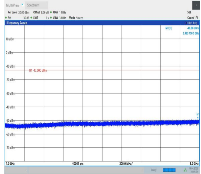
Band5-5MHz-QPSK-20525-1RB#0-1000~3000-PASS
