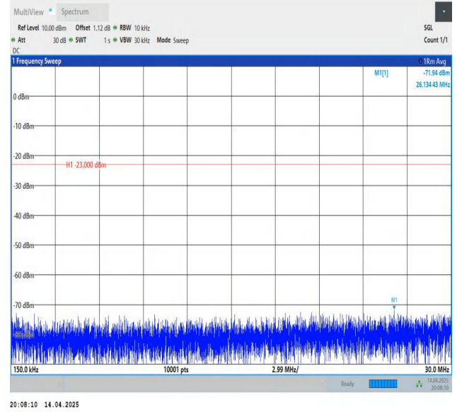
Band5-10MHz-QPSK-20525-1RB#0-0.15~30-PASS
