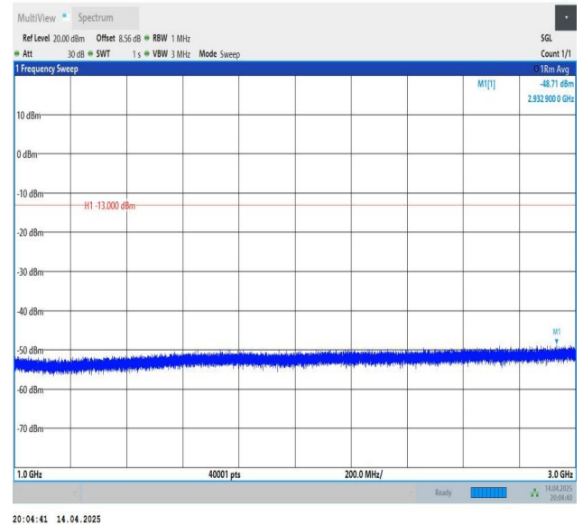
Band5-5MHz-QPSK-20425-1RB#0-1000~3000-PASS
