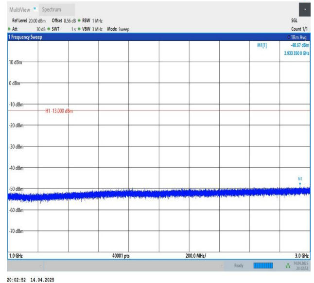
Band5-3MHz-QPSK-20525-1RB#0-1000~3000-PASS
