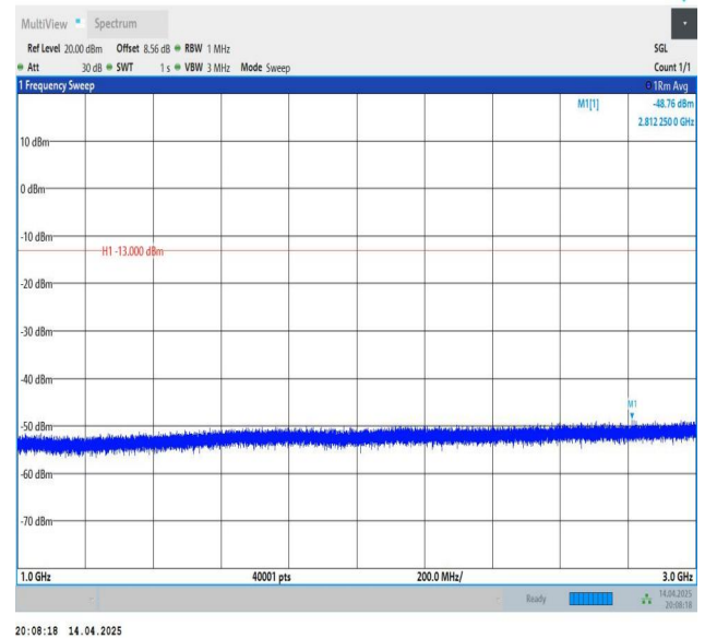
Band5-10MHz-QPSK-20525-1RB#0-1000~3000-PASS
