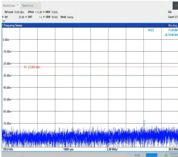
Band5-5MHz-QPSK-20425-1RB#24-0.15~30-PASS
