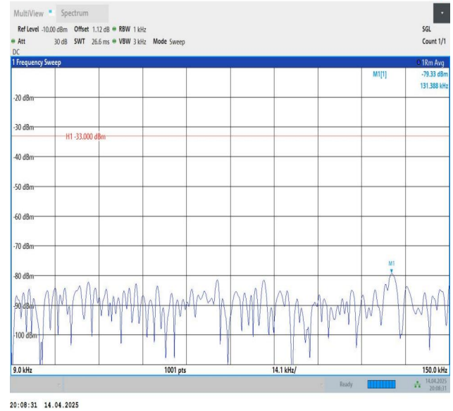
Band5-10MHz-QPSK-20525-1RB#49-0.009~0.15-PASS
