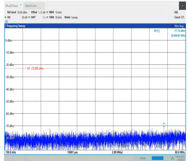
Band5-5MHz-QPSK-20525-1RB#0-0.15~30-PASS
