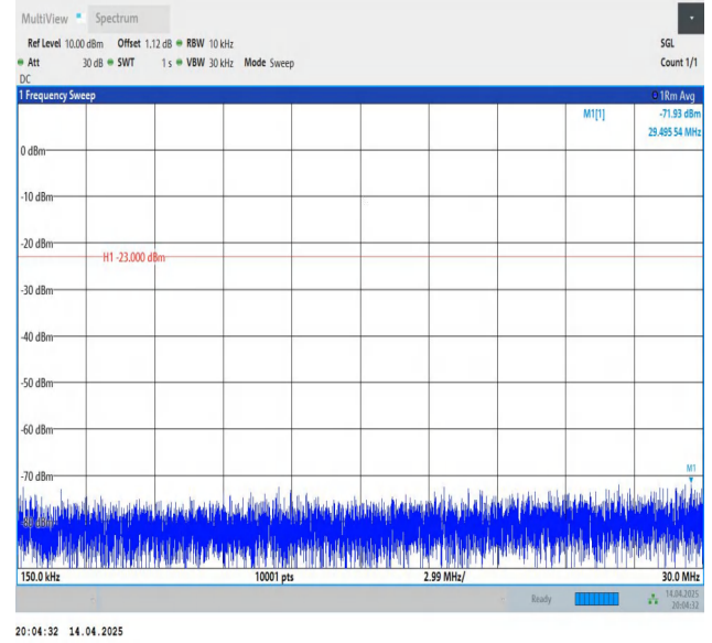
Band5-5MHz-QPSK-20425-1RB#0-0.15~30-PASS
