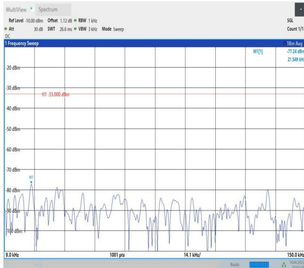
Band5-10MHz-QPSK-20450-1RB#0-0.009~0.15-PASS
