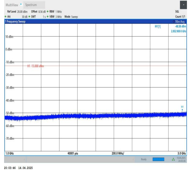
Band5-3MHz-QPSK-20635-1RB#0-1000~3000-PASS
