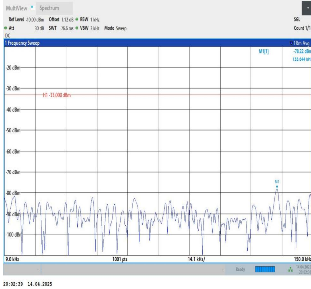
Band5-3MHz-QPSK-20525-1RB#0-0.009~0.15-PASS
