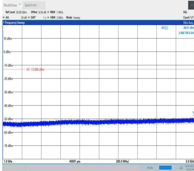
Band5-3MHz-QPSK-20525-1RB#14-1000~3000-PASS
