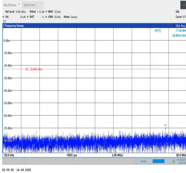
Band5-5MHz-QPSK-20525-1RB#24-0.15~30-PASS
