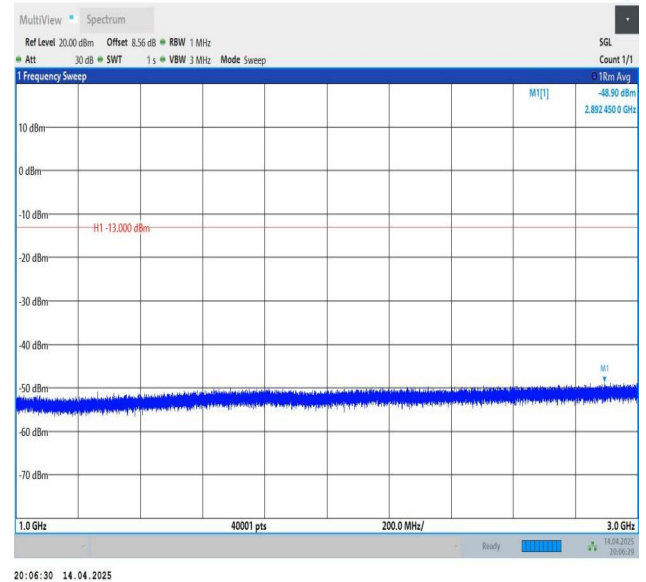
Band5-5MHz-QPSK-20625-1RB#0-1000~3000-PASS
