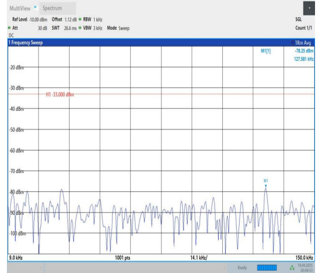
Band5-5MHz-QPSK-20425-1RB#24-0.009~0.15-PASS
