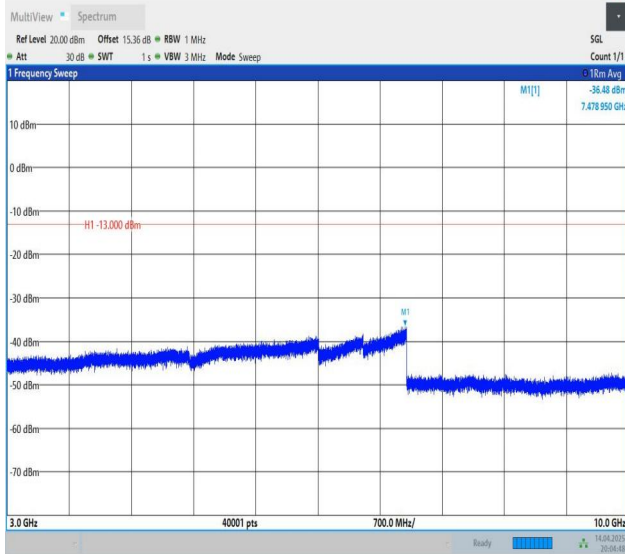
Band5-5MHz-QPSK-20425-1RB#0-3000~10000-PASS
