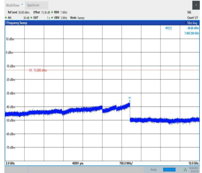
Band5-3MHz-QPSK-20525-1RB#14-3000~10000-PASS
