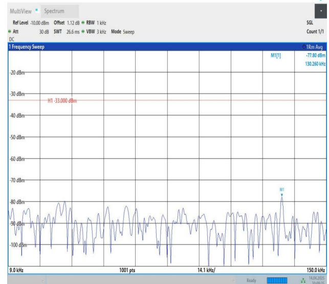
Band5-10MHz-QPSK-20600-1RB#49.0.009~0.15-PASS
