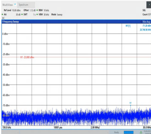
Band5-5MHz-QPSK-20625-1RB#24-0.15~30-PASS
