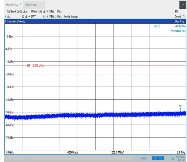
Band5-10MHz-QPSK-20450-1RB#0-1000~3000-PASS
