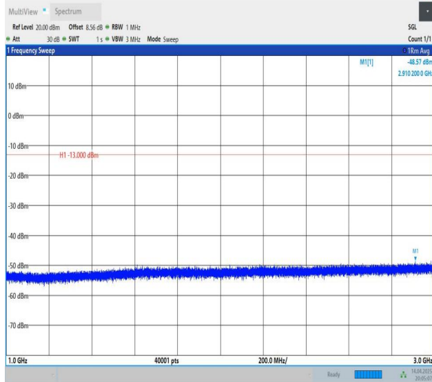
Band5-5MHz-QPSK-20425-1RB#24-1000~3000-PASS
