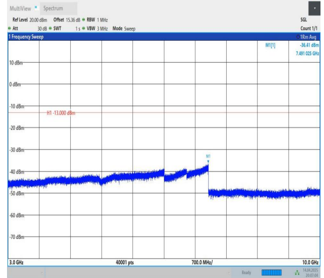
Band5-5MHz-QPSK-20625-1RB#24-3000~10000-PASS
