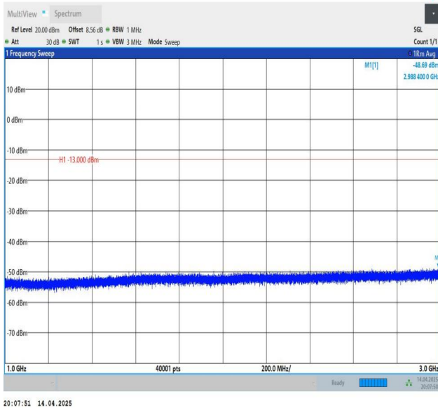
Band5-10MHz-QPSK-20450-1RB#49-1000~3000-PASS
