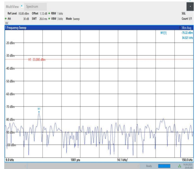
Band5-5MHz-QPSK-20525-1RB#24-0.009~0.15-PASS
