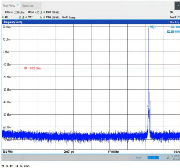
Band5-5MHz-QPSK-20425-1RB#0-30~1000-PASS
