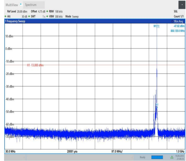
Band5-10MHz-QPSK-20600-1RB#49-30~1000-PASS
