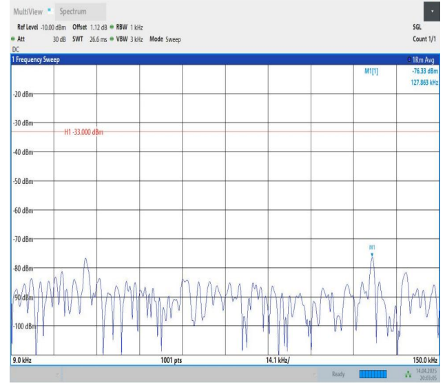
Band5-3MHz-QPSK-20525-1RB#14-0.009~0.15-PASS
