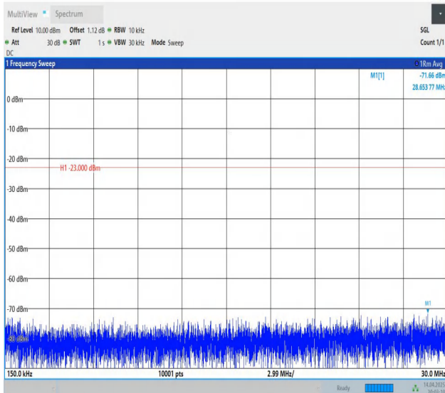
Band5-3MHz-QPSK-20525-1RB#14-0.15~30-PASS
