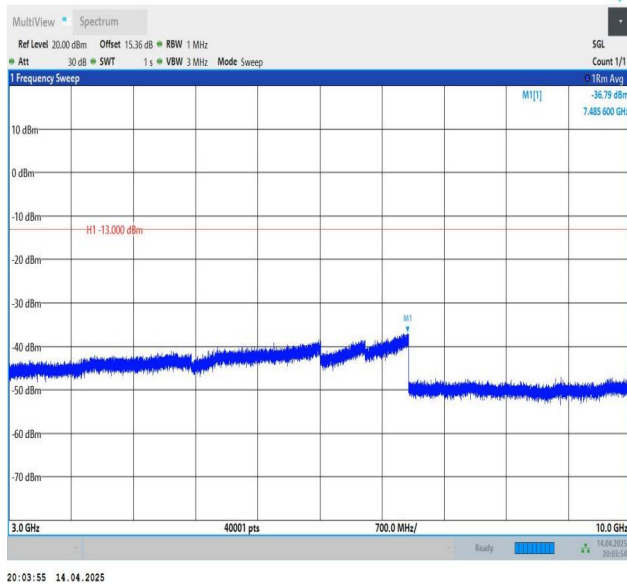
Band5-3MHz-QPSK-20635-1RB#0-3000~10000-PASS
