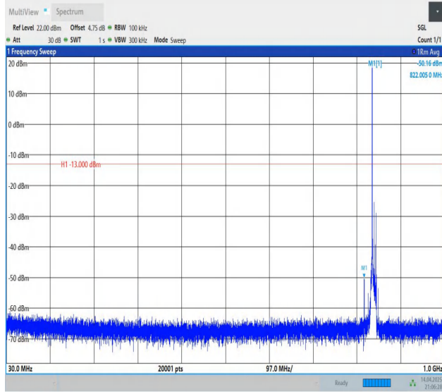
Band5-10MHz-QPSK-20600-1RB#0-30~1000-PASS
