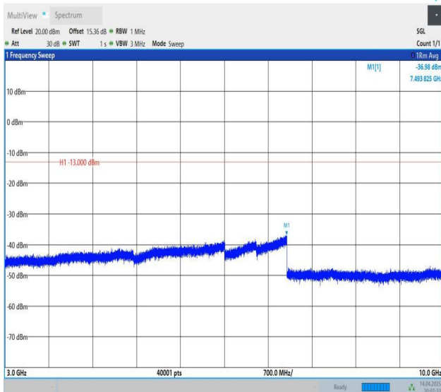
Band5-10MHz-QPSK-20450-1RB#0-3000~10000-PASS
