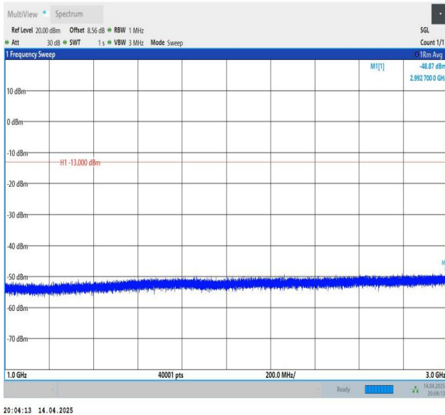
Band5-3MHz-QPSK-20635-1RB#14-1000~3000-PASS
