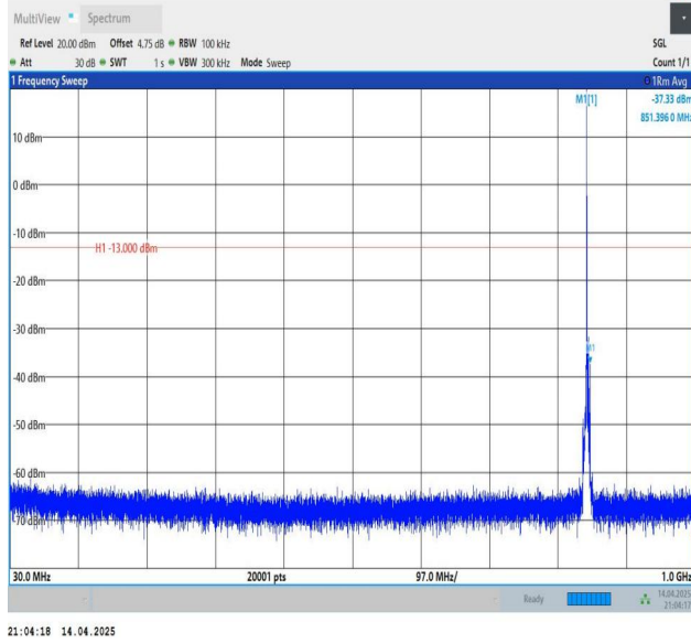
Band5-3MHz-QPSK-20635-1RB#0-30~1000-PASS
