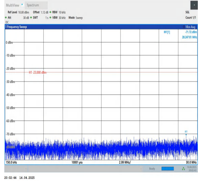
Band5-3MHz-QPSK-20525-1RB#0-0.15~30-PASS
