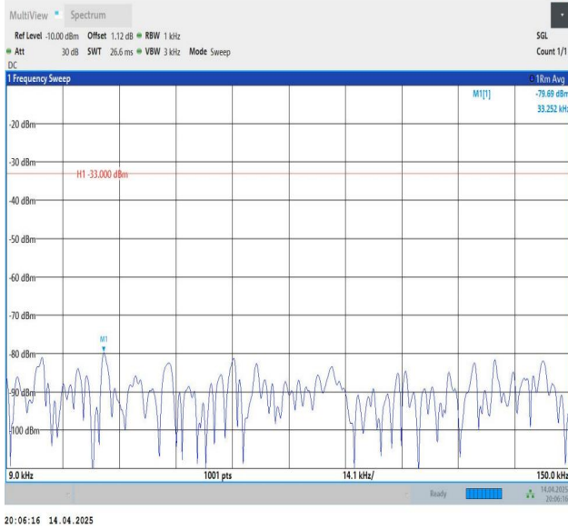
Band5-5MHz-QPSK-20625-1RB#0-0.009~0.15-PASS
