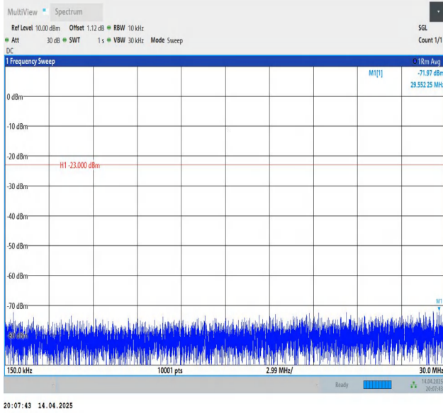
Band5-10MHz-QPSK-20450-1RB#49-0.15~30-PASS
