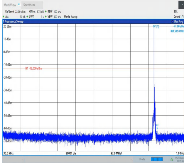
Band5-5MHz-QPSK-20525-1RB#0-30~1000-PASS
