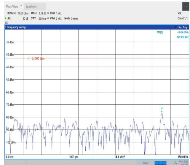
Band5-10MHz-QPSK-20450-1RB#49-0.009~0.15-PASS
