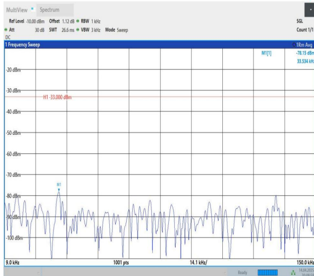
Band5-10MHz-QPSK-20600-1RB#0-0.009~0.15-PASS
