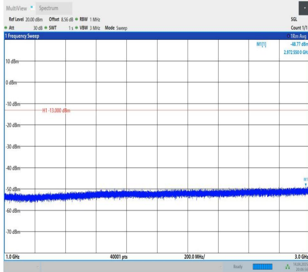
Band5-5MHz-QPSK-20625-1RB#24-1000~3000-PASS
