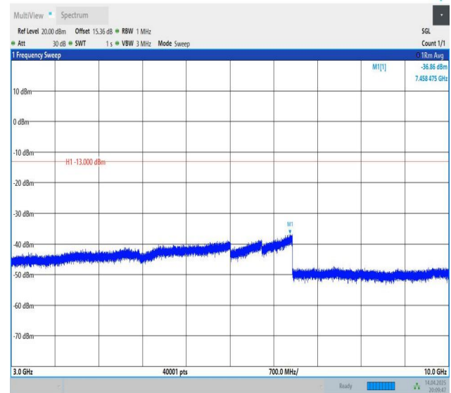
Band5-10MHz-QPSK-20600-1RB#49-3000~10000-PASS
