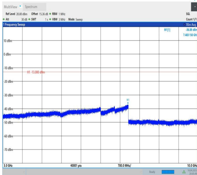
Band5-5MHz-QPSK-20525-1RB#0-3000~10000-PASS
