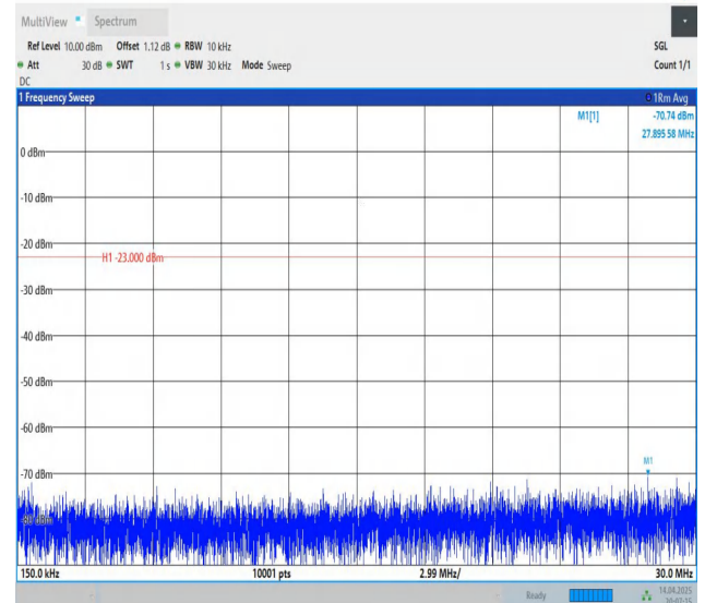
Band5-10MHz-QPSK-20450-1RB#0-0.15~30-PASS
