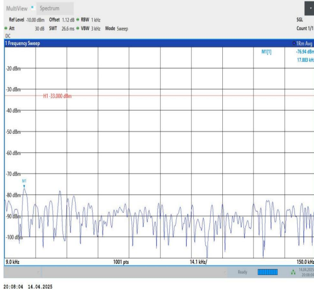
Band5-10MHz-QPSK-20525-1RB#0-0.009~0.15-PASS
