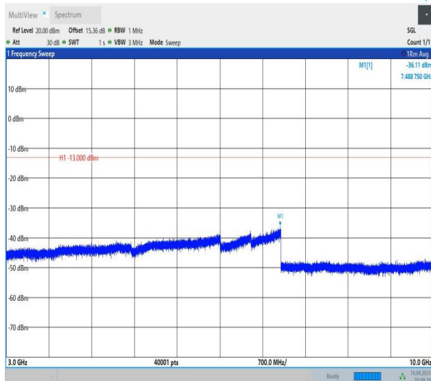
Band5-10MHz-QPSK-20600-1RB#0-3000~10000-PASS
