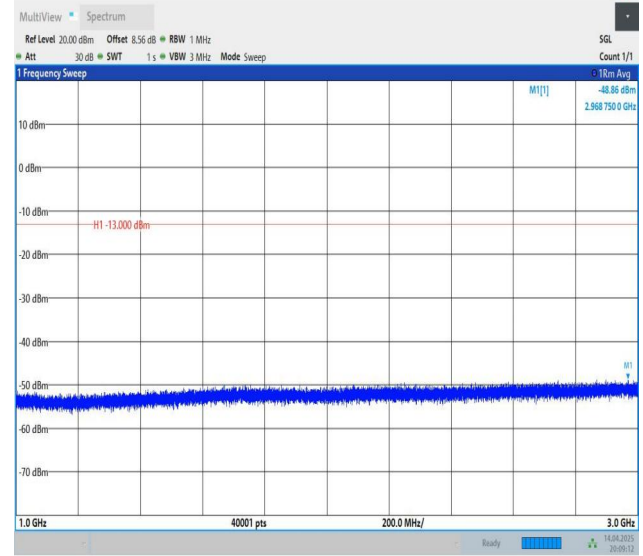
Band5-10MHz-QPSK-20600-1RB#0-1000~3000-PASS
