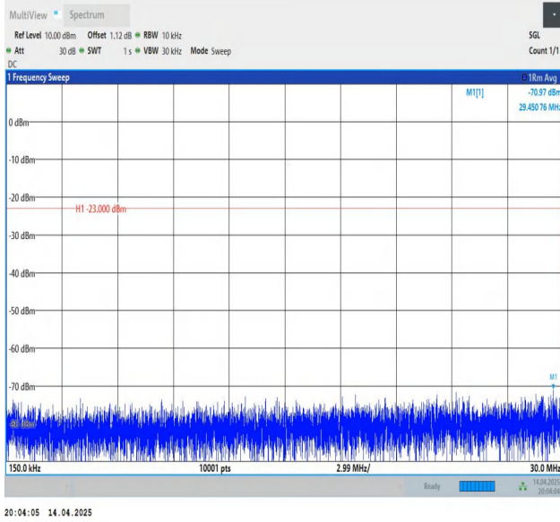
Band5-3MHz-QPSK-20635-1RB#14-0.15~30-PASS
