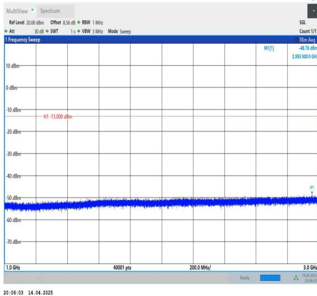
Band5-5MHz-QPSK-20525-1RB#24-1000~3000-PASS
