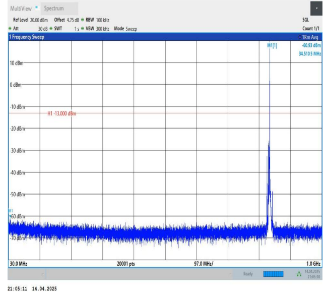
Band5-5MHz-QPSK-20525-1RB#24-30~1000-PASS
