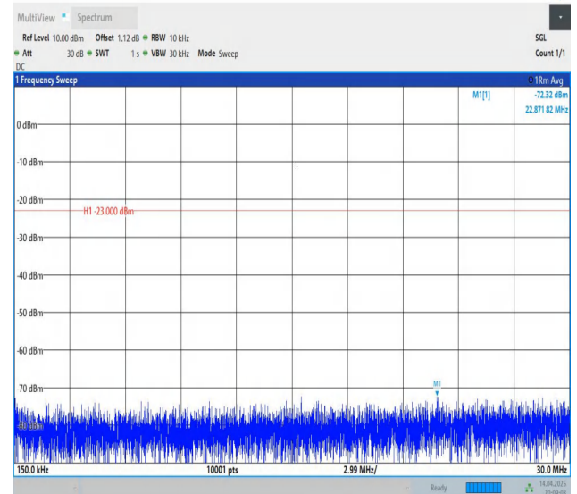
Band5-10MHz-QPSK-20600-1RB#0-0.15~30-PASS
