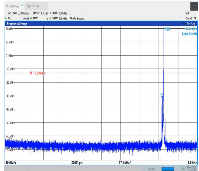
Band5-5MHz-QPSK-20425-1RB#24-30~1000-PASS
