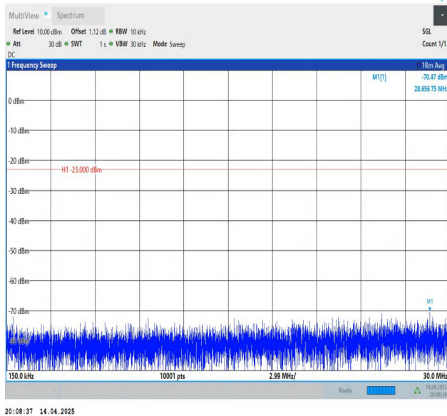
Band5-10MHz-QPSK-20525-1RB#49-0.15~30-PASS
