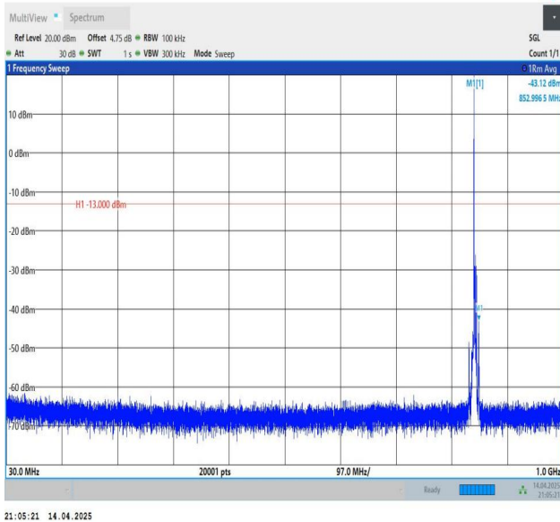
Band5-5MHz-QPSK-20625-1RB#0-30~1000-PASS
