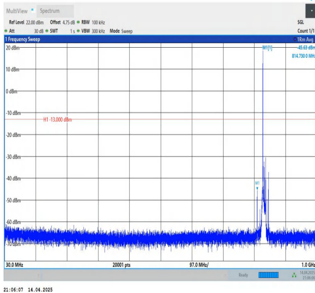
Band5-10MHz-QPSK-20525-1RB#0-30~1000-PASS
