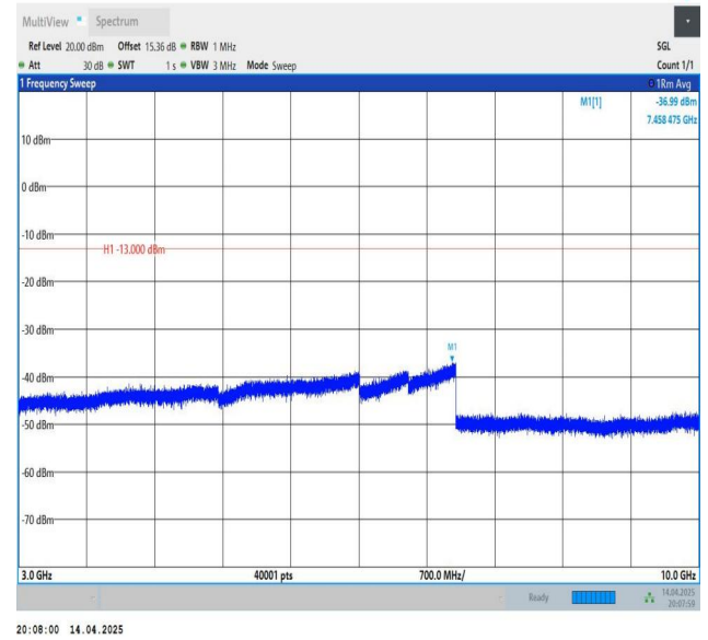
Band5-10MHz-QPSK-20450-1RB#49-3000~10000-PASS
