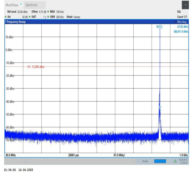
Band5-3MHz-QPSK-20635-1RB#14-30~1000-PASS
