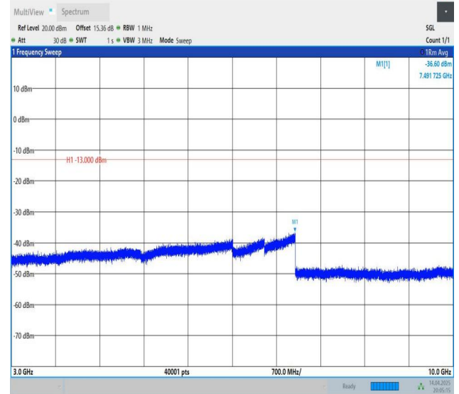
Band5-5MHz-QPSK-20425-1RB#24-3000~10000-PASS
