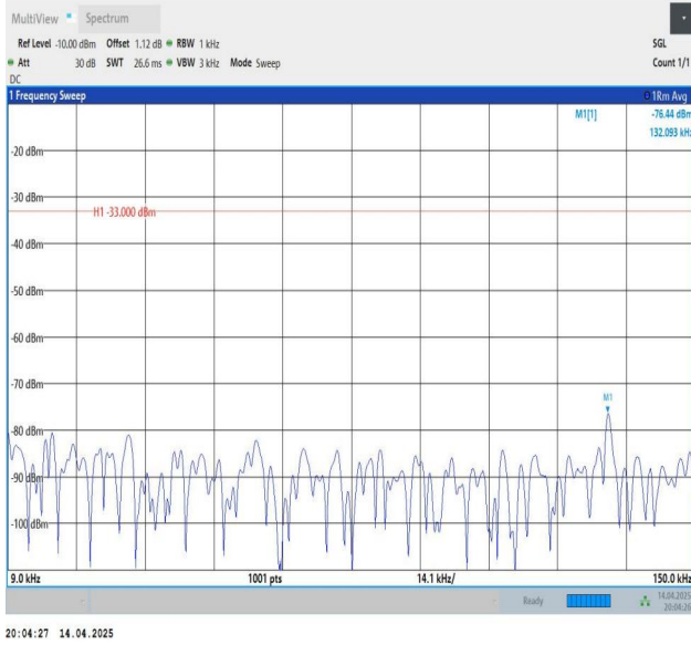
Band5-5MHz-QPSK-20425-1RB#0-0.009~0.15-PASS
