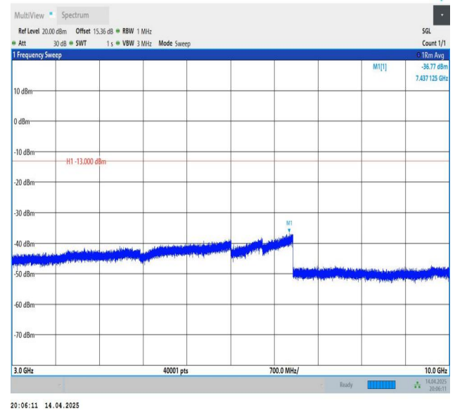
Band5-5MHz-QPSK-20525-1RB#24-3000~10000-PASS
