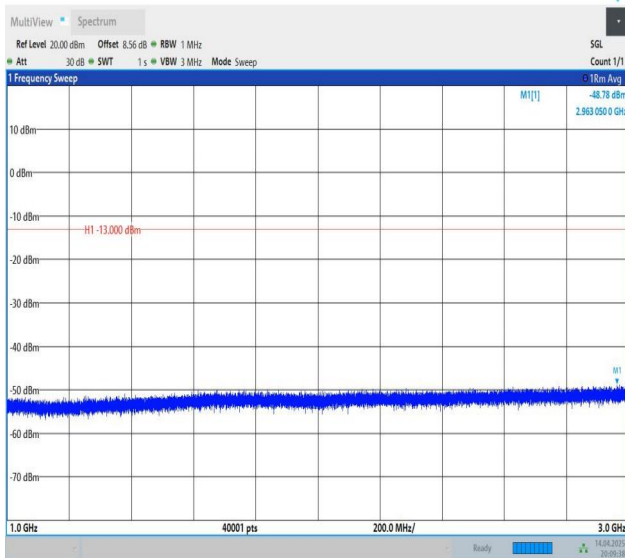
Band5-10MHz-QPSK-20600-1RB#49-1000~3000-PASS
