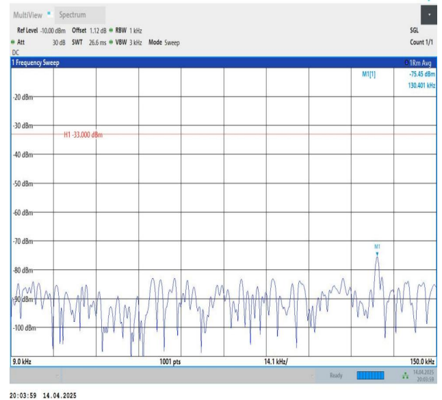
Band5-3MHz-QPSK-20635-1RB#14-0.009~0.15-PASS
