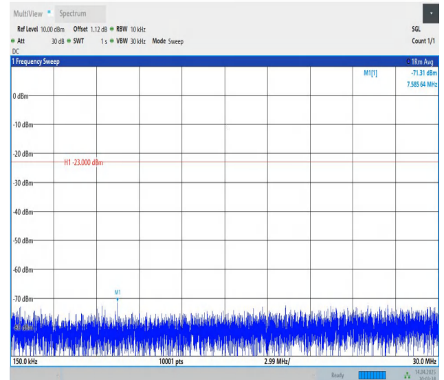
Band5-3MHz-QPSK-20635-1RB#0-0.15~30-PASS
