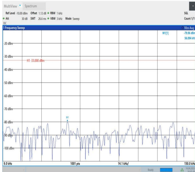
Band5-3MHz-QPSK-20415-1RB#0-0.009~0.15-PASS
