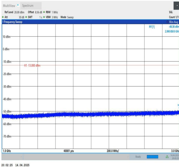
Band5-3MHz-QPSK-20415-1RB#14-1000~3000-PASS
