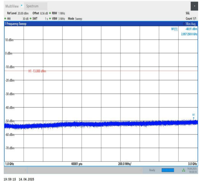
Band5-1.4MHz-QPSK-20407-1RB#0-1000~3000-PASS
