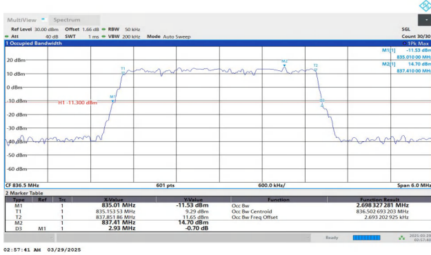
Band5-3MHz-QPSK-20525-15RB#0-PASS
