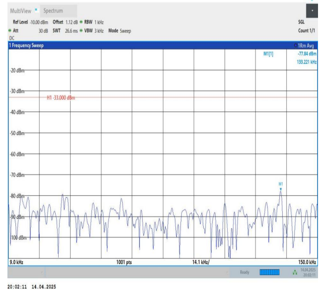
Band5-3MHz-QPSK-20415-1RB#14-0.009~0.15-PASS
