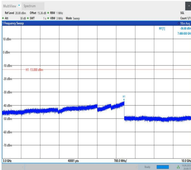
Band5-1.4MHz-QPSK-20525-1RB#0-3000~10000-PASS
