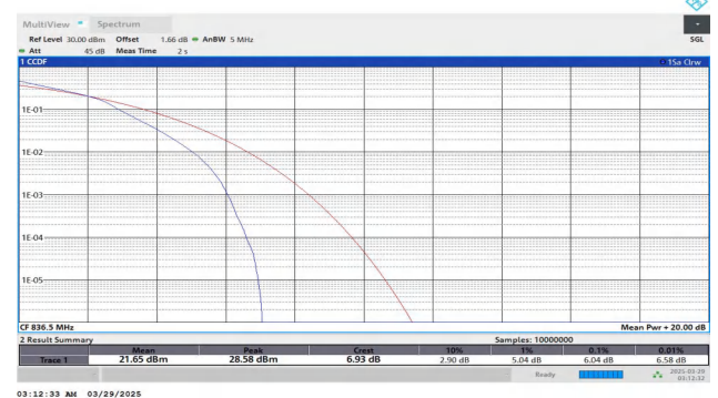
Band5-5MHz-16QAM-20525-25RB#0-PASS
