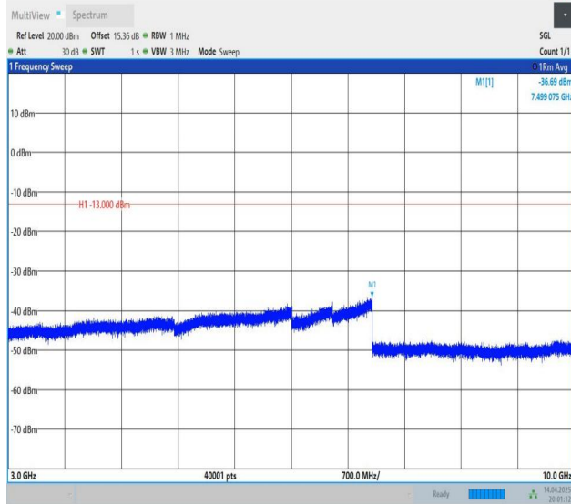
Band5-1.4MHz-QPSK-20643-1RB#0-3000~10000-PASS
