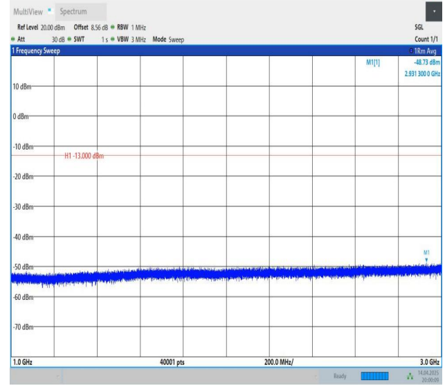
Band5-1.4MHz-QPSK-20525-1RB#0-1000~3000-PASS
