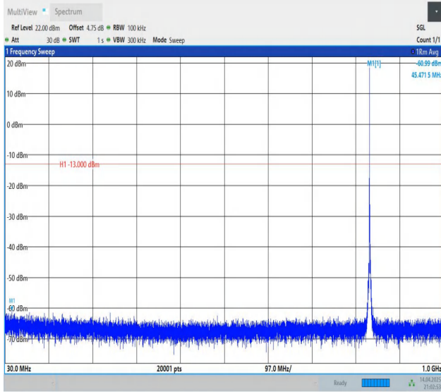
Band5-1.4MHz-QPSK-20525-1RB#0-30~1000-PASS
