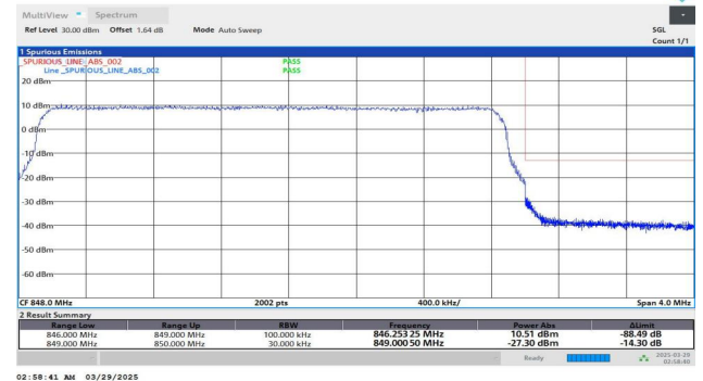
Band5-3MHz-QPSK-20635-15RB#0-PASS
