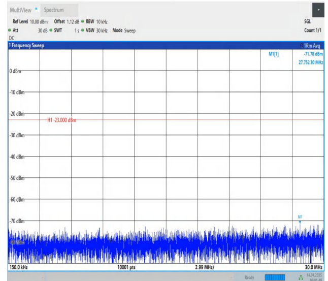
Band5-3MHz-QPSK-20415-1RB#0-0.15~30-PASS
