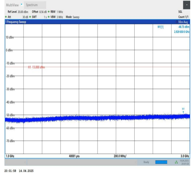
Band5-3MHz-QPSK-20415-1RB#0-1000~3000-PASS
