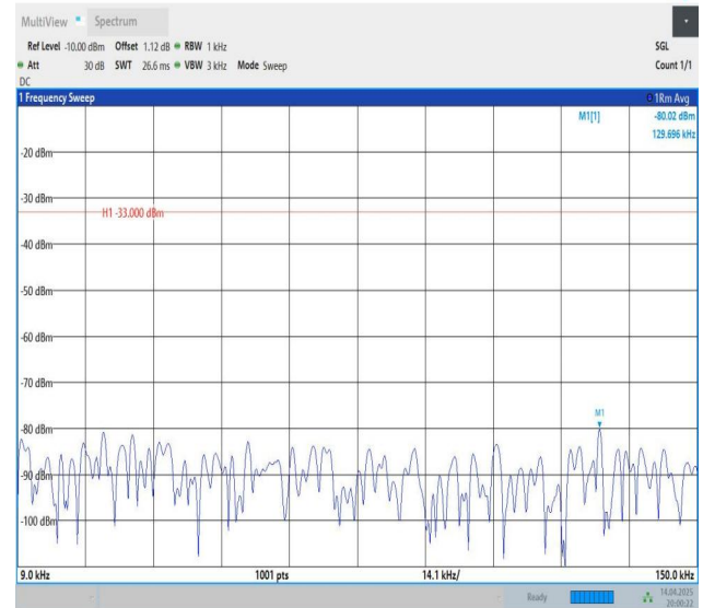
Band5-1.4MHz-QPSK-20525-1RB#5-0.009~0.15-PASS
