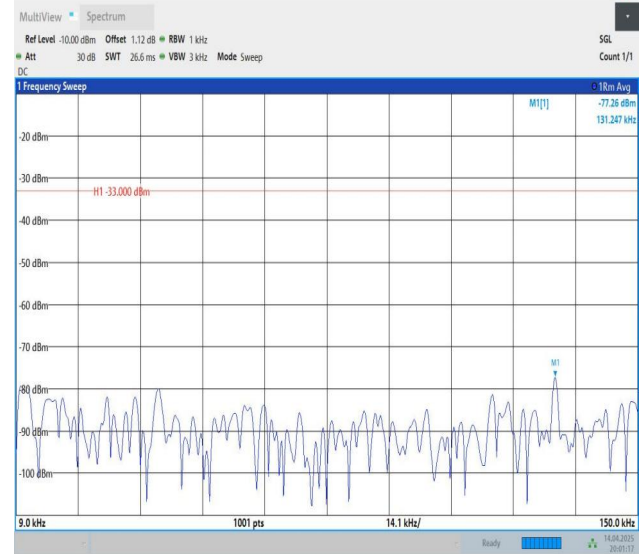
Band5-1.4MHz-QPSK-20643-1RB#5-0.009~0.15-PASS
