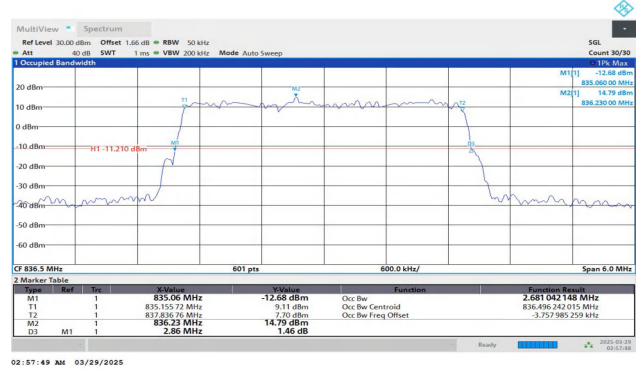
Band5-3MHz-16QAM-20525-15RB#0-PASS
