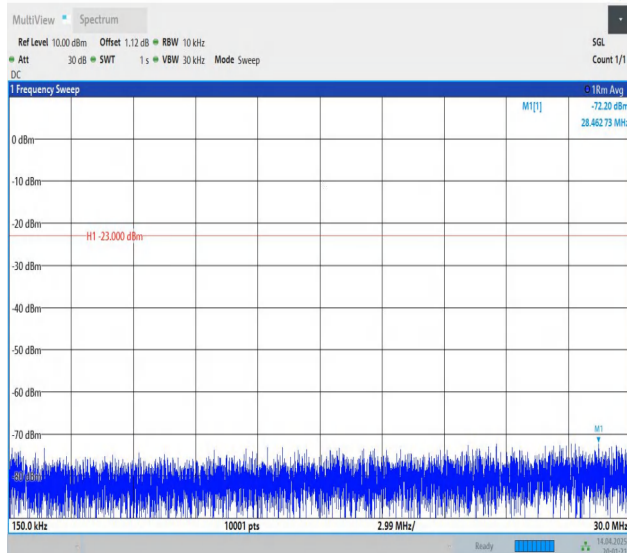
Band5-1.4MHz-QPSK-20643-1RB#5-0.15~30-PASS
