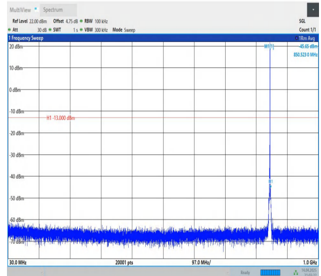
Band5-1.4MHz-QPSK-20643-1RB#5-30~1000-PASS
