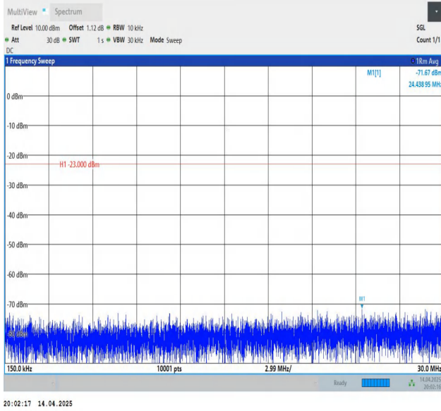
Band5-3MHz-QPSK-20415-1RB#14-0.15~30-PASS
