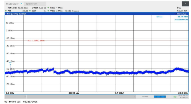
Band4-20MHz-QPSK-20175-1RB#99-3000~20000-PASS
