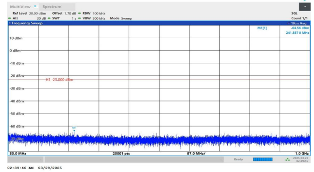
Band4-20MHz-QPSK-20175-1RB#99-30~1000-PASS
