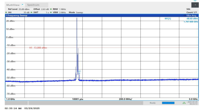
Band4-15MHz-QPSK-20325-1RB#0-1000~3000-PASS
