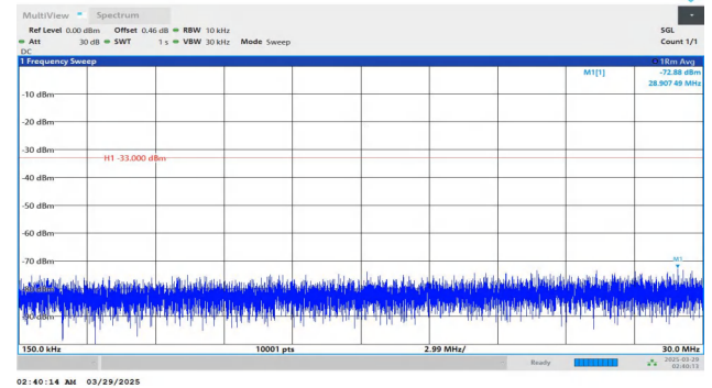
Band4-20MHz-QPSK-20300-1RB#0-0.15~30-PASS
