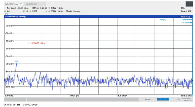
Band4-10MHz-QPSK-20175-1RB#49-0.009~0.15-PASS
