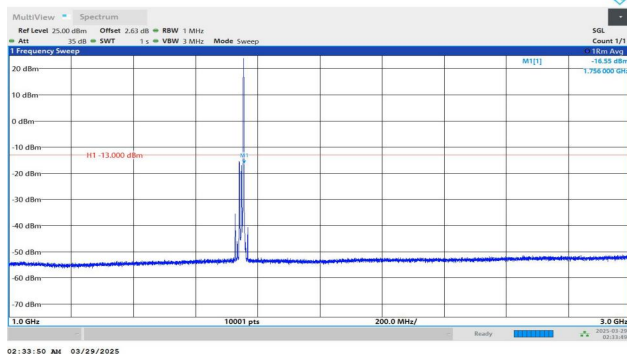
Band4-15MHz-QPSK-20325-1RB#74-1000~3000-PASS
