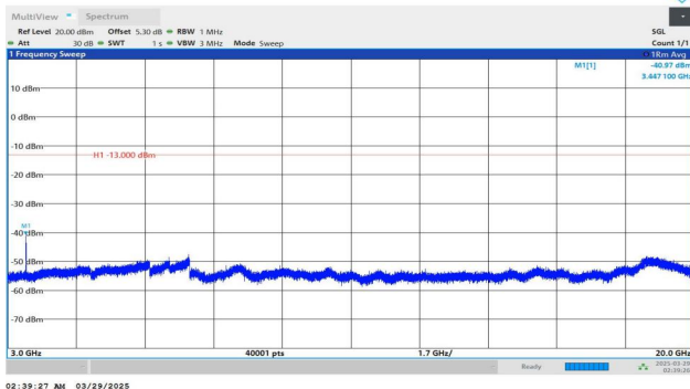
Band4-20MHz-QPSK-20175-1RB#0-3000~20000-PASS
