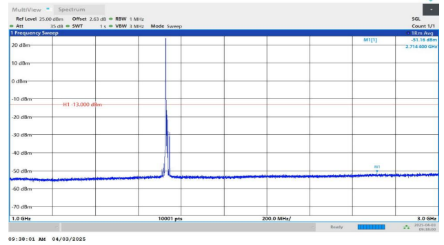
Band4-10MHz-QPSK-20175-1RB#0-1000~3000-PASS
