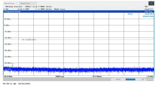
Band4-10MHz-QPSK-20175-1RB#49-30~1000-PASS
