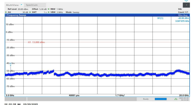
Band4-15MHz-QPSK-20325-1RB#74-3000~20000-PASS
