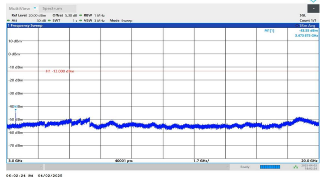
Band4-10MHz-QPSK-20175-1RB#49-3000~20000-PASS
