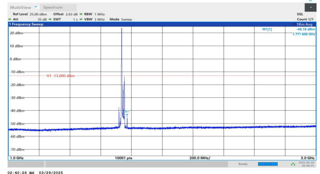
Band4-20MHz-QPSK-20300-1RB#0-1000~3000-PASS
