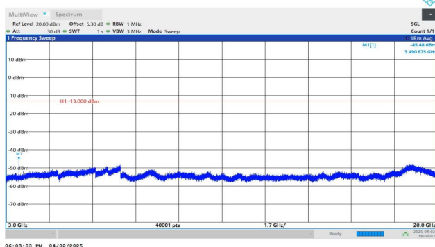
Band4-10MHz-QPSK-20350-1RB#0-3000~20000-PASS
