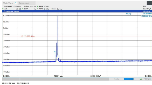
Band4-20MHz-QPSK-20175-1RB#99-1000~3000-PASS
