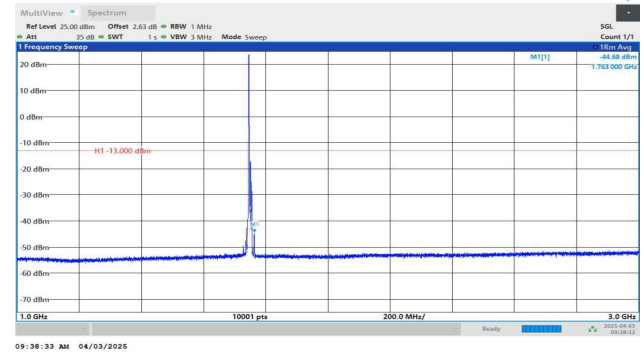
Band4-10MHz-QPSK-20350-1RB#0-1000~3000-PASS
