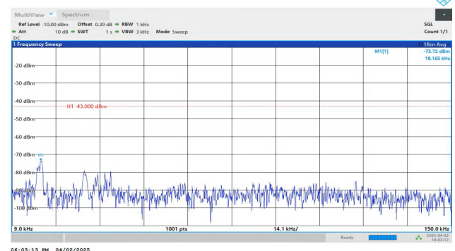
Band4-10MHz-QPSK-20350-1RB#49-0.009~0.15-PASS
