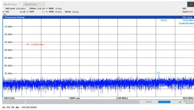
Band4-20MHz-QPSK-20175-1RB#99-0.15~30-PASS
