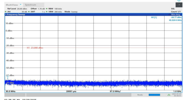
Band4-20MHz-QPSK-20050-1RB#99-30~1000-PASS
