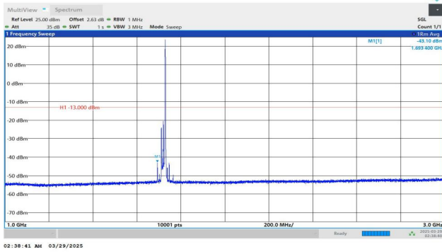
Band4-20MHz-QPSK-20050-1RB#99-1000~3000-PASS
