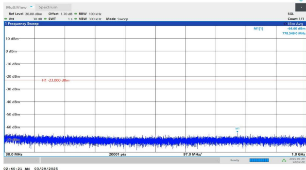
Band4-20MHz-QPSK-20300-1RB#0-30~1000-PASS
