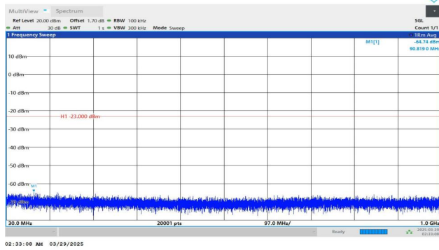
Band4-15MHz-QPSK-20325-1RB#0-30~1000-PASS
