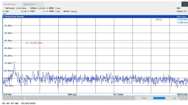
Band4-20MHz-QPSK-20300-1RB#0-0.009~0.15-PASS
