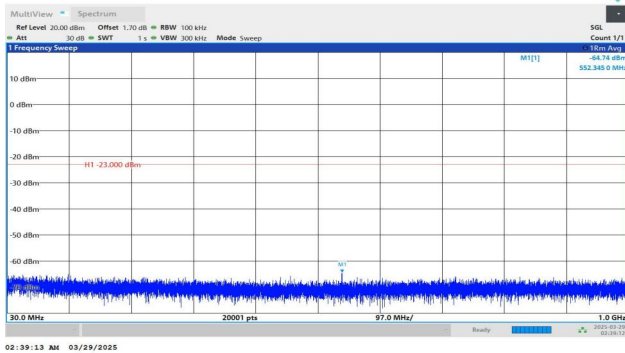
Band4-20MHz-QPSK-20175-1RB#0-30~1000-PASS
