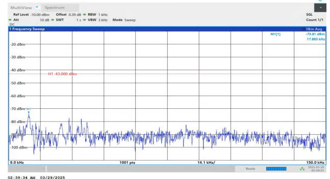
Band4-20MHz-QPSK-20175-1RB#99-0.009~0.15-PASS
