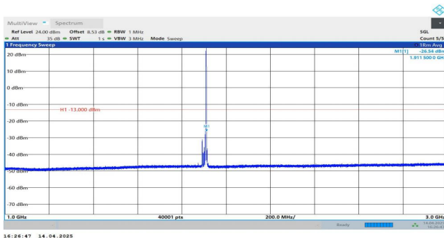
Band2-10MHz-QPSK-19150-1RB#49-1000~3000-PASS
