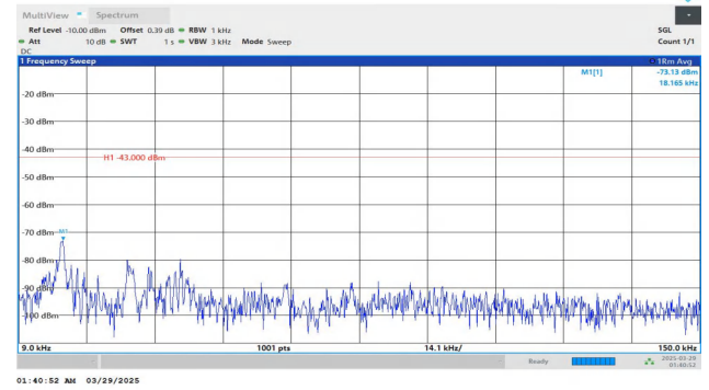
Band2-15MHz-QPSK-19125-1RB#74-0.009~0.15-PASS
