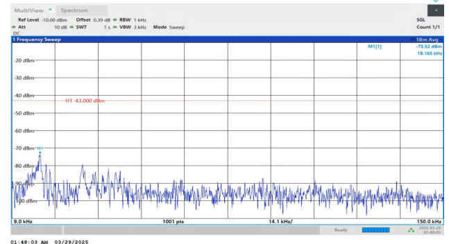
Band2-20MHz-QPSK-19100-1RB#99-0.009~0.15-PASS
