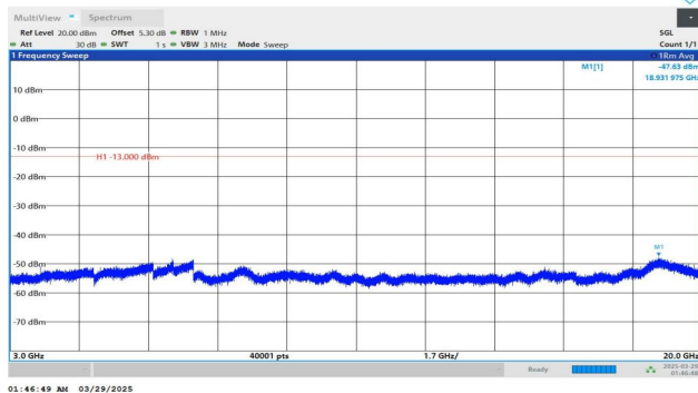
Band2-20MHz-QPSK-18900-1RB#0-3000~20000-PASS
