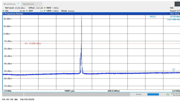
Band2-10MHz-QPSK-18900-1RB#49-1000~3000-PASS
