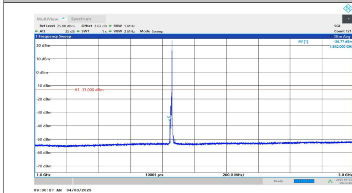
Band2-10MHz-QPSK-18650-1RB#49-1000~3000-PASS
