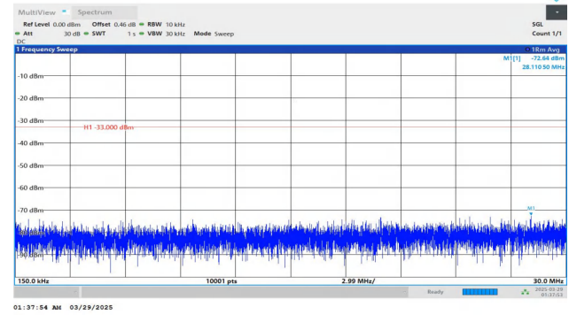
Band2-15MHz-QPSK-18675-1RB#0-0.15~30-PASS
