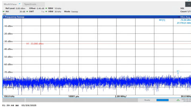
Band2-15MHz-QPSK-18900-1RB#74-0.15~30-PASS
