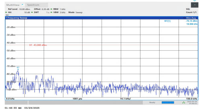
Band2-20MHz-QPSK-18900-1RB#99-0.009~0.15-PASS
