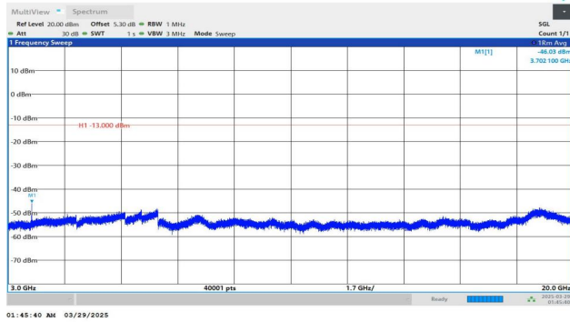
Band2-20MHz-QPSK-18700-1RB#0-3000~20000-PASS
