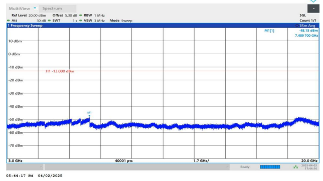
Band2-5MHz-QPSK-19175-1RB#24-3000~20000-PASS
