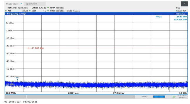
Band2-10MHz-QPSK-18900-1RB#49-30~1000-PASS
