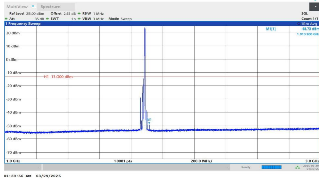
Band2-15MHz-QPSK-18900-1RB#74-1000~3000-PASS
