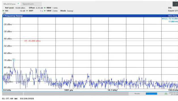
Band2-15MHz-QPSK-18675-1RB#0-0.009~0.15-PASS
