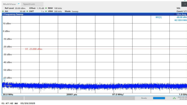
Band2-20MHz-QPSK-19100-1RB#0-30~1000-PASS
