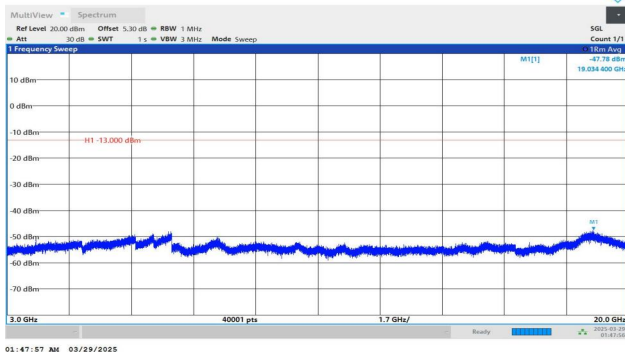
Band2-20MHz-QPSK-19100-1RB#0-3000~20000-PASS
