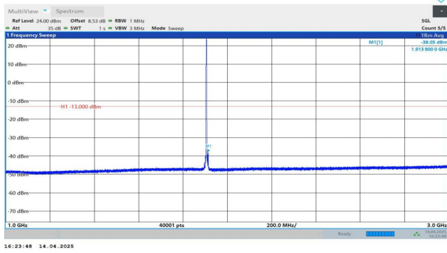
Band2-5MHz-QPSK-19175-1RB#24-1000~3000-PASS
