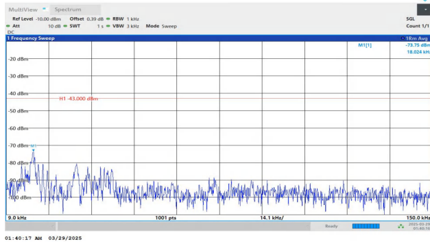
Band2-15MHz-QPSK-19125-1RB#0-0.009~0.15-PASS
