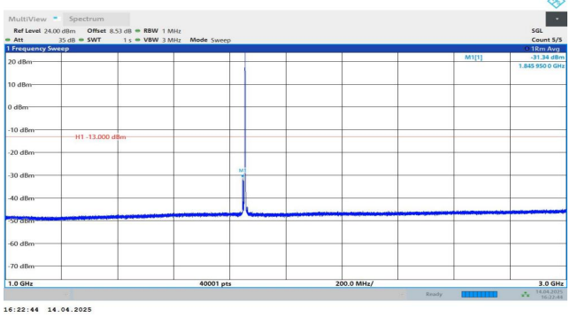
Band2-10MHz-QPSK-18650-1RB#0-1000~3000-PASS
