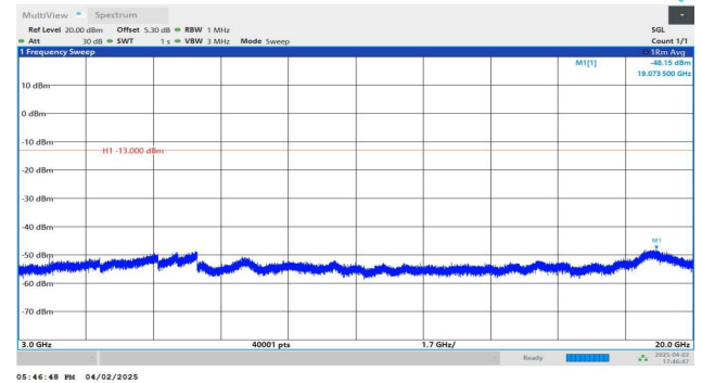
Band2-10MHz-QPSK-18900-1RB#49-3000~20000-PASS
