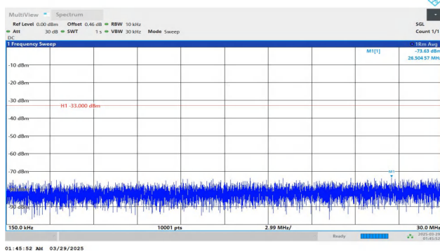
Band2-20MHz-QPSK-18700-1RB#99-0.15~30-PASS
