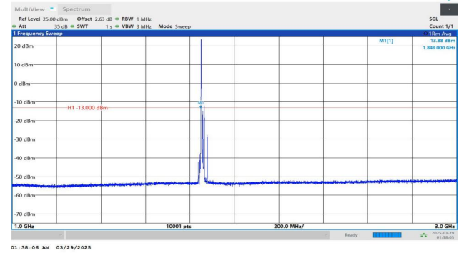
Band2-15MHz-QPSK-18675-1RB#0-1000~3000-PASS
