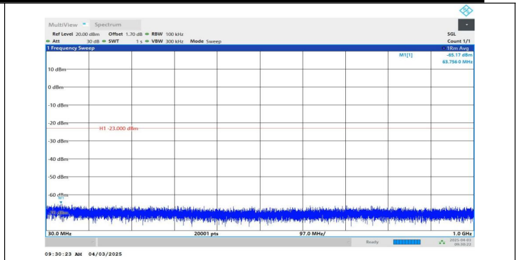
Band2-10MHz-QPSK-18650-1RB#49-30~1000-PASS
