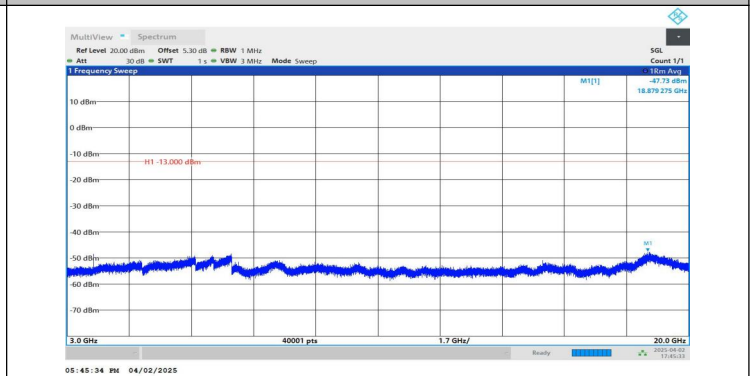
Band2-10MHz-QPSK-18650-1RB#49-3000~20000-PASS
