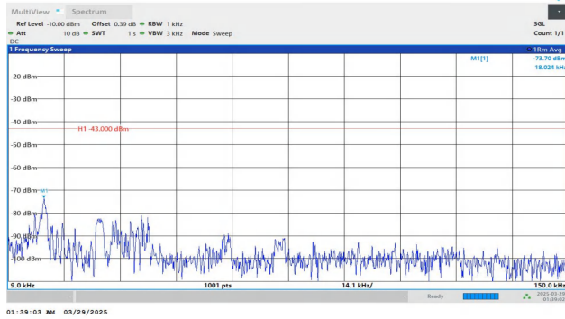
Band2-15MHz-QPSK-18900-1RB#0-0.009~0.15-PASS
