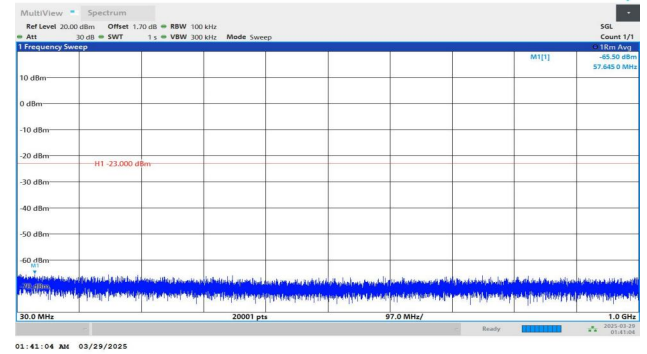
Band2-15MHz-QPSK-19125-1RB#74-30~1000-PASS
