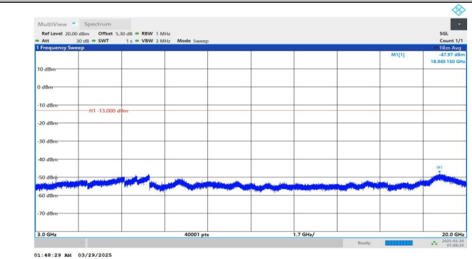
Band2-20MHz-QPSK-19100-1RB#99-3000~20000-PASS
