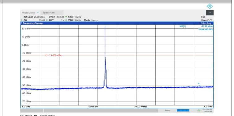
Band2-10MHz-QPSK-18900-1RB#0-1000~3000-PASS
