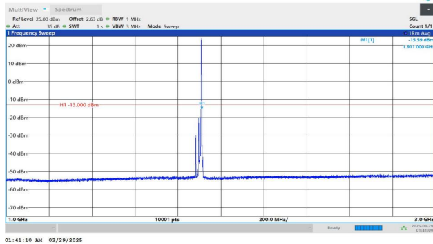
Band2-15MHz-QPSK-19125-1RB#74-1000~3000-PASS
