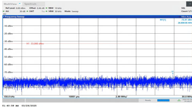
Band2-15MHz-QPSK-19125-1RB#74-0.15~30-PASS
