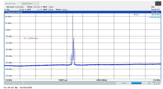
Band2-15MHz-QPSK-18900-1RB#0-1000~3000-PASS
