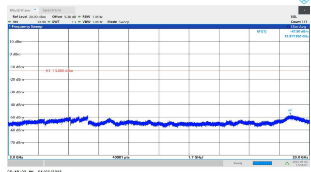
Band2-10MHz-QPSK-19150-1RB#49-3000~20000-PASS
