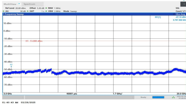
Band2-15MHz-QPSK-19125-1RB#0-3000~20000-PASS
