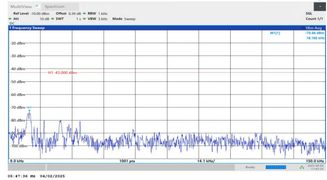
Band2-10MHz-QPSK-19150-1RB#49-0.009~0.15-PASS
