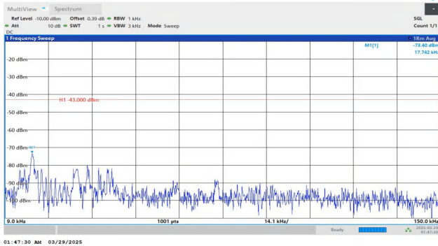
Band2-20MHz-QPSK-19100-1RB#0-0.009~0.15-PASS
