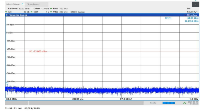
Band2-15MHz-QPSK-18900-1RB#74-30~1000-PASS
