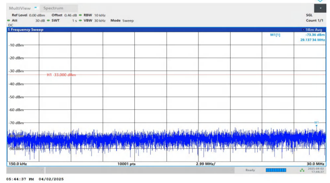
Band2-10MHz-QPSK-18650-1RB#0-0.15~30-PASS
