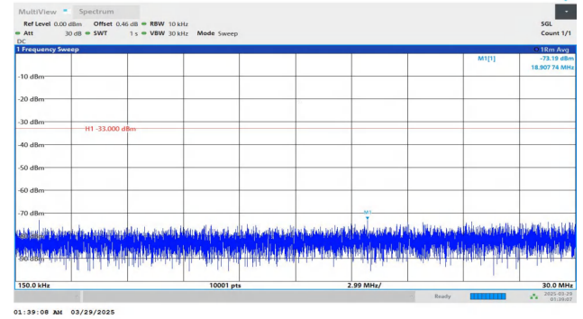
Band2-15MHz-QPSK-18900-1RB#0-0.15~30-PASS
