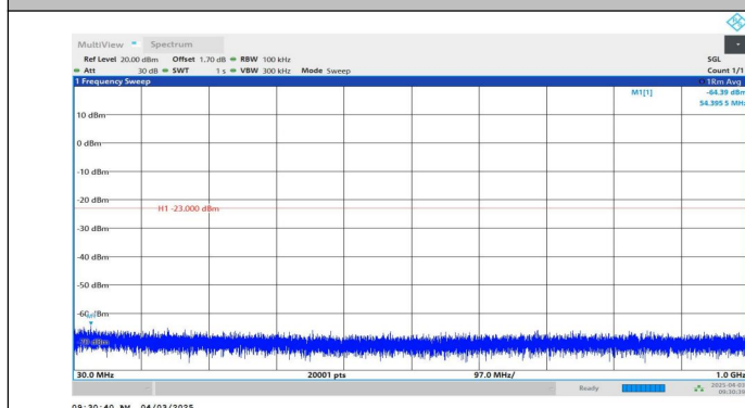
Band2-10MHz-QPSK-18900-1RB#0-30~1000-PASS
