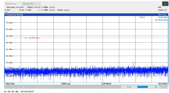
Band2-15MHz-QPSK-19125-1RB#0-0.15~30-PASS
