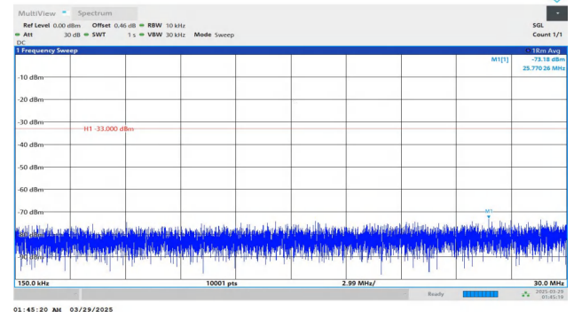
Band2-20MHz-QPSK-18700-1RB#0-0.15~30-PASS
