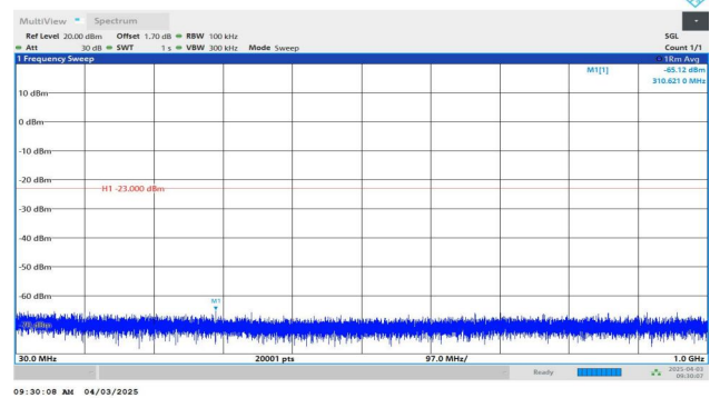
Band2-10MHz-QPSK-18650-1RB#0-30~1000-PASS
