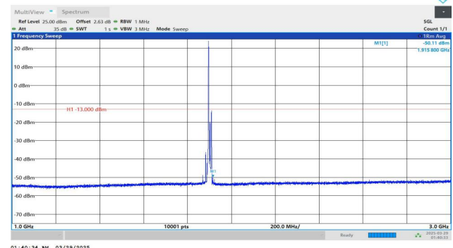
Band2-15MHz-QPSK-19125-1RB#0-1000~3000-PASS
