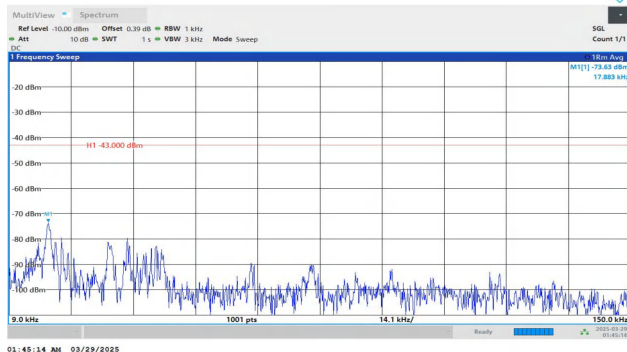
Band2-20MHz-QPSK-18700-1RB#0-0.009~0.15-PASS
