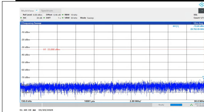
Band2-20MHz-QPSK-19100-1RB#99-0.15~30-PASS
