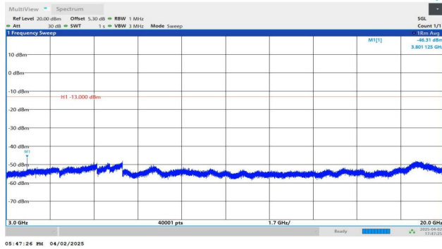
Band2-10MHz-QPSK-19150-1RB#0-3000~20000-PASS
