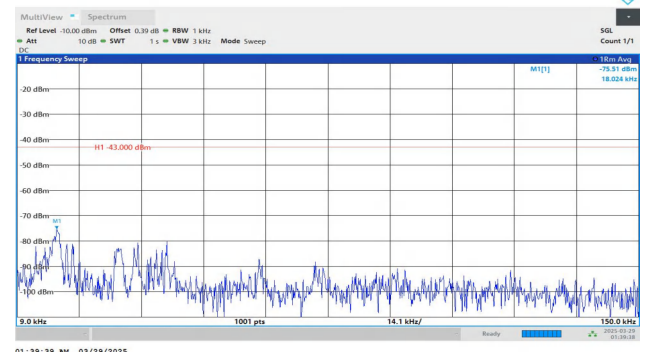
Band2-15MHz-QPSK-18900-1RB#74-0.009~0.15-PASS
