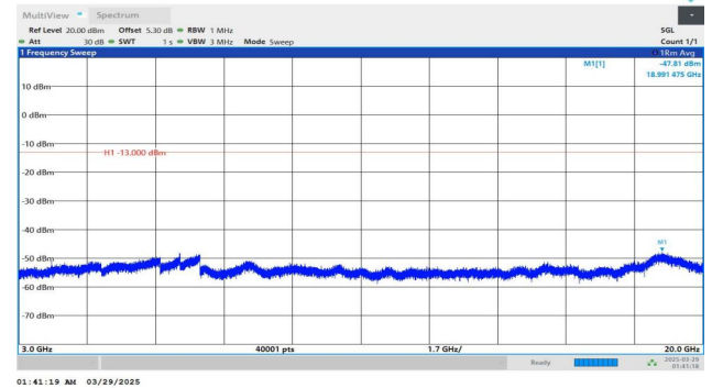
Band2-15MHz-QPSK-19125-1RB#74-3000~20000-PASS
