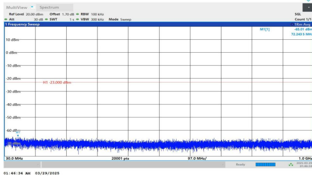
Band2-20MHz-QPSK-18900-1RB#0-30~1000-PASS
