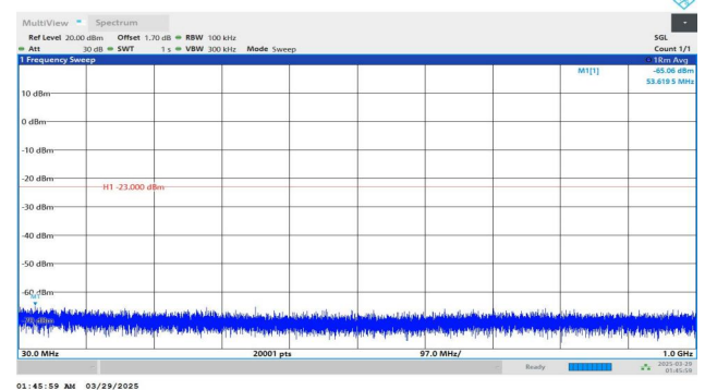
Band2-20MHz-QPSK-18700-1RB#99-30~1000-PASS
