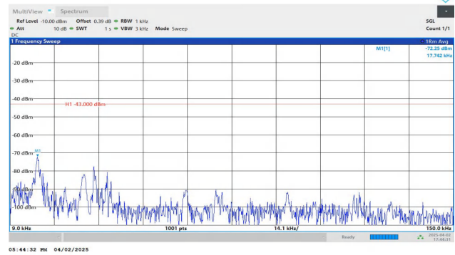
Band2-10MHz-QPSK-18650-1RB#0-0.009~0.15-PASS
