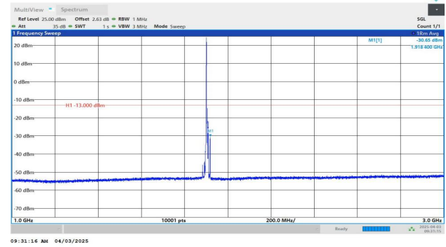
Band2-10MHz-QPSK-19150-1RB#0-1000~3000-PASS
