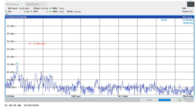
Band2-15MHz-QPSK-18675-1RB#74-0.009~0.15-PASS
