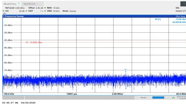
Band2-10MHz-QPSK-18900-1RB#49-0.15~30-PASS
