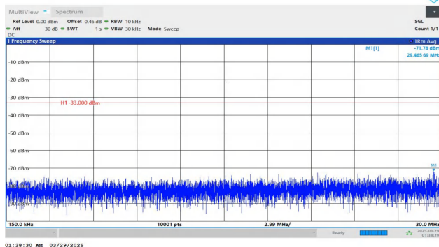
Band2-15MHz-QPSK-18675-1RB#74-0.15~30-PASS
