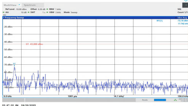
Band2-10MHz-QPSK-19150-1RB#0-0.009~0.15-PASS
