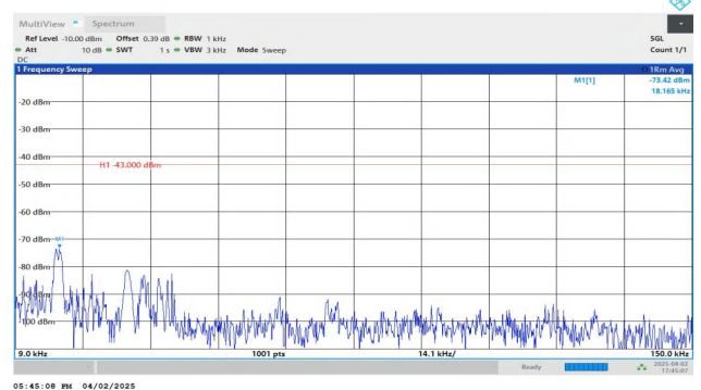
Band2-10MHz-QPSK-18650-1RB#49-0.009~0.15-PASS
