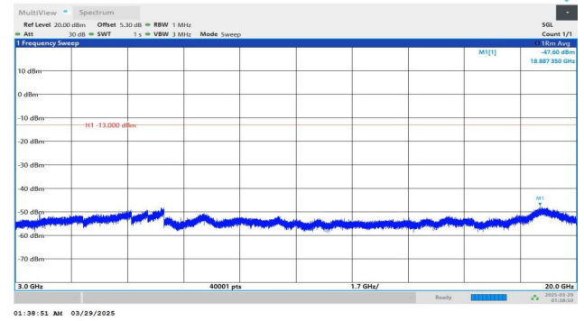
Band2-15MHz-QPSK-18675-1RB#74-3000~20000-PASS
