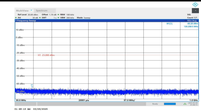
Band2-20MHz-QPSK-19100-1RB#99-30~1000-PASS
