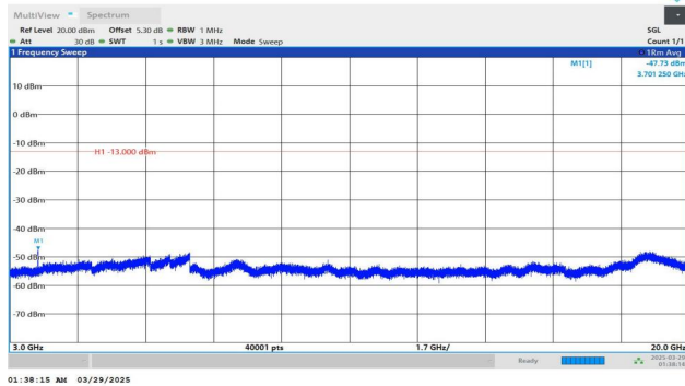
Band2-15MHz-QPSK-18675-1RB#0-3000~20000-PASS
