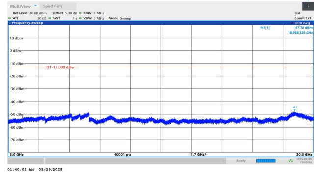
Band2-15MHz-QPSK-18900-1RB#74-3000~20000-PASS
