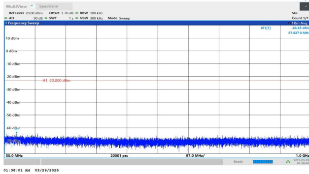
Band2-15MHz-QPSK-18675-1RB#0-30~1000-PASS
