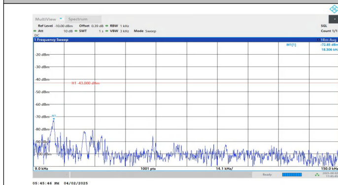
Band2-10MHz-QPSK-18900-1RB#0-0.009~0.15-PASS
