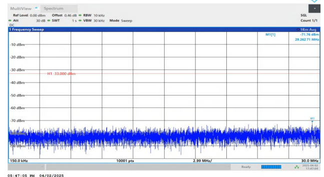
Band2-10MHz-QPSK-19150-1RB#0-0.15~30-PASS
