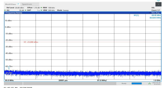
Band2-20MHz-QPSK-18900-1RB#99-30~1000-PASS
