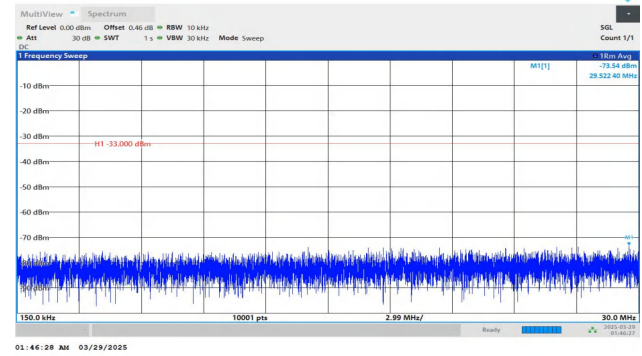
Band2-20MHz-QPSK-18900-1RB#0-0.15~30-PASS
