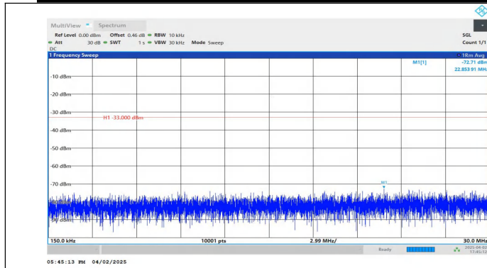
Band2-10MHz-QPSK-18650-1RB#49-0.15~30-PASS
