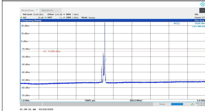
Band2-20MHz-QPSK-19100-1RB#99-1000~3000-PASS
