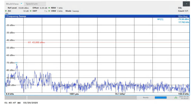
Band2-20MHz-QPSK-18700-1RB#99-0.009~0.15-PASS
