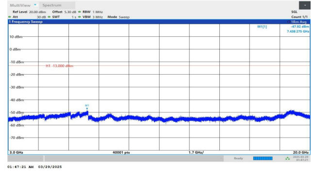
Band2-20MHz-QPSK-18900-1RB#99-3000~20000-PASS
