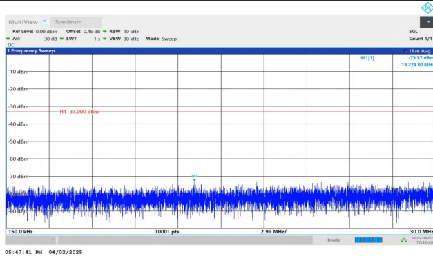
Band2-10MHz-QPSK-19150-1RB#49-0.15~30-PASS
