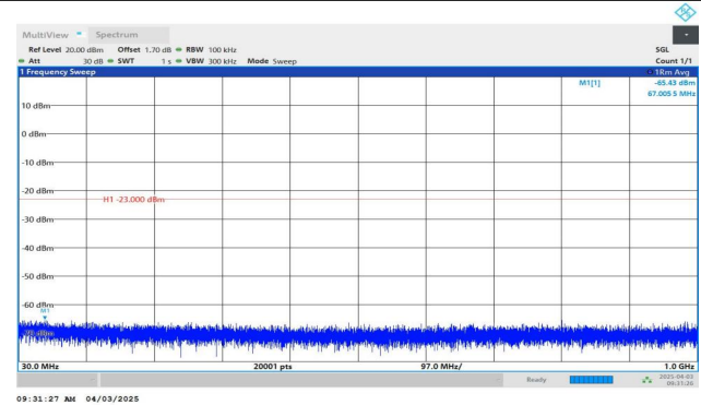
Band2-10MHz-QPSK-19150-1RB#49-30~1000-PASS
