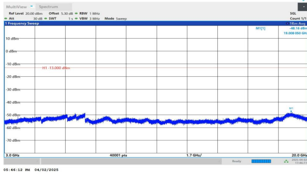
Band2-10MHz-QPSK-18900-1RB#0-3000~20000-PASS
