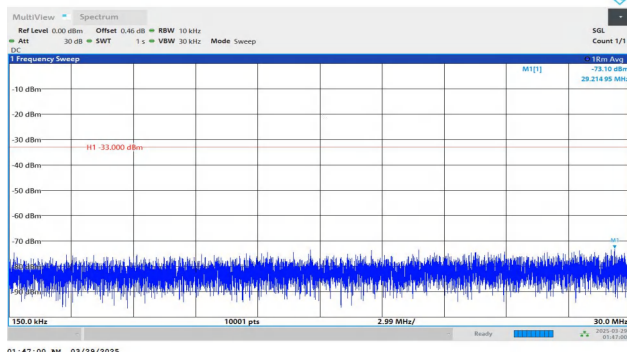
Band2-20MHz-QPSK-18900-1RB#99-0.15~30-PASS
