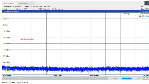
Band2-15MHz-QPSK-18900-1RB#0-30~1000-PASS
