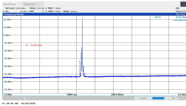
Band2-15MHz-QPSK-18675-1RB#74-1000~3000-PASS
