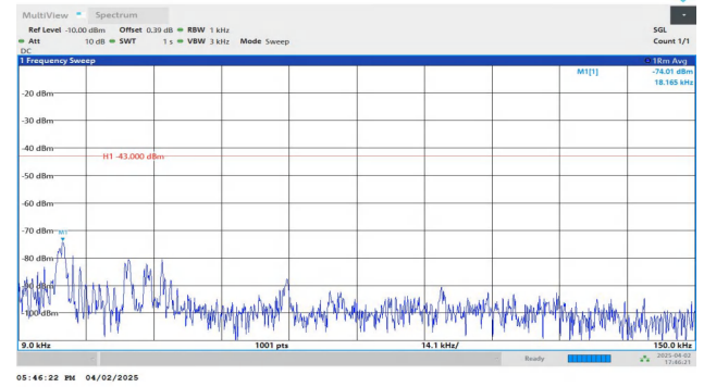
Band2-10MHz-QPSK-18900-1RB#49-0.009~0.15-PASS
