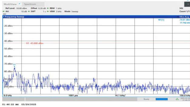
Band2-20MHz-QPSK-18900-1RB#0-0.009~0.15-PASS
