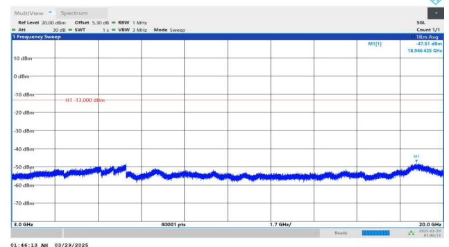
Band2-20MHz-QPSK-18700-1RB#99-3000~20000-PASS
