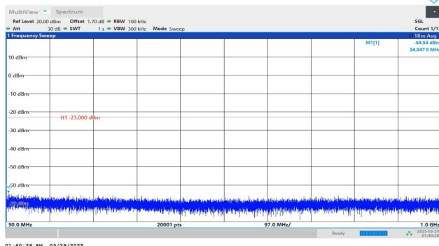
Band2-15MHz-QPSK-19125-1RB#0-30~1000-PASS
