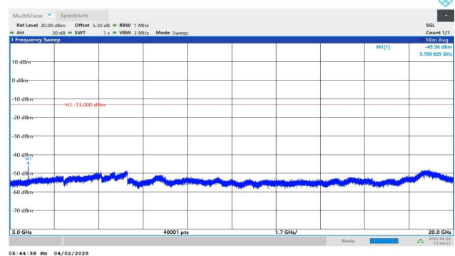
Band2-10MHz-QPSK-18650-1RB#0-3000~20000-PASS
