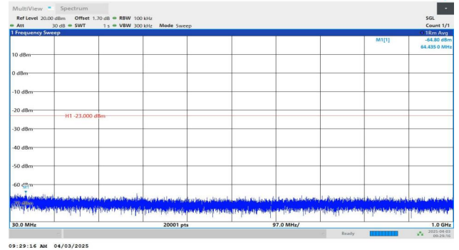
Band2-5MHz-QPSK-18900-1RB#24-30~1000-PASS
