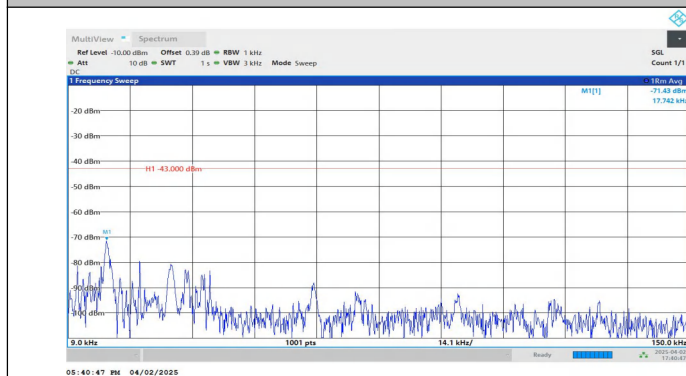
Band2-5MHz-QPSK-18625-1RB#0-0.009~0.15-PASS
