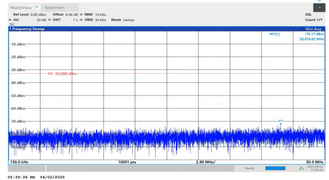
Band2-3MHz-QPSK-19185-1RB#0-0.15~30-PASS
