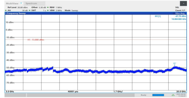
Band2-1.4MHz-QPSK-19193-1RB#5-3000~20000-PASS
