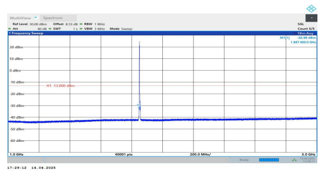
Band2-3MHz-QPSK-18615-1RB#0-1000~3000-PASS
