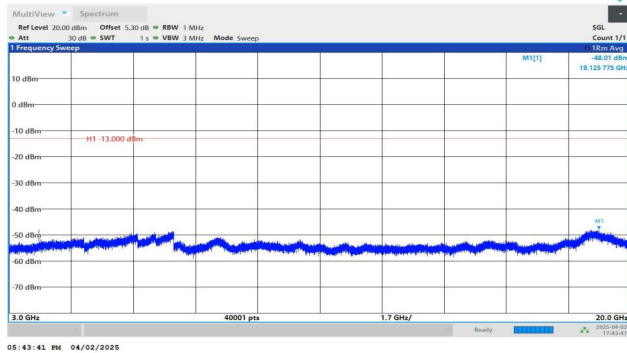
Band2-5MHz-QPSK-19175-1RB#0-3000~20000-PASS
