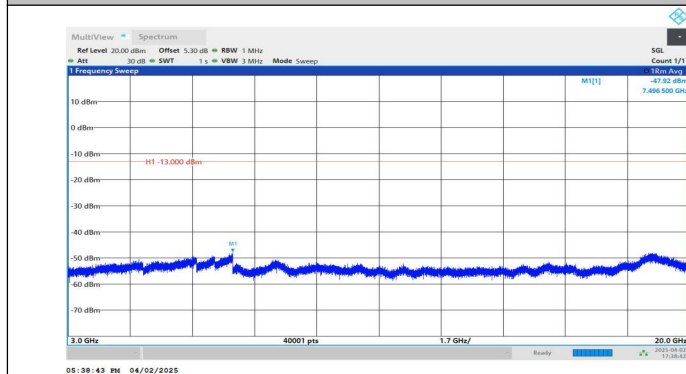
Band2-3MHz-QPSK-18900-1RB#0-3000~20000-PASS
