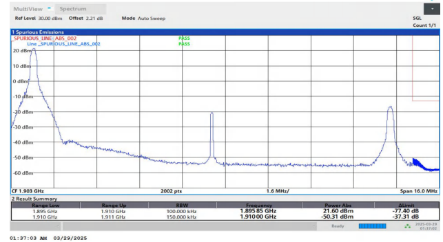
Band2-15MHz-QPSK-18675-1RB#74-PASS
