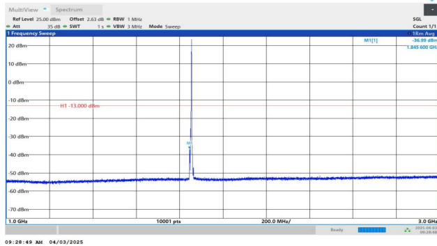
Band2-5MHz-QPSK-18625-1RB#24-1000~3000-PASS
