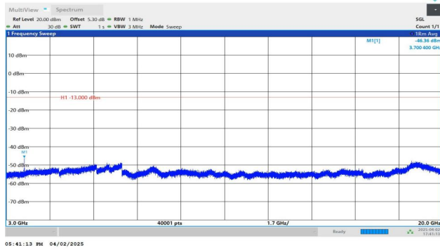
Band2-5MHz-QPSK-18625-1RB#0-3000~20000-PASS
