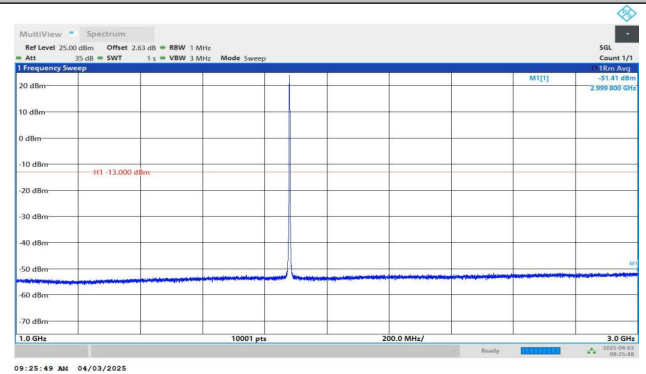
Band2-1.4MHz-QPSK-18900-1RB#0-1000~3000-PASS
