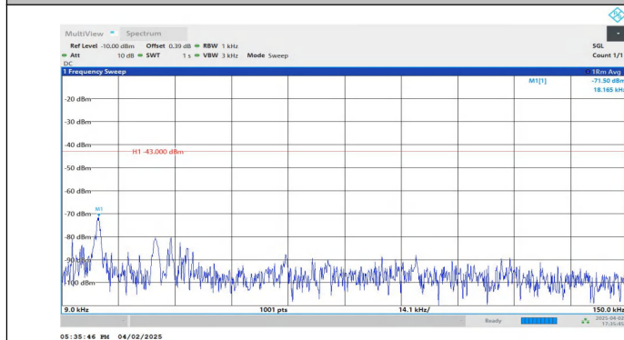
Band2-1.4MHz-QPSK-19193-1RB#0-0.009~0.15-PASS
