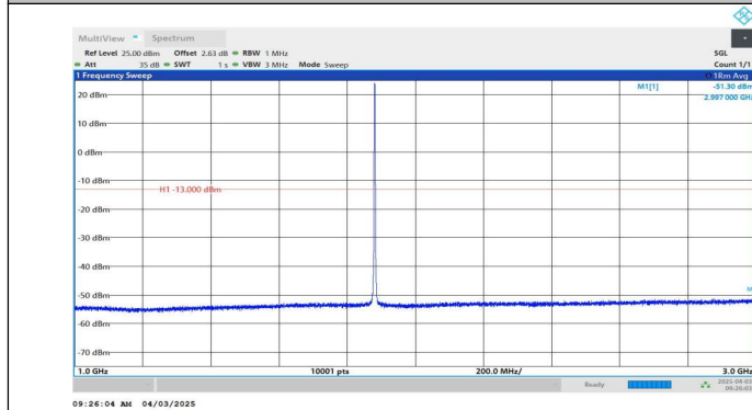
Band2-1.4MHz-QPSK-18900-1RB#5-1000~3000-PASS
