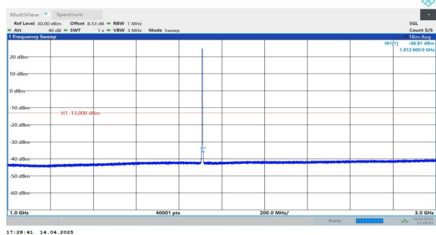
Band2-1.4MHz-QPSK-19193-1RB#5-1000~3000-PASS
