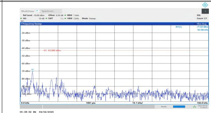
Band2-3MHz-QPSK-18900-1RB#14-0.009~0.15-PASS
