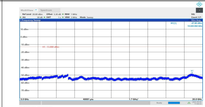
Band2-3MHz-QPSK-19185-1RB#14-3000~20000-PASS
