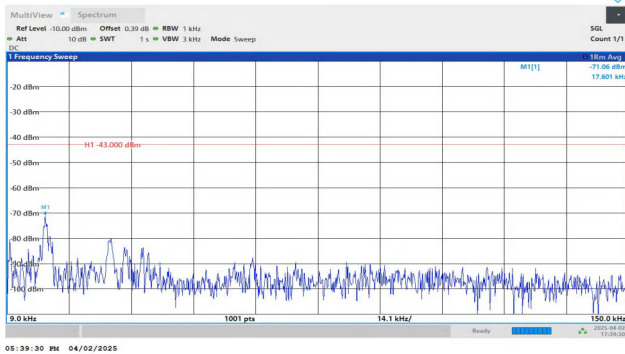
Band2-3MHz-QPSK-19185-1RB#0-0.009~0.15-PASS
