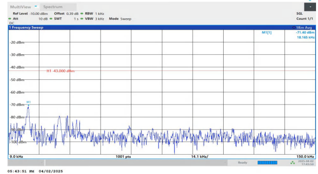
Band2-5MHz-QPSK-19175-1RB#24-0.009~0.15-PASS
