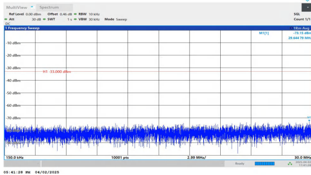
Band2-5MHz-QPSK-18625-1RB#24-0.15~30-PASS
