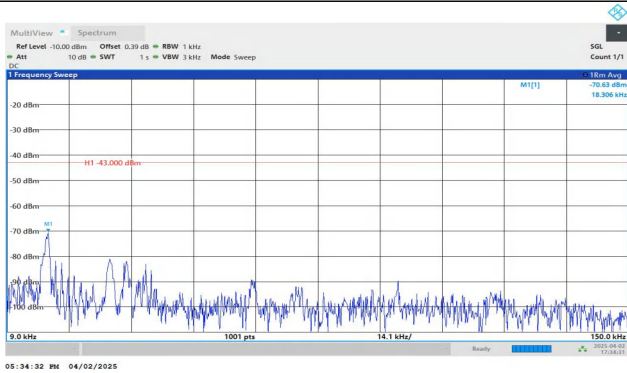
Band2-1.4MHz-QPSK-18900-1RB#0-0.009~0.15-PASS
