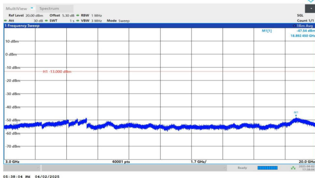
Band2-3MHz-QPSK-18615-1RB#14-3000~20000-PASS
