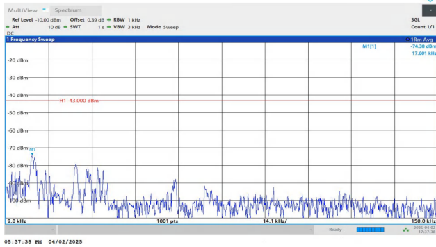
Band2-3MHz-QPSK-18615-1RB#14-0.009~0.15-PASS
