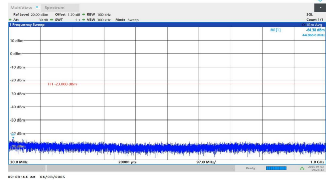
Band2-5MHz-QPSK-18625-1RB#24-30~1000-PASS
