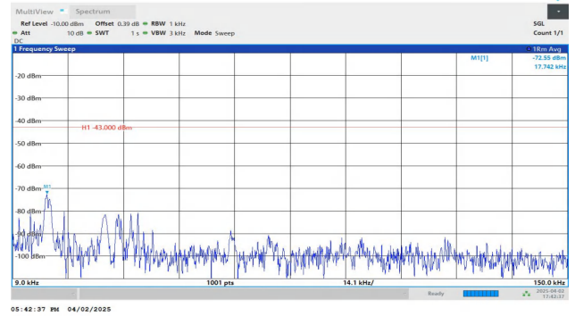
Band2-5MHz-QPSK-18900-1RB#24-0.009~0.15-PASS
