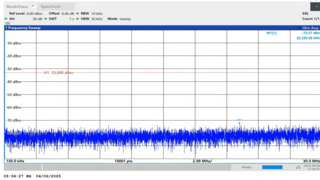
Band2-1.4MHz-QPSK-19193-1RB#5-0.15~30-PASS
