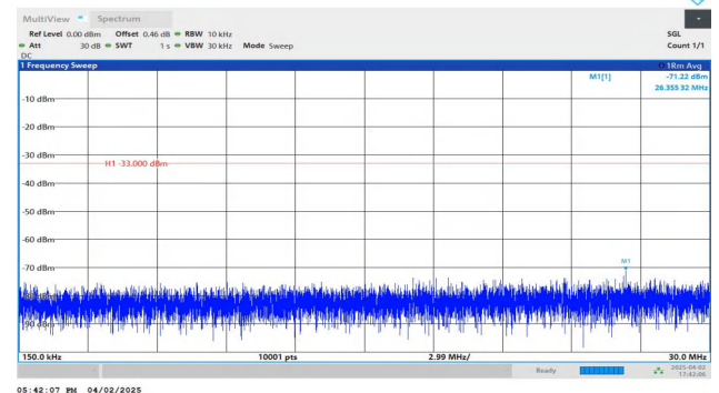
Band2-5MHz-QPSK-18900-1RB#0-0.15~30-PASS
