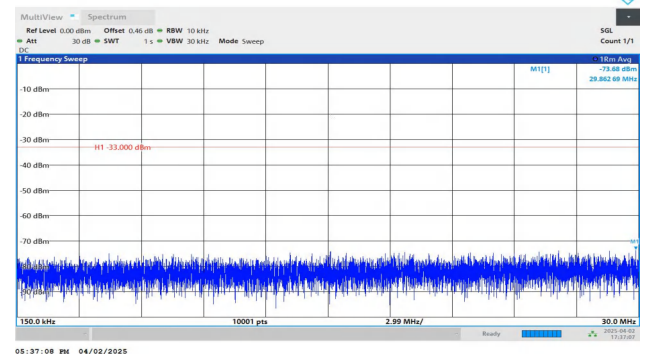
Band2-3MHz-QPSK-18615-1RB#0-0.15~30-PASS
