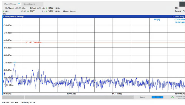
Band2-5MHz-QPSK-19175-1RB#0-0.009~0.15-PASS
