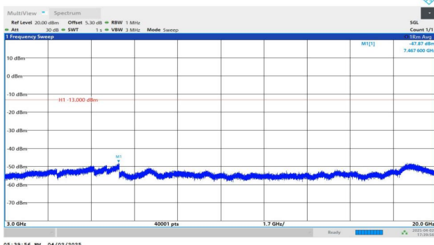
Band2-3MHz-QPSK-19185-1RB#0-3000~20000-PASS
