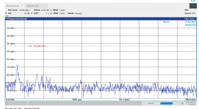
Band2-3MHz-QPSK-19185-1RB#14-0.009~0.15-PASS
