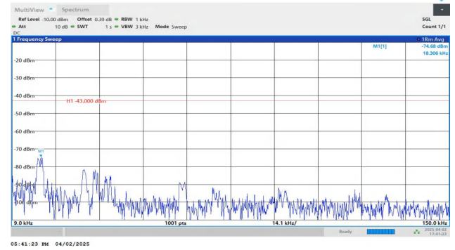
Band2-5MHz-QPSK-18625-1RB#24-0.009~0.15-PASS
