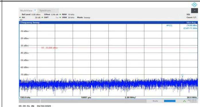
Band2-1.4MHz-QPSK-19193-1RB#0-0.15~30-PASS
