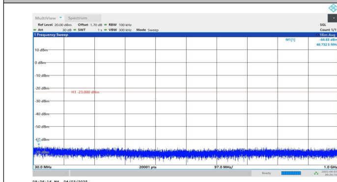
Band2-1.4MHz-QPSK-19193-1RB#0-30~1000-PASS
