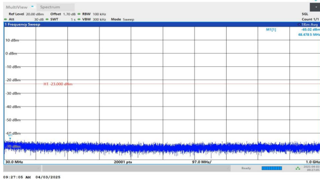
Band2-3MHz-QPSK-18615-1RB#14-30~1000-PASS
