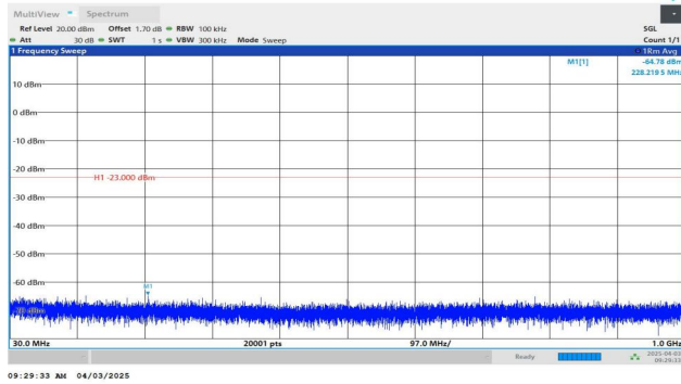
Band2-5MHz-QPSK-19175-1RB#0-30~1000-PASS
