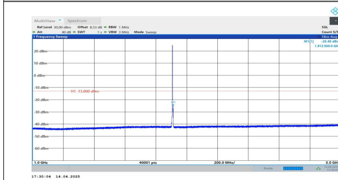
Band2-3MHz-QPSK-19185-1RB#14-1000~3000-PASS
