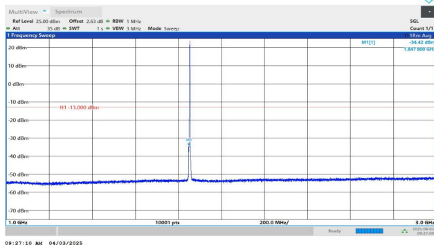
Band2-3MHz-QPSK-18615-1RB#14-1000~3000-PASS
