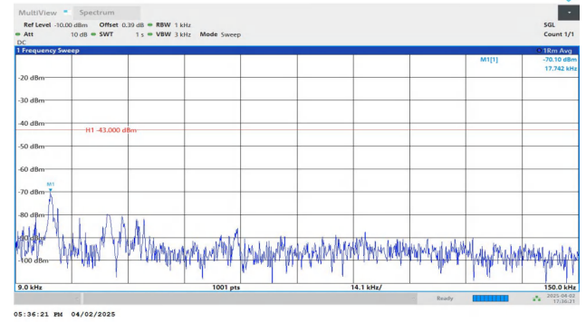
Band2-1.4MHz-QPSK-19193-1RB#5-0.009~0.15-PASS
