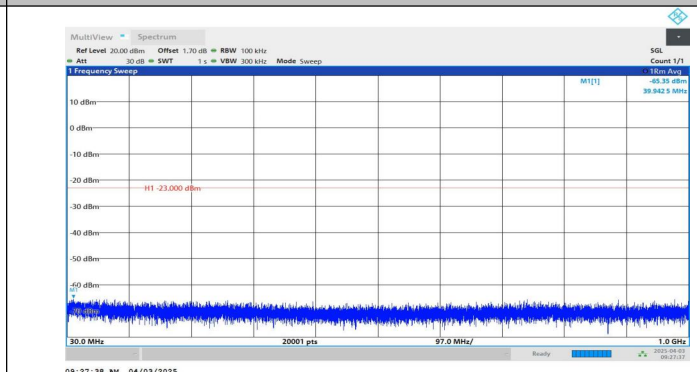
Band2-3MHz-QPSK-18900-1RB#14-30~1000-PASS
