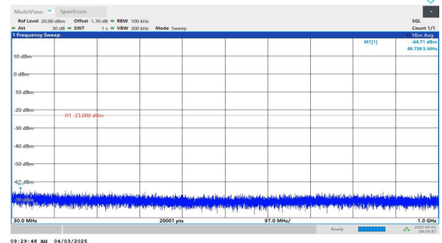
Band2-5MHz-QPSK-19175-1RB#24-30~1000-PASS
