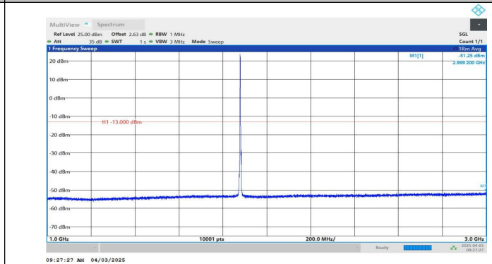
Band2-3MHz-QPSK-18900-1RB#0-1000~3000-PASS
