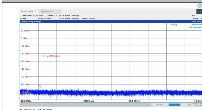
Band2-5MHz-QPSK-18625-1RB#0-30~1000-PASS
