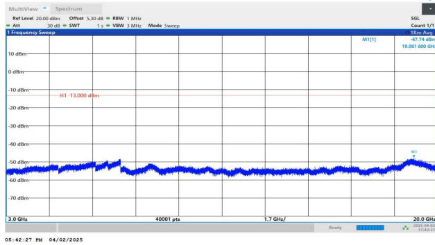
Band2-5MHz-QPSK-18900-1RB#0-3000~20000-PASS
