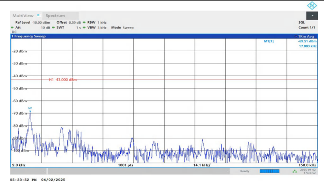
Band2-1.4MHz-QPSK-18607-1RB#5-0.009~0.15-PASS
