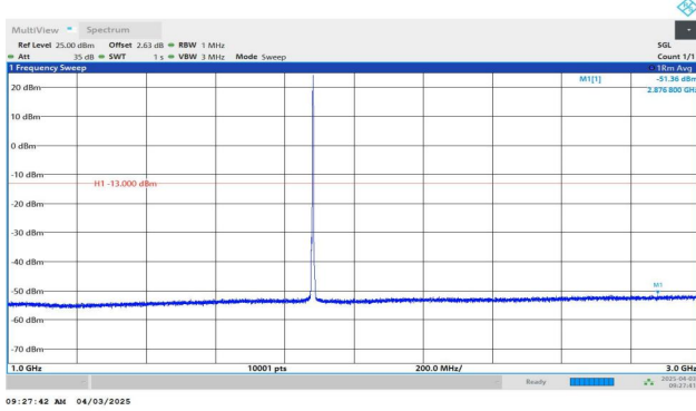
Band2-3MHz-QPSK-18900-1RB#14-1000~3000-PASS
