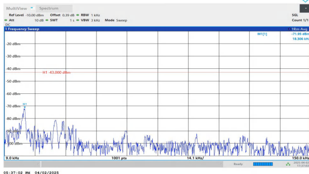
Band2-3MHz-QPSK-18615-1RB#0-0.009~0.15-PASS
