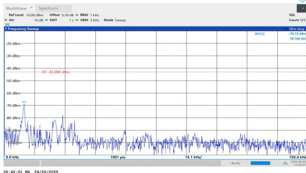
Band2-5MHz-QPSK-18900-1RB#0-0.009~0.15-PASS
