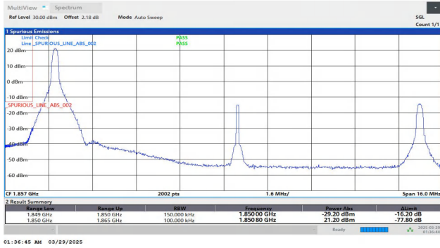
Band2-15MHz-QPSK-18675-1RB#0-PASS
