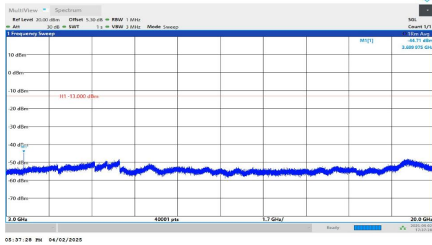
Band2-3MHz-QPSK-18615-1RB#0-3000~20000-PASS
