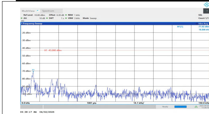
Band2-3MHz-QPSK-18900-1RB#0-0.009~0.15-PASS
