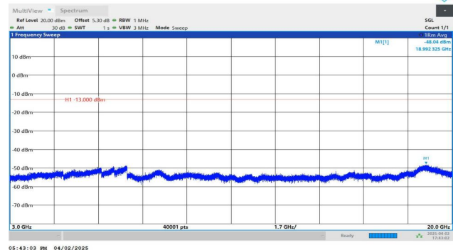
Band2-5MHz-QPSK-18900-1RB#24-3000~20000-PASS
