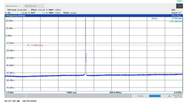
Band2-3MHz-QPSK-19185-1RB#0-1000~3000-PASS
