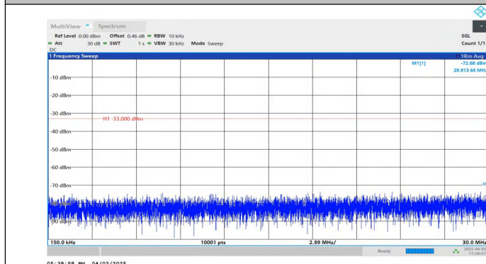
Band2-3MHz-QPSK-18900-1RB#14-0.15~30-PASS
