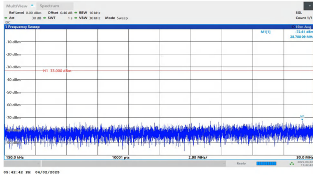
Band2-5MHz-QPSK-18900-1RB#24-0.15~30-PASS
