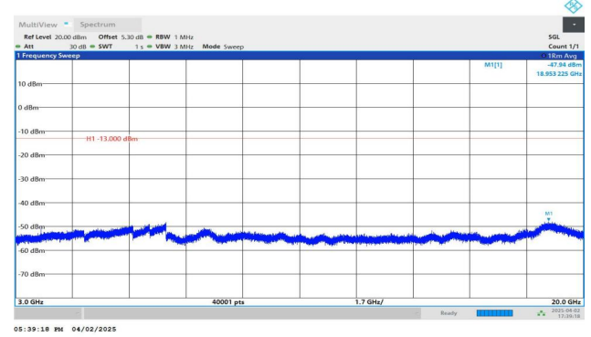
Band2-3MHz-QPSK-18900-1RB#14-3000~20000-PASS
