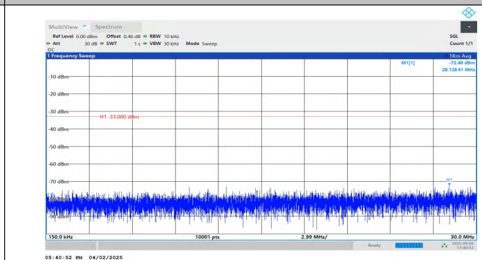
Band2-5MHz-QPSK-18625-1RB#0-0.15~30-PASS
