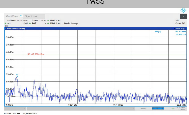
Band2-1.4MHz-QPSK-18900-1RB#5-0.009~0.15-PASS
