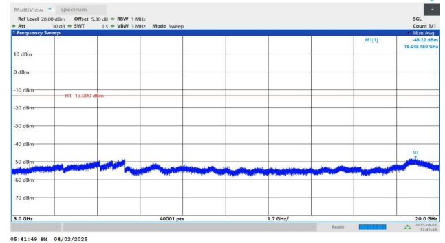
Band2-5MHz-QPSK-18625-1RB#24-3000~20000-PASS
