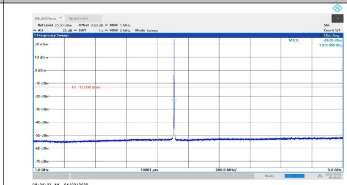
Band2-1.4MHz-QPSK-19193-1RB#0-1000~3000-PASS
