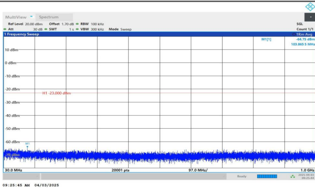
Band2-1.4MHz-QPSK-18900-1RB#0-30~1000-PASS
