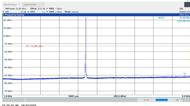
Band2-5MHz-QPSK-18900-1RB#24-1000~3000-PASS
