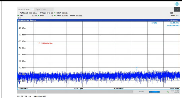
Band2-3MHz-QPSK-18900-1RB#0-0.15~30-PASS
