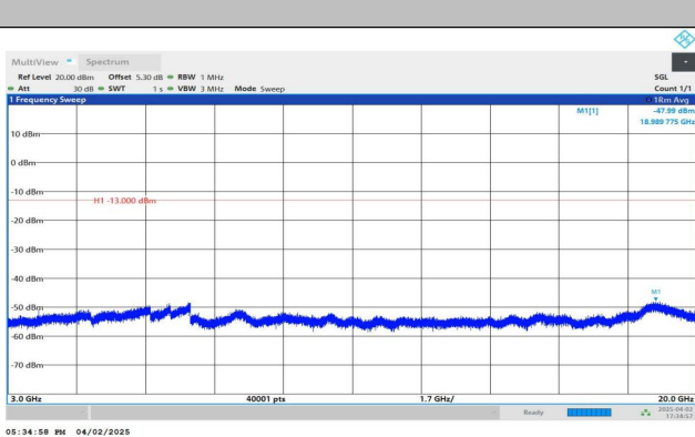
Band2-1.4MHz-QPSK-18900-1RB#0-3000~20000-PASS
