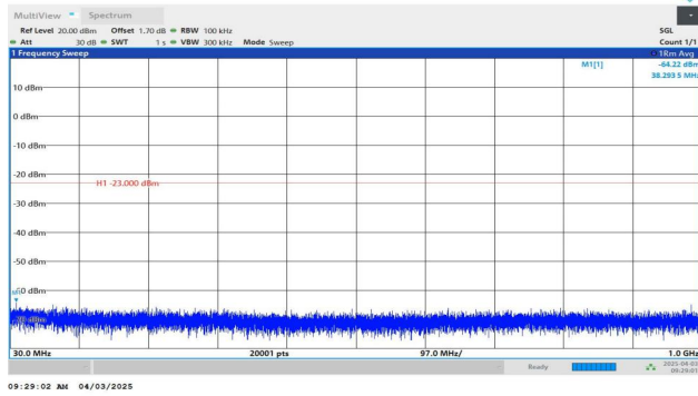
Band2-5MHz-QPSK-18900-1RB#0-30~1000-PASS
