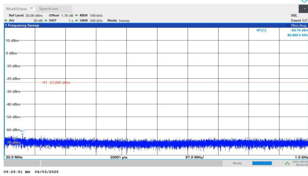
Band2-3MHz-QPSK-18615-1RB#0-30~1000-PASS
