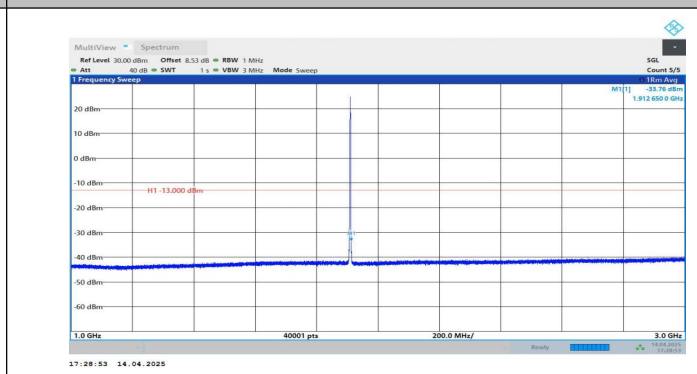
Band2-5MHz-QPSK-18625-1RB#0-1000~3000-PASS
