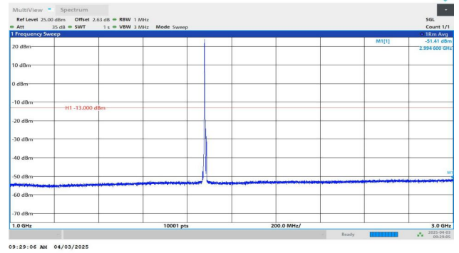
Band2-5MHz-QPSK-18900-1RB#0-1000~3000-PASS
