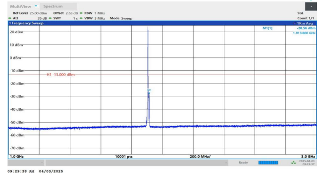
Band2-5MHz-QPSK-19175-1RB#0-1000~3000-PASS
