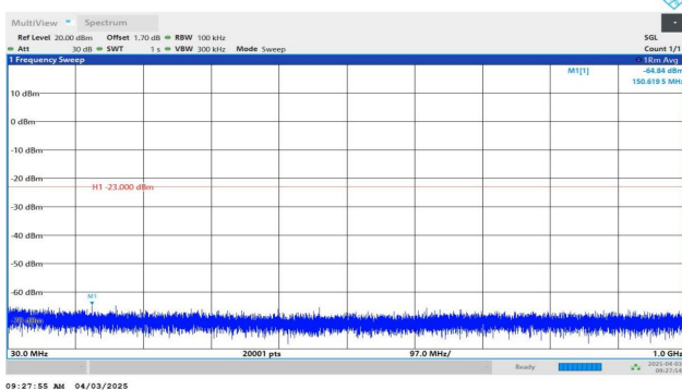
Band2-3MHz-QPSK-19185-1RB#0-30~1000-PASS
