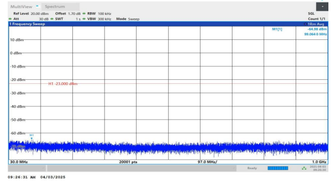
Band2-1.4MHz-QPSK-19193-1RB#5-30~1000-PASS
