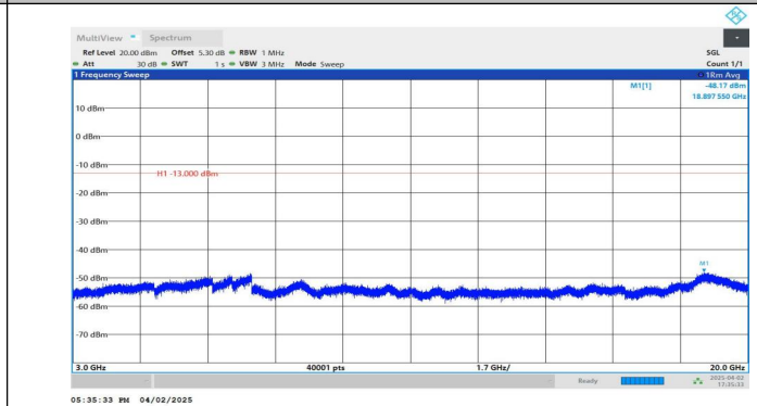
Band2-1.4MHz-QPSK-18900-1RB#5-3000~20000-PASS
