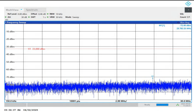
Band2-1.4MHz-QPSK-18900-1RB#0-0.15~30-PASS
