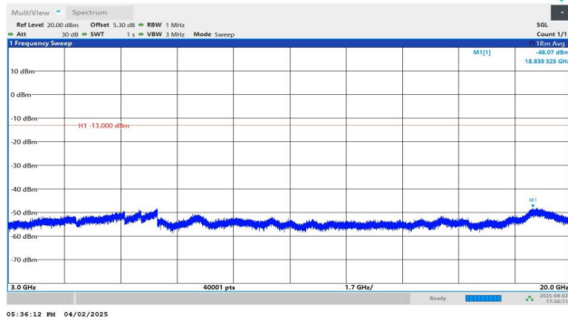
Band2-1.4MHz-QPSK-19193-1RB#0-3000~20000-PASS
