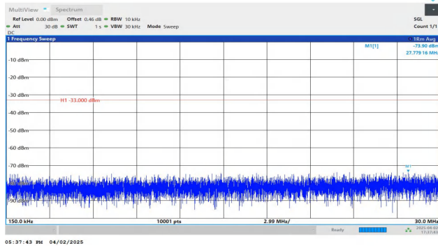
Band2-3MHz-QPSK-18615-1RB#14-0.15~30-PASS
