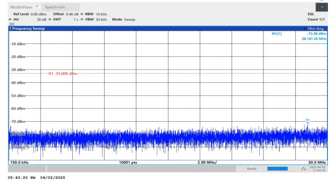
Band2-5MHz-QPSK-19175-1RB#0-0.15~30-PASS
