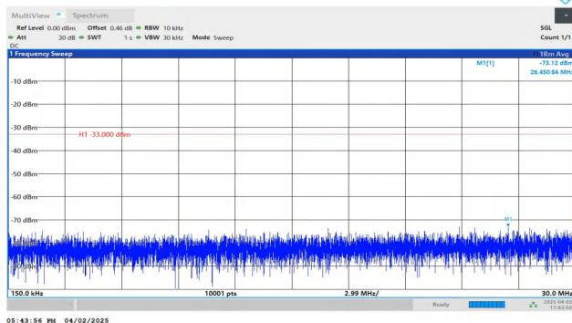
Band2-5MHz-QPSK-19175-1RB#24-0.15~30-PASS
