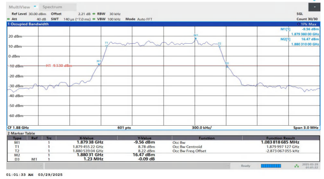
Band2-1.4MHz-16QAM-18900-6RB#0-PASS
