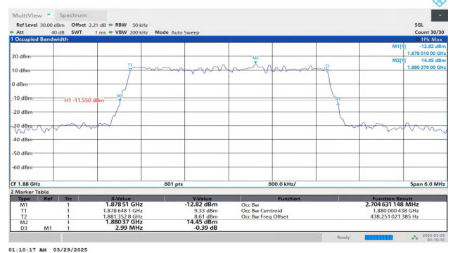
Band2-3MHz-16QAM-18900-15RB#0-PASS
