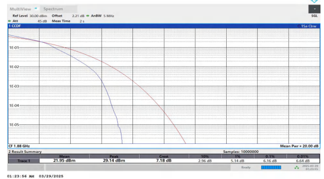
Band2-5MHz-16QAM-18900-25RB#0-PASS
