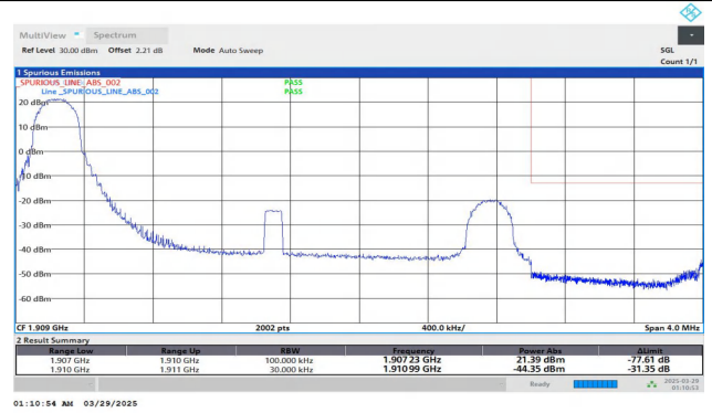
Band2-3MHz-QPSK-19185-1RB#0-PASS
