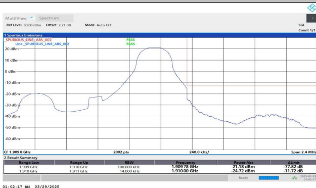
Band2-1.4MHz-QPSK-19193-1RB#0-PASS
