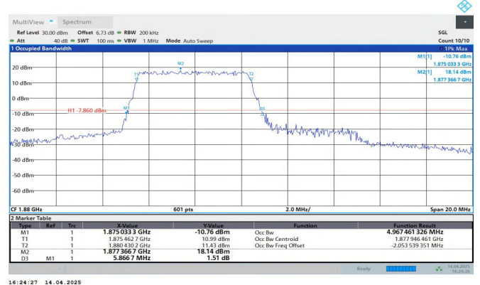
Band2-5MHz-16QAM-18900-25RB#0-PASS
