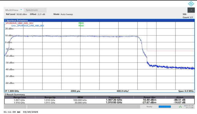
Band2-3MHz-QPSK-19185-15RB#0-PASS
