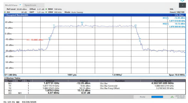
Band2-5MHz-16QAM-18900-25RB#0-PASS
