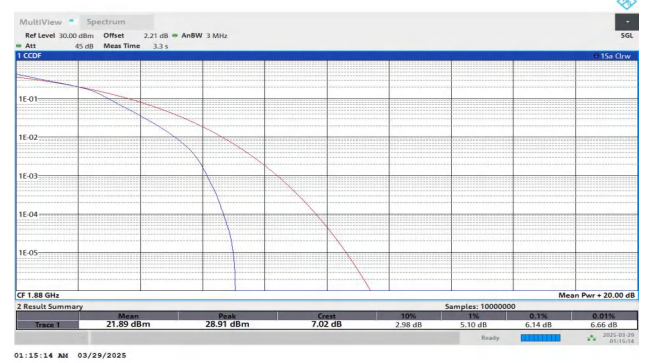
Band2-3MHz-16QAM-18900-15RB#0-PASS
