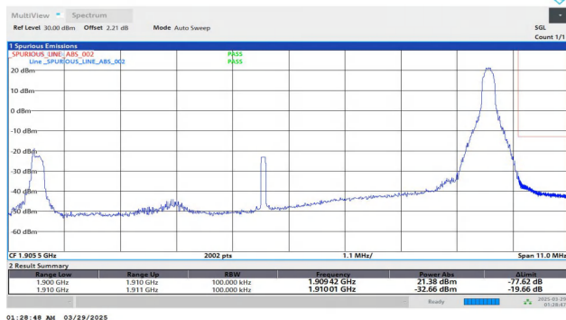
Band2-10MHz-QPSK-19150-1RB#49-PASS
