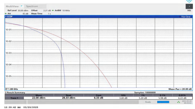
Band2-10MHz-16QAM-18900-27RB#0-PASS
