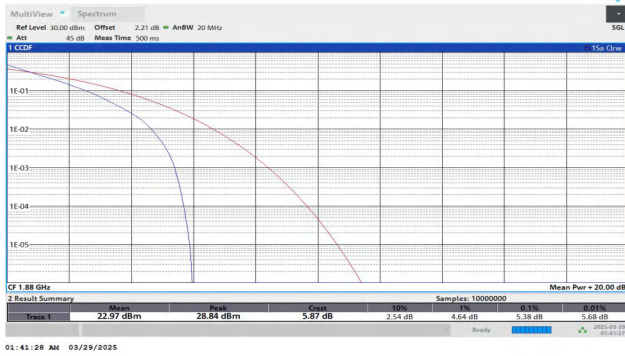
Band2-15MHz-QPSK-18900-75RB#0-PASS
