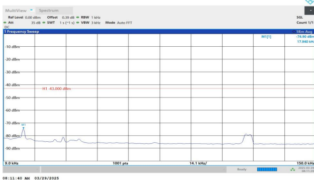
Band4-1513-2-0.009~0.15MHz-PASS
