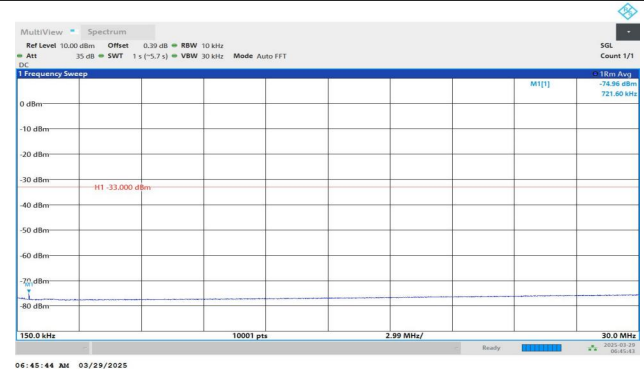
Band4-1513-2-0.15~30MHz-PASS
