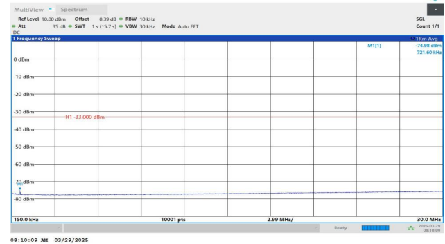
Band4-1312-2-0.15~30MHz-PASS
