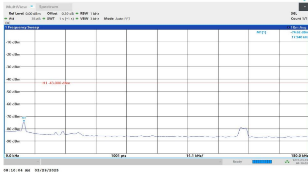
Band4-1312-2-0.009~0.15MHz-PASS
