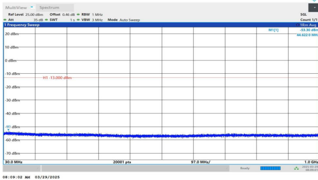
Band4-1513-1-30~1000MHz-PASS
