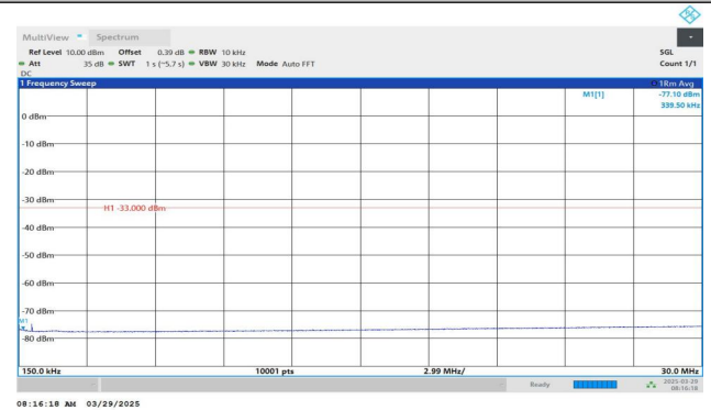
Band4-1312-4-0.15~30MHz-PASS
