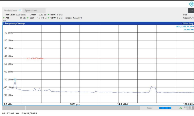
Band4-1312-1-0.009~0.15MHz-PASS
