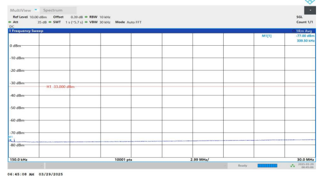
Band4-1413-2-0.15~30MHz-PASS
