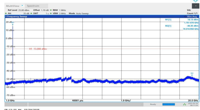
Band4-1513-2-1000~20000MHz-PASS
