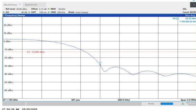
Band4-1513-2-PASS
