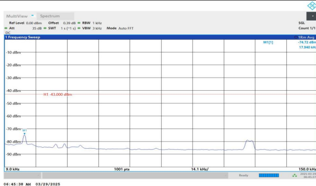
Band4-1513-2-0.009~0.15MHz-PASS
