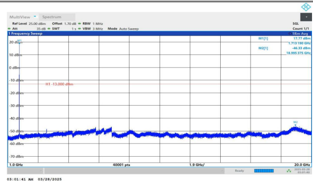
Band4-1312-1000~20000MHz-PASS
