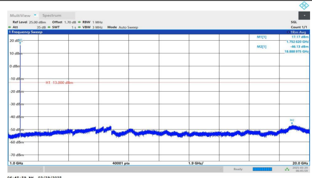
Band4-1513-2-1000~20000MHz-PASS
