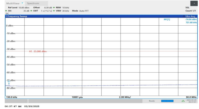
Band4-1413-1-0.15~30MHz-PASS
