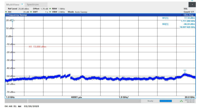
Band4-1312-3-1000~20000MHz-PASS
