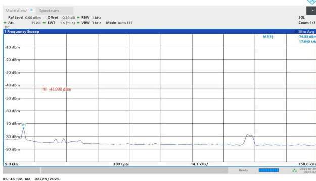
Band4-1413-2-0.009~0.15MHz-PASS
