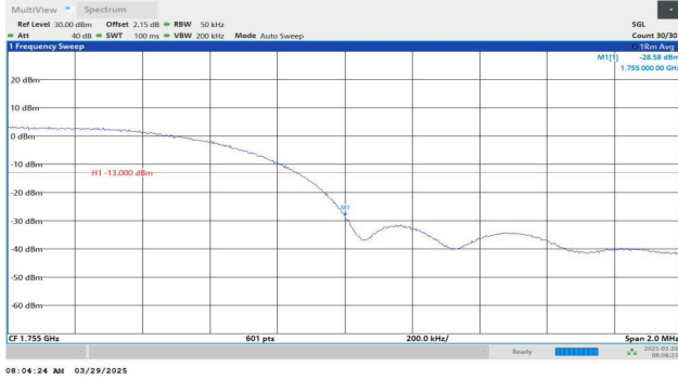
Band4-1513-4-PASS
