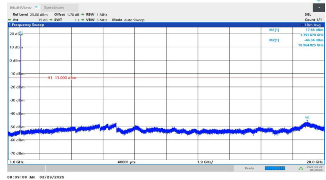
Band4-1513-1-1000~20000MHz-PASS
