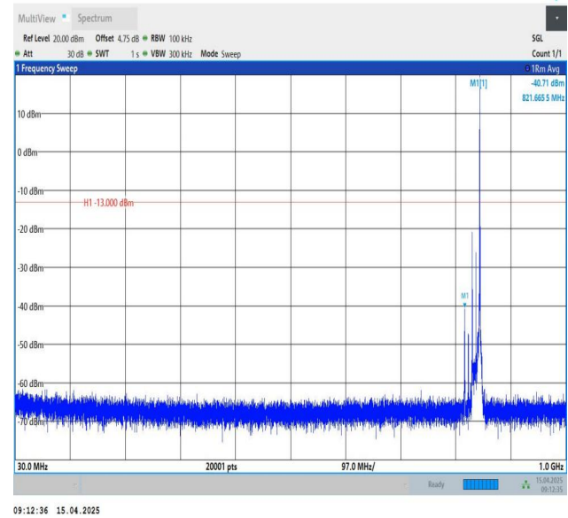
Band26(824-849)-15MHz-QPSK-26965-1RB#74-30~1000-PASS
