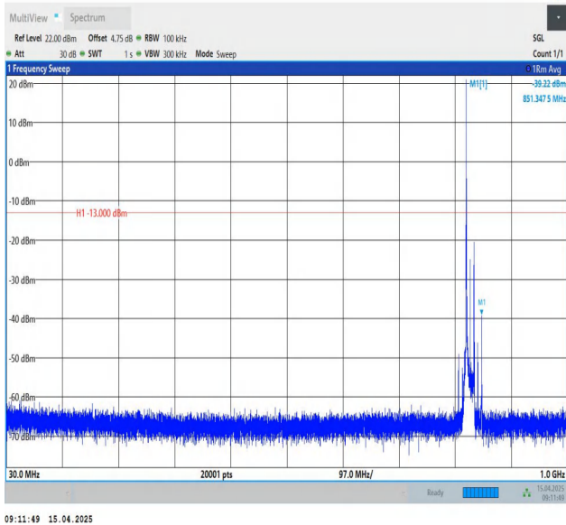
Band26(824-849)-15MHz-QPSK-26865-1RB#0-30~1000-PASS
