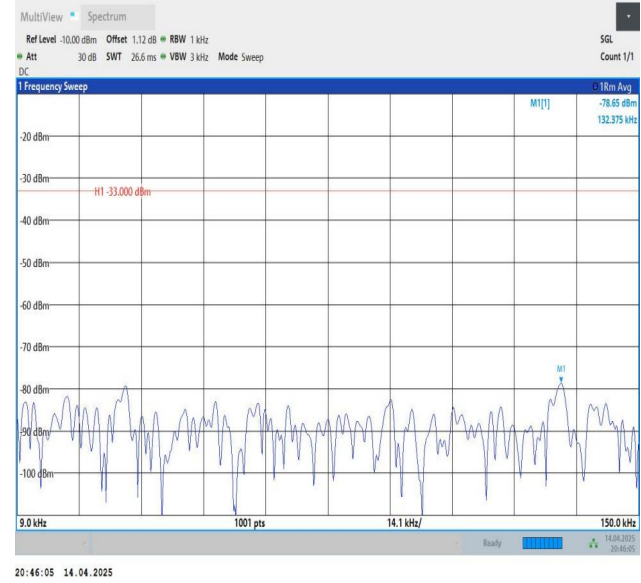
Band26(824-849)-15MHz-QPSK-26965-1RB#74-0.009~0.15-PASS
