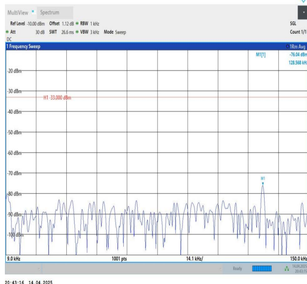
Band26(824-849)-10MHz-QPSK-26990-1RB#49-0.009~0.15-PASS
