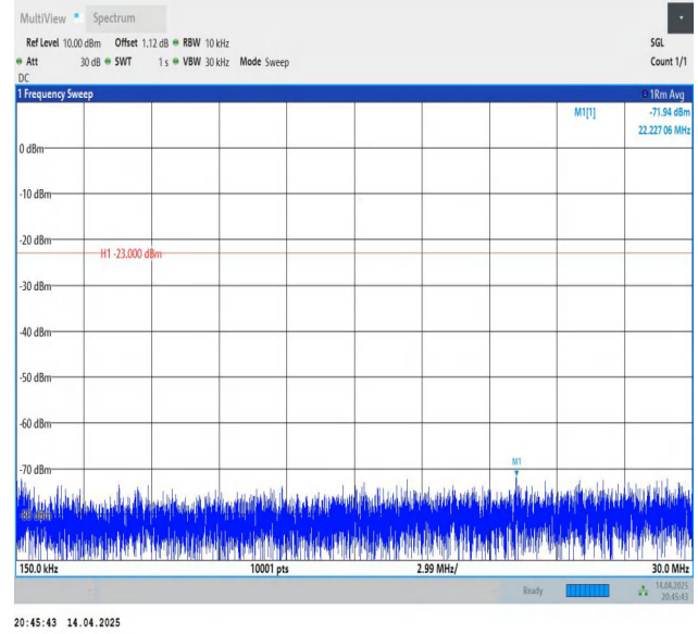
Band26(824-849)-15MHz-QPSK-26965-1RB#0-0.15~30-PASS
