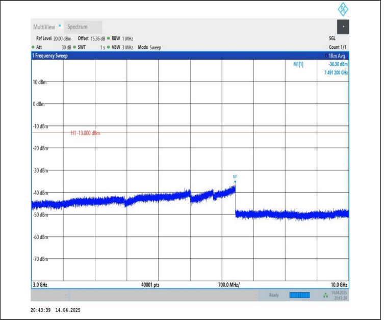
Band26(824-849)-10MHz-QPSK-26990-1RB#49-3000~10000-PAS
