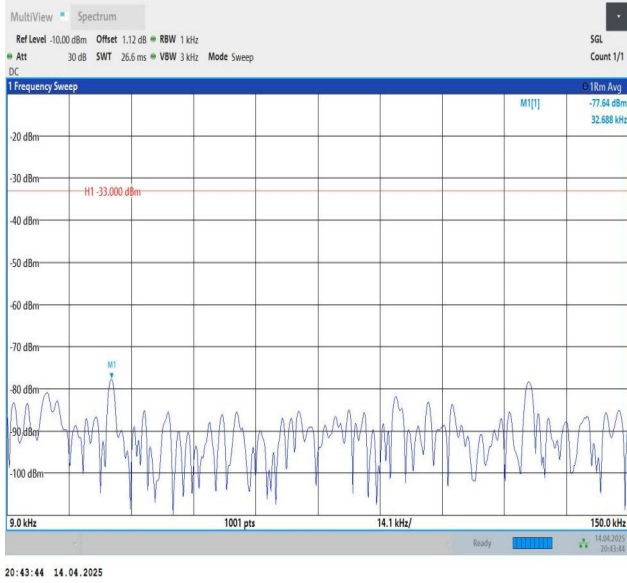
Band26(824-849)-15MHz-QPSK-26865-1RB#0-0.009~0.15-PASS
