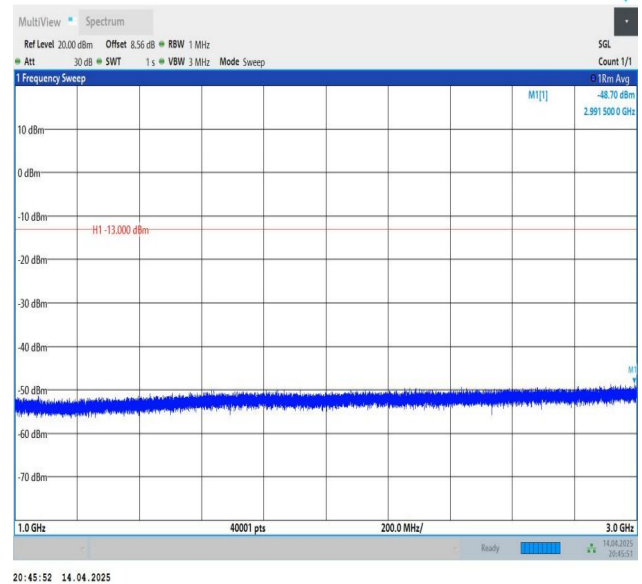
Band26(824-849)-15MHz-QPSK-26965-1RB#0-1000~3000-PASS
