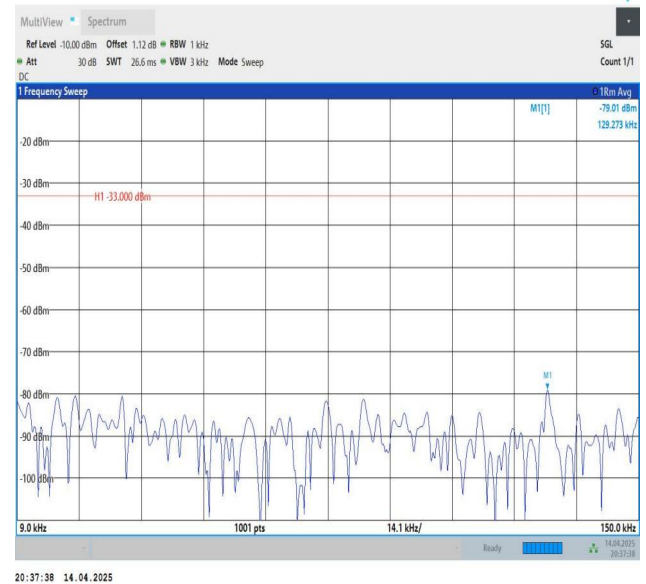
Band26(824-849)-3MHz-QPSK-27025-1RB#14-0.009~0.15-PASS
