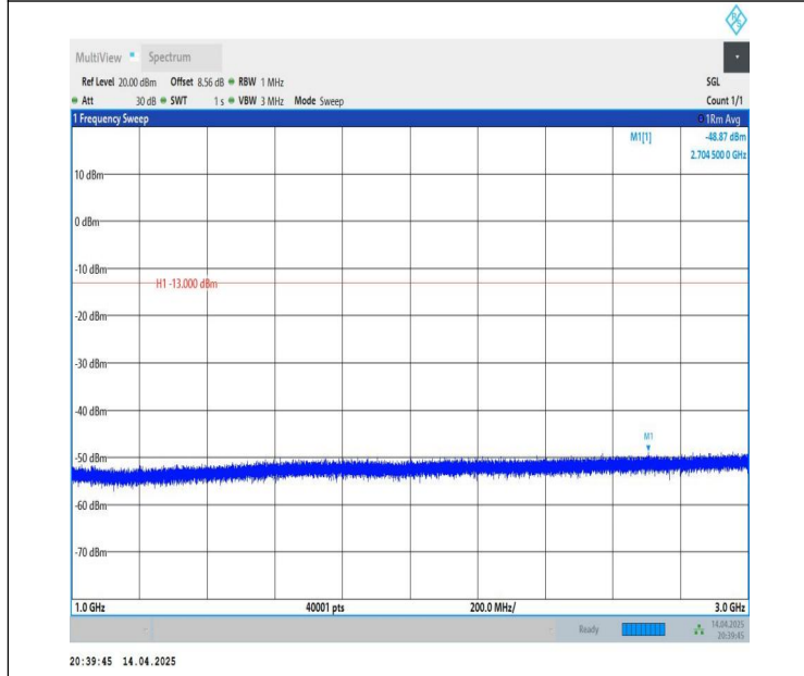
Band26(824-849)-5MHz-QPSK-26915-1RB#24-1000~3000-PASS
