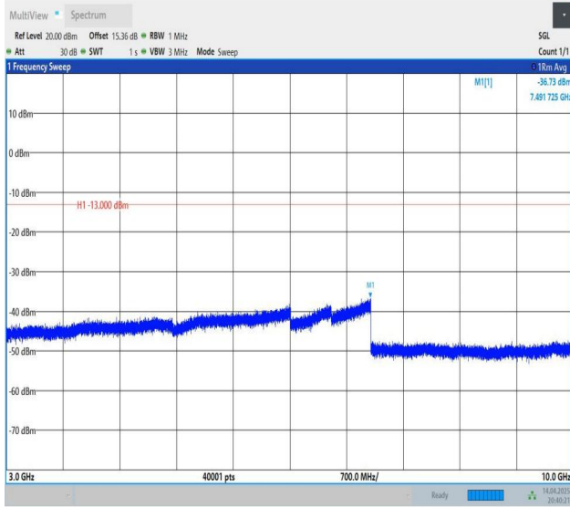
Band26(824-849)-5MHz-QPSK-27015-1RB#0-3000~10000-PASS
