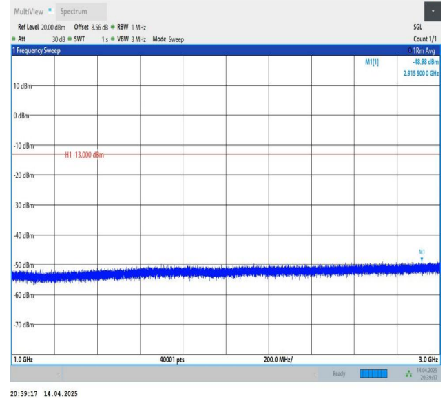
Band26(824-849)-5MHz-QPSK-26915-1RB#0-1000~3000-PASS
