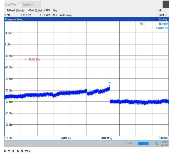
Band26(824-849)-1.4MHz-QPSK-27033-1RB#5-3000~10000-PASS
