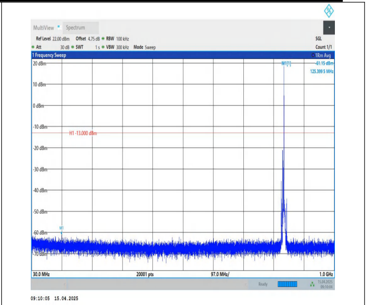
Band26(824-849)-5MHz-QPSK-26915-1RB#24-30~1000-PASS
