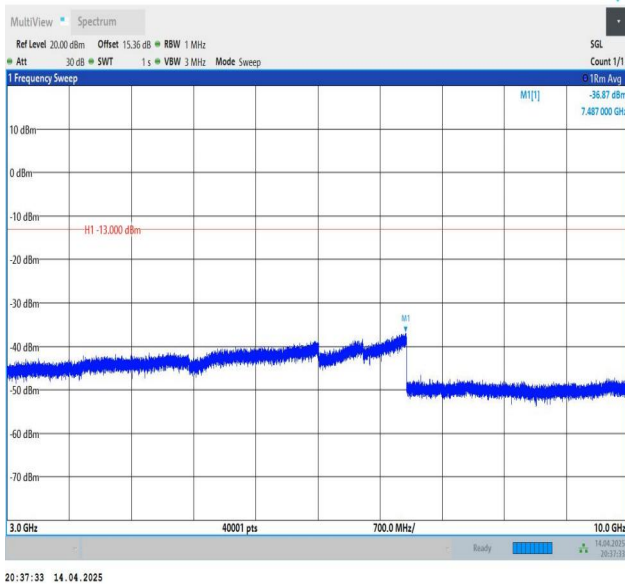
Band26(824-849)-3MHz-QPSK-27025-1RB#0-3000~10000-PASS
