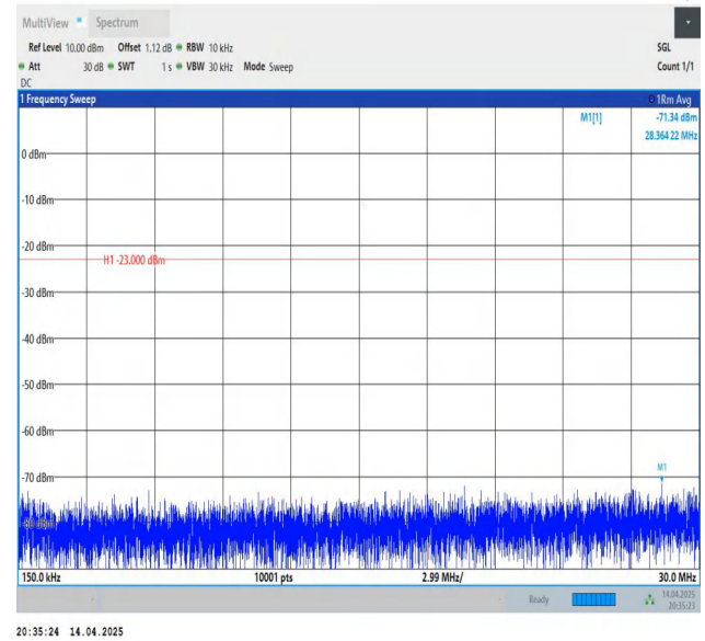
Band26(824-849)-3MHz-QPSK-26805-1RB#0-0.15~30-PASS
