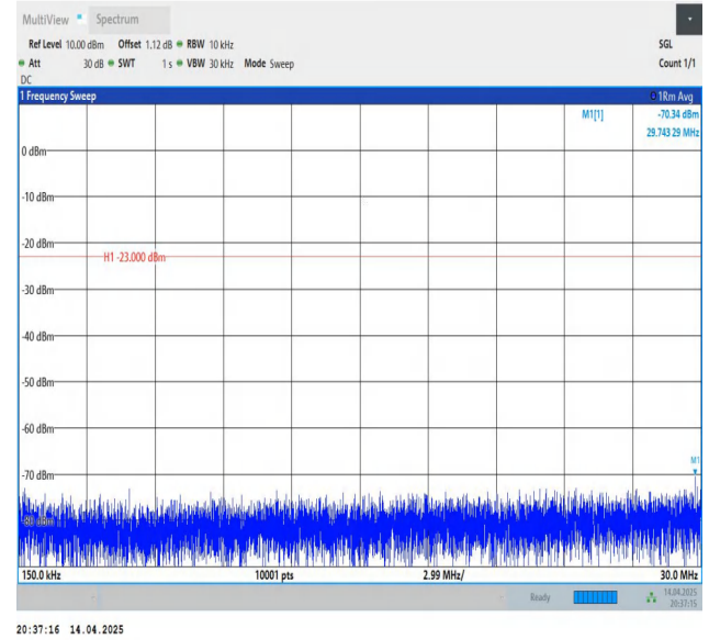
Band26(824-849)-3MHz-QPSK-27025-1RB#0-0.15~30-PASS
