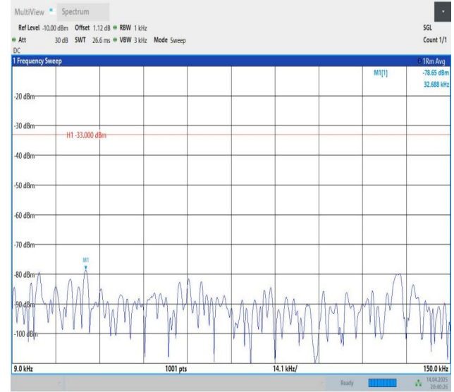
Band26(824-849)-5MHz-QPSK-27015-1RB#24-0.009~0.15-PASS
