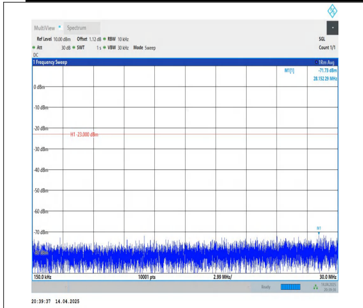
Band26(824-849)-5MHz-QPSK-26915-1RB#24-0.15~30-PASS
