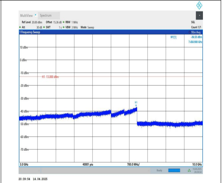
Band26(824-849)-5MHz-QPSK-26915-1RB#24-3000~10000-PASS
