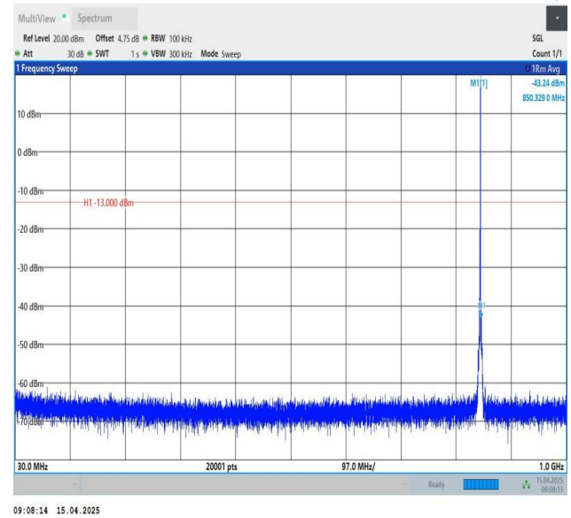
Band26(824-849)-1.4MHz-QPSK-27033-1RB#5-30~1000-PASS
