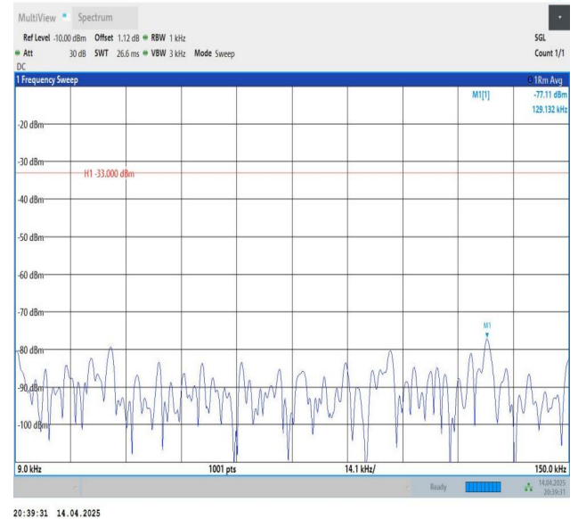
Band26(824-849)-5MHz-QPSK-26915-1RB#24-0.009~0.15-PASS
