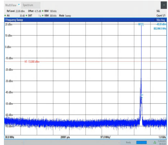
Band26(824-849)-5MHz-QPSK-27015-1RB#24-30~1000-PASS
