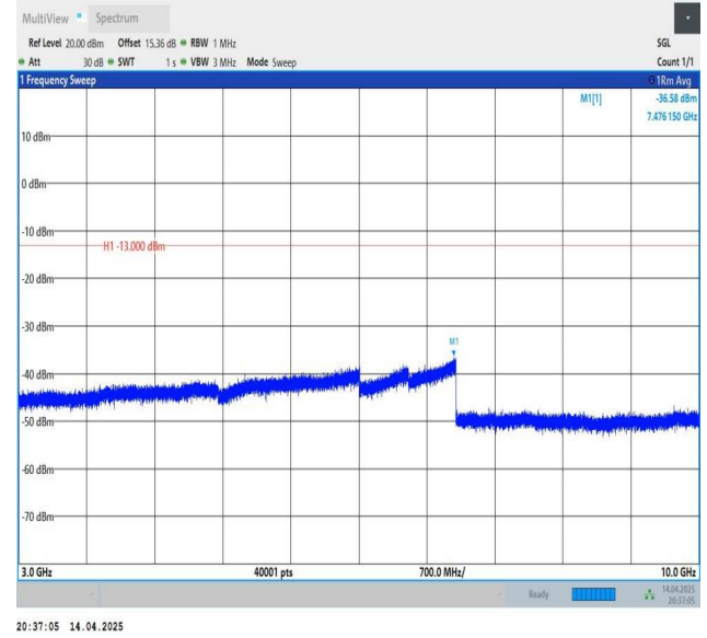
Band26(824-849)-3MHz-QPSK-26915-1RB#14-3000~10000-PASS
