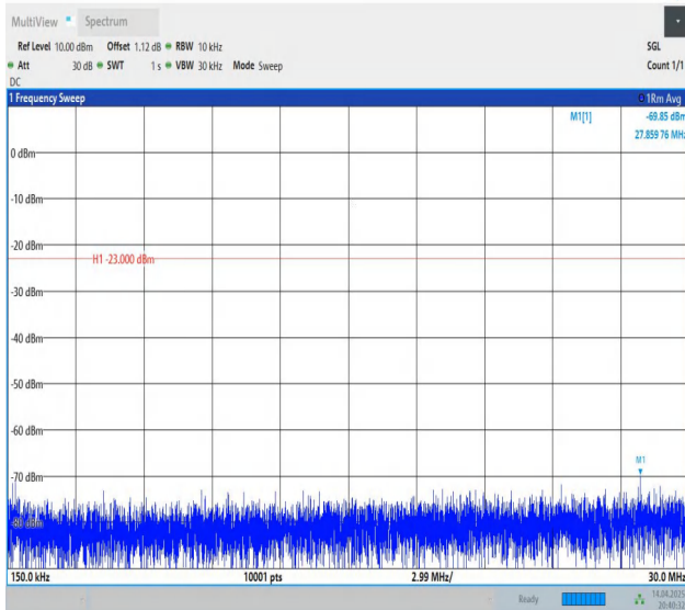
Band26(824-849)-5MHz-QPSK-27015-1RB#24-0.15~30-PASS
