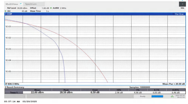
Band26(824-849)-1.4MHz-16QAM-26915-6RB#0-PASS
