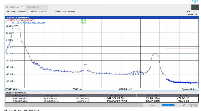
Band26(824-849)-5MHz-QPSK-27015-1RB#0-PASS
