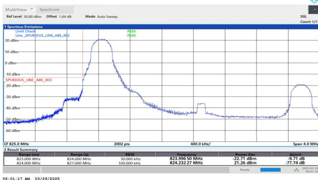
Band26(824-849)-1.4MHz-QPSK-27033-1RB#5-PASS
