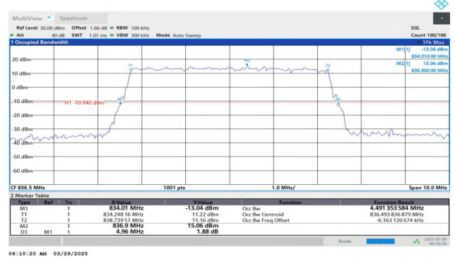
Band26(824-849)-5MHz-16QAM-26915-25RB#0-PASS
