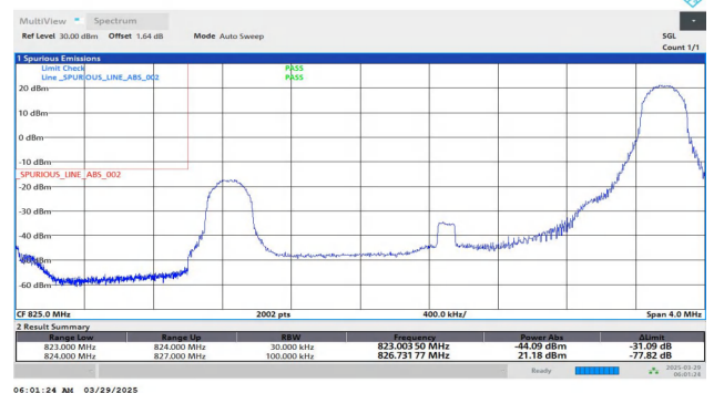
Band26(824-849)-1.4MHz-QPSK-27033-6RB#0-PASS
