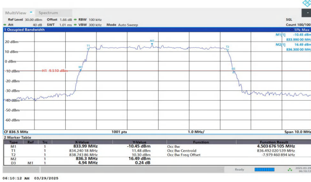
Band26(824-849)-5MHz-QPSK-26915-25RB#0-PASS
