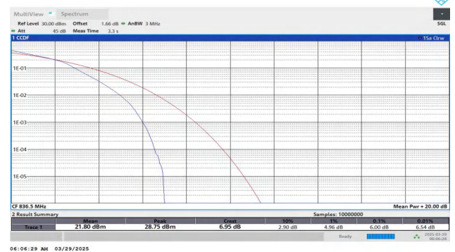
Band26(824-849)-3MHz-16QAM-26915-15RB#0-PASS
