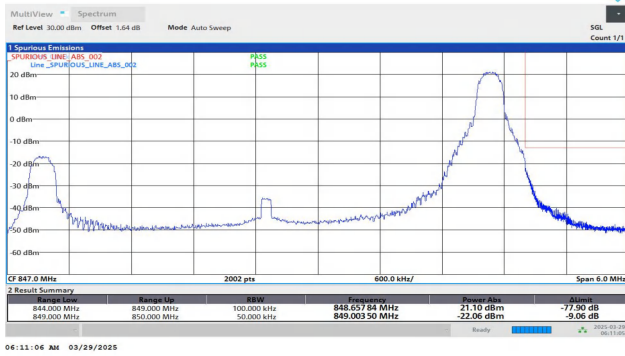
Band26(824-849)-5MHz-QPSK-27015-1RB#24-PASS
