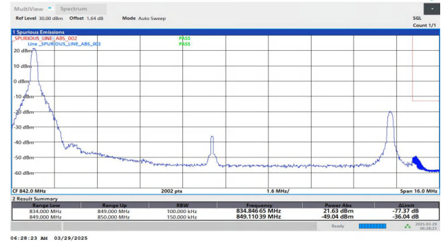
Band26(824-849)-15MHz-QPSK-26965-1RB#0-PASS
