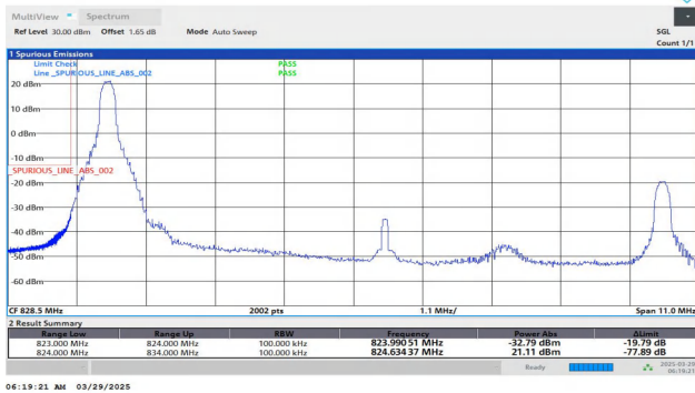
Band26(824-849)-10MHz-QPSK-26840-1RB#0-PASS
