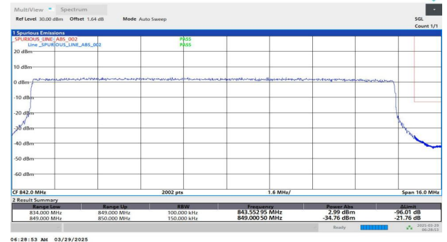
Band26(824-849)-15MHz-QPSK-26965-75RB#0-PASS
