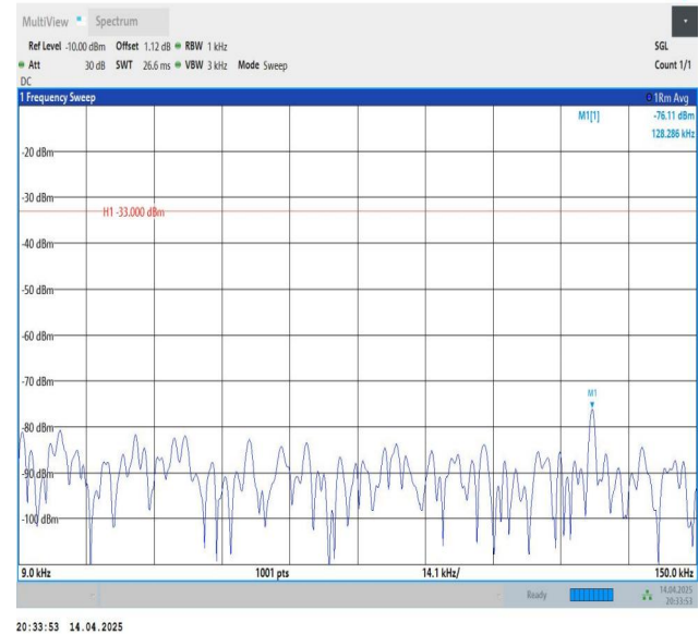
Band26(824-849)-1.4MHz-QPSK-26915-1RB#5-0.009~0.15-PASS
