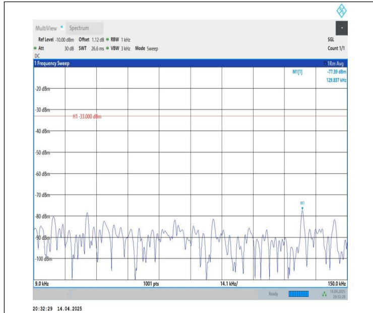
Band26(824-849)-1.4MHz-QPSK-26797-1RB#0-0.009~0.15-PASS
