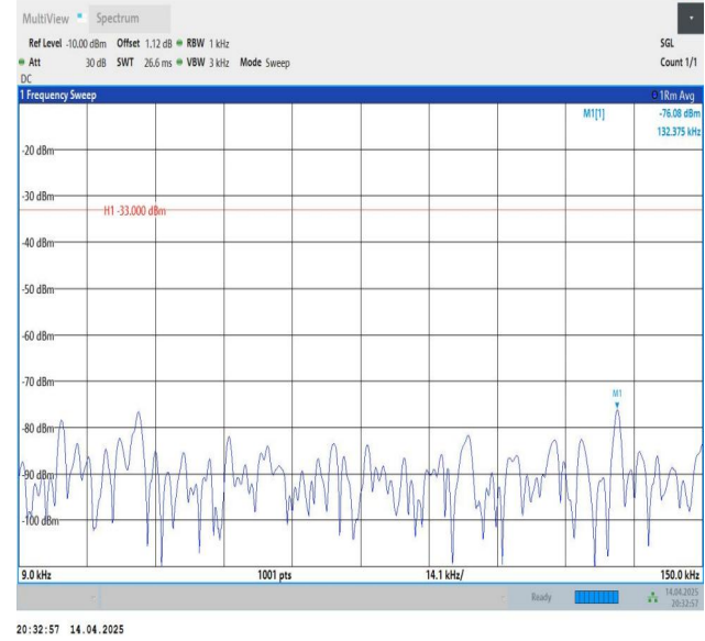
Band26(824-849)-1.4MHz-QPSK-26797-1RB#5-0.009~0.15-PASS
