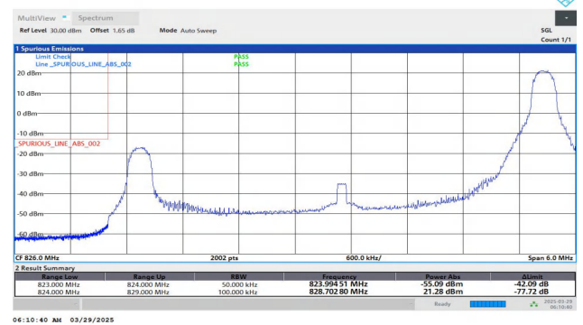
Band26(824-849)-5MHz-QPSK-26815-1RB#24-PASS
