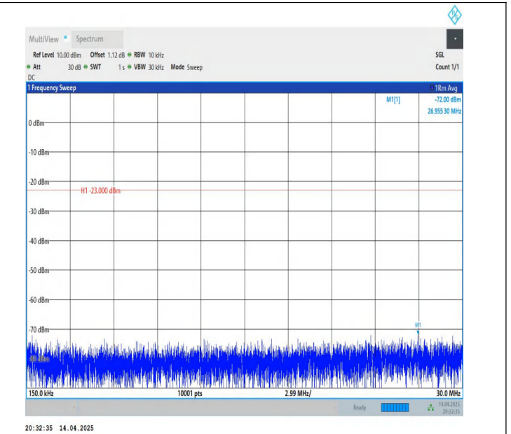
Band26(824-849)-1.4MHz-QPSK-26797-1RB#0-0.15~30-PASS
