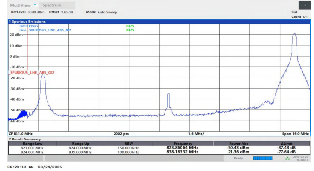
Band26(824-849)-15MHz-QPSK-26865-1RB#74-PASS
