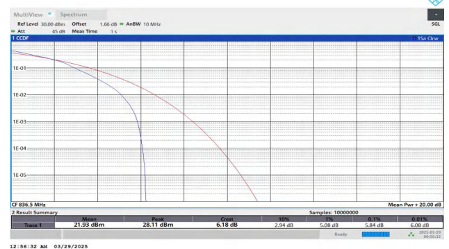
Band26(824-849)-10MHz-16QAM-26915-27RB#0-PASS
