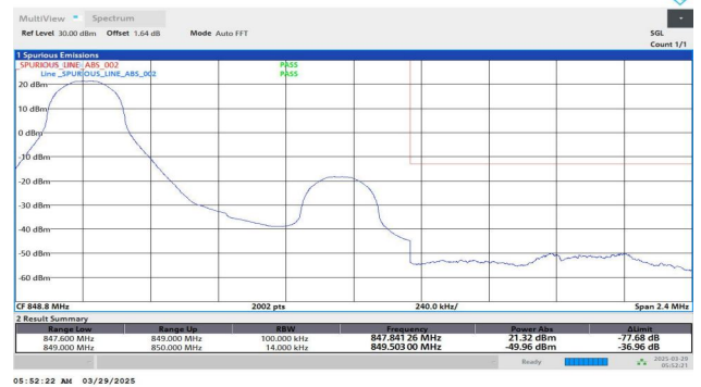
Band26(824-849)-1.4MHz-QPSK-27033-1RB#0-PASS
