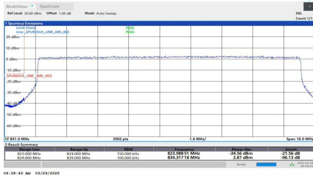
Band26(824-849)-15MHz-QPSK-26865-75RB#0-PASS
