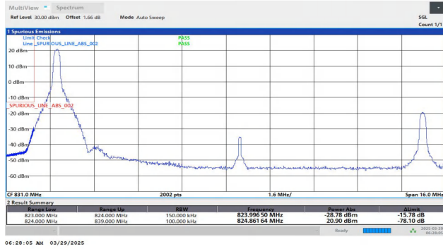
Band26(824-849)-15MHz-QPSK-26865-1RB#0-PASS
