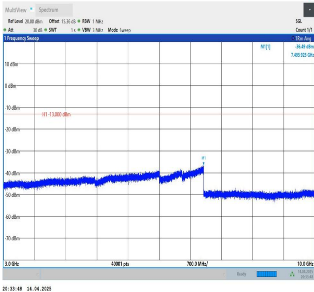
Band26(824-849)-1.4MHz-QPSK-26915-1RB#0-3000~10000-PASS
