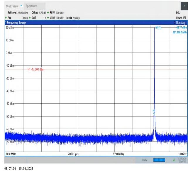
Band26(824-849)-1.4MHz-QPSK-26797-1RB#5-30~1000-PASS
