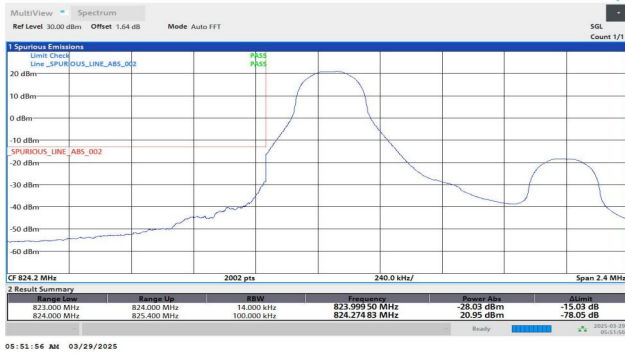
Band26(824-849)-1.4MHz-QPSK-26797-1RB#0-PASS
