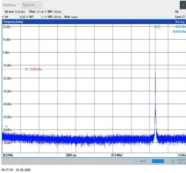
Band26(824-849)-1.4MHz-QPSK-26915-1RB#0-30~1000-PASS
