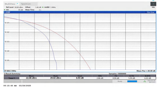
Band26(824-849)-5MHz-16QAM-26915-25RB#0-PASS
