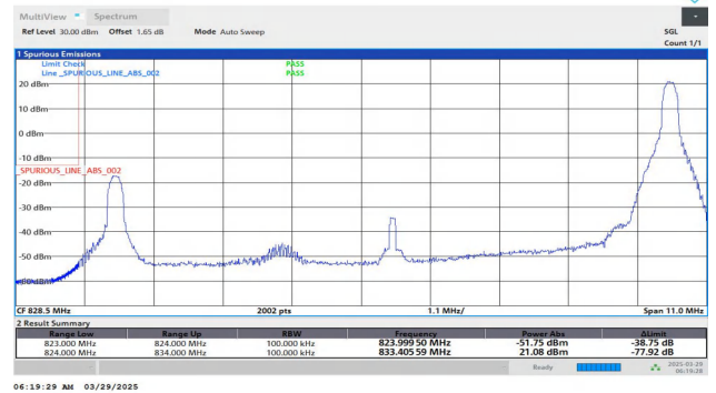
Band26(824-849)-10MHz-QPSK-26840-1RB#49-PASS
