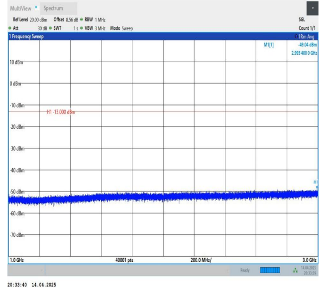
Band26(824-849)-1.4MHz-QPSK-26915-1RB#0-1000~3000-PASS
