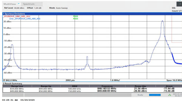
Band26(824-849)-15MHz-QPSK-26965-1RB#74-PASS
