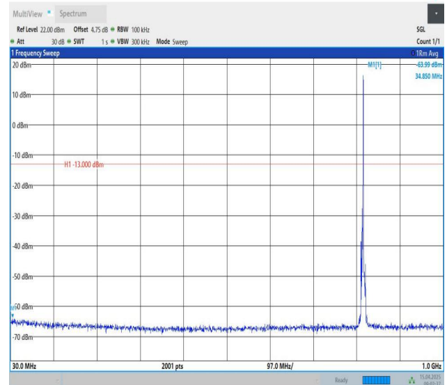
Band26(814-824)-3MHz-QPSK-26740-1RB#14-30~1000-PASS
