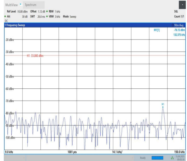
Band26(814-824)-3MHz-QPSK-26740-1RB#14-0.009~0.15-PASS
