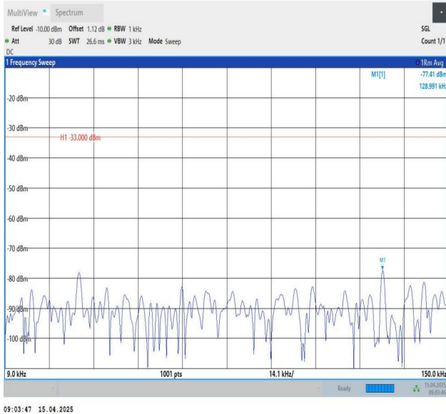
Band26(814-824)-5MHz-QPSK-26740-1RB#0-0.009~0.15-PASS
