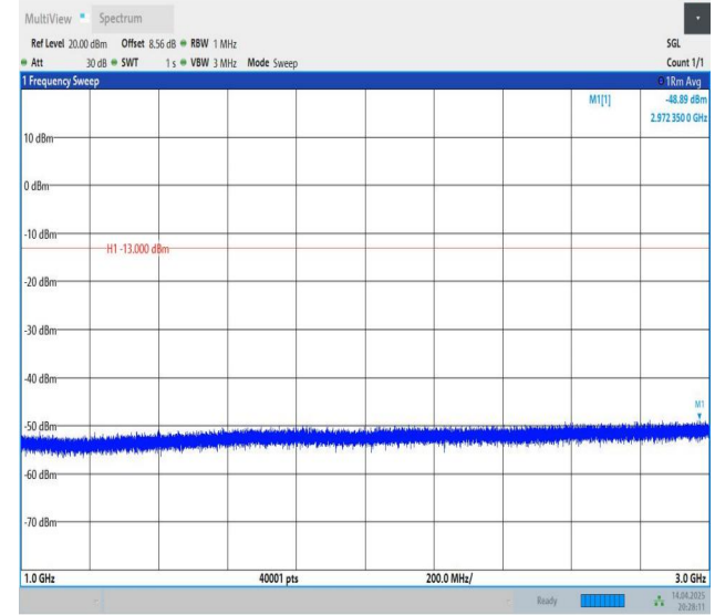
Band26(814-824)-3MHz-QPSK-26775-1RB#0-1000~3000-PASS
