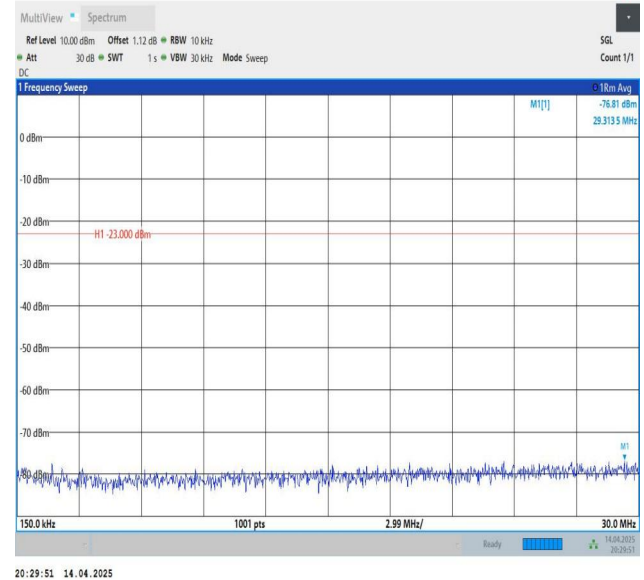
Band26(814-824)-5MHz-QPSK-26740-1RB#0-0.15~30-PASS
