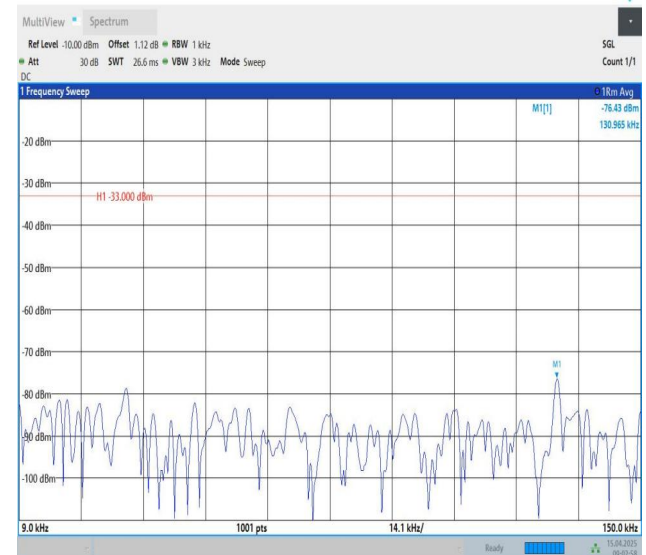
Band26(814-824)-3MHz-QPSK-26775-1RB#14-0.009~0.15-PASS
