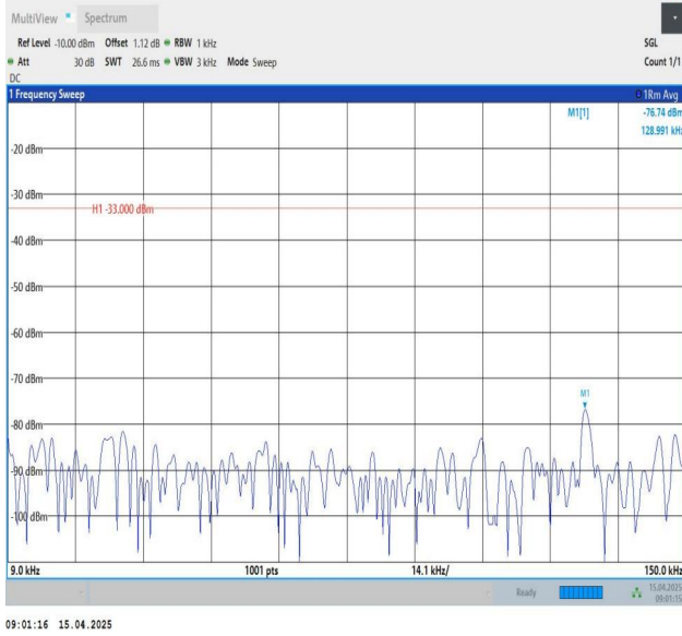
Band26(814-824)-1.4MHz-QPSK-26783-1RB#0-0.009~0.15-PASS
