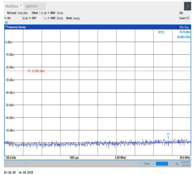
Band26(814-824)-1.4MHz-QPSK-26740-1RB#0-0.15~30-PASS
