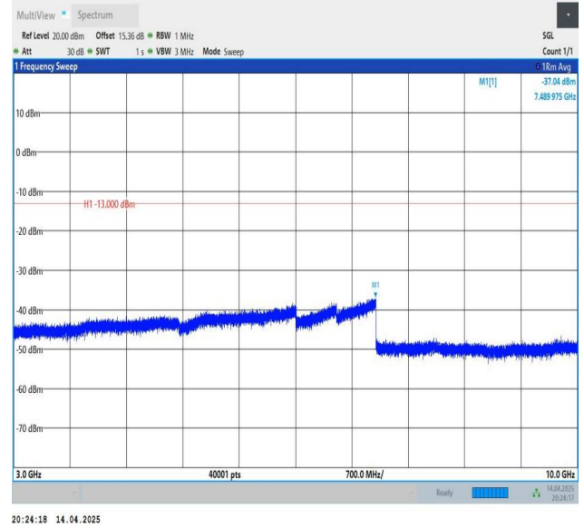
Band26(814-824)-1.4MHz-QPSK-26697-1RB#5-3000~10000-PASS S
