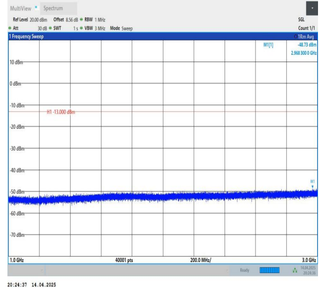
Band26(814-824)-1.4MHz-QPSK-26740-1RB#0-1000~3000-PASS
