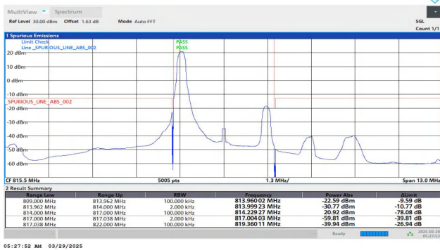
Band26(814-824)-1.4MHz-QPSK-26783-1RB#5-PASS
