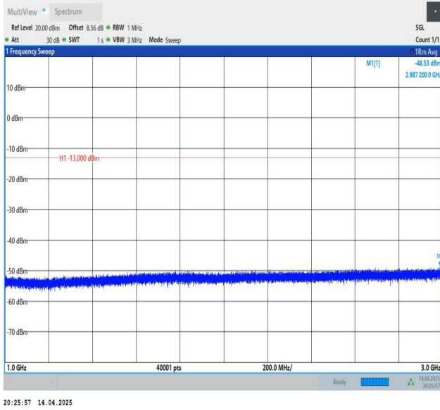
Band26(814-824)-1.4MHz-QPSK-26783-1RB#5-1000~3000-PASS
