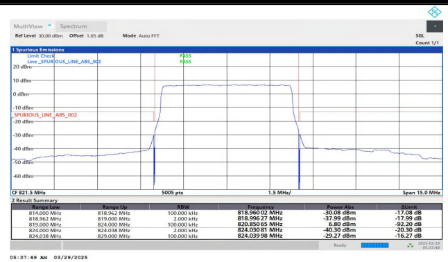
Band26(814-824)-5MHz-QPSK-26765-25RB#0-PASS
