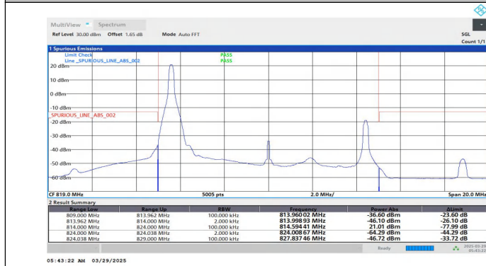
Band26(814-824)-10MHz-QPSK-26740-1RB#0-PASS
