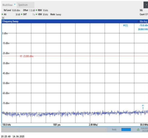
Band26(814-824)-1.4MHz-QPSK-26783-1RB#5-0.15~30-PASS
