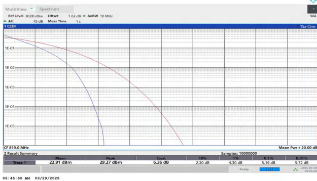
Band26(814-824)-10MHz-QPSK-26740-50RB#0-PASS
