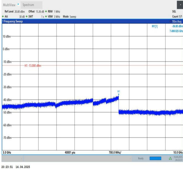
Band26(814-824)-1.4MHz-QPSK-26697-1RB#0-3000~10000-PAS S
