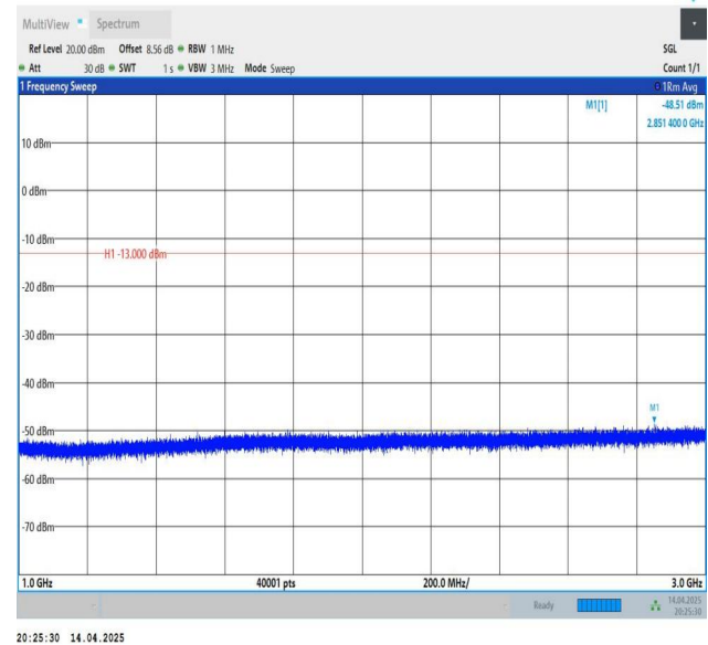
Band26(814-824)-1.4MHz-QPSK-26783-1RB#0-1000~3000-PASS
