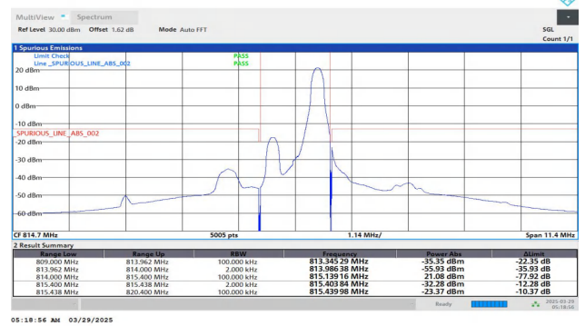
Band26(814-824)-1.4MHz-QPSK-26697-1RB#5-PASS
