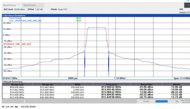
Band26(814-824)-1.4MHz-QPSK-26697-6RB#0-PASS
