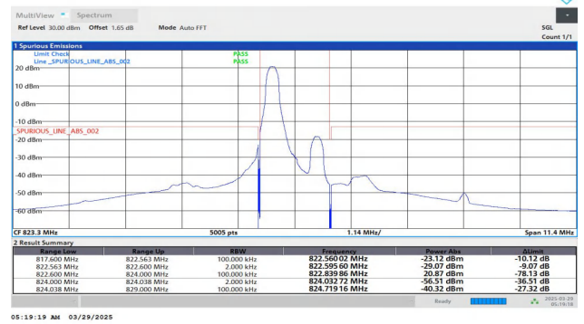
Band26(814-824)-1.4MHz-QPSK-26783-1RB#0-PASS
