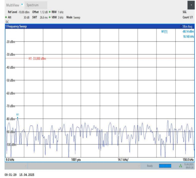
Band26(814-824)-1.4MHz-QPSK-26783-1RB#5-0.009~0.15-PASS
