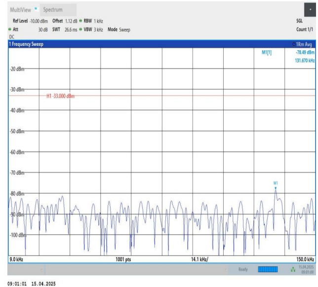
Band26(814-824)-1.4MHz-QPSK-26740-1RB#5-0.009~0.15-PASS
