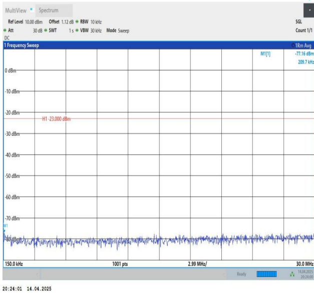
Band26(814-824)-1.4MHz-QPSK-26697-1RB#5-0.15~30-PASS
