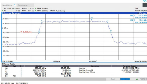
Band26(814-824)-5MHz-QPSK-26740-25RB#0-PASS
