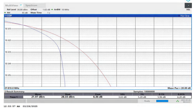
Band26(814-824)-10MHz-16QAM-26740-27RB#0-PASS
