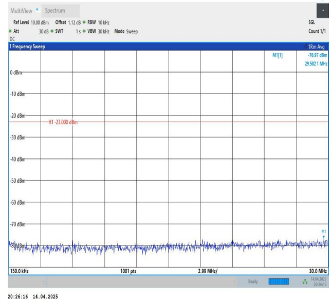
Band26(814-824)-3MHz-QPSK-26705-1RB#0-0.15~30-PASS
