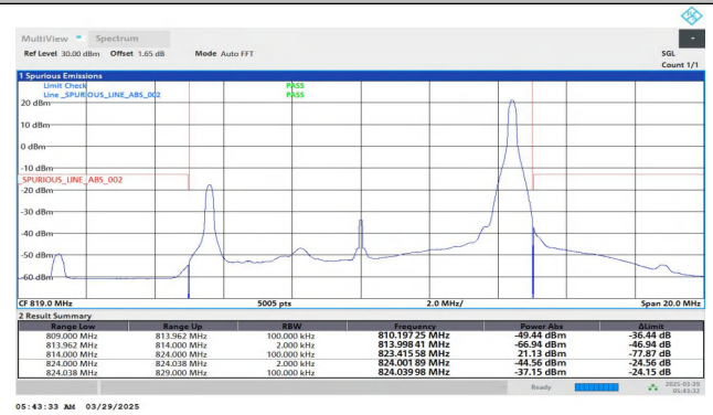
Band26(814-824)-10MHz-QPSK-26740-1RB#49-PASS
