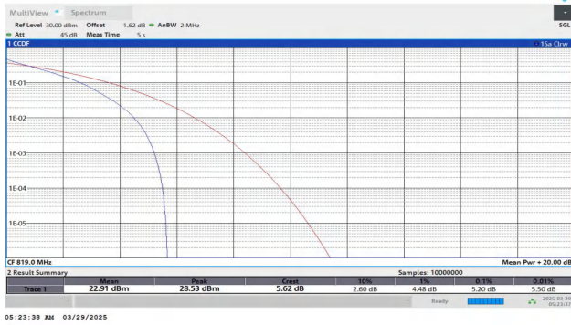
Band26(814-824)-1.4MHz-QPSK-26740-6RB#0-PASS
