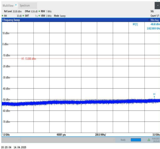
Band26(814-824)-1.4MHz-QPSK-26740-1RB#5-1000~3000-PASS
