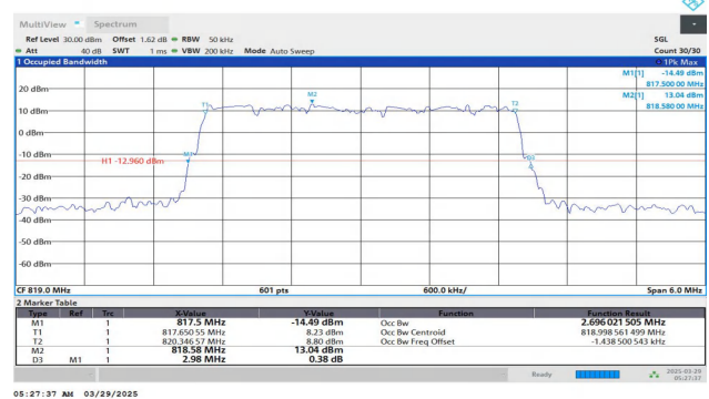
Band26(814-824)-3MHz-16QAM-26740-15RB#0-PASS
