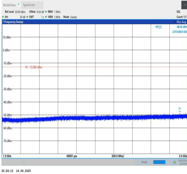
Band26(814-824)-1.4MHz-QPSK-26697-1RB#5-1000~3000-PASS
