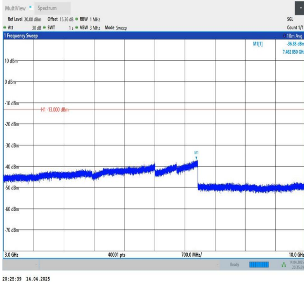
Band26(814-824)-1.4MHz-QPSK-26783-1RB#0-3000~10000-PAS S
