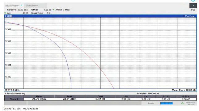
Band26(814-824)-3MHz-16QAM-26740-15RB#0-PASS
