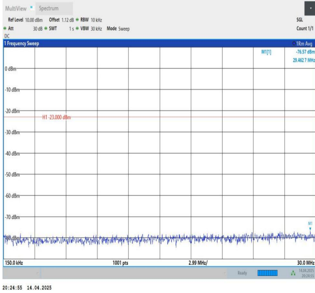
Band26(814-824)-1.4MHz-QPSK-26740-1RB#5-0.15~30-PASS
