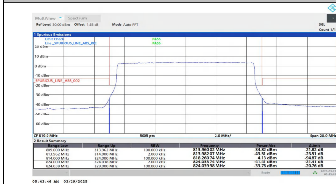
Band26(814-824)-10MHz-QPSK-26740-50RB#0-PASS
