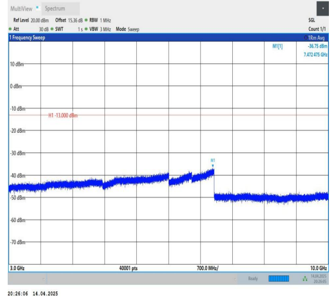
Band26(814-824)-1.4MHz-QPSK-26783-1RB#5-3000~10000-PASS S
