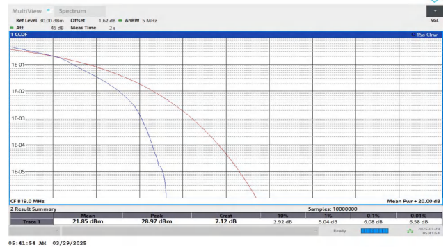
Band26(814-824)-5MHz-16QAM-26740-25RB#0-PASS
