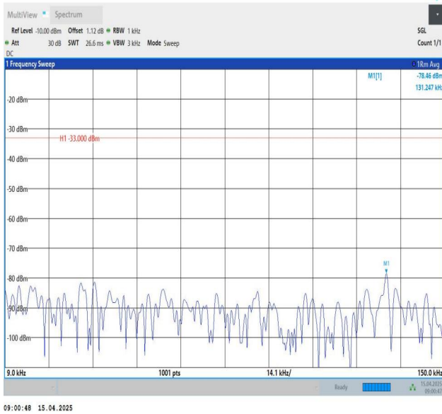
Band26(814-824)-1.4MHz-QPSK-26740-1RB#0-0.009~0.15-PASS
