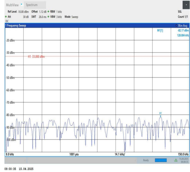
Band26(814-824)-1.4MHz-QPSK-26697-1RB#5-0.009~0.15-PASS
