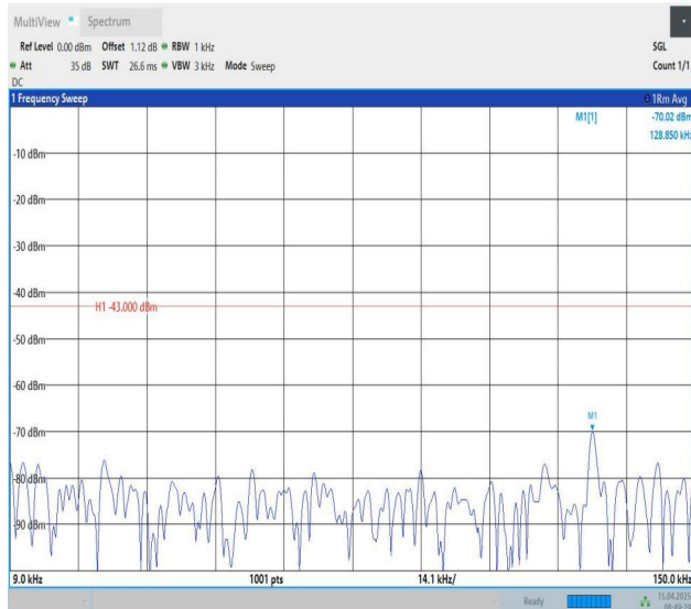
Band25-10MHz-QPSK-26640-1RB#0-0.009~0.15-PASS
