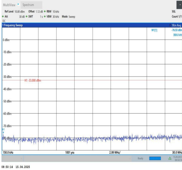
Band25-10MHz-QPSK-26640-1RB#49-0.15~30-PASS
