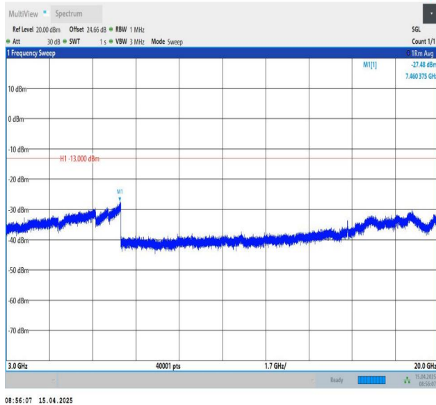
Band25-20MHz-QPSK-26140-1RB#0-3000~20000-PASS
