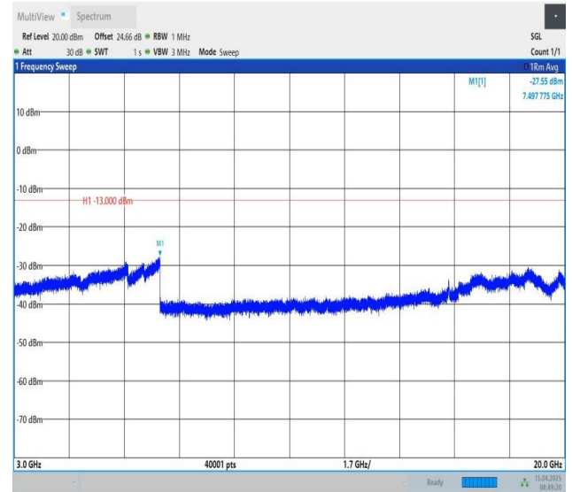
Band25-10MHz-QPSK-26365-1RB#49-3000~20000-PASS
