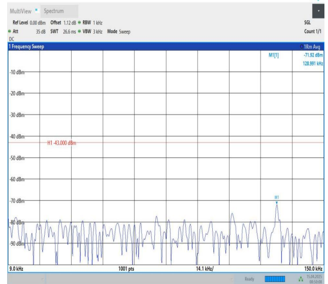
Band25-10MHz-QPSK-26640-1RB#49-0.009~0.15-PASS
