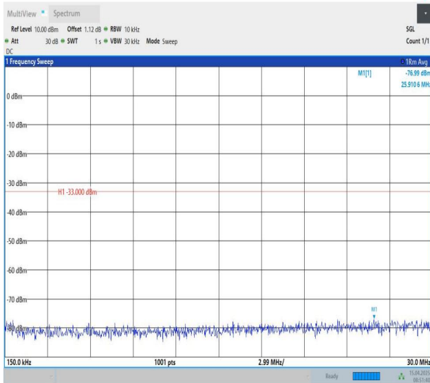
Band25-15MHz-QPSK-26115-1RB#74-0.15~30-PASS
