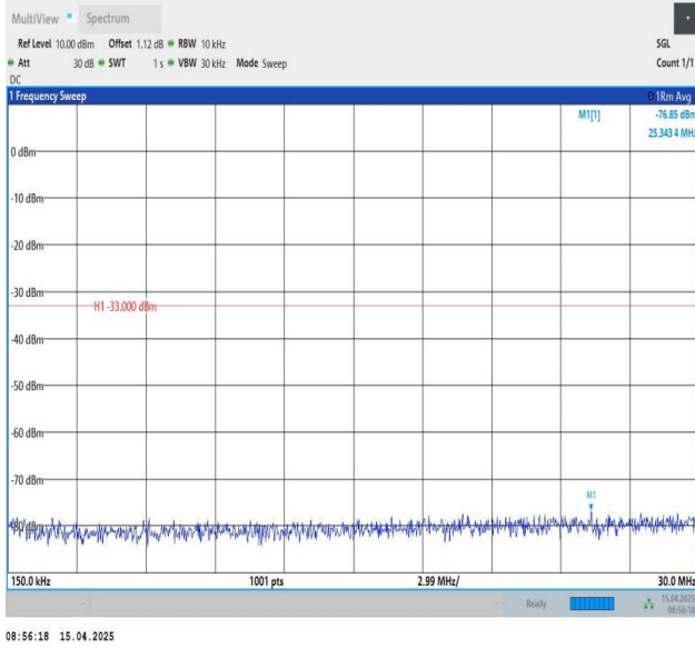
Band25-20MHz-QPSK-26140-1RB#99-0.15~30-PASS
