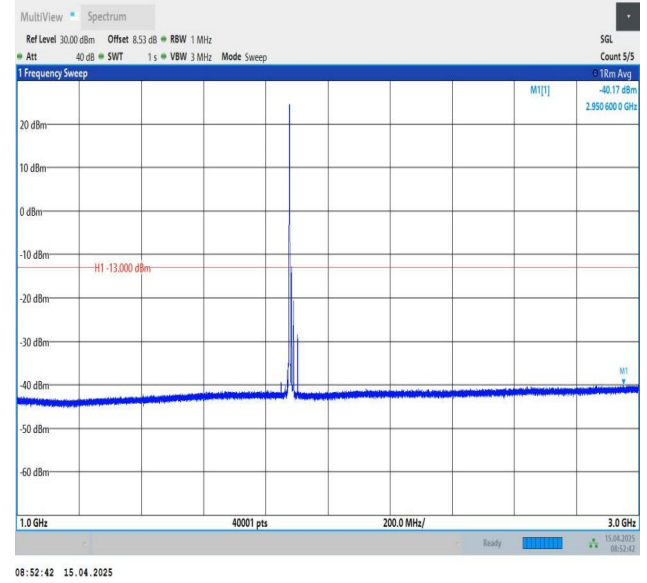
Band25-15MHz-QPSK-26365-1RB#0-1000~3000-PASS
