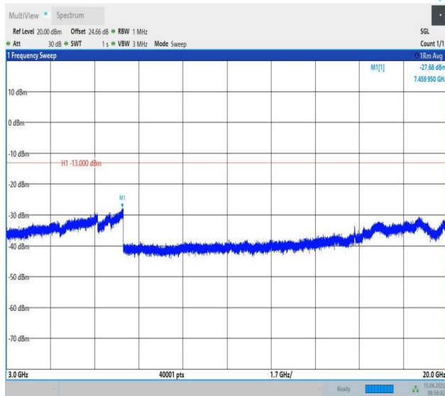
Band25-10MHz-QPSK-26640-1RB#0-3000~20000-PASS
