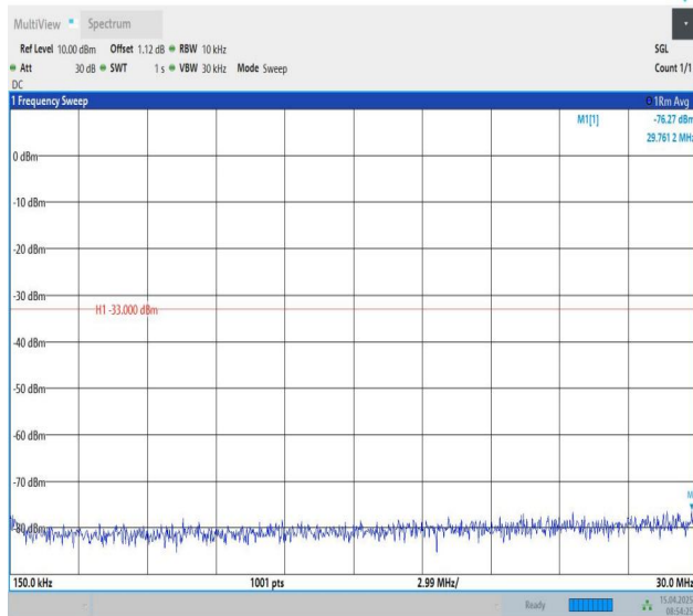
Band25-15MHz-QPSK-26615-1RB#74-0.15~30-PASS
