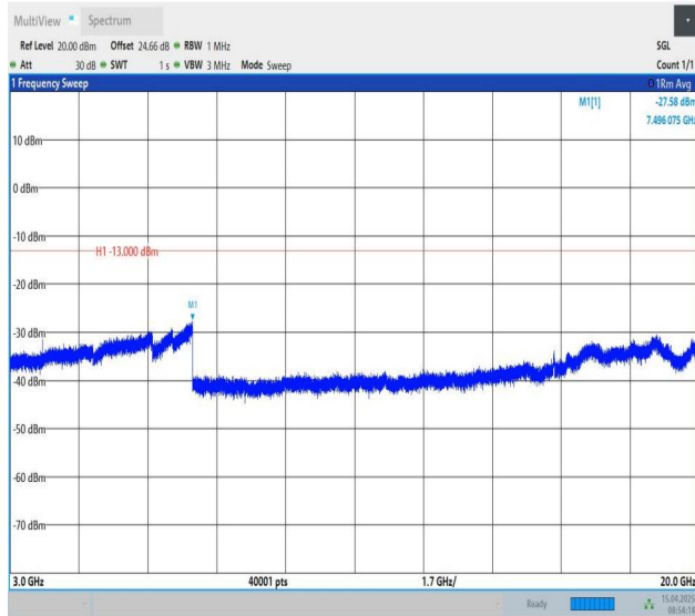
Band25-15MHz-QPSK-26615-1RB#0-3000~20000-PASS
