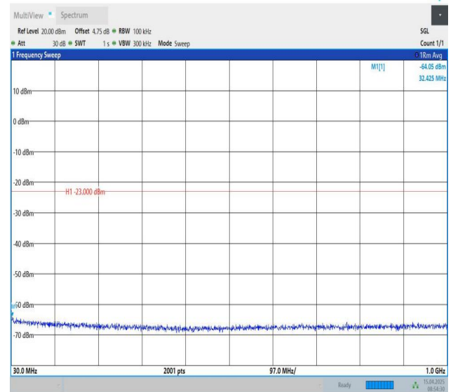
Band25-15MHz-QPSK-26615-1RB#74-30~1000-PASS
