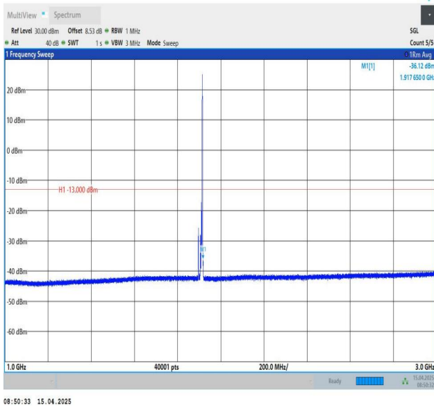
Band25-10MHz-QPSK-26640-1RB#49-1000~3000-PASS
