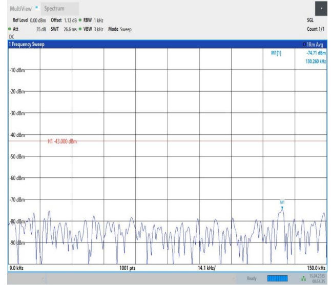
Band25-15MHz-QPSK-26115-1RB#74-0.009~0.15-PASS
