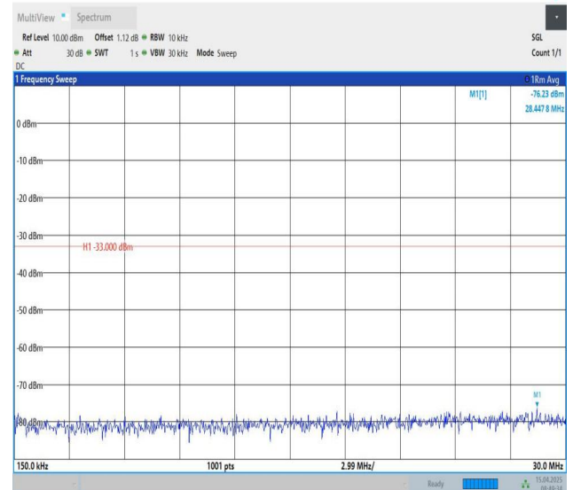
Band25-10MHz-QPSK-26640-1RB#0-0.15~30-PASS
