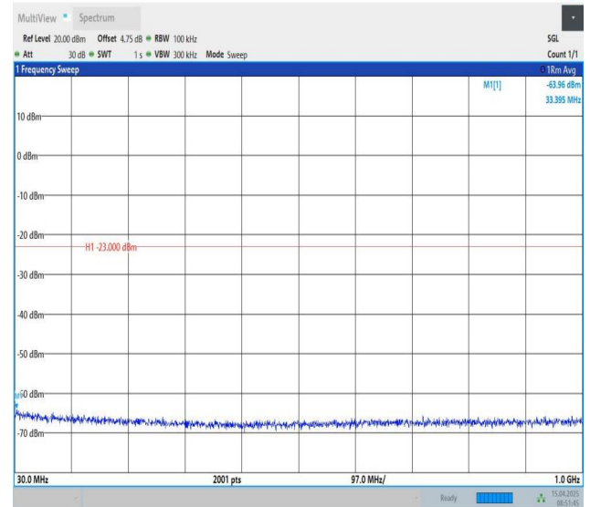
Band25-15MHz-QPSK-26115-1RB#74-30~1000-PASS
