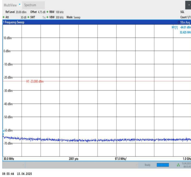
Band25-20MHz-QPSK-26140-1RB#0-30~1000-PASS
