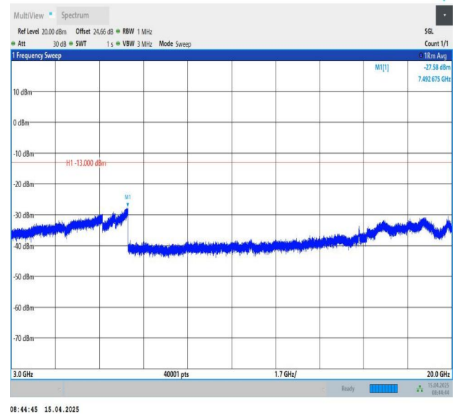
Band25-5MHz-QPSK-26365-1RB#24-3000~20000-PASS
