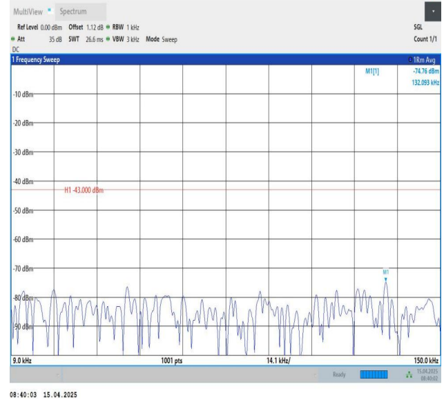
Band25-3MHz-QPSK-26365-1RB#14-0.009~0.15-PASS
