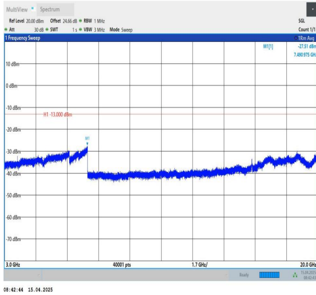
Band25-5MHz-QPSK-26065-1RB#0-3000~20000-PASS
