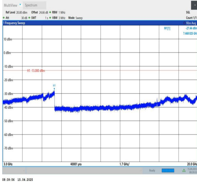
Band25-3MHz-QPSK-26365-1RB#0-3000~20000-PASS
