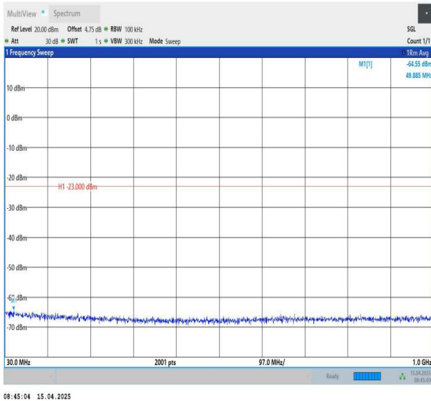
Band25-5MHz-QPSK-26665-1RB#0-30~1000-PASS
