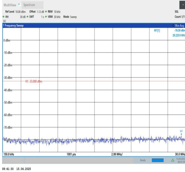
Band25-3MHz-QPSK-26675-1RB#14-0.15~30-PASS
