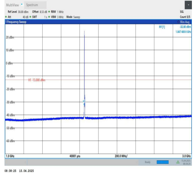
Band25-3MHz-QPSK-26055-1RB#0-1000~3000-PASS
