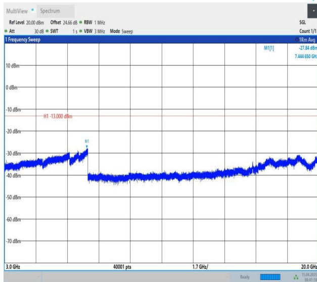
Band25-3MHz-QPSK-26675-1RB#0-3000~20000-PASS
