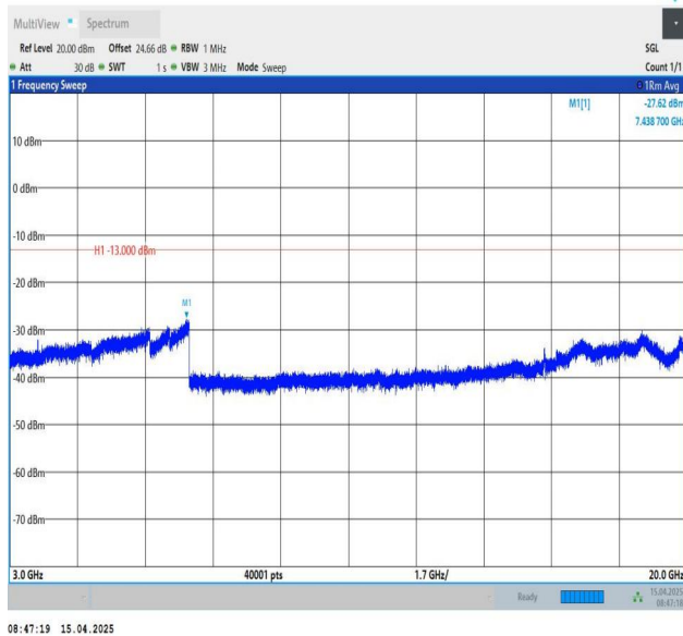
Band25-10MHz-QPSK-26090-1RB#0-3000~20000-PASS
