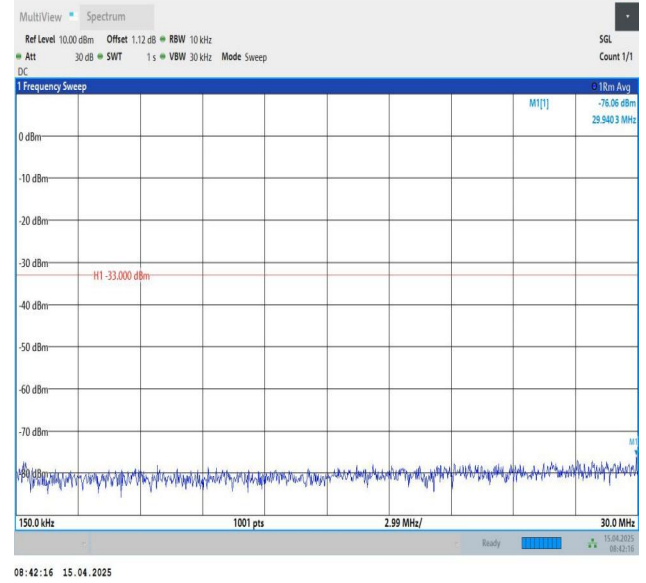
Band25-5MHz-QPSK-26065-1RB#0-0.15~30-PASS
