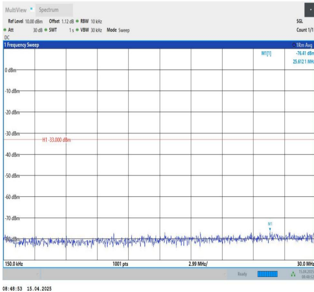
Band25-10MHz-QPSK-26365-1RB#49-0.15~30-PASS
