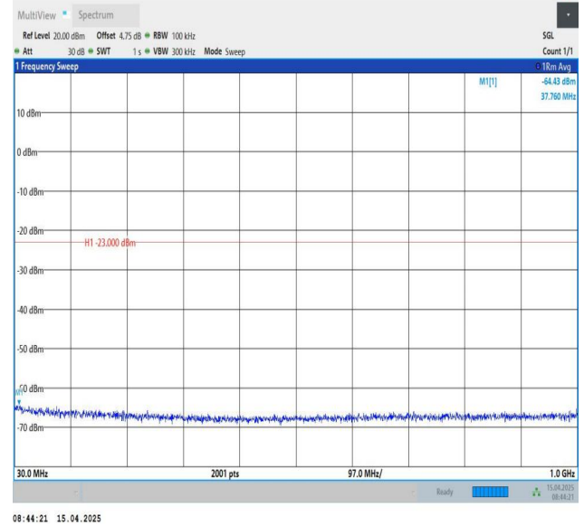
Band25-5MHz-QPSK-26365-1RB#24-30~1000-PASS
