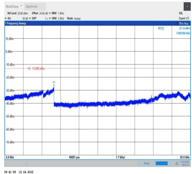
Band25-3MHz-QPSK-26675-1RB#14-3000~20000-PASS
