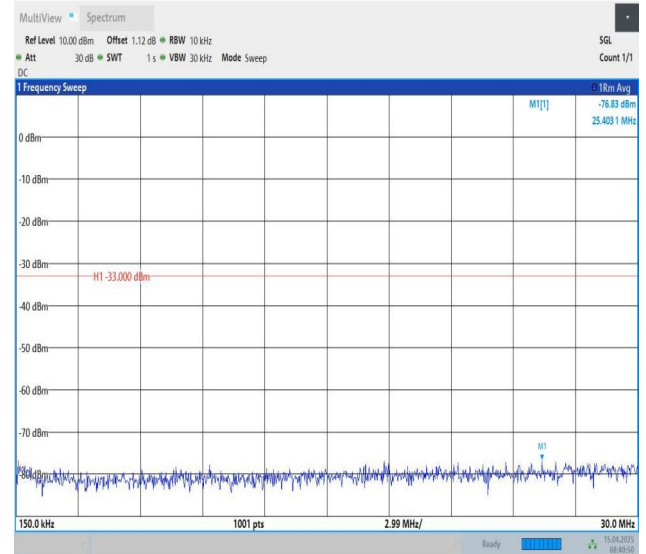
Band25-3MHz-QPSK-26675-1RB#0-0.15~30-PASS
