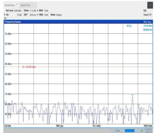
Band25-5MHz-QPSK-26365-1RB#24-0.009~0.15-PASS
