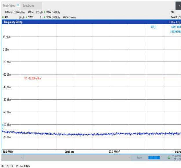
Band25-3MHz-QPSK-26365-1RB#0-30~1000-PASS
