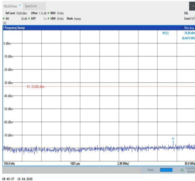
Band25-3MHz-QPSK-26365-1RB#14-0.15~30-PASS
