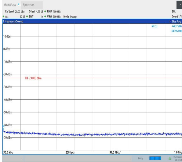
Band25-3MHz-QPSK-26675-1RB#0-30~1000-PASS
