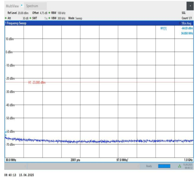
Band25-3MHz-QPSK-26365-1RB#14-30~1000-PASS
