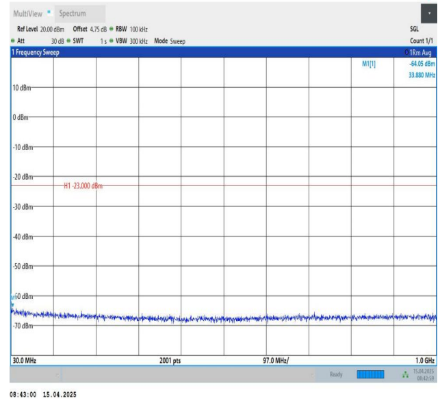
Band25-5MHz-QPSK-26065-1RB#24-30~1000-PASS
