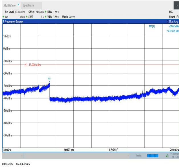
Band25-5MHz-QPSK-26665-1RB#0-3000~20000-PASS
