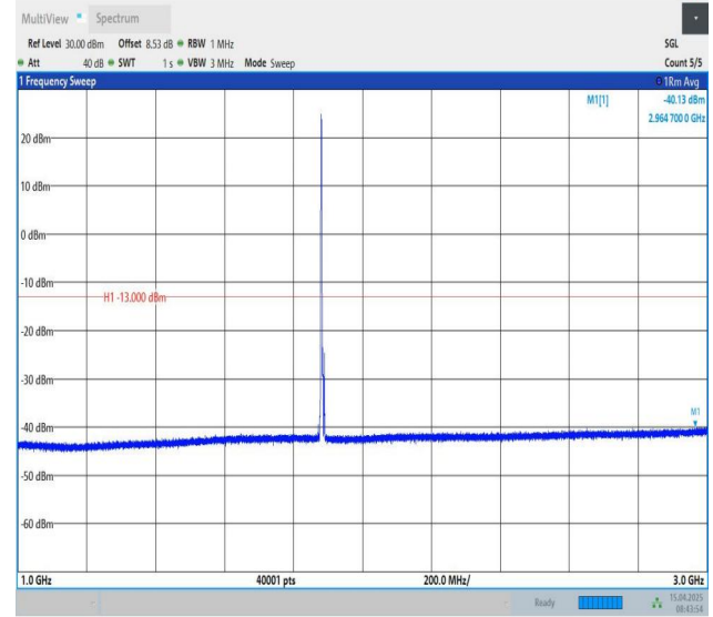
Band25-5MHz-QPSK-26365-1RB#0-1000~3000-PASS
