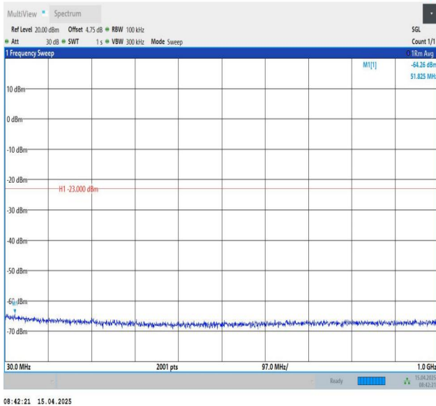
Band25-5MHz-QPSK-26065-1RB#0-30~1000-PASS
