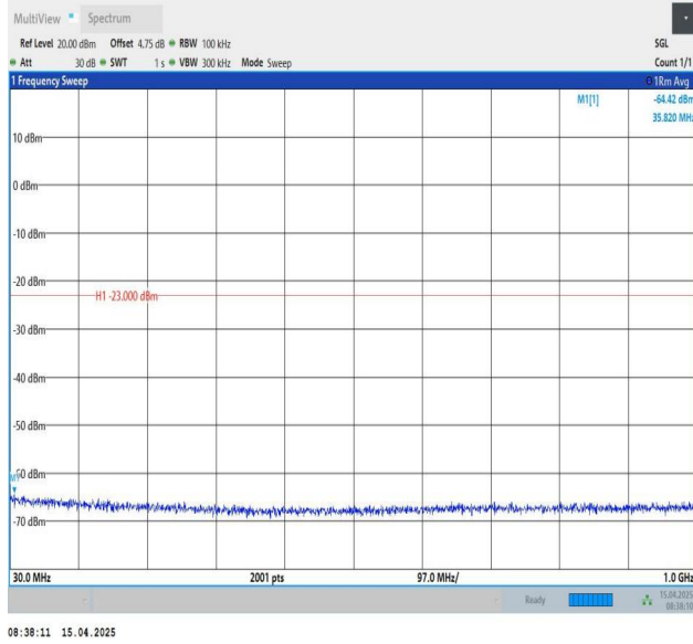
Band25-3MHz-QPSK-26055-1RB#0-30~1000-PASS
