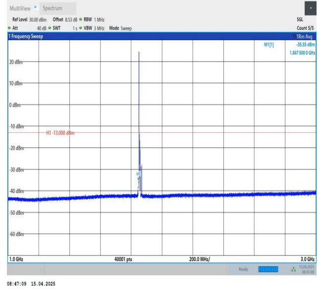
Band25-10MHz-QPSK-26090-1RB#0-1000~3000-PASS
