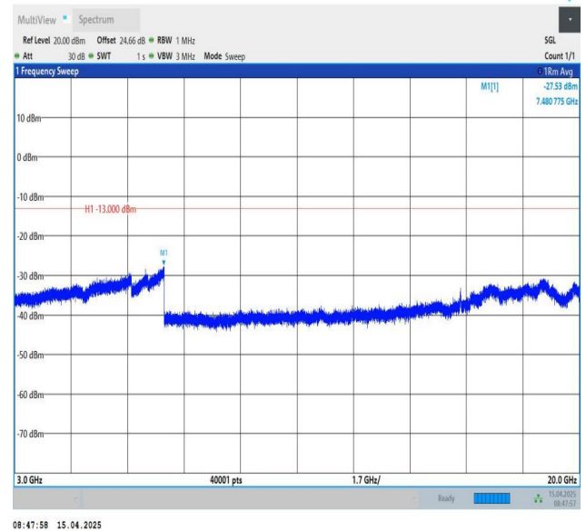
Band25-10MHz-QPSK-26090-1RB#49-3000~20000-PASS
