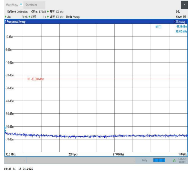
Band25-3MHz-QPSK-26055-1RB#14-30~1000-PASS
