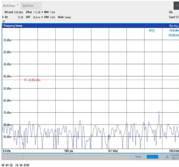
Band25-5MHz-QPSK-26365-1RB#0-0.009~0.15-PASS
