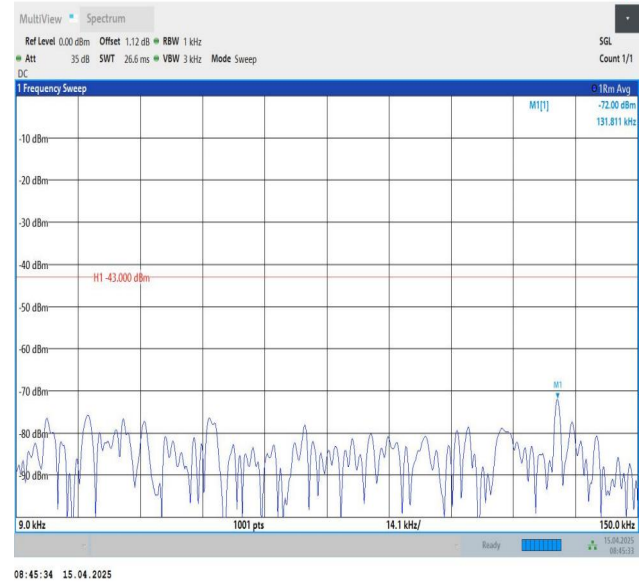
Band25-5MHz-QPSK-26665-1RB#24-0.009~0.15-PASS
