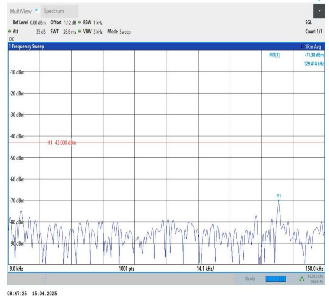
Band25-10MHz-QPSK-26090-1RB#49-0.009~0.15-PASS
