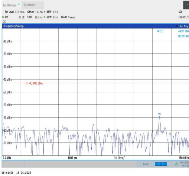
Band25-5MHz-QPSK-26665-1RB#0-0.009~0.15-PASS
