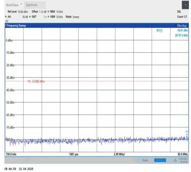
Band25-5MHz-QPSK-26665-1RB#0-0.15~30-PASS
