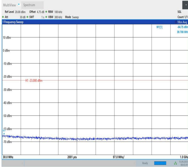
Band25-5MHz-QPSK-26365-1RB#0-30~1000-PASS
