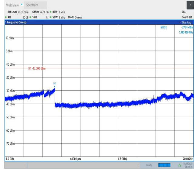
Band25-3MHz-QPSK-26365-1RB#14-3000~20000-PASS
