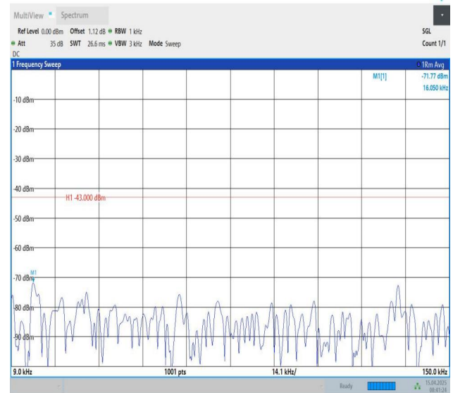
Band25-3MHz-QPSK-26675-1RB#14-0.009~0.15-PASS
