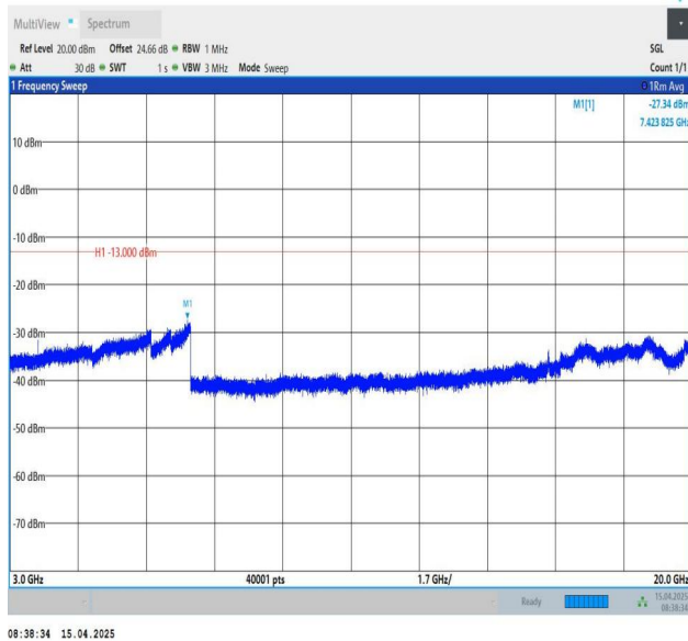
Band25-3MHz-QPSK-26055-1RB#0-3000~20000-PASS
