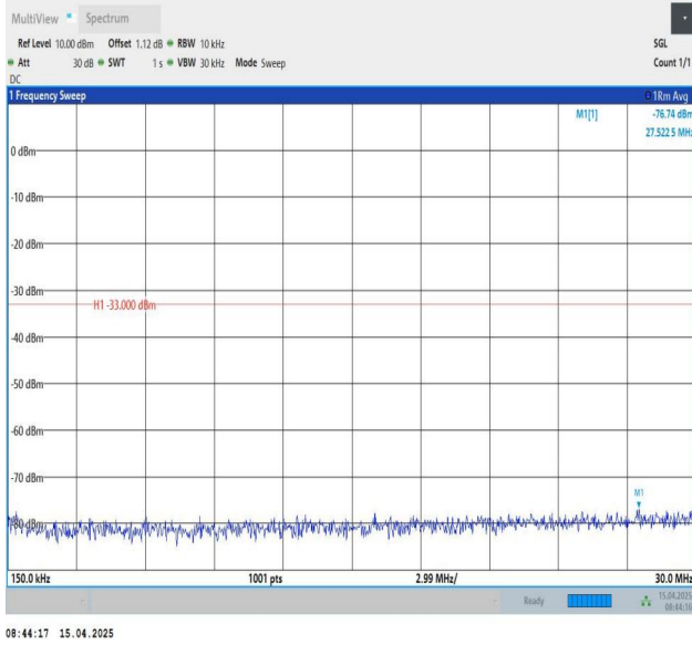
Band25-5MHz-QPSK-26365-1RB#24-0.15~30-PASS
