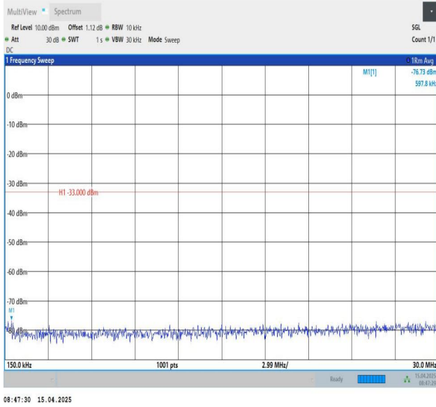
Band25-10MHz-QPSK-26090-1RB#49-0.15~30-PASS
