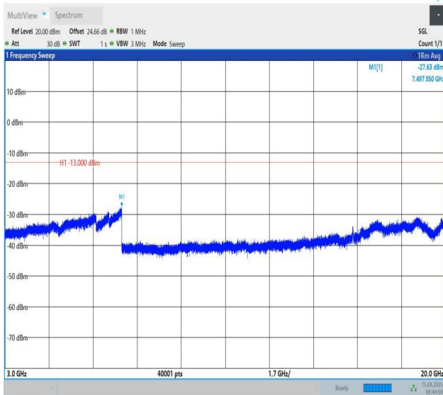
Band25-5MHz-QPSK-26365-1RB#0-3000~20000-PASS
