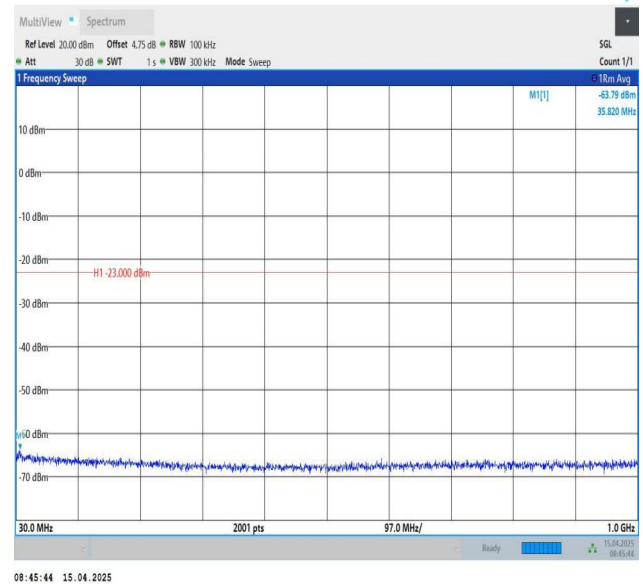
Band25-5MHz-QPSK-26665-1RB#24-30~1000-PASS
