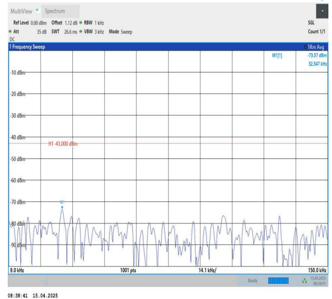
Band25-3MHz-QPSK-26055-1RB#14-0.009~0.15-PASS
