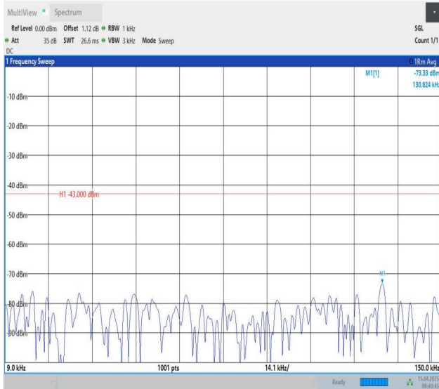
Band25-3MHz-QPSK-26675-1RB#0-0.009~0.15-PASS
