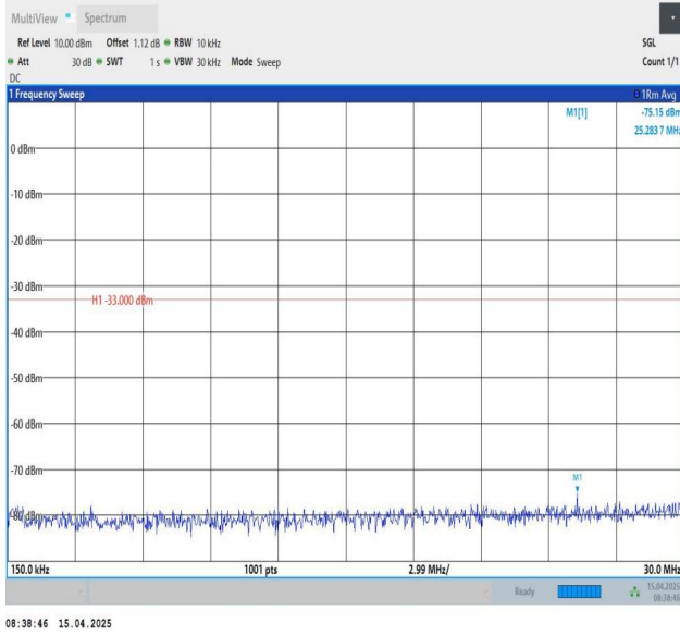
Band25-3MHz-QPSK-26055-1RB#14-0.15~30-PASS
