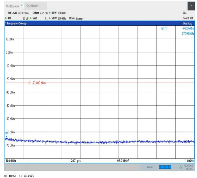
Band25-10MHz-QPSK-26365-1RB#49-30~1000-PASS
