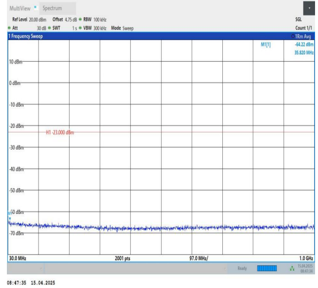
Band25-10MHz-QPSK-26090-1RB#49-30~1000-PASS
