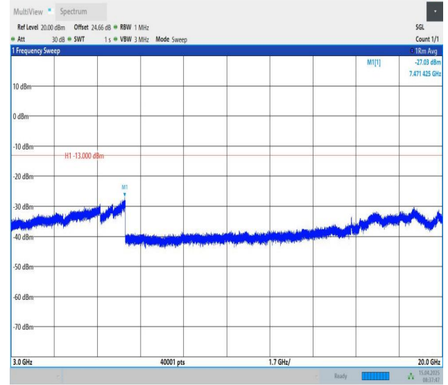
Band25-1.4MHz-QPSK-26683-1RB#5-3000~20000-PASS
