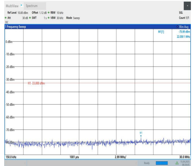
Band25-3MHz-QPSK-26055-1RB#0-0.15~30-PASS
