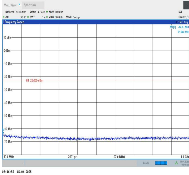
Band25-10MHz-QPSK-26090-1RB#0-30~1000-PASS
