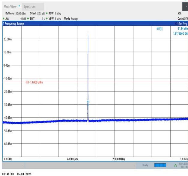
Band25-3MHz-QPSK-26675-1RB#14-1000~3000-PASS
