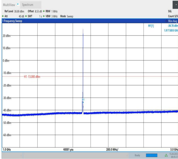
Band25-5MHz-QPSK-26665-1RB#24-1000~3000-PASS
