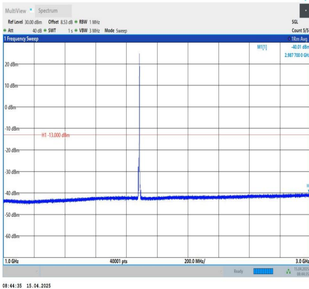
Band25-5MHz-QPSK-26365-1RB#24-1000~3000-PASS
