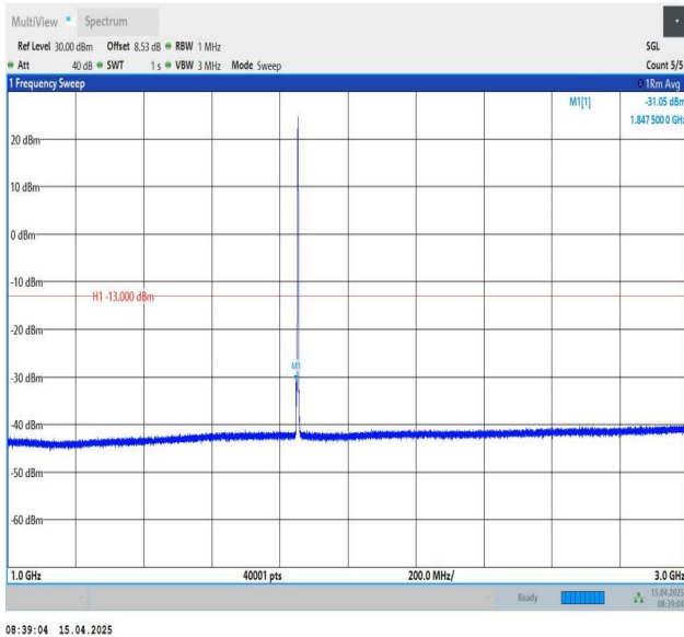
Band25-3MHz-QPSK-26055-1RB#14-1000~3000-PASS
