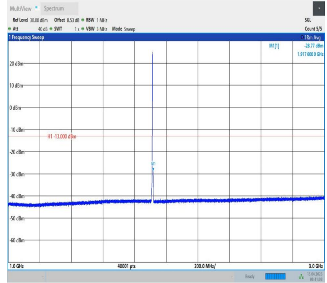
Band25-3MHz-QPSK-26675-1RB#0-1000~3000-PASS
