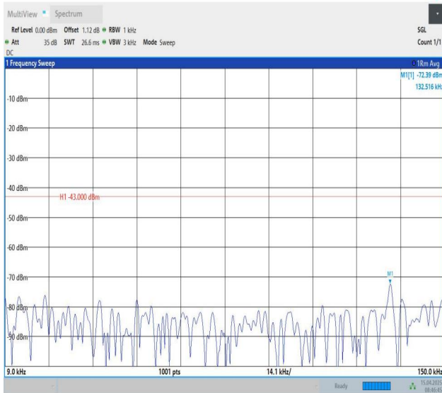
Band25-10MHz-QPSK-26090-1RB#0-0.009~0.15-PASS
