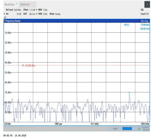
Band25-5MHz-QPSK-26065-1RB#24-0.009~0.15-PASS
