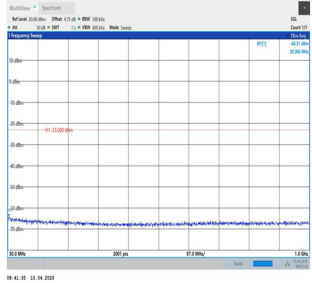
Band25-3MHz-QPSK-26675-1RB#14-30~1000-PASS
