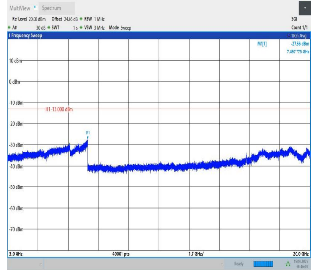
Band25-5MHz-QPSK-26665-1RB#24-3000~20000-PASS
