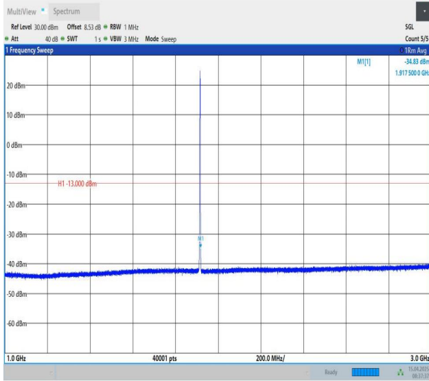
Band25-1.4MHz-QPSK-26683-1RB#5-1000~3000-PASS
