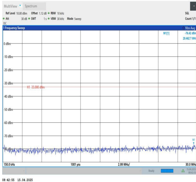
Band25-5MHz-QPSK-26065-1RB#24-0.15~30-PASS
