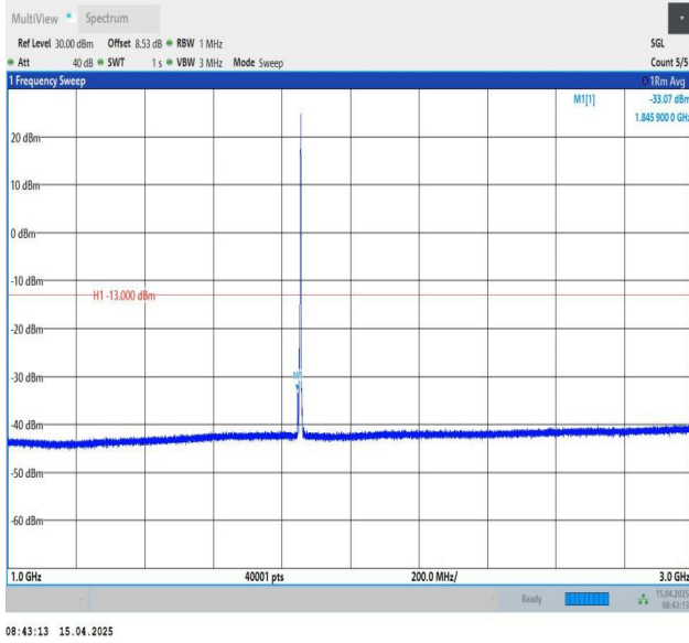
Band25-5MHz-QPSK-26065-1RB#24-1000~3000-PASS
