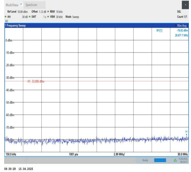
Band25-3MHz-QPSK-26365-1RB#0-0.15~30-PASS
