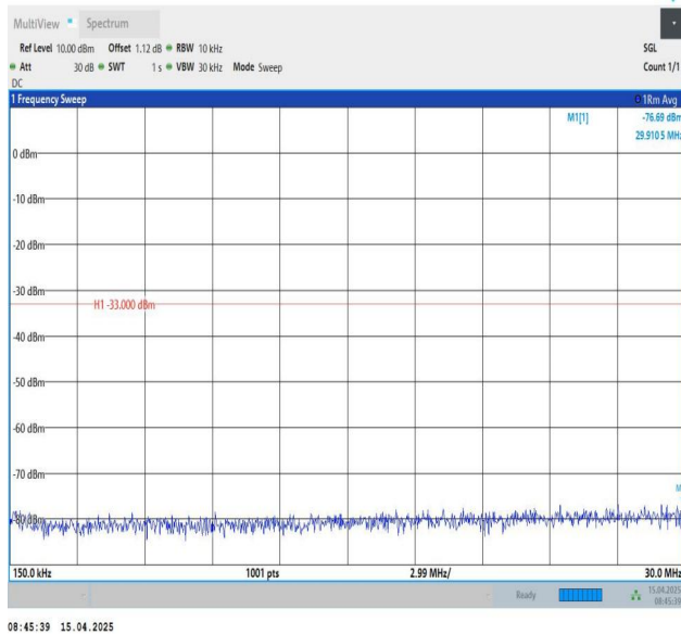
Band25-5MHz-QPSK-26665-1RB#24-0.15~30-PASS
