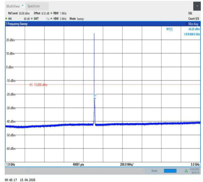
Band25-5MHz-QPSK-26665-1RB#0-1000~3000-PASS
