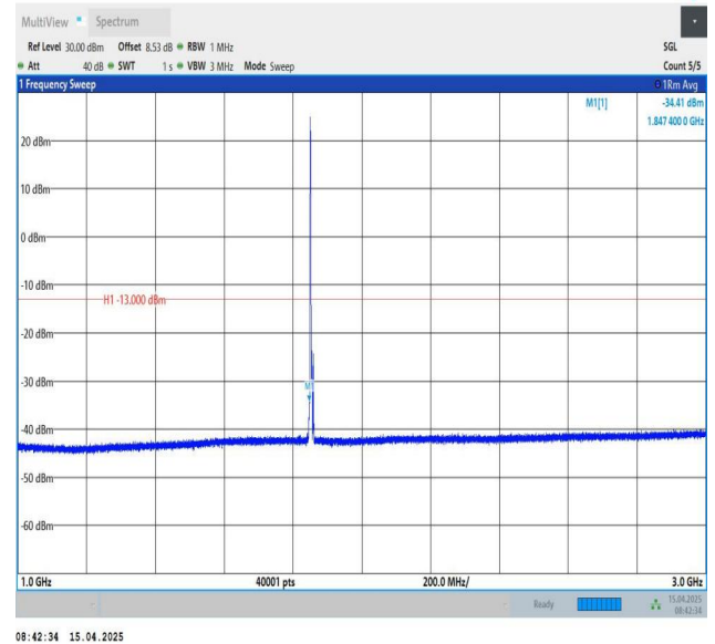
Band25-5MHz-QPSK-26065-1RB#0-1000~3000-PASS
