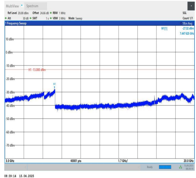
Band25-3MHz-QPSK-26055-1RB#14-3000~20000-PASS
