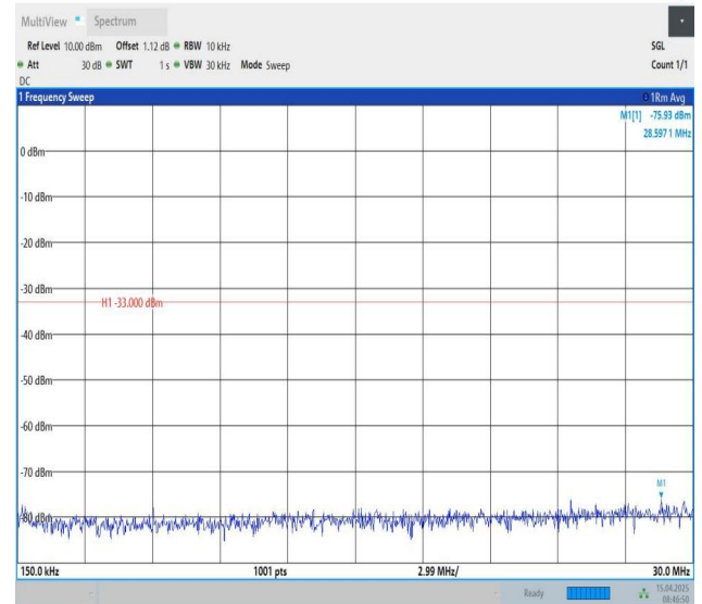
Band25-10MHz-QPSK-26090-1RB#0-0.15~30-PASS
