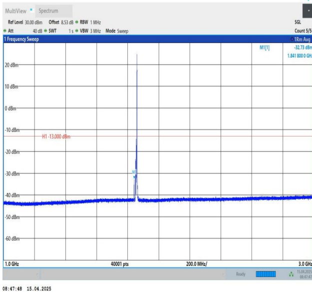
Band25-10MHz-QPSK-26090-1RB#49-1000~3000-PASS
