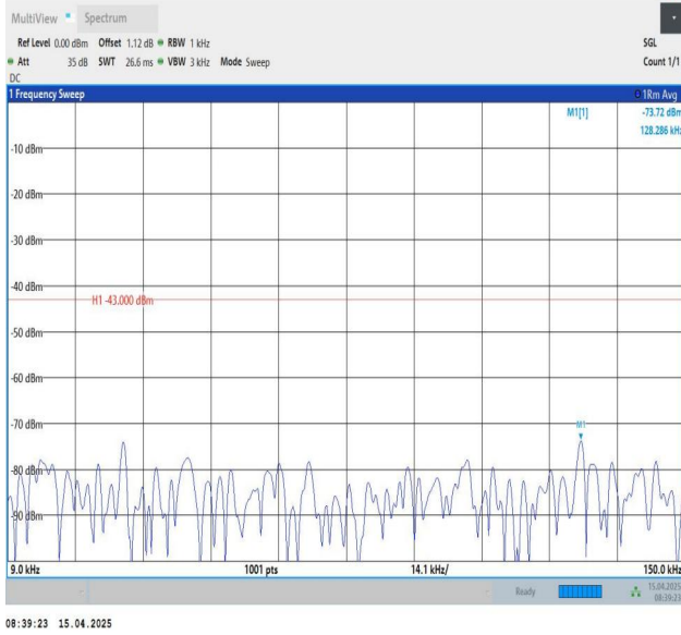
Band25-3MHz-QPSK-26365-1RB#0-0.009~0.15-PASS
