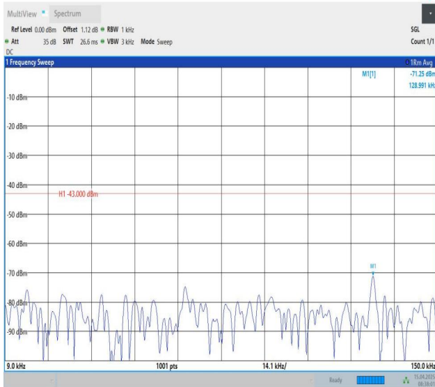
Band25-3MHz-QPSK-26055-1RB#0-0.009~0.15-PASS
