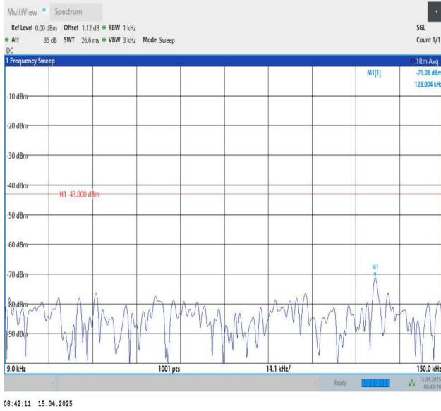
Band25-5MHz-QPSK-26065-1RB#0-0.009~0.15-PASS
