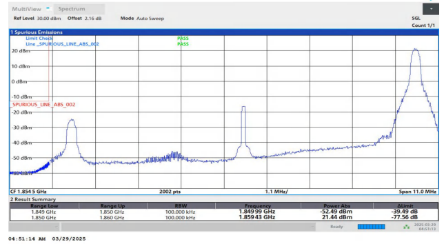
Band25-10MHz-QPSK-26090-1RB#49-PASS
