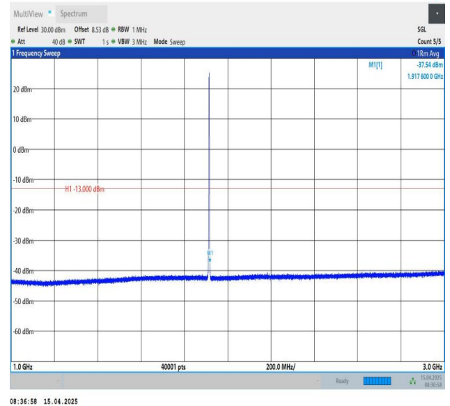
Band25-1.4MHz-QPSK-26683-1RB#0-1000~3000-PASS
