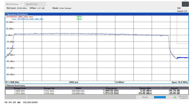
Band25-15MHz-QPSK-26615-75RB#0-PASS
