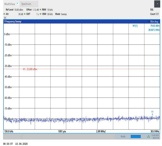
Band25-1.4MHz-QPSK-26047-1RB#0-0.15~30-PASS
