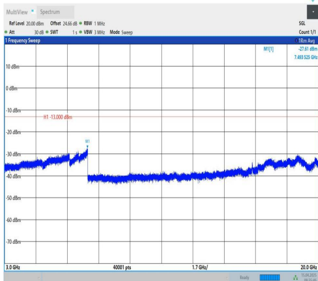
Band25-1.4MHz-QPSK-26365-1RB#0-3000~20000-PASS
