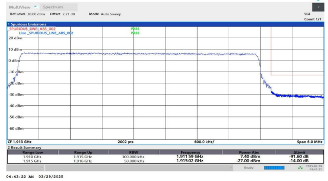
Band25-5MHz-QPSK-26665-25RB#0-PASS
