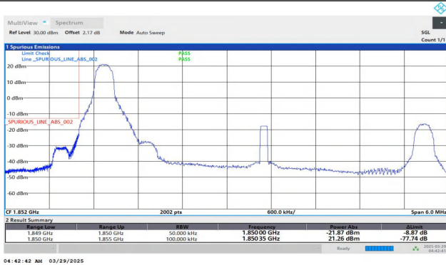
Band25-5MHz-QPSK-26065-1RB#0-PASS
