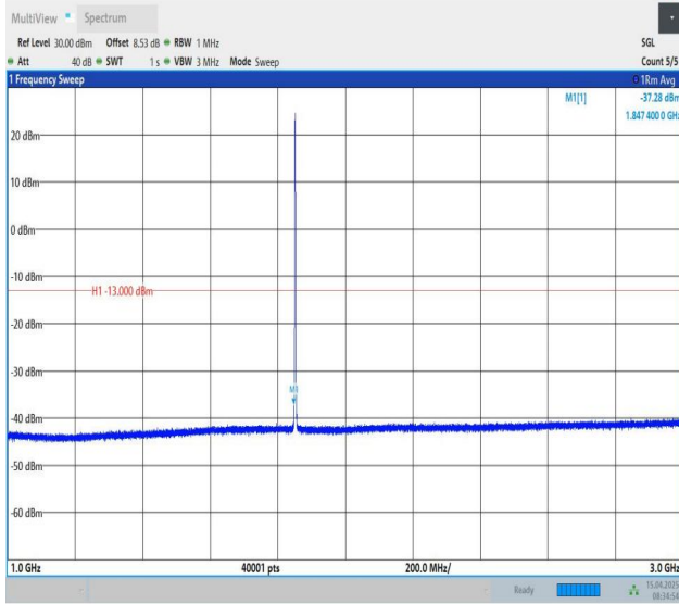
Band25-1.4MHz-QPSK-26047-1RB#5-1000~3000-PASS
