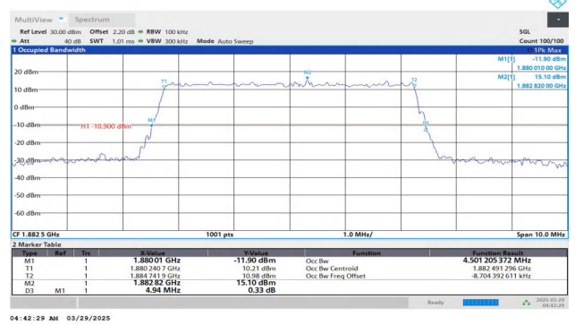
Band25-5MHz-16QAM-26365-25RB#0-PASS
