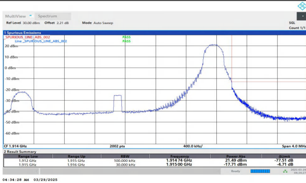
Band25-3MHz-QPSK-26675-1RB#14-PASS
