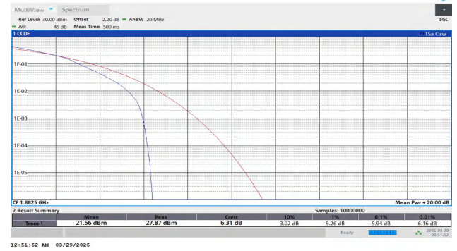
Band25-15MHz-16QAM-26365-27RB#0-PASS
