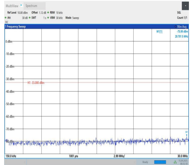
Band25-1.4MHz-QPSK-26365-1RB#0-0.15~30-PASS
