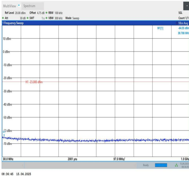
Band25-1.4MHz-QPSK-26683-1RB#0-30~1000-PASS
