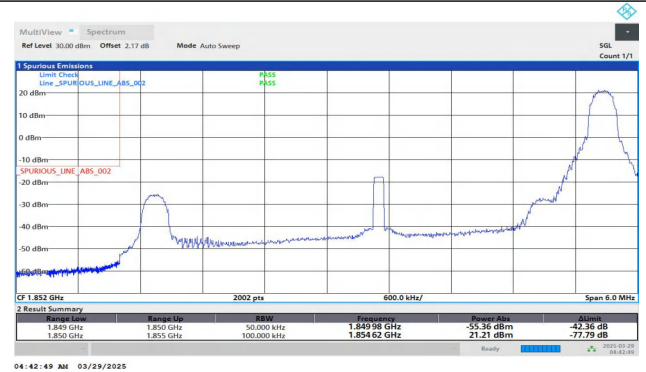
Band25-5MHz-QPSK-26065-1RB#24-PASS
