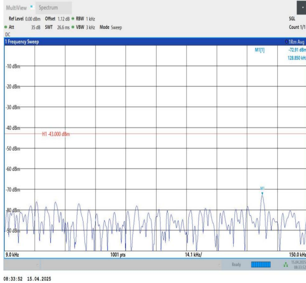
Band25-1.4MHz-QPSK-26047-1RB#0-0.009~0.15-PASS
