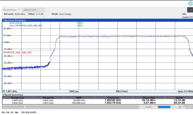
Band25-3MHz-QPSK-26055-15RB#0-PASS
