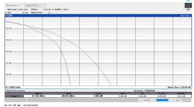
Band25-5MHz-16QAM-26365-25RB#0-PASS
