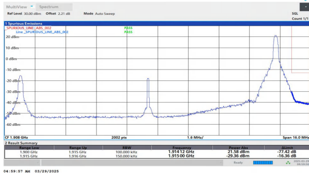
Band25-15MHz-QPSK-26615-1RB#74-PASS
