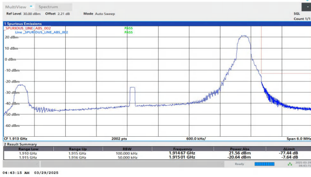
Band25-5MHz-QPSK-26665-1RB#24-PASS
