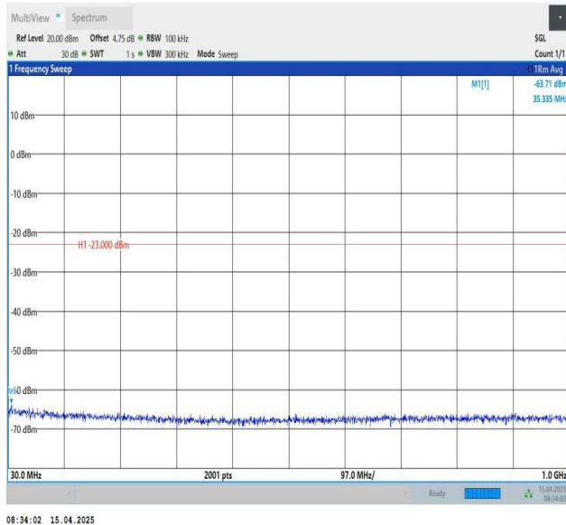
Band25-1.4MHz-QPSK-26047-1RB#0-30~1000-PASS
