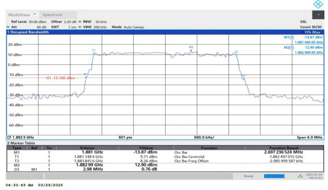
Band25-3MHz-16QAM-26365-15RB#0-PASS
