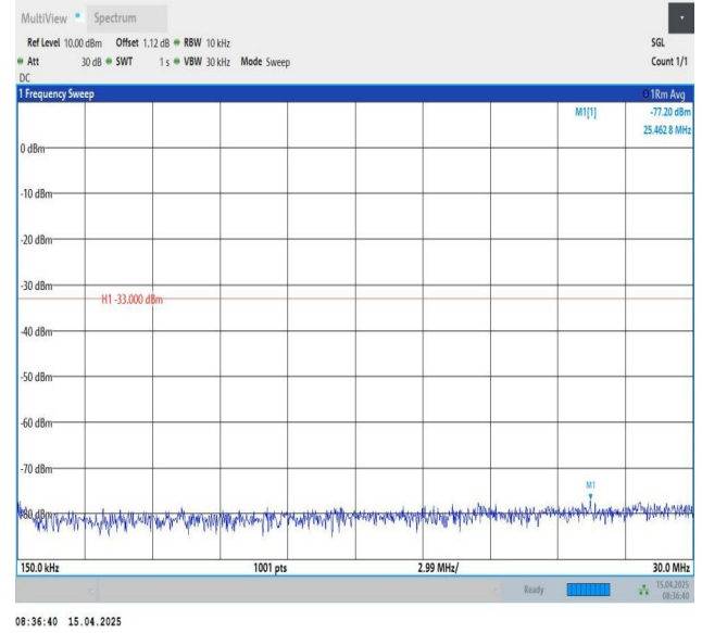
Band25-1.4MHz-QPSK-26683-1RB#0-0.15~30-PASS
