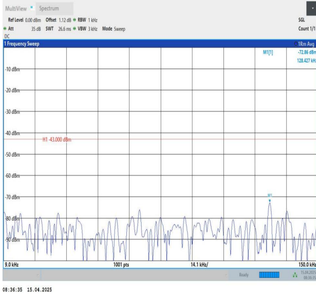
Band25-1.4MHz-QPSK-26683-1RB#0-0.009~0.15-PASS
