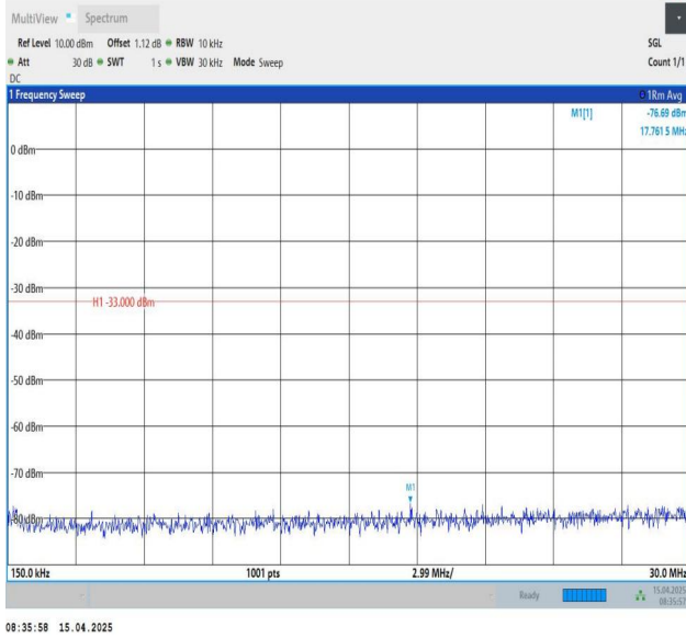
Band25-1.4MHz-QPSK-26365-1RB#5-0.15~30-PASS
