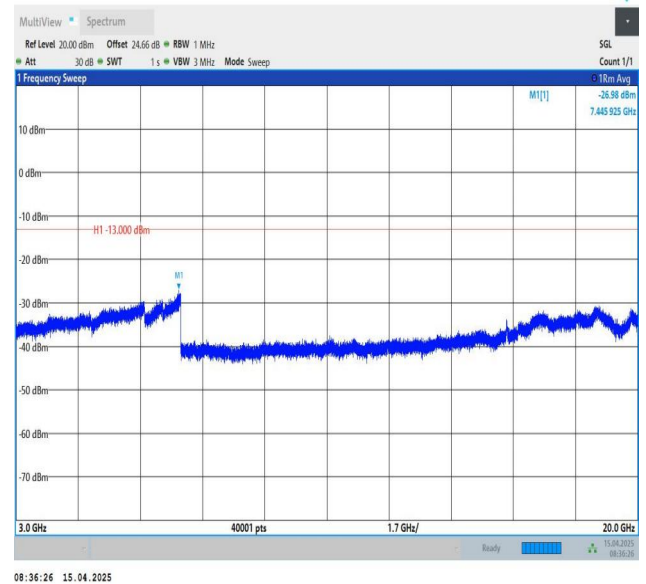
Band25-1.4MHz-QPSK-26365-1RB#5-3000~20000-PASS
