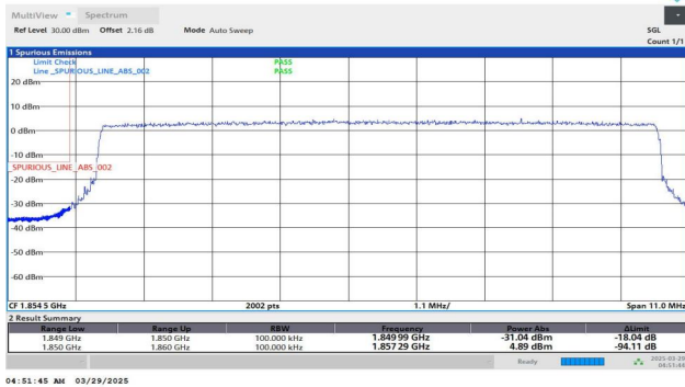
Band25-10MHz-QPSK-26090-50RB#0-PASS
