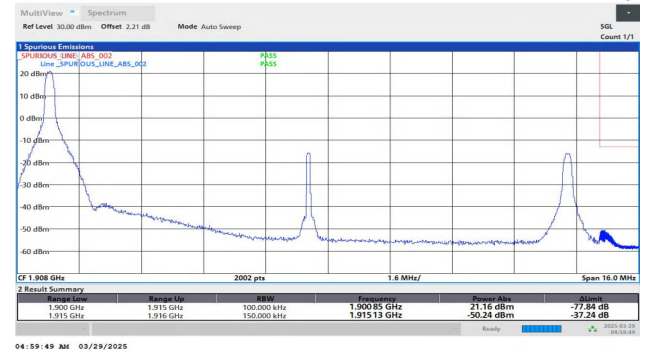
Band25-15MHz-QPSK-26615-1RB#0-PASS
