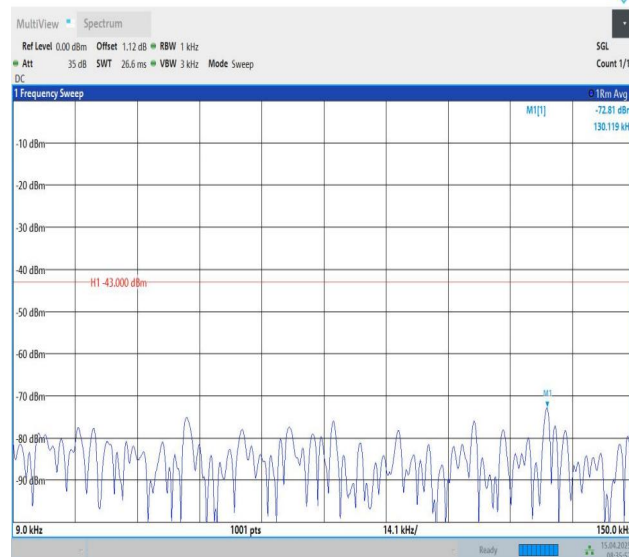
Band25-1.4MHz-QPSK-26365-1RB#5-0.009~0.15-PASS
