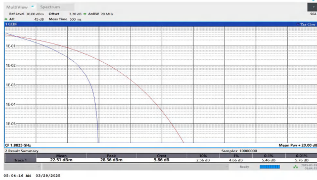
Band25-15MHz-QPSK-26365-75RB#0-PASS
