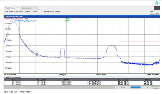
Band25-3MHz-QPSK-26675-1RB#0-PASS
