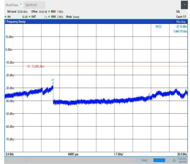
Band25-1.4MHz-QPSK-26047-1RB#5-3000~20000-PASS
