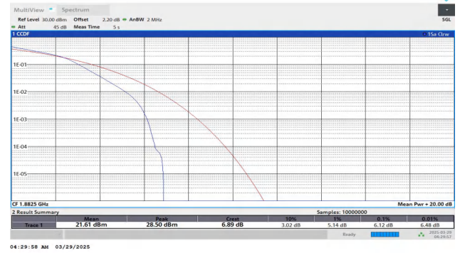
Band25-1.4MHz-16QAM-26365-6RB#0-PASS
