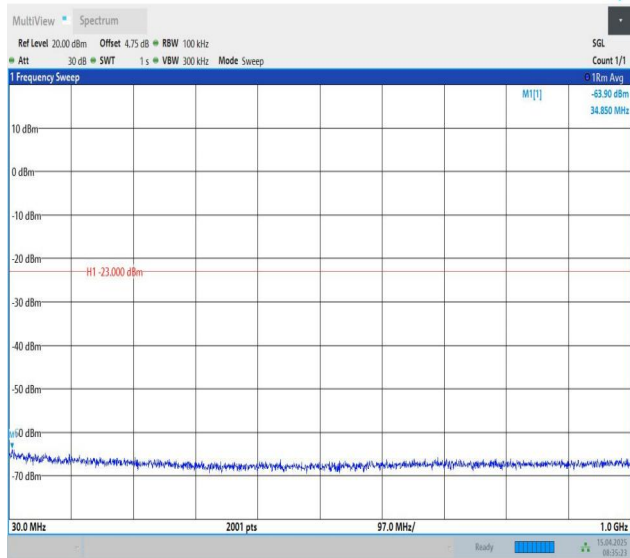
Band25-1.4MHz-QPSK-26365-1RB#0-30~1000-PASS
