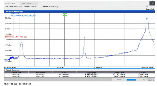
Band25-15MHz-QPSK-26115-1RB#74-PASS
