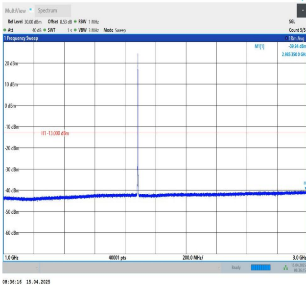
Band25-1.4MHz-QPSK-26365-1RB#5-1000~3000-PASS
