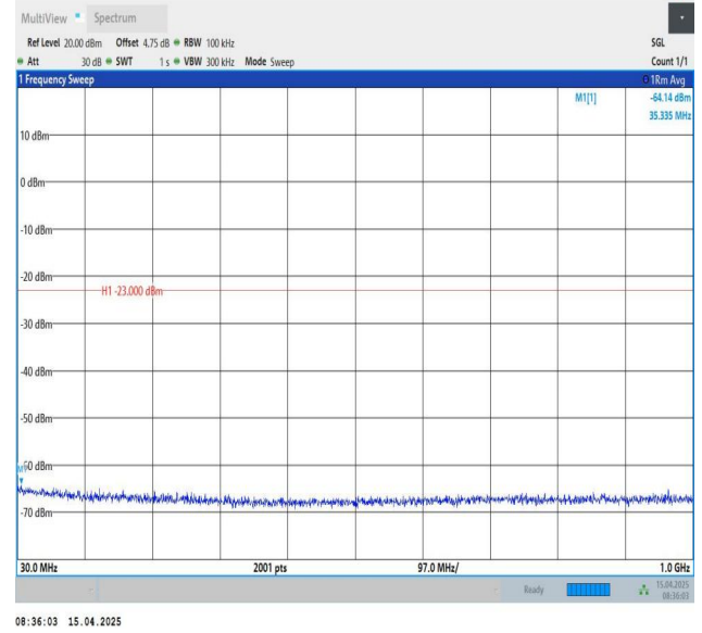
Band25-1.4MHz-QPSK-26365-1RB#5-30~1000-PASS
