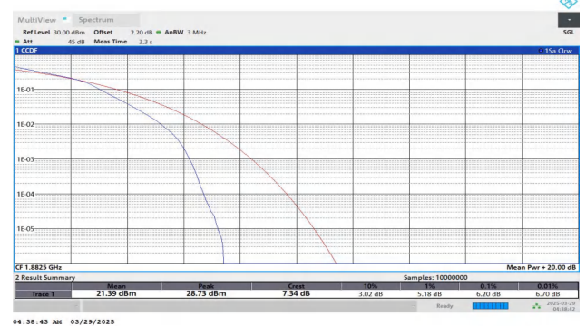
Band25-3MHz-16QAM-26365-15RB#0-PASS
