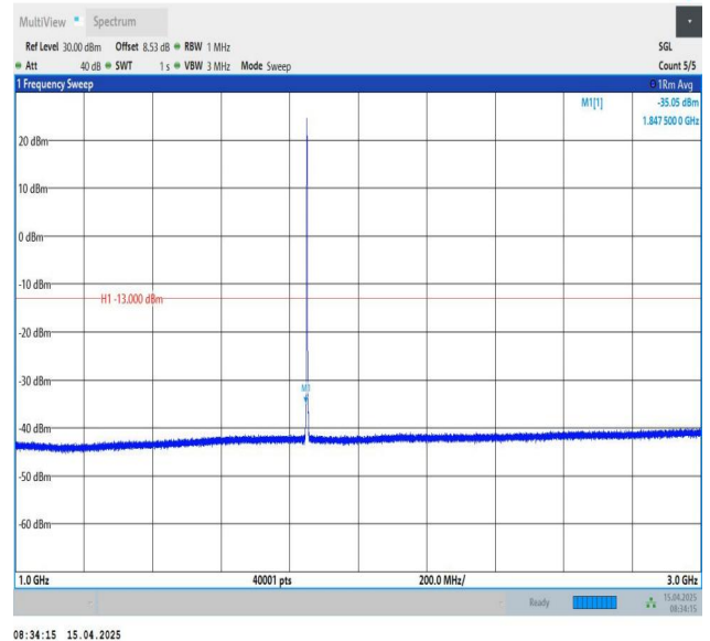
Band25-1.4MHz-QPSK-26047-1RB#0-1000~3000-PASS
