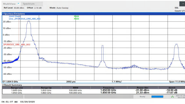
Band25-10MHz-QPSK-26090-1RB#0-PASS
