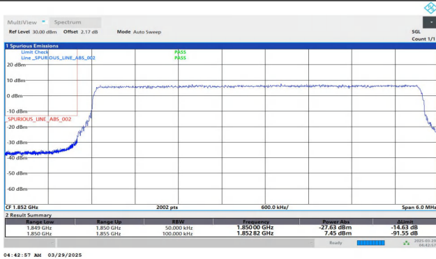
Band25-5MHz-QPSK-26065-25RB#0-PASS
