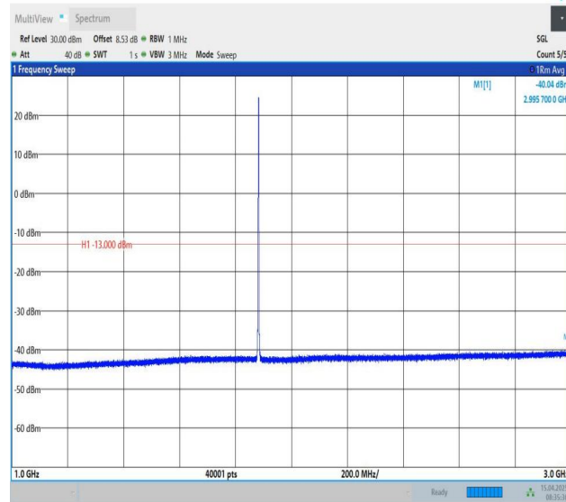
Band25-1.4MHz-QPSK-26365-1RB#0-1000~3000-PASS
