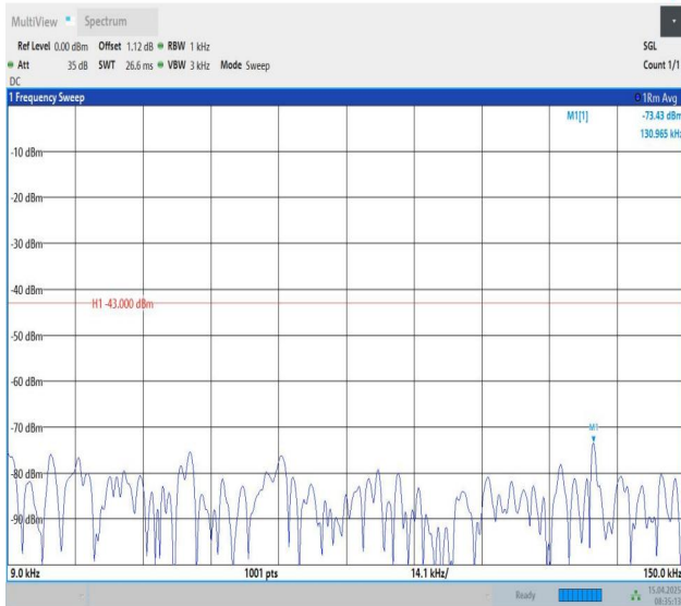
Band25-1.4MHz-QPSK-26365-1RB#0-0.009~0.15-PASS
