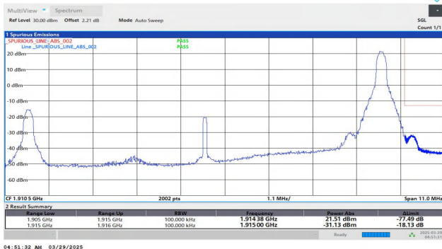
Band25-10MHz-QPSK-26640-1RB#49-PASS
