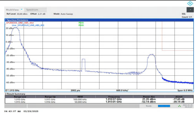
Band25-5MHz-QPSK-26665-1RB#0-PASS
