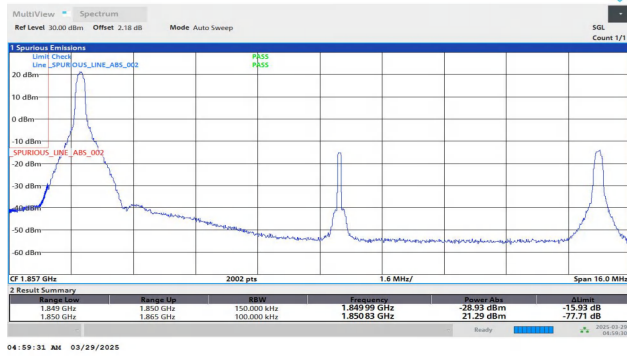
Band25-15MHz-QPSK-26115-1RB#0-PASS
