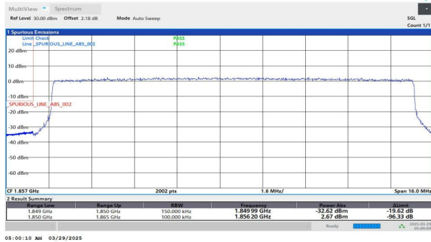
Band25-15MHz-QPSK-26115-75RB#0-PASS
