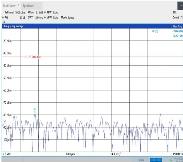
Band12-5MHz-QPSK-23095-1RB#0-0.009~0.15-PASS
