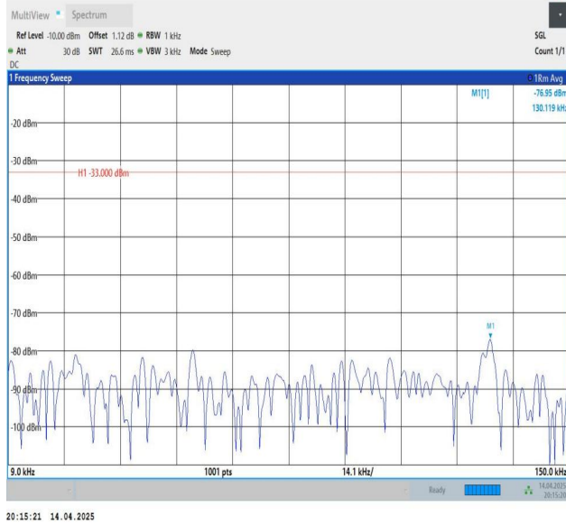
Band12-5MHz-QPSK-23035-1RB#0-0.009~0.15-PASS
