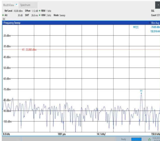
Band12-3MHz-QPSK-23165-1RB#0-0.009~0.15-PASS
