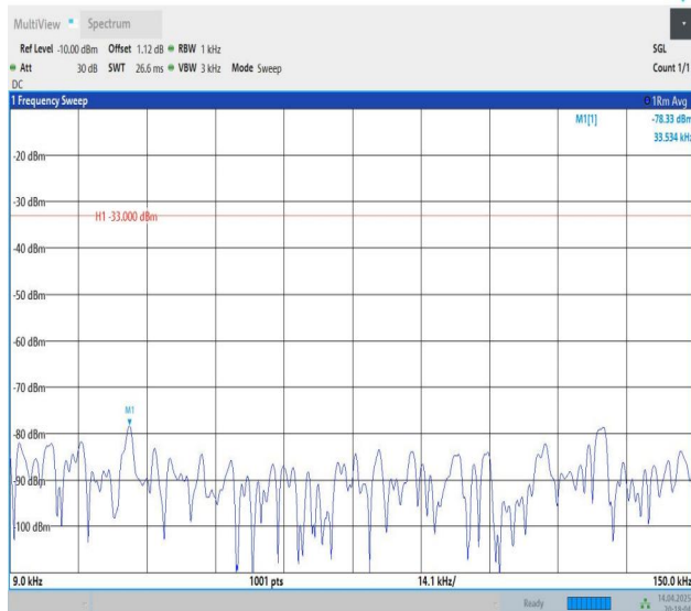
Band12-10MHz-QPSK-23060-1RB#0-0.009~0.15-PASS
