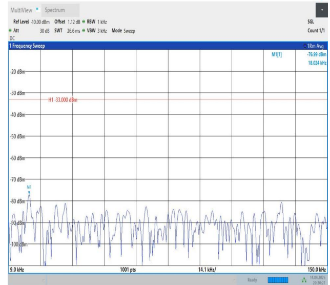
Band12-10MHz-QPSK-23130-1RB#49-0.009~0.15-PASS
