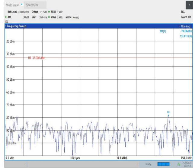
Band12-5MHz-QPSK-23155-1RB#24-0.009~0.15-PASS
