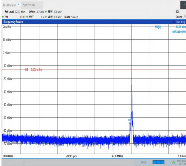
Band12-10MHz-QPSK-23130-1RB#0-30~1000-PASS
