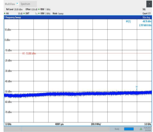
Band12-10MHz-QPSK-23130-1RB#0-1000~3000-PASS
