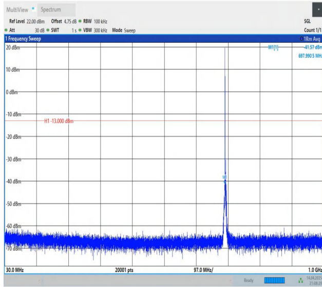
Band12-3MHz-QPSK-23025-1RB#0-30~1000-PASS
