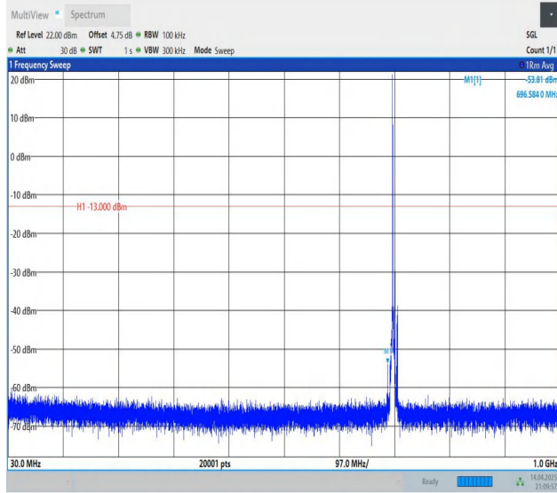
Band12-5MHz-QPSK-23095-1RB#0-30~1000-PASS
