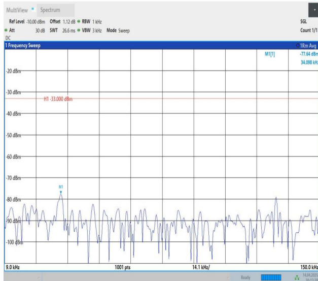
Band12-3MHz-QPSK-23025-1RB#0-0.009~0.15-PASS
