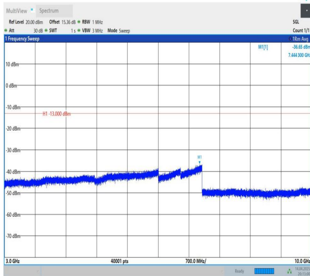
Band12-3MHz-QPSK-23025-1RB#0-3000~10000-PASS
