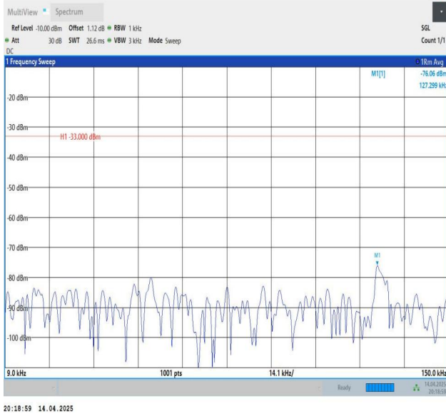
Band12-10MHz-QPSK-23095-1RB#0-0.009~0.15-PASS
