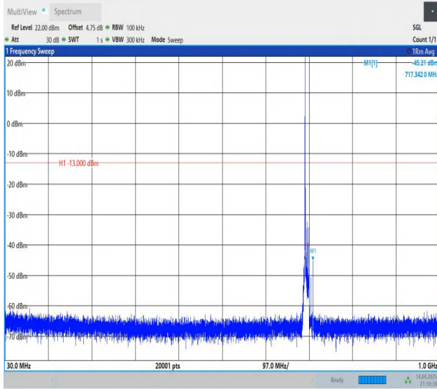
Band12-10MHz-QPSK-23060-1RB#0-30~1000-PASS
