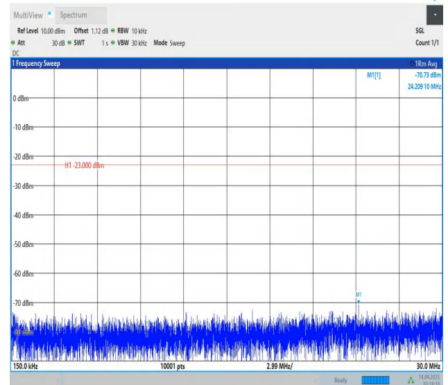
Band12-10MHz-QPSK-23060-1RB#0-0.15~30-PASS
