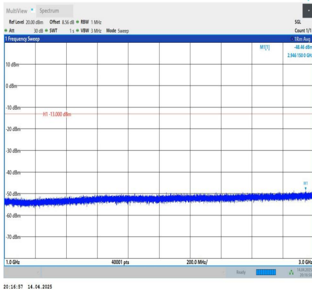
Band12-5MHz-QPSK-23095-1RB#24-1000~3000-PASS
