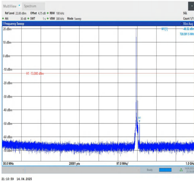
Band12-10MHz-QPSK-23095-1RB#0-30~1000-PASS
