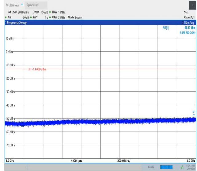
Band12-10MHz-QPSK-23060-1RB#0-1000~3000-PASS
