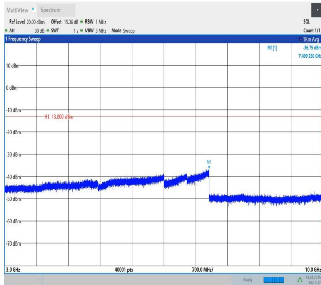
Band12-5MHz-QPSK-23095-1RB#0-3000~10000-PASS
