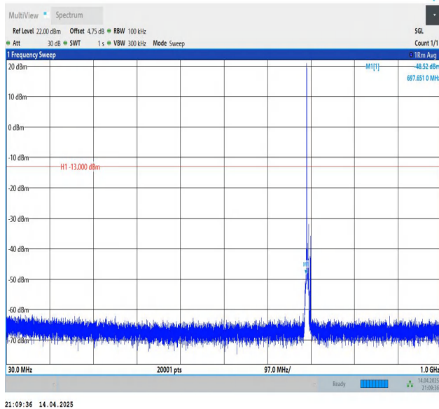
Band12-5MHz-QPSK-23035-1RB#0-30~1000-PASS
