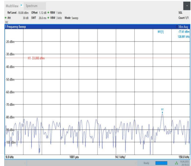
Band12-10MHz-QPSK-23060-1RB#49-0.009~0.15-PASS
