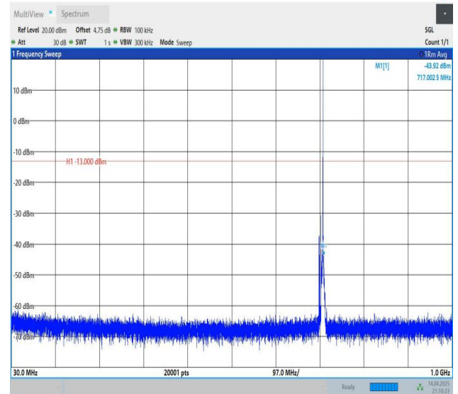
Band12-5MHz-QPSK-23155-1RB#24-30~1000-PASS
