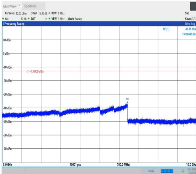
Band12-10MHz-QPSK-23130-1RB#0-3000~10000-PASS
