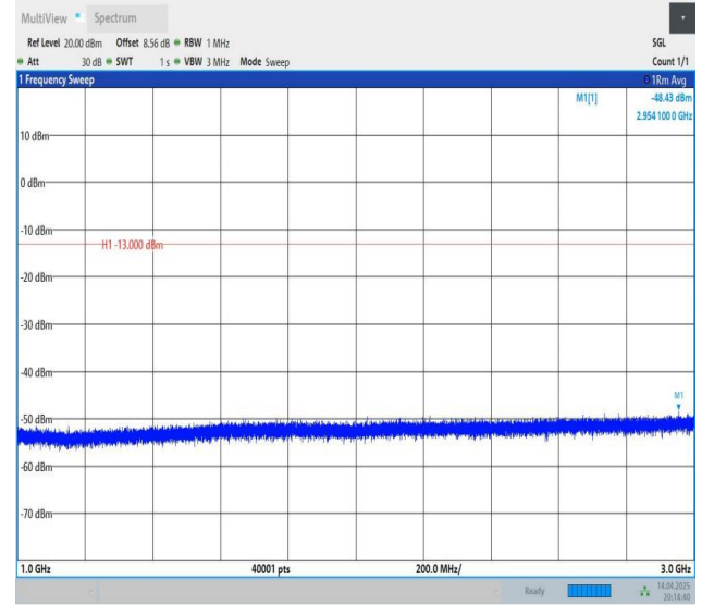
Band12-3MHz-QPSK-23165-1RB#0-1000~3000-PASS
