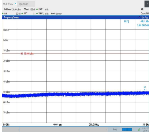
Band12-3MHz-QPSK-23095-1RB#14-1000~3000-PASS
