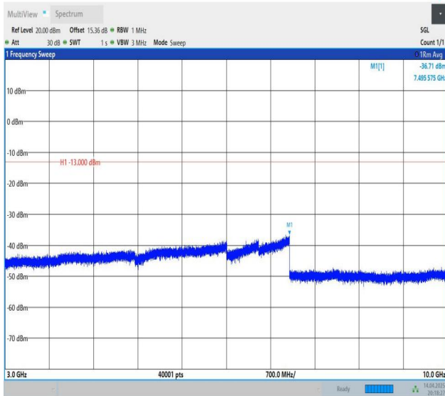
Band12-10MHz-QPSK-23060-1RB#0-3000~10000-PASS
