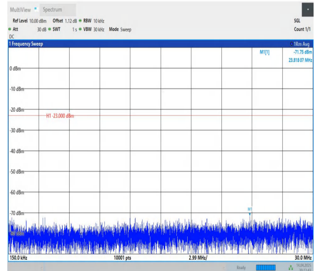
Band12-3MHz-QPSK-23025-1RB#0-0.15~30-PASS
