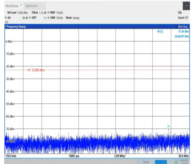
Band12-5MHz-QPSK-23095-1RB#0-0.15~30-PASS
