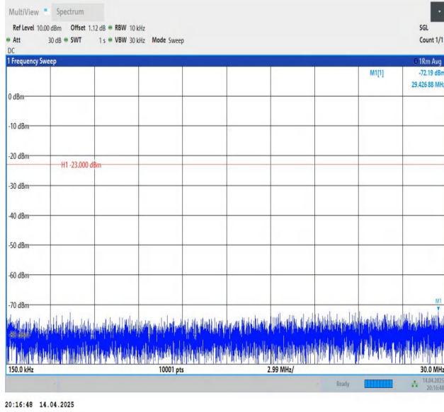
Band12-5MHz-QPSK-23095-1RB#24-0.15~30-PASS
