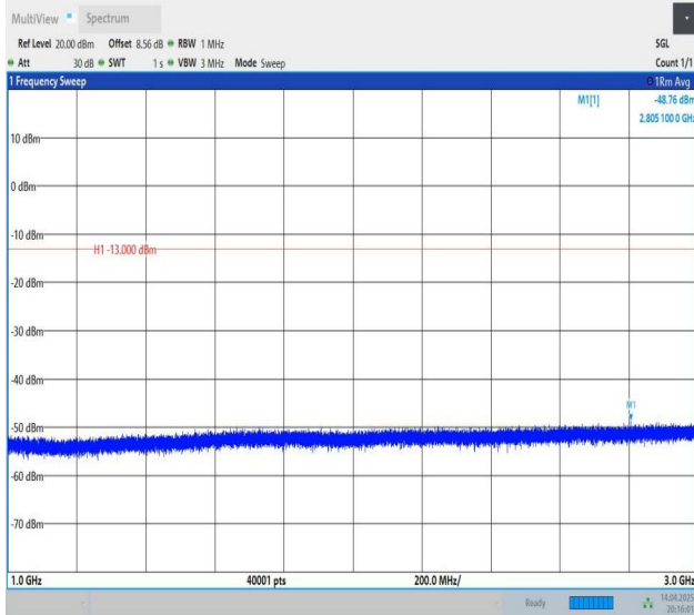
Band12-5MHz-QPSK-23035-1RB#24-1000~3000-PASS
