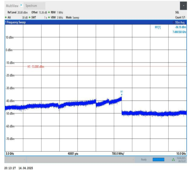
Band12-3MHz-QPSK-23025-1RB#14-3000~10000-PASS
