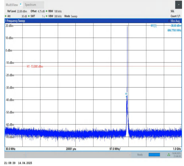
Band12-3MHz-QPSK-23025-1RB#14-30~1000-PASS
