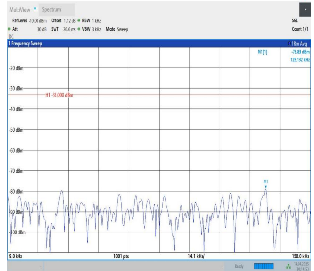
Band12-3MHz-QPSK-23165-1RB#14-0.009~0.15-PASS
