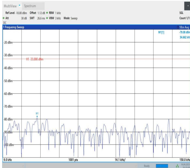
Band12-1.4MHz-QPSK-23095-1RB#0-0.009~0.15-PASS
