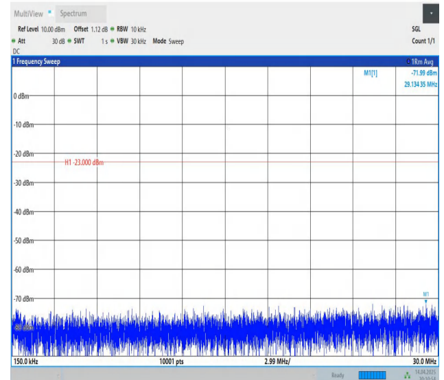
Band12-1.4MHz-QPSK-23095-1RB#0-0.15~30-PASS
