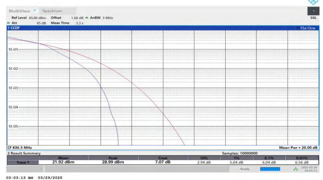
Band5-3MHz-16QAM-20525-15RB#0-PASS
