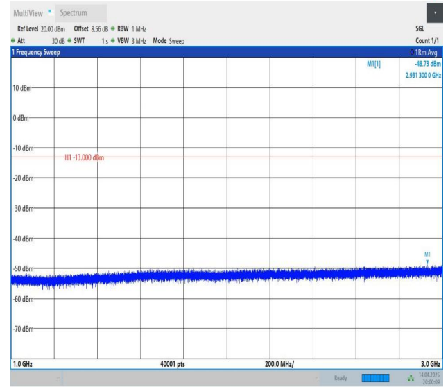
Band5-1.4MHz-QPSK-20525-1RB#0-1000~3000-PASS
