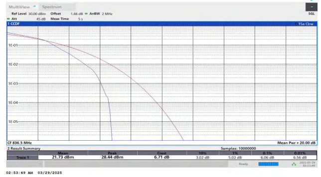
Band5-1.4MHz-16QAM-20525-6RB#0-PASS
