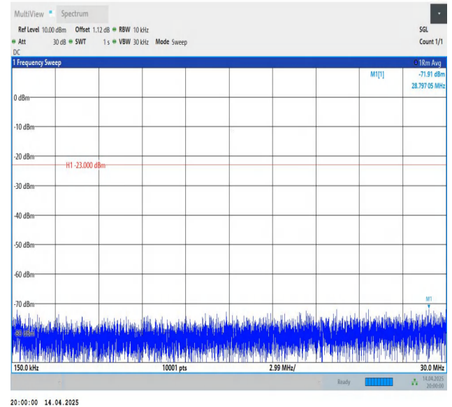
Band5-1.4MHz-QPSK-20525-1RB#0-0.15~30-PASS
