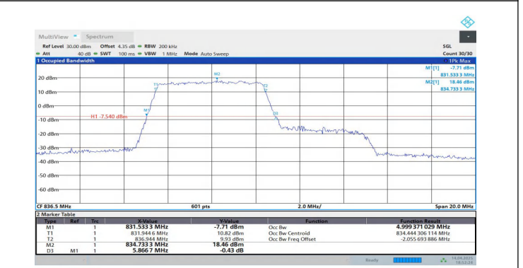
Band5-5MHz-16QAM-20525-25RB#0-PASS
