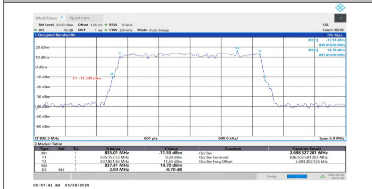
Band5-3MHz-QPSK-20525-15RB#0-PASS
