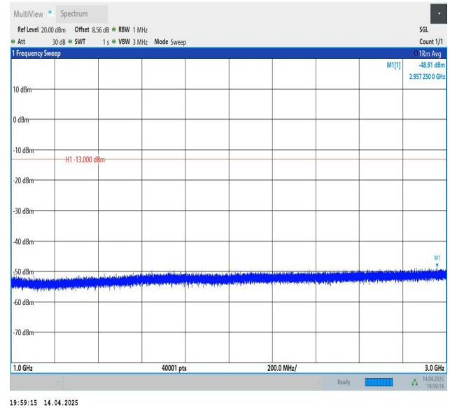
Band5-1.4MHz-QPSK-20407-1RB#0-1000~3000-PASS
