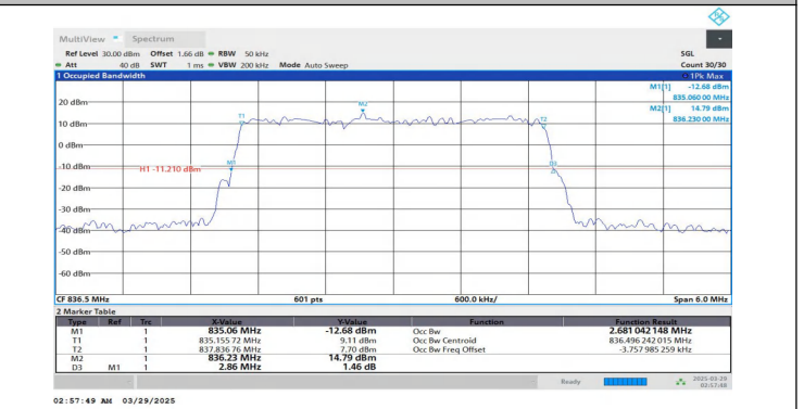
Band5-3MHz-16QAM-20525-15RB#0-PASS
