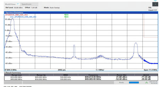
Band5-10MHz-QPSK-20600-1RB#0-PASS
