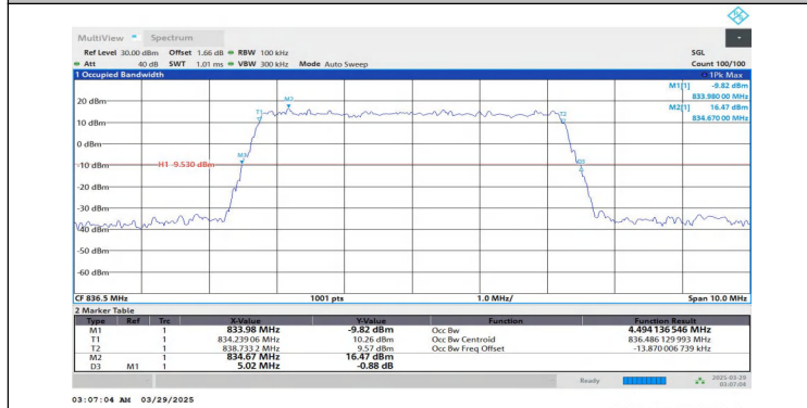
Band5-5MHz-QPSK-20525-25RB#0-PASS
