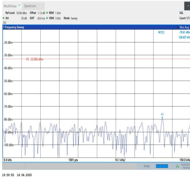
Band5-1.4MHz-QPSK-20525-1RB#0-0.009~0.15-PASS
