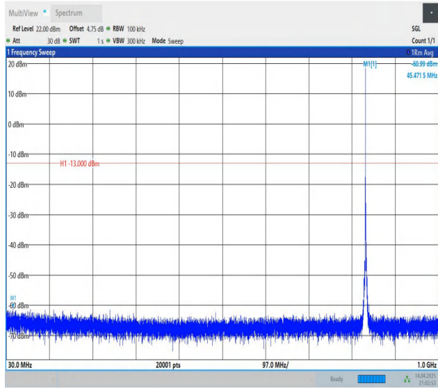
Band5-1.4MHz-QPSK-20525-1RB#0-30~1000-PASS
