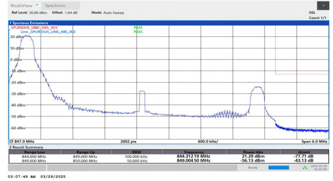
Band5-5MHz-QPSK-20625-1RB#0-PASS
