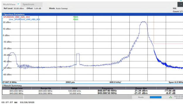
Band5-5MHz-QPSK-20625-1RB#24-PASS
