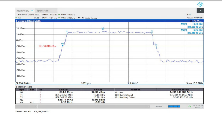
Band5-5MHz-16QAM-20525-25RB#0-PASS
