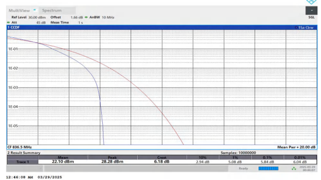
Band5-10MHz-16QAM-20525-27RB#0-PASS
