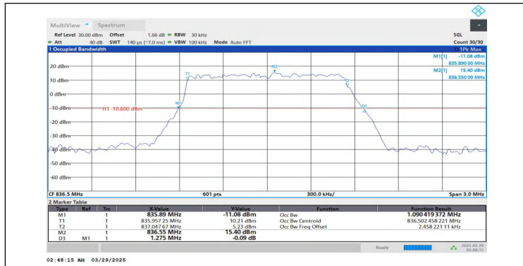
Band5-1.4MHz-QPSK-20525-6RB#0-PASS
