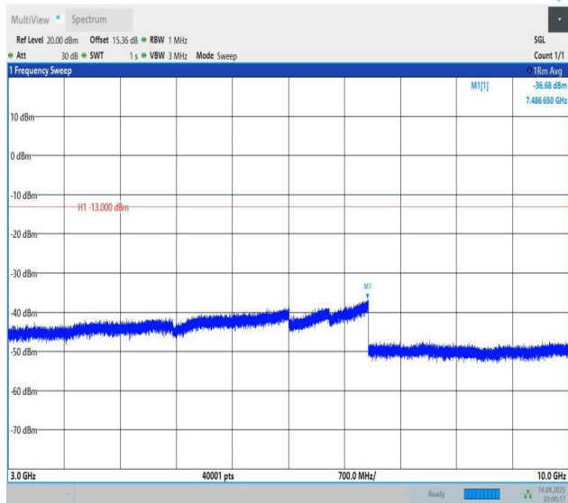
Band5-1.4MHz-QPSK-20525-1RB#0-3000~10000-PASS
