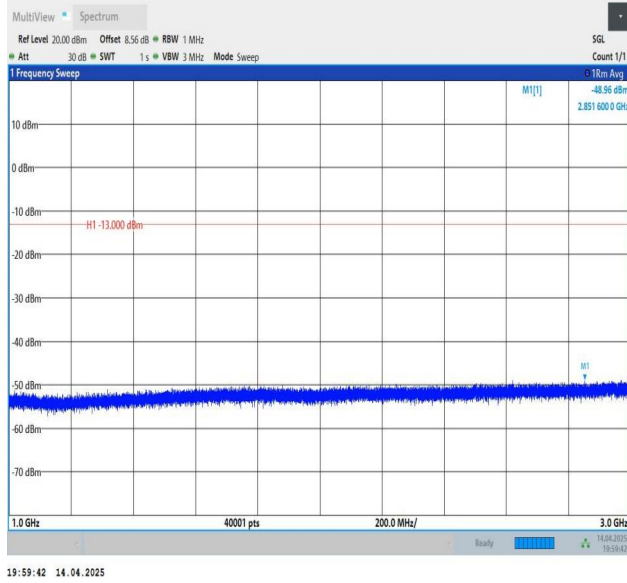
Band5-1.4MHz-QPSK-20407-1RB#5-1000~3000-PASS
