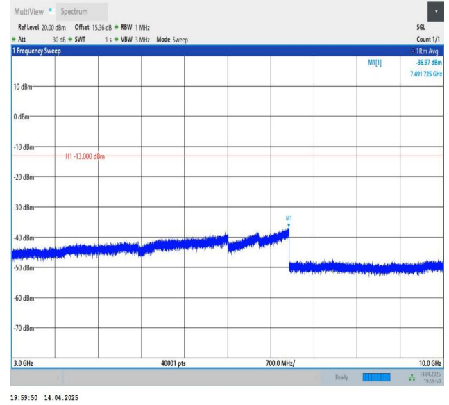
Band5-1.4MHz-QPSK-20407-1RB#5-3000~10000-PASS
