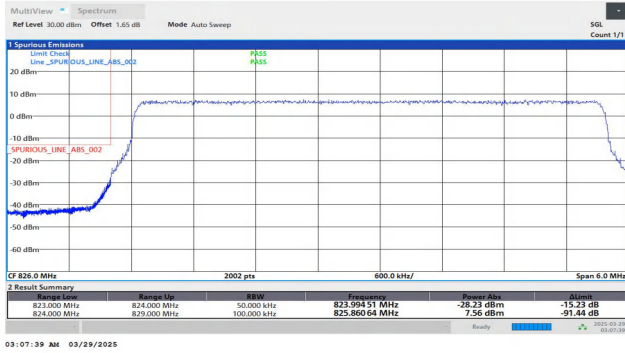
Band5-5MHz-QPSK-20425-25RB#0-PASS
