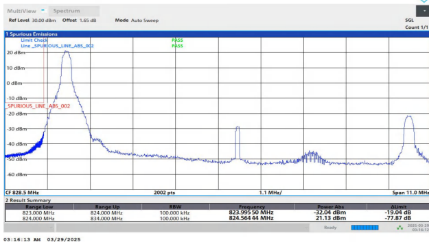
Band5-10MHz-QPSK-20450-1RB#0-PASS
