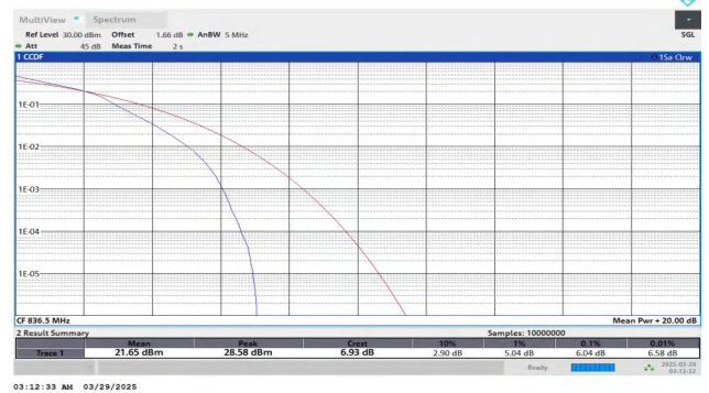
Band5-5MHz-16QAM-20525-25RB#0-PASS
