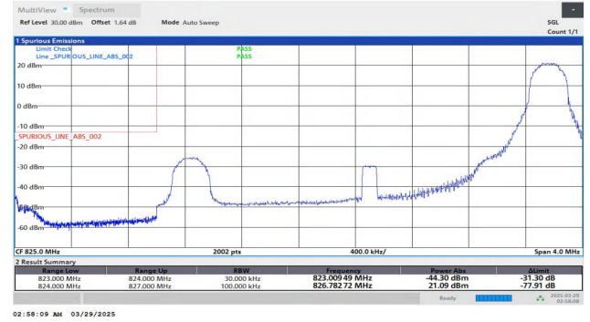
Band5-3MHz-QPSK-20415-1RB#14-PASS
