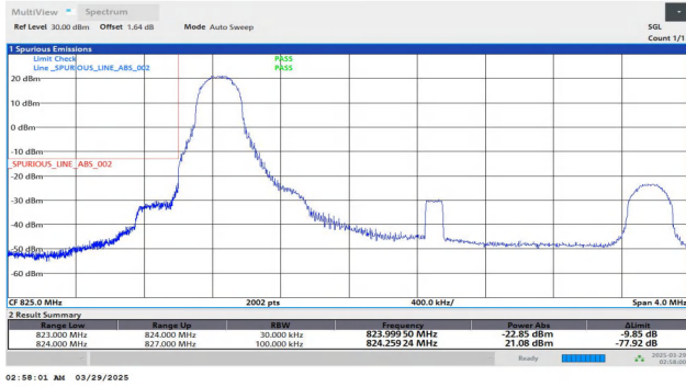
Band5-3MHz-QPSK-20415-1RB#0-PASS
