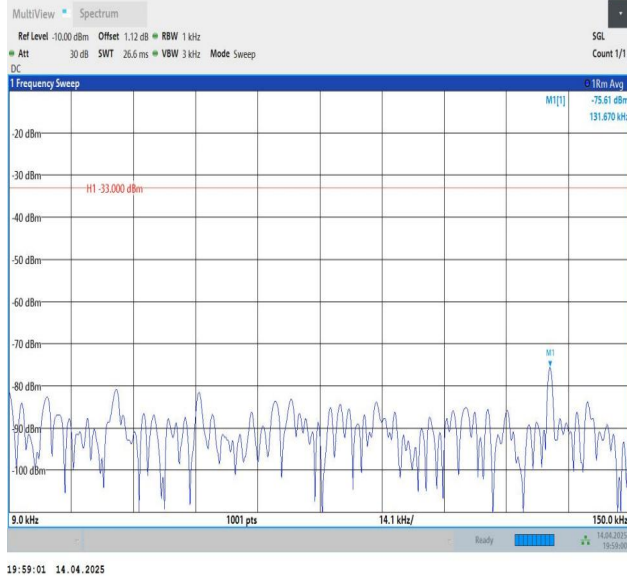
Band5-1.4MHz-QPSK-20407-1RB#0-0.009~0.15-PASS
