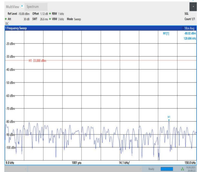
Band5-1.4MHz-QPSK-20525-1RB#5-0.009~0.15-PASS
