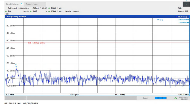
Band4-20MHz-QPSK-20050-1RB#99-0.009~0.15-PASS
