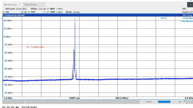
Band4-15MHz-QPSK-20325-1RB#74-1000~3000-PASS
