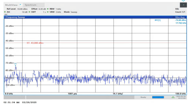
Band4-15MHz-QPSK-20025-1RB#74-0.009~0.15-PASS
