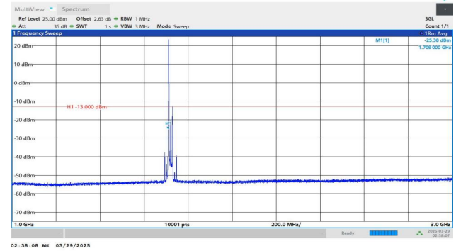
Band4-20MHz-QPSK-20050-1RB#0-1000~3000-PASS
