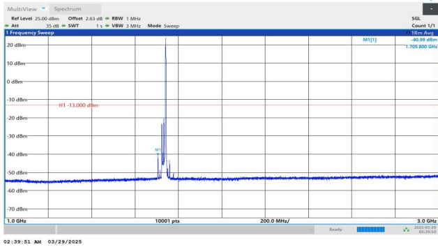
Band4-20MHz-QPSK-20175-1RB#99-1000~3000-PASS
