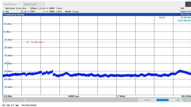
Band4-20MHz-QPSK-20050-1RB#0-3000~20000-PASS
