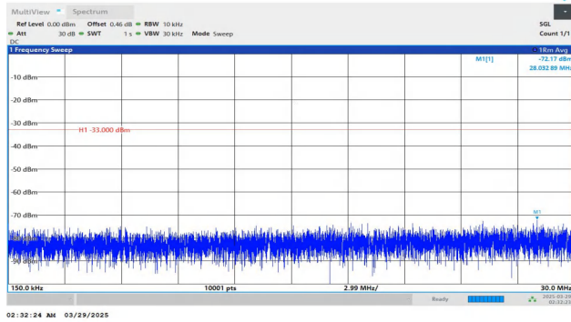
Band4-15MHz-QPSK-20175-1RB#74-0.15~30-PASS
