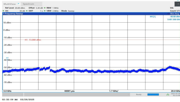
Band4-15MHz-QPSK-20175-1RB#0-3000~20000-PASS
