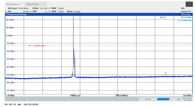
Band4-10MHz-QPSK-20175-1RB#0-1000~3000-PASS
