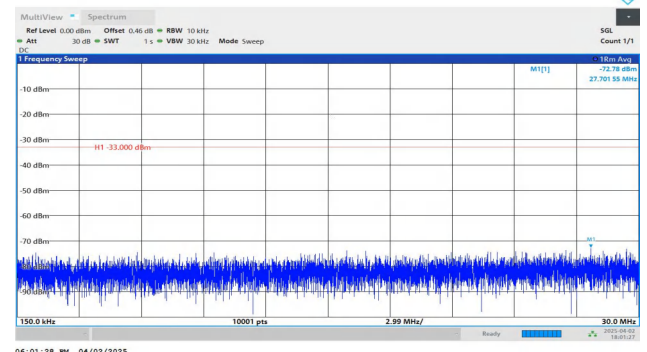
Band4-10MHz-QPSK-20175-1RB#0-0.15~30-PASS
