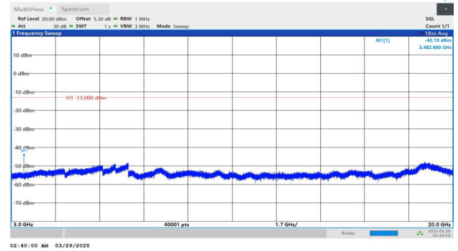
Band4-20MHz-QPSK-20175-1RB#99-3000~20000-PASS
