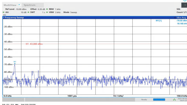
Band4-10MHz-QPSK-20175-1RB#0-0.009~0.15-PASS
