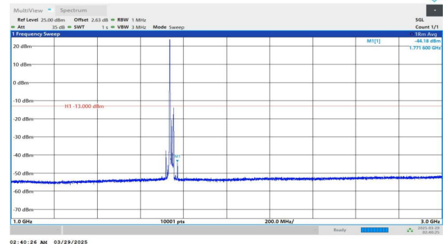
Band4-20MHz-QPSK-20300-1RB#0-1000~3000-PASS
