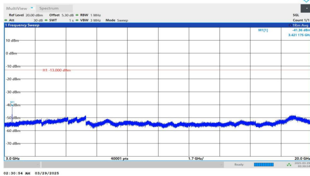
Band4-15MHz-QPSK-20025-1RB#0-3000~20000-PASS
