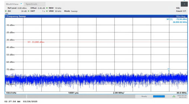
Band4-20MHz-QPSK-20050-1RB#0-0.15~30-PASS
