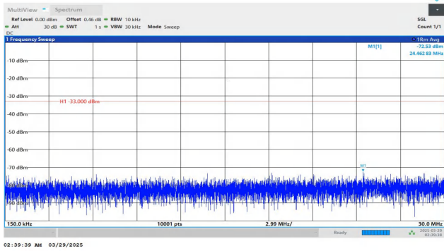
Band4-20MHz-QPSK-20175-1RB#99-0.15~30-PASS
