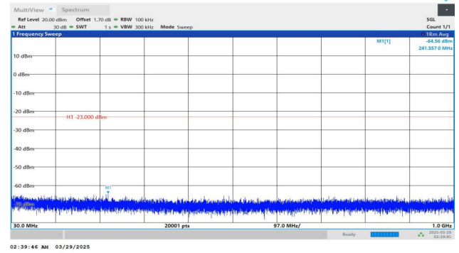
Band4-20MHz-QPSK-20175-1RB#99-30~1000-PASS
