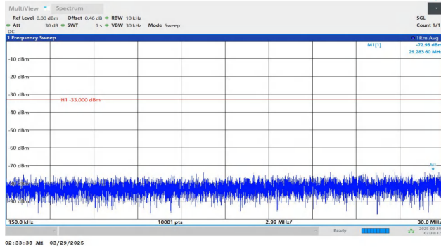
Band4-15MHz-QPSK-20325-1RB#74-0.15~30-PASS
