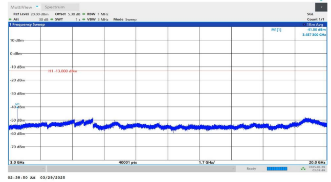
Band4-20MHz-QPSK-20050-1RB#99-3000~20000-PASS
