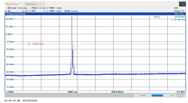
Band4-15MHz-QPSK-20325-1RB#0-1000~3000-PASS
