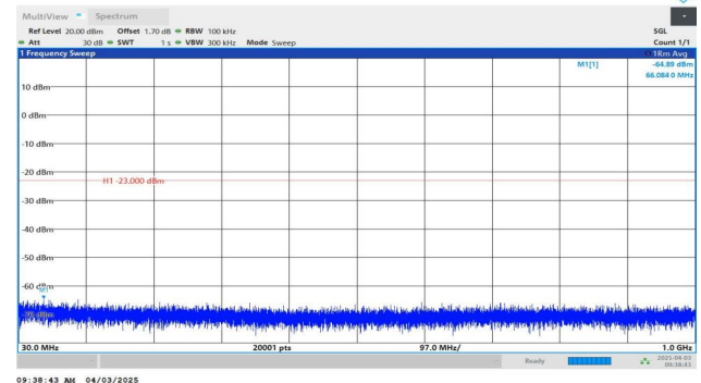
Band4-10MHz-QPSK-20350-1RB#49-30~1000-PASS
