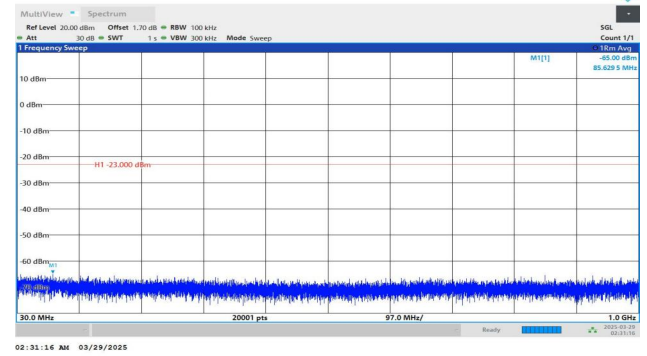
Band4-15MHz-QPSK-20025-1RB#74-30~1000-PASS
