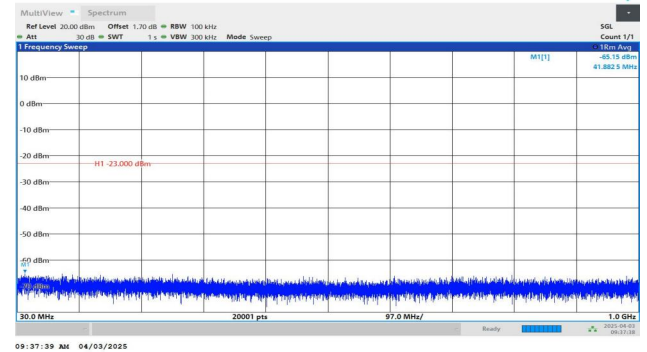
Band4-10MHz-QPSK-20000-1RB#49-30~1000-PASS
