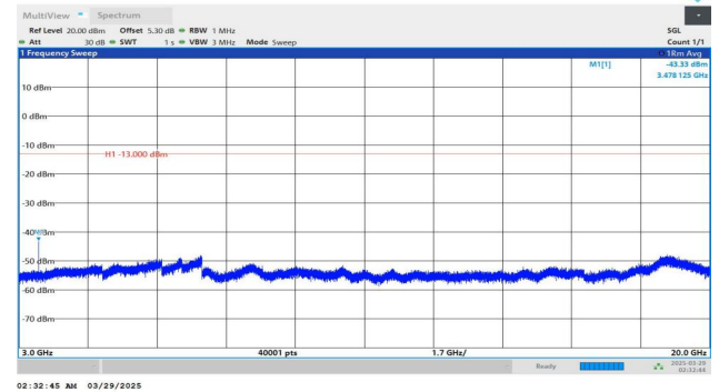
Band4-15MHz-QPSK-20175-1RB#74-3000~20000-PASS
