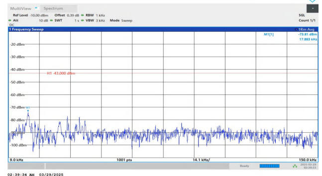
Band4-20MHz-QPSK-20175-1RB#99-0.009~0.15-PASS
