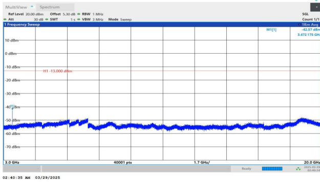
Band4-20MHz-QPSK-20300-1RB#0-3000~20000-PASS
