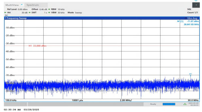
Band4-15MHz-QPSK-20025-1RB#0-0.15~30-PASS
