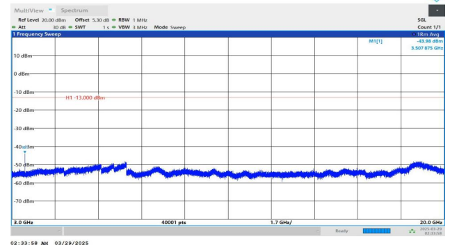
Band4-15MHz-QPSK-20325-1RB#74-3000~20000-PASS
