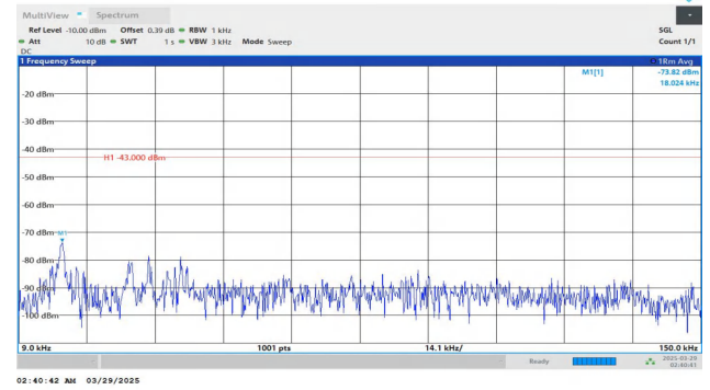
Band4-20MHz-QPSK-20300-1RB#99-0.009~0.15-PASS
