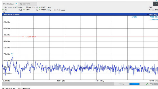
Band4-15MHz-QPSK-20325-1RB#0-0.009~0.15-PASS
