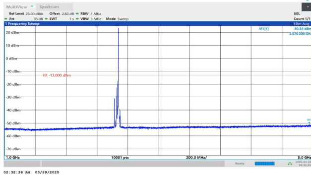
Band4-15MHz-QPSK-20175-1RB#74-1000~3000-PASS
