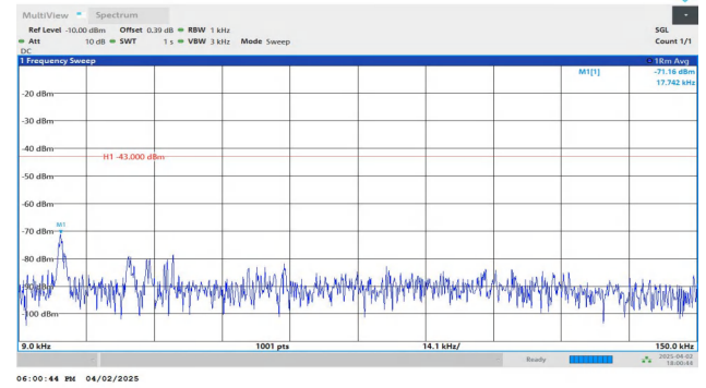
Band4-10MHz-QPSK-20000-1RB#49-0.009~0.15-PASS
