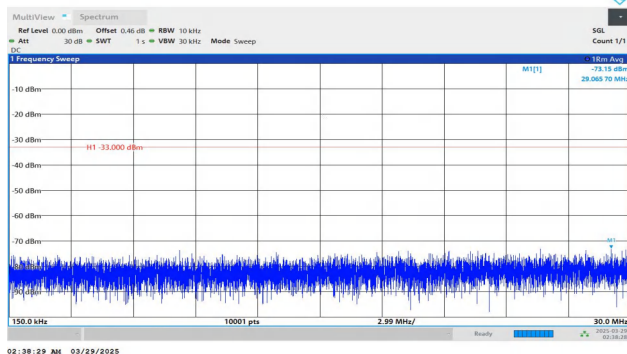
Band4-20MHz-QPSK-20050-1RB#99-0.15~30-PASS
