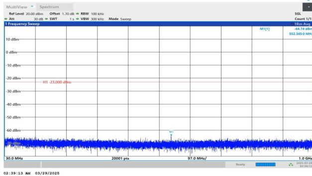
Band4-20MHz-QPSK-20175-1RB#0-30~1000-PASS
