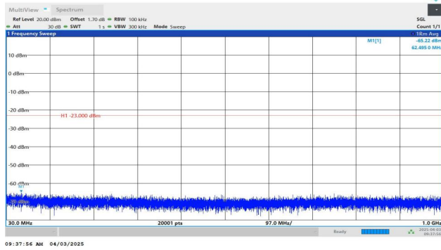
Band4-10MHz-QPSK-20175-1RB#0-30~1000-PASS
