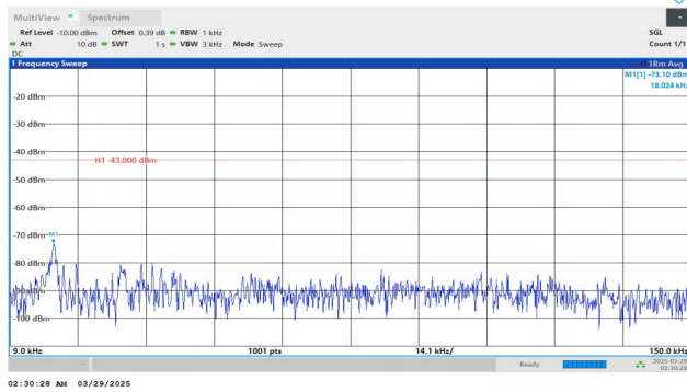
Band4-15MHz-QPSK-20025-1RB#0-0.009~0.15-PASS
