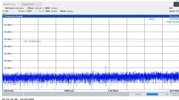
Band4-10MHz-QPSK-20350-1RB#49-0.15~30-PASS
