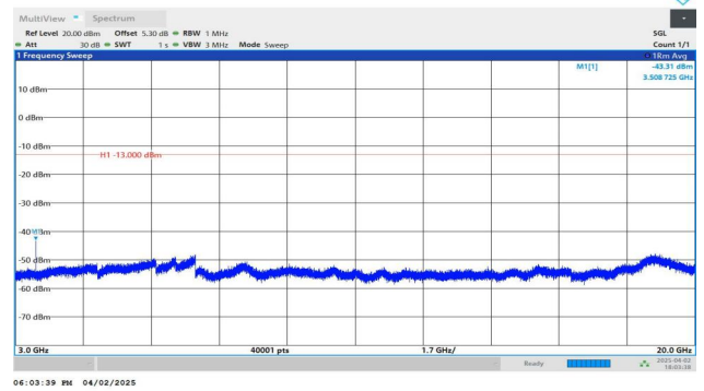
Band4-10MHz-QPSK-20350-1RB#49-3000~20000-PASS
