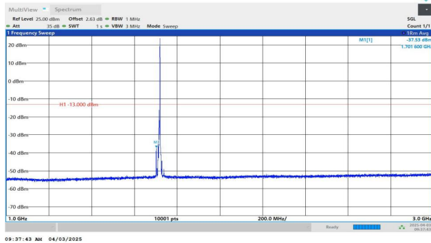
Band4-10MHz-QPSK-20000-1RB#49-1000~3000-PASS
