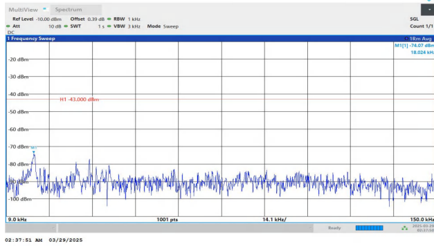
Band4-20MHz-QPSK-20050-1RB#0-0.009~0.15-PASS
