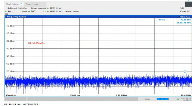
Band4-20MHz-QPSK-20300-1RB#0-0.15~30-PASS
