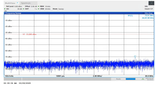
Band4-20MHz-QPSK-20175-1RB#0-0.15~30-PASS
