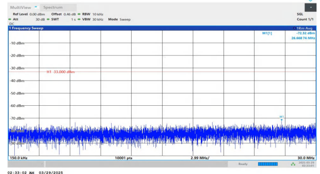
Band4-15MHz-QPSK-20325-1RB#0-0.15~30-PASS
