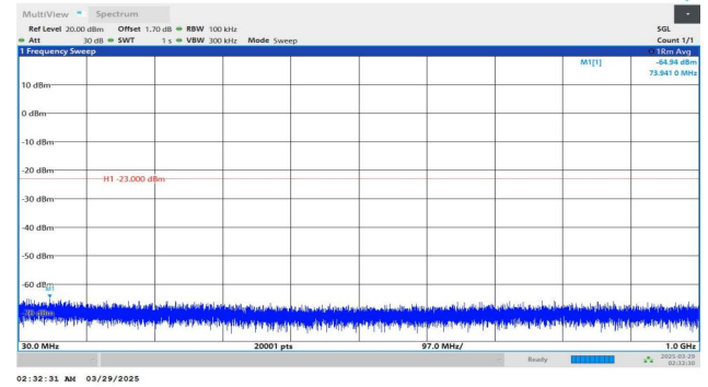
Band4-15MHz-QPSK-20175-1RB#74-30~1000-PASS
