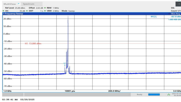
Band4-20MHz-QPSK-20050-1RB#99-1000~3000-PASS
