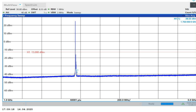
Band4-10MHz-QPSK-20350-1RB#49-1000~3000-PASS
