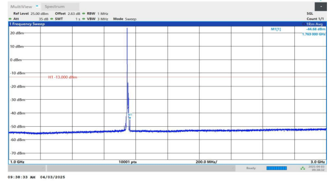
Band4-10MHz-QPSK-20350-1RB#0-1000~3000-PASS
