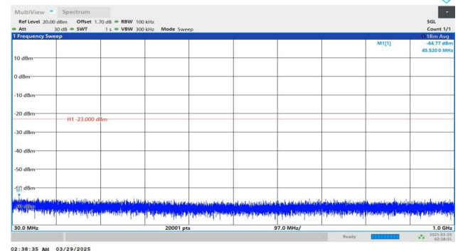
Band4-20MHz-QPSK-20050-1RB#99-30~1000-PASS
