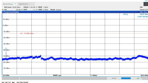
Band4-20MHz-QPSK-20175-1RB#0-3000~20000-PASS
