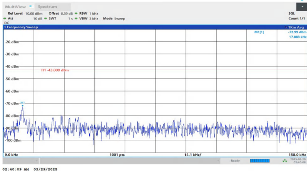
Band4-20MHz-QPSK-20300-1RB#0-0.009~0.15-PASS
