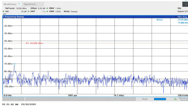
Band4-15MHz-QPSK-20175-1RB#0-0.009~0.15-PASS
