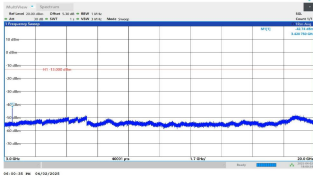
Band4-10MHz-QPSK-20000-1RB#0-3000~20000-PASS
