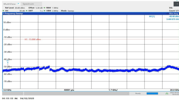
Band4-10MHz-QPSK-20350-1RB#0-3000~20000-PASS
