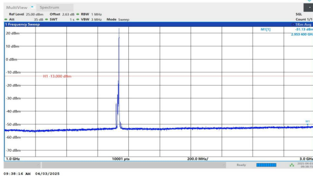
Band4-10MHz-QPSK-20175-1RB#49-1000~3000-PASS
