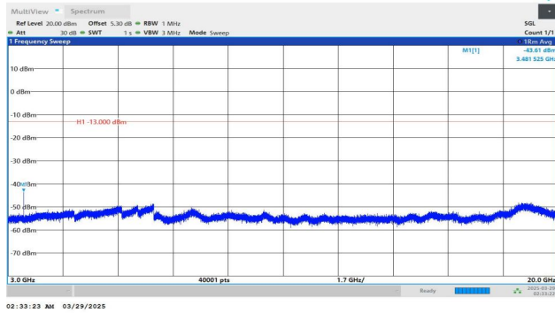
Band4-15MHz-QPSK-20325-1RB#0-3000~20000-PASS
