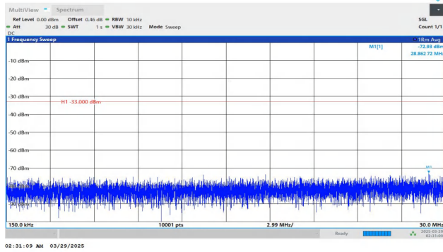
Band4-15MHz-QPSK-20025-1RB#74-0.15~30-PASS
