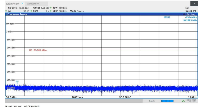
Band4-15MHz-QPSK-20325-1RB#74-30~1000-PASS
