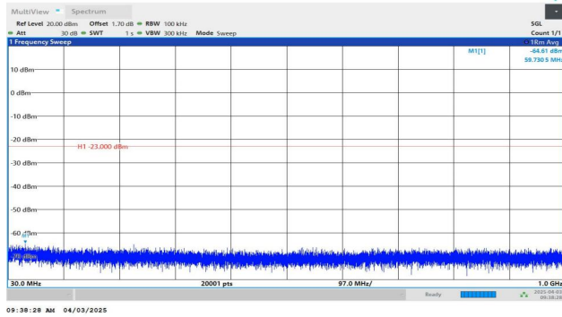
Band4-10MHz-QPSK-20350-1RB#0-30~1000-PASS
