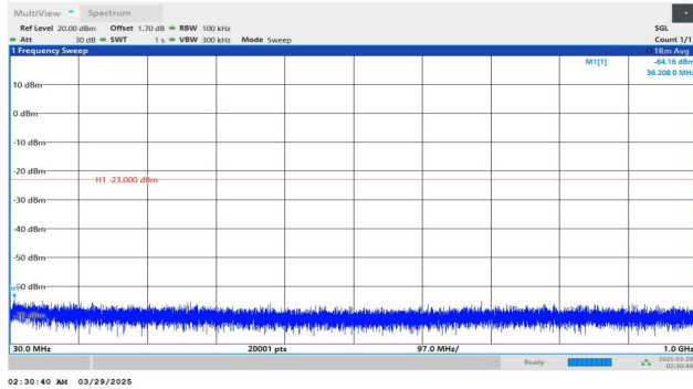
Band4-15MHz-QPSK-20025-1RB#0-30~1000-PASS
