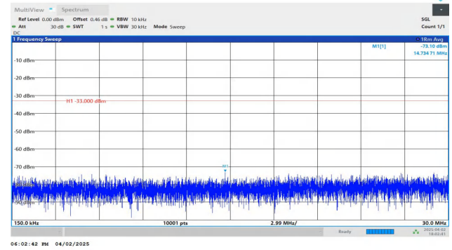
Band4-10MHz-QPSK-20350-1RB#0-0.15~30-PASS
