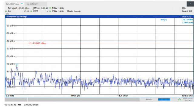
Band4-15MHz-QPSK-20325-1RB#74-0.009~0.15-PASS
