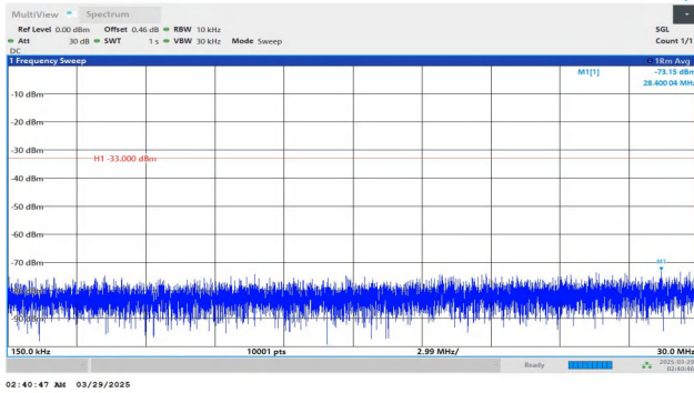
Band4-20MHz-QPSK-20300-1RB#99-0.15~30-PASS
