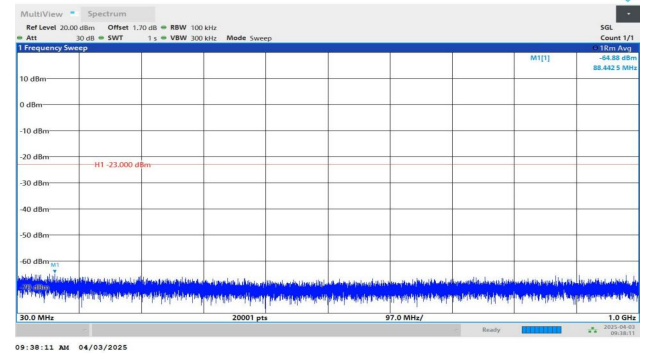
Band4-10MHz-QPSK-20175-1RB#49-30~1000-PASS
