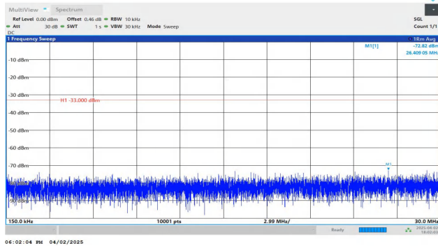
Band4-10MHz-QPSK-20175-1RB#49-0.15~30-PASS
