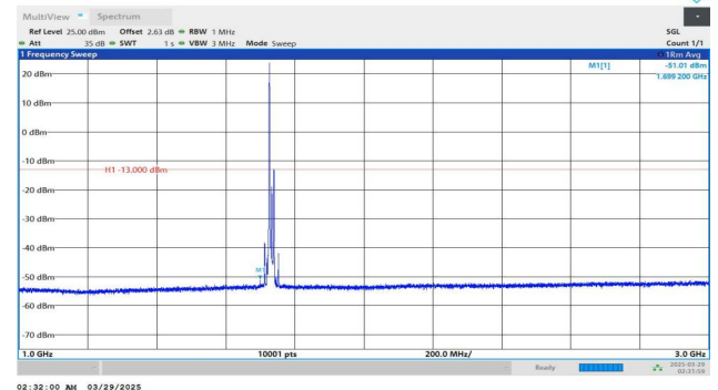
Band4-15MHz-QPSK-20175-1RB#0-1000~3000-PASS
