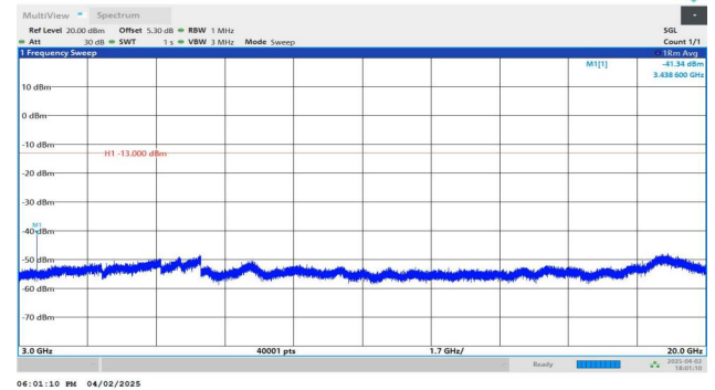
Band4-10MHz-QPSK-20000-1RB#49-3000~20000-PASS
