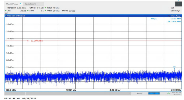
Band4-15MHz-QPSK-20175-1RB#0-0.15~30-PASS
