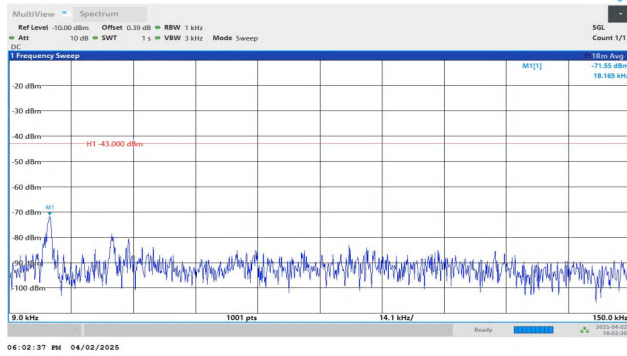
Band4-10MHz-QPSK-20350-1RB#0-0.009~0.15-PASS
