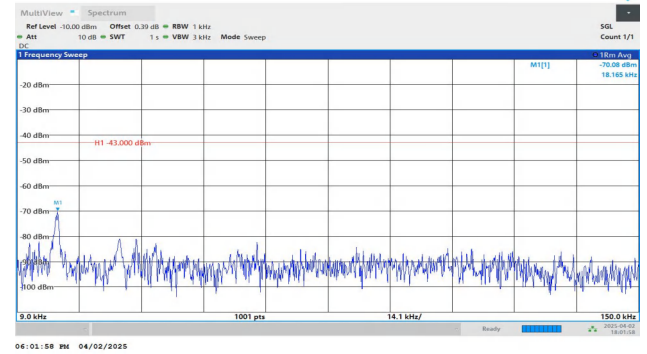
Band4-10MHz-QPSK-20175-1RB#49-0.009~0.15-PASS
