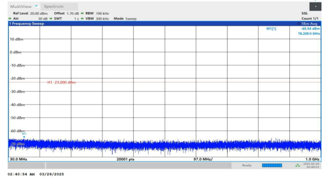
Band4-20MHz-QPSK-20300-1RB#99-30~1000-PASS
