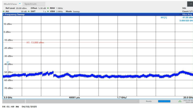
Band4-10MHz-QPSK-20175-1RB#0-3000~20000-PASS
