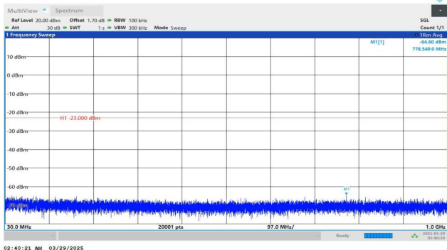
Band4-20MHz-QPSK-20300-1RB#0-30~1000-PASS
