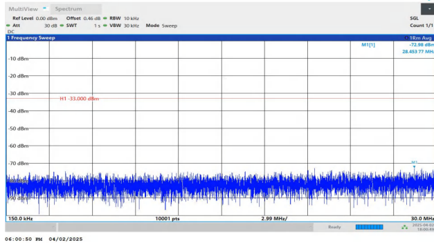
Band4-10MHz-QPSK-20000-1RB#49-0.15~30-PASS
