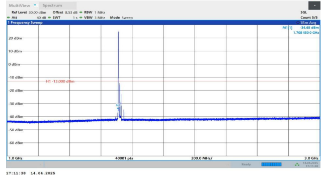
Band4-15MHz-QPSK-20025-1RB#0-1000~3000-PASS
