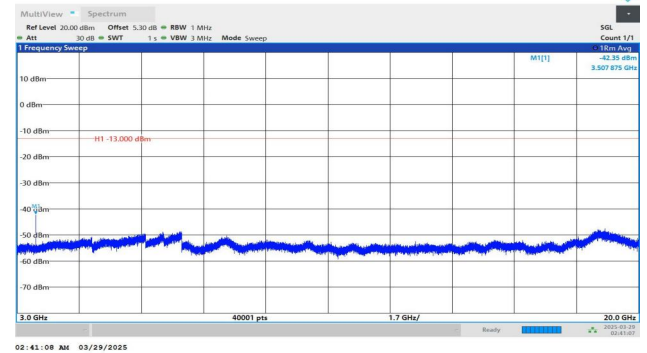
Band4-20MHz-QPSK-20300-1RB#99-3000~20000-PASS
