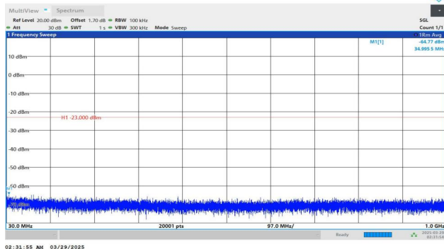
Band4-15MHz-QPSK-20175-1RB#0-30~1000-PASS
