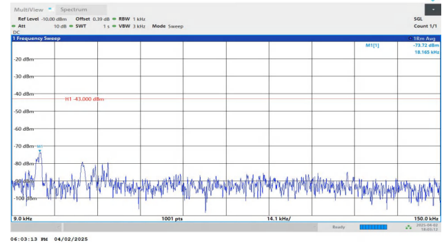
Band4-10MHz-QPSK-20350-1RB#49-0.009~0.15-PASS
