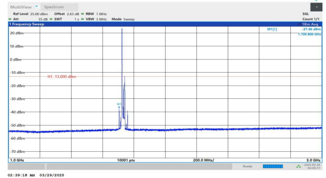
Band4-20MHz-QPSK-20175-1RB#0-1000~3000-PASS
