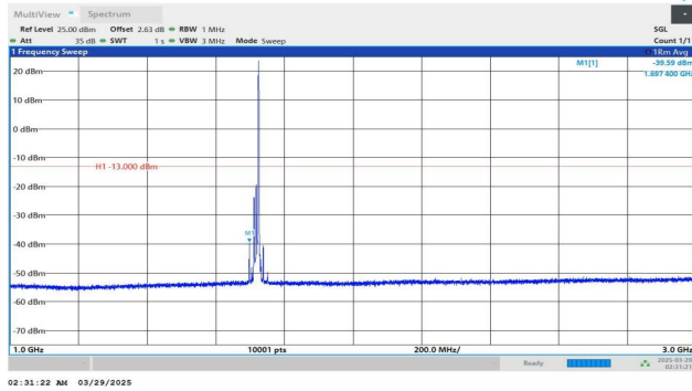
Band4-15MHz-QPSK-20025-1RB#74-1000~3000-PASS
