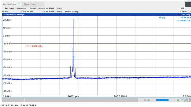
Band4-20MHz-QPSK-20300-1RB#99-1000~3000-PASS
