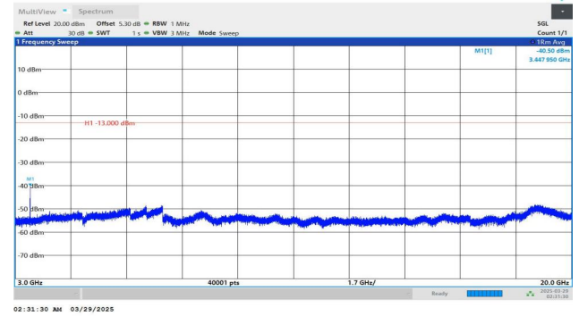
Band4-15MHz-QPSK-20025-1RB#74-3000~20000-PASS
