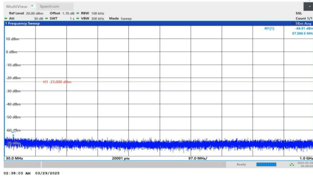
Band4-20MHz-QPSK-20050-1RB#0-30~1000-PASS
