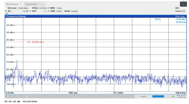
Band4-15MHz-QPSK-20175-1RB#74-0.009~0.15-PASS
