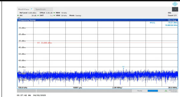
Band4-5MHz-QPSK-20175-1RB#0-0.15~30-PASS
