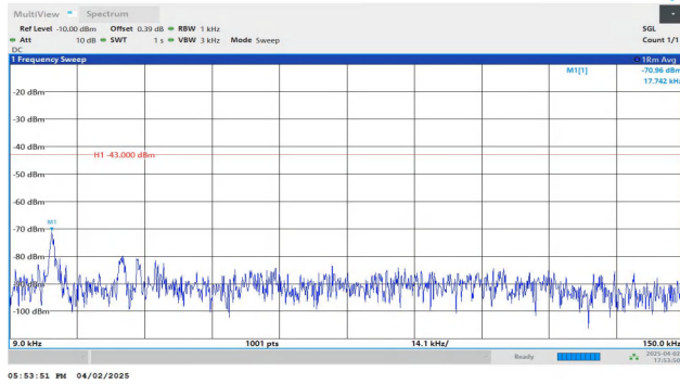
Band4-3MHz-QPSK-20175-1RB#0-0.009~0.15-PASS
