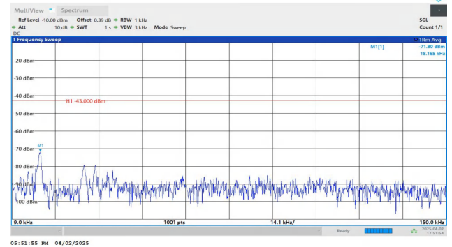
Band4-1.4MHz-QPSK-20393-1RB#5-0.009~0.15-PASS
