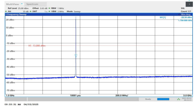
Band4-1.4MHz-QPSK-20393-1RB#0-1000~3000-PASS
