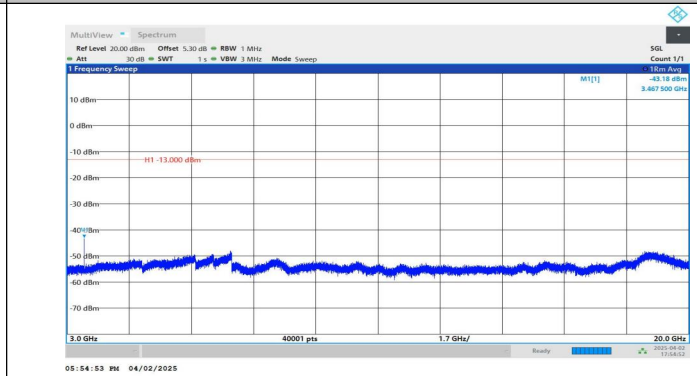
Band4-3MHz-QPSK-20175-1RB#14-3000~20000-PASS
