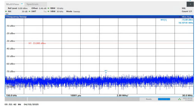
Band4-3MHz-QPSK-19965-1RB#0-0.15~30-PASS
