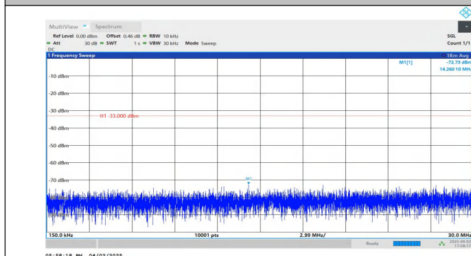
Band4-5MHz-QPSK-20175-1RB#24-0.15~30-PASS
