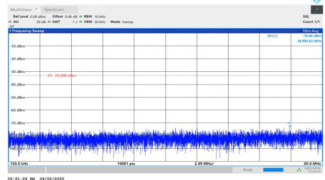
Band4-1.4MHz-QPSK-20393-1RB#0-0.15~30-PASS
