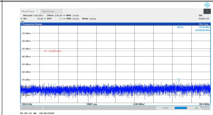
Band4-3MHz-QPSK-20385-1RB#0-0.15~30-PASS
