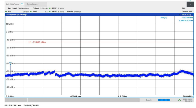
Band4-5MHz-QPSK-20175-1RB#24-3000~20000-PASS
