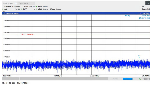
Band4-1.4MHz-QPSK-19957-1RB#5-0.15~30-PASS
