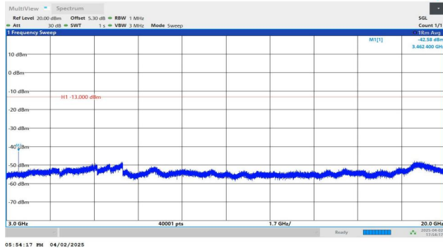
Band4-3MHz-QPSK-20175-1RB#0-3000~20000-PASS
