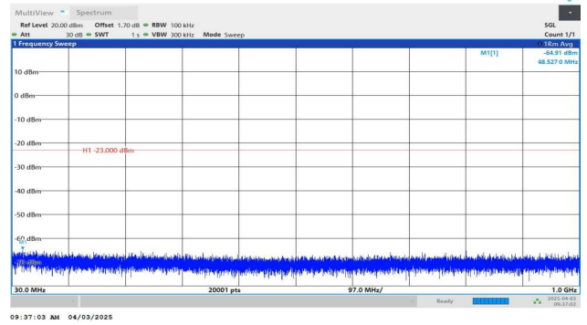
Band4-5MHz-QPSK-20375-1RB#24-30~1000-PASS
