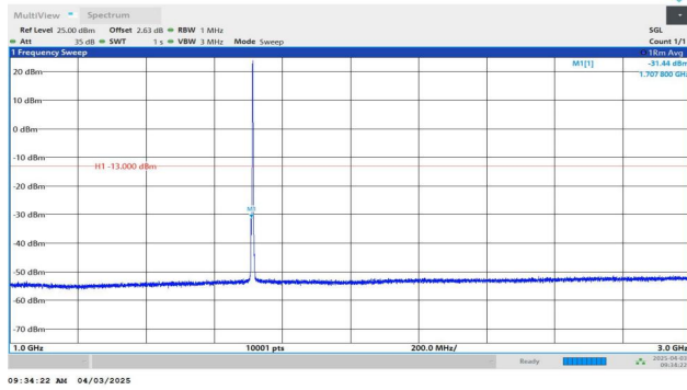
Band4-3MHz-QPSK-19965-1RB#14-1000~3000-PASS
