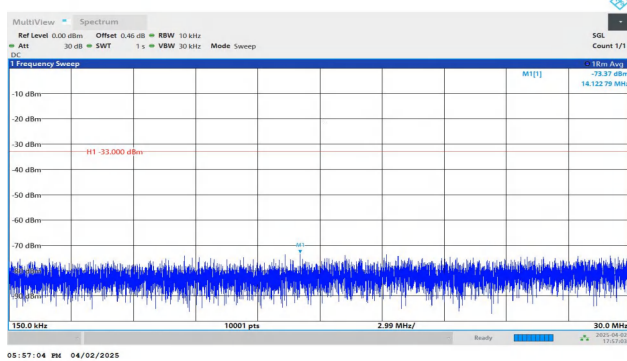
Band4-5MHz-QPSK-19975-1RB#24-0.15~30-PASS
