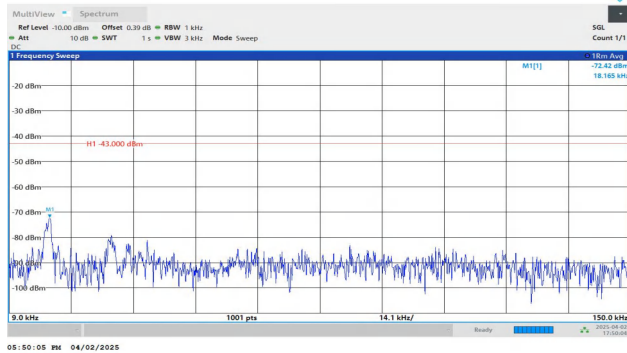
Band4-1.4MHz-QPSK-20175-1RB#0-0.009~0.15-PASS
