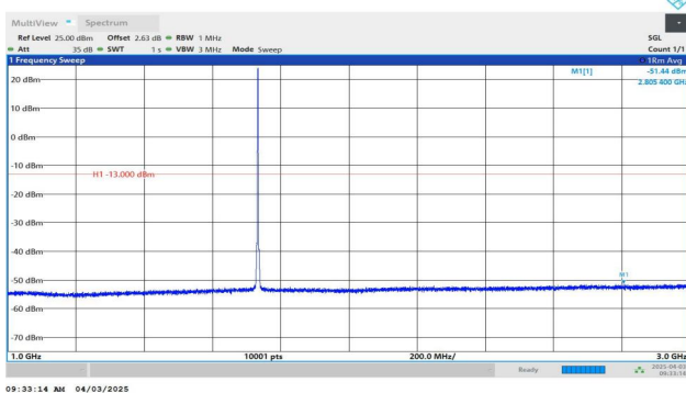
Band4-1.4MHz-QPSK-20175-1RB#5-1000~3000-PASS
