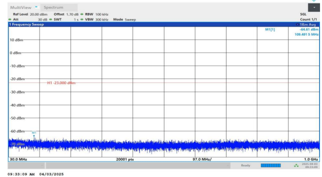
Band4-1.4MHz-QPSK-20175-1RB#5-30~1000-PASS
