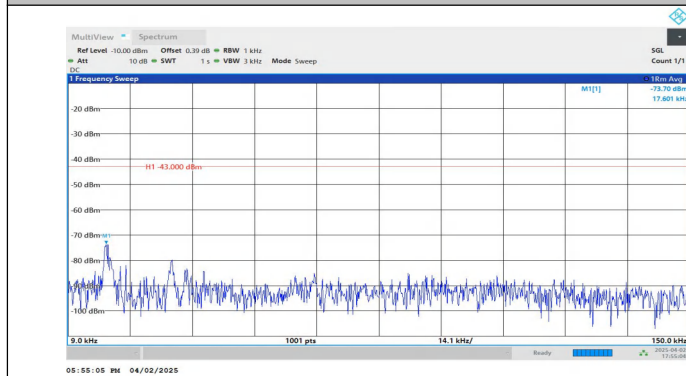
Band4-3MHz-QPSK-20385-1RB#0-0.009~0.15-PASS
