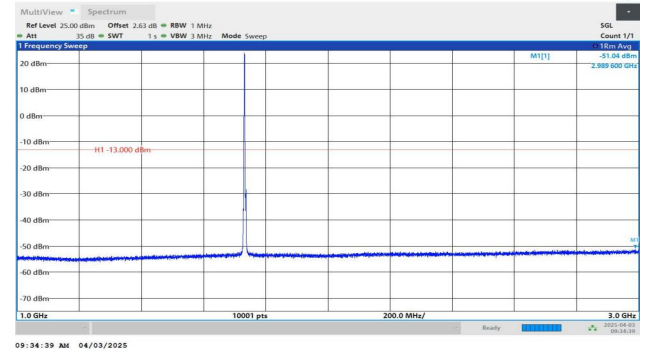
Band4-3MHz-QPSK-20175-1RB#0-1000~3000-PASS
