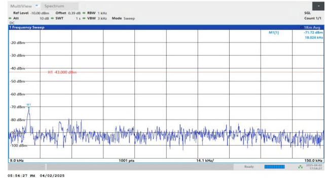
Band4-3MHz-QPSK-20175-1RB#14-0.009~0.15-PASS
