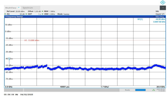
Band4-3MHz-QPSK-20385-1RB#14-3000~20000-PASS
