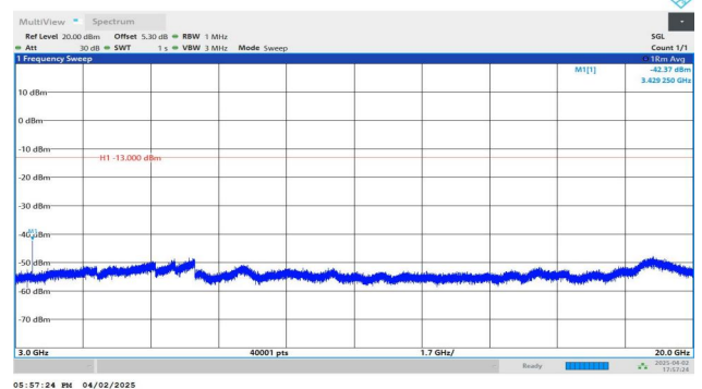
Band4-5MHz-QPSK-19975-1RB#24-3000~20000-PASS
