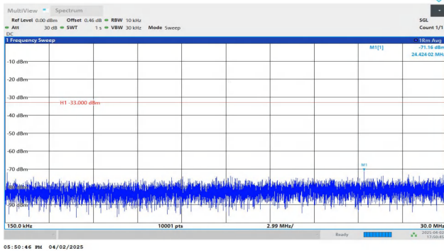
Band4-1.4MHz-QPSK-20175-1RB#5-0.15~30-PASS
