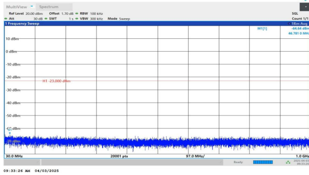
Band4-1.4MHz-QPSK-20393-1RB#0-30~1000-PASS
