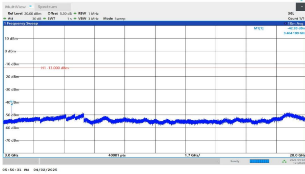
Band4-1.4MHz-QPSK-20175-1RB#0-3000~20000-PASS
