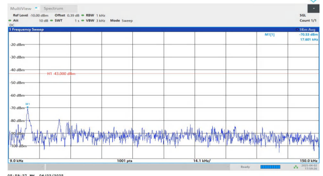
Band4-5MHz-QPSK-20375-1RB#24-0.009~0.15-PASS
