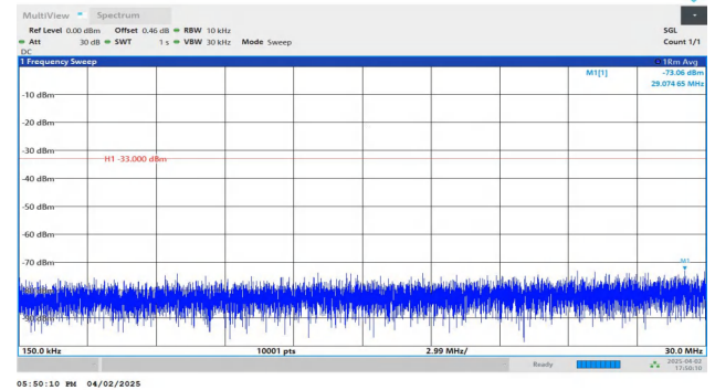
Band4-1.4MHz-QPSK-20175-1RB#0-0.15~30-PASS
