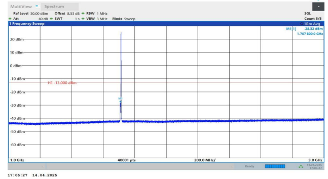
Band4-3MHz-QPSK-19965-1RB#0-1000~3000-PASS
