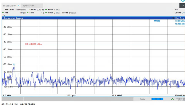
Band4-1.4MHz-QPSK-20393-1RB#0-0.009~0.15-PASS
