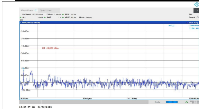
Band4-5MHz-QPSK-20175-1RB#0-0.009~0.15-PASS
