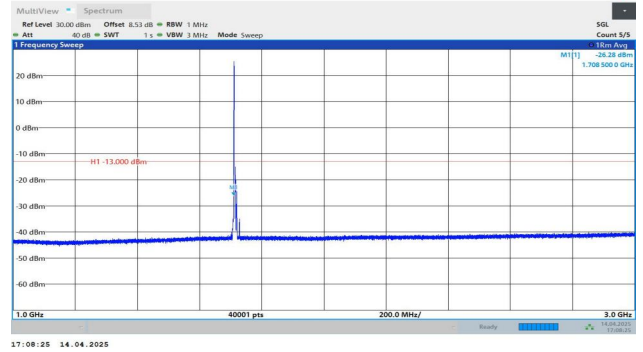
Band4-10MHz-QPSK-20000-1RB#0-1000~3000-PASS
