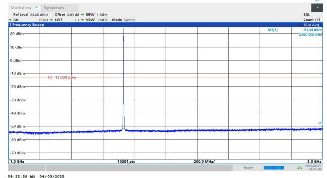
Band4-1.4MHz-QPSK-20175-1RB#0-1000~3000-PASS
