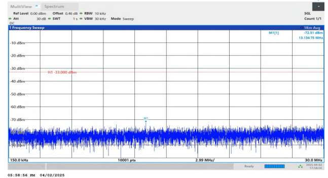
Band4-5MHz-QPSK-20375-1RB#0-0.15~30-PASS
