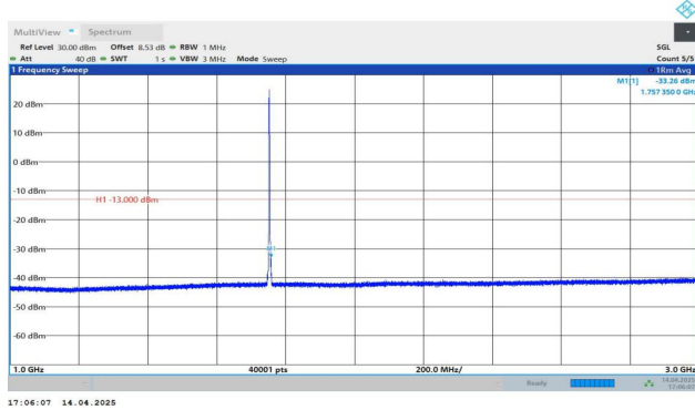
Band4-3MHz-QPSK-20385-1RB#14-1000~3000-PASS
