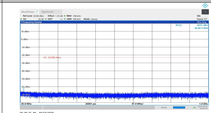
Band4-5MHz-QPSK-20175-1RB#24-30~1000-PASS
