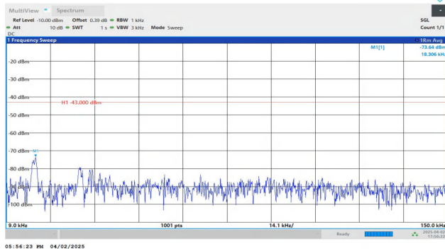
Band4-5MHz-QPSK-19975-1RB#0-0.009~0.15-PASS
