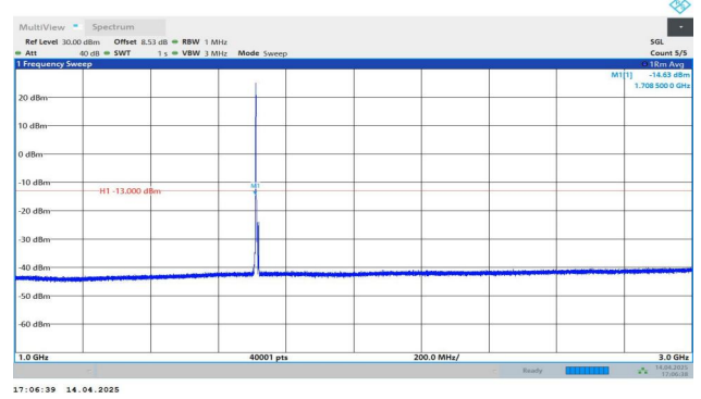
Band4-5MHz-QPSK-19975-1RB#0-1000~3000-PASS
