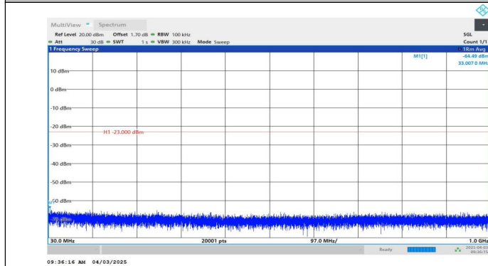
Band4-5MHz-QPSK-20175-1RB#0-30~1000-PASS
