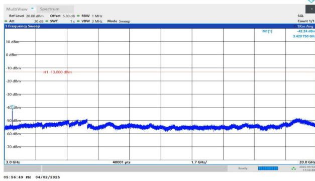
Band4-5MHz-QPSK-19975-1RB#0-3000~20000-PASS
