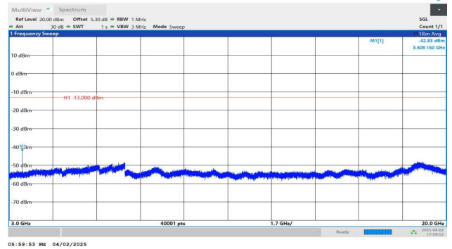
Band4-5MHz-QPSK-20375-1RB#24-3000~20000-PASS
