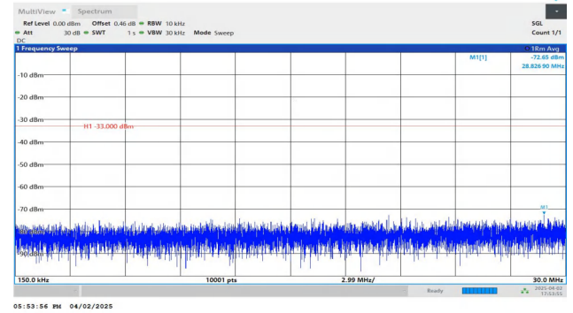
Band4-3MHz-QPSK-20175-1RB#0-0.15~30-PASS
