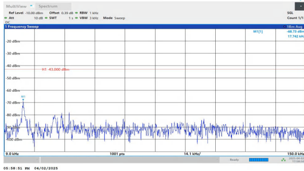
Band4-5MHz-QPSK-20375-1RB#0-0.009~0.15-PASS
