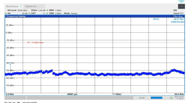
Band4-1.4MHz-QPSK-20393-1RB#5-3000~20000-PASS
