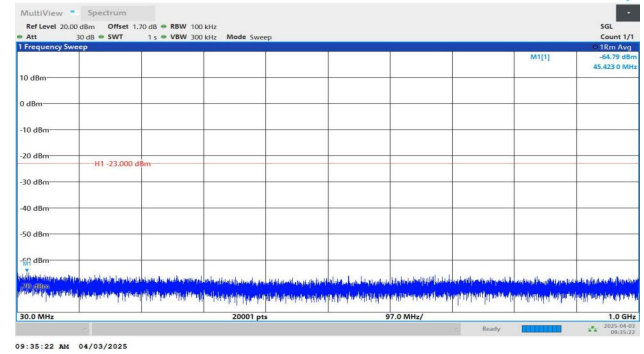
Band4-3MHz-QPSK-20385-1RB#14-30~1000-PASS
