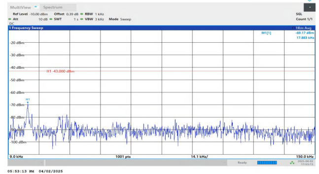
Band4-3MHz-QPSK-19965-1RB#14-0.009~0.15-PASS
