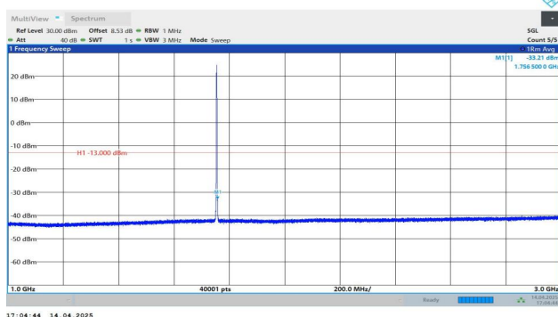
Band4-1.4MHz-QPSK-20393-1RB#5-1000~3000-PASS
