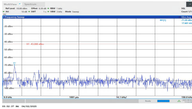
Band4-3MHz-QPSK-19965-1RB#0-0.009~0.15-PASS
