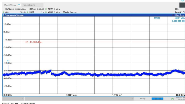
Band4-5MHz-QPSK-20375-1RB#0-3000~20000-PASS
