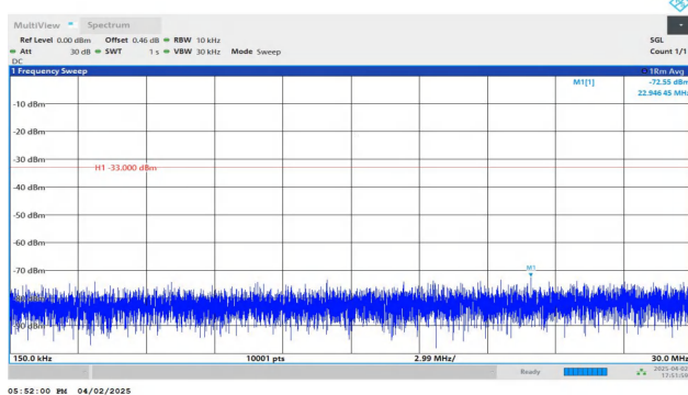
Band4-1.4MHz-QPSK-20393-1RB#5-0.15~30-PASS
