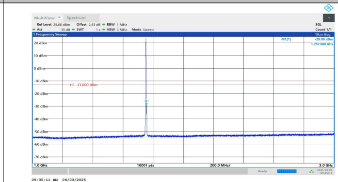
Band4-3MHz-QPSK-20385-1RB#0-1000~3000-PASS
