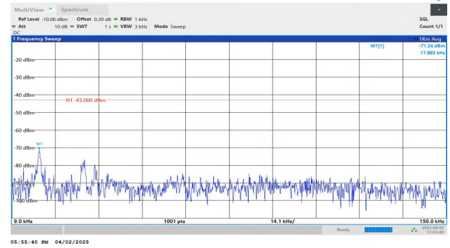
Band4-3MHz-QPSK-20385-1RB#14-0.009~0.15-PASS
