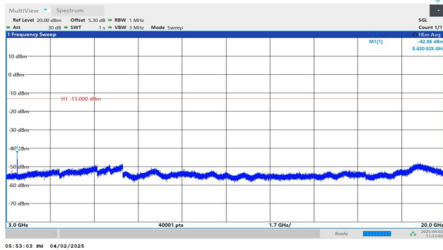
Band4-3MHz-QPSK-19965-1RB#0-3000~20000-PASS
