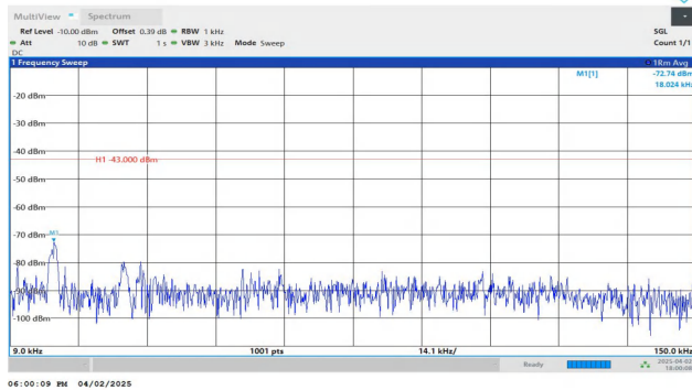
Band4-10MHz-QPSK-20000-1RB#0-0.009~0.15-PASS
