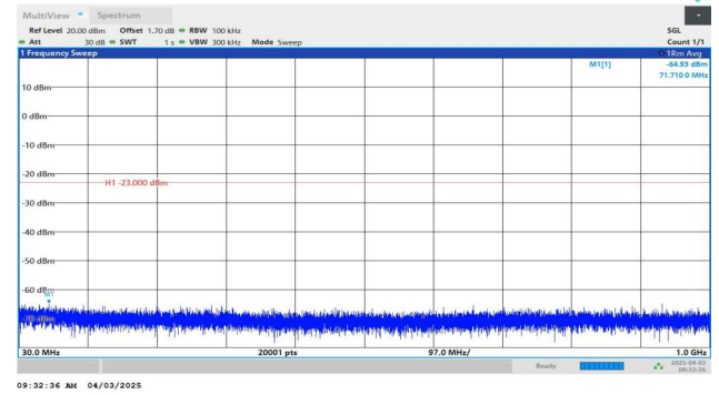
Band4-1.4MHz-QPSK-19957-1RB#5-30~1000-PASS
