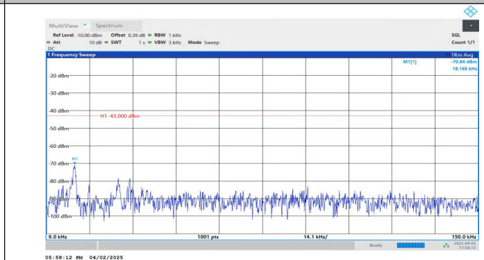
Band4-5MHz-QPSK-20175-1RB#24-0.009~0.15-PASS
