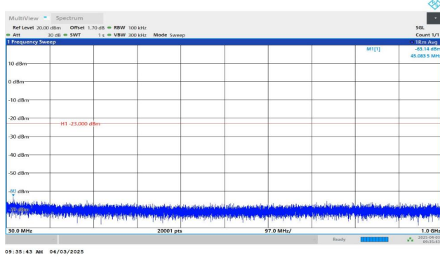
Band4-5MHz-QPSK-19975-1RB#0-30~1000-PASS
