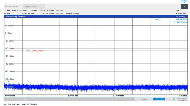
Band4-5MHz-QPSK-19975-1RB#24-30~1000-PASS
