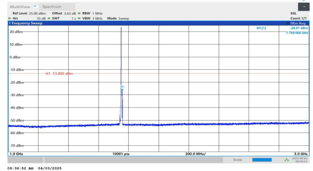
Band4-5MHz-QPSK-20375-1RB#0-1000~3000-PASS
