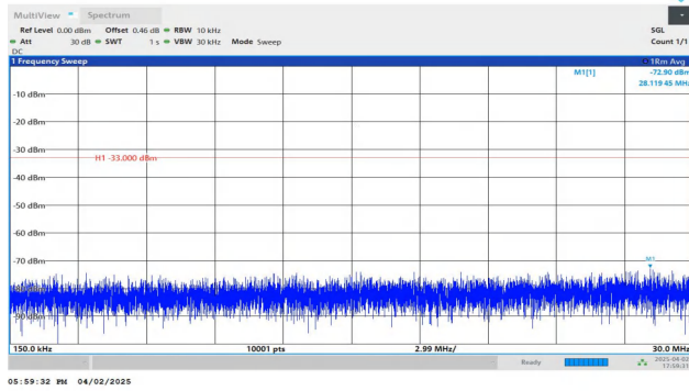
Band4-5MHz-QPSK-20375-1RB#24-0.15~30-PASS
