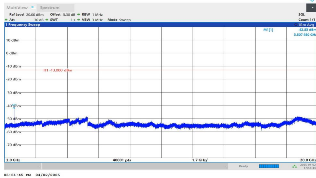
Band4-1.4MHz-QPSK-20393-1RB#0-3000~20000-PASS
