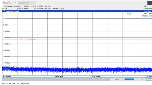
Band4-3MHz-QPSK-20175-1RB#0-30~1000-PASS
