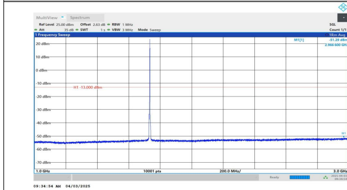
Band4-3MHz-QPSK-20175-1RB#14-1000~3000-PASS
