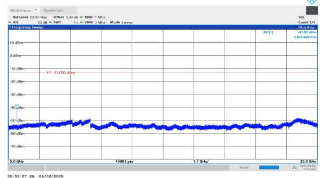
Band4-1.4MHz-QPSK-20175-1RB#5-3000~20000-PASS
