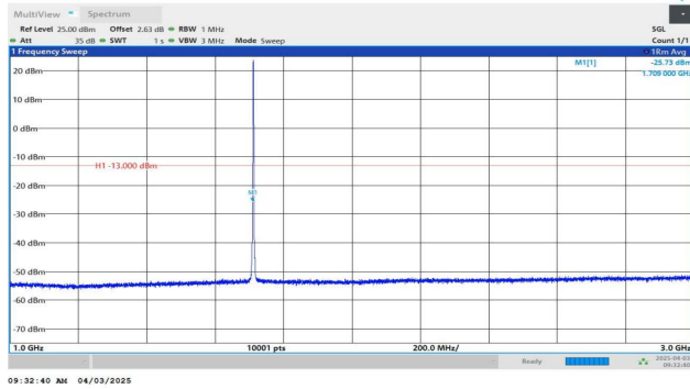
Band4-1.4MHz-QPSK-19957-1RB#5-1000~3000-PASS
