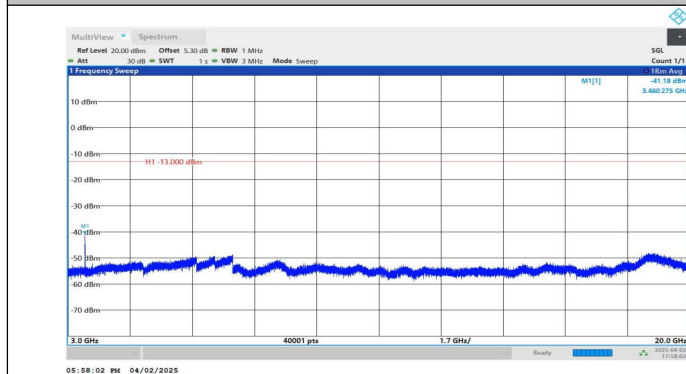
Band4-5MHz-QPSK-20175-1RB#0-3000~20000-PASS
