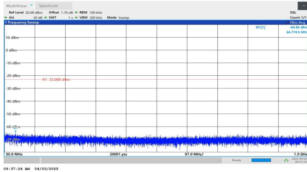
Band4-10MHz-QPSK-20000-1RB#0-30~1000-PASS
