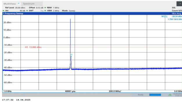
Band4-5MHz-QPSK-20375-1RB#24-1000~3000-PASS
