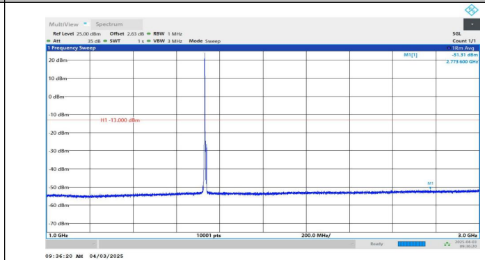
Band4-5MHz-QPSK-20175-1RB#0-1000~3000-PASS
