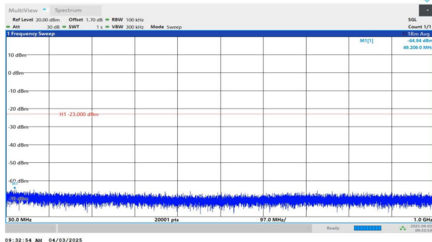
Band4-1.4MHz-QPSK-20175-1RB#0-30~1000-PASS
