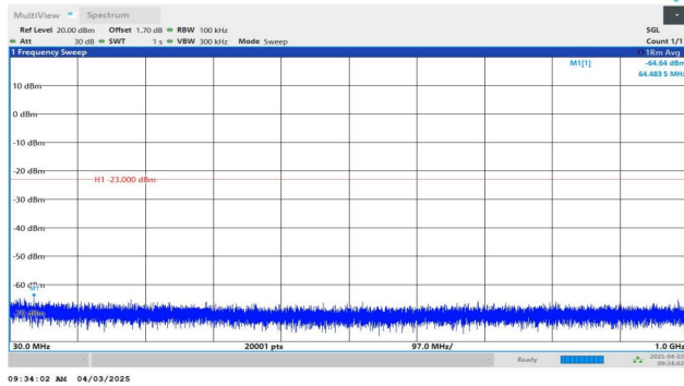
Band4-3MHz-QPSK-19965-1RB#0-30~1000-PASS
