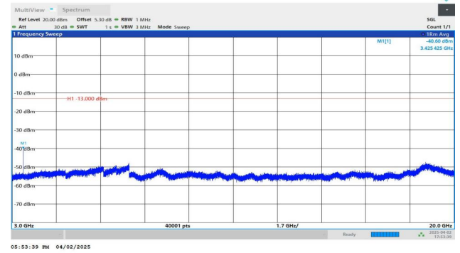
Band4-3MHz-QPSK-19965-1RB#14-3000~20000-PASS
