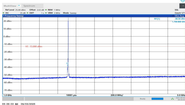
Band4-5MHz-QPSK-19975-1RB#24-1000~3000-PASS
