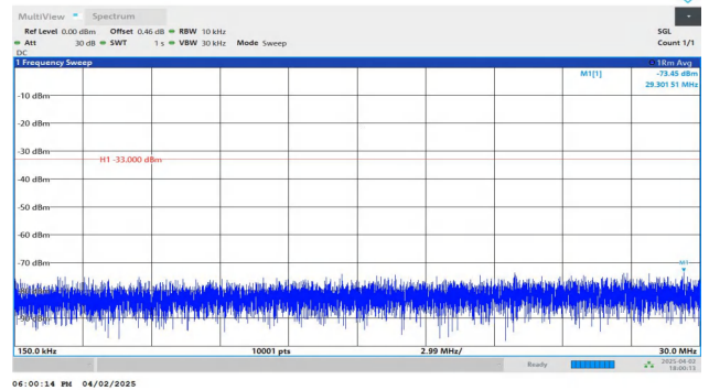
Band4-10MHz-QPSK-20000-1RB#0-0.15~30-PASS
