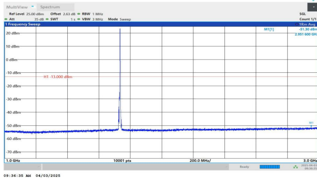
Band4-5MHz-QPSK-20175-1RB#24-1000~3000-PASS
