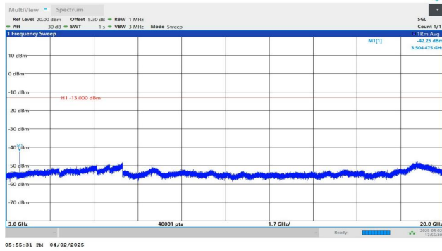
Band4-3MHz-QPSK-20385-1RB#0-3000~20000-PASS
