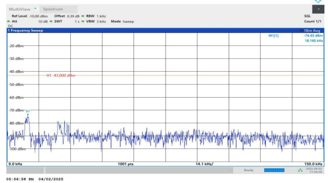
Band4-5MHz-QPSK-19975-1RB#24-0.009~0.15-PASS
