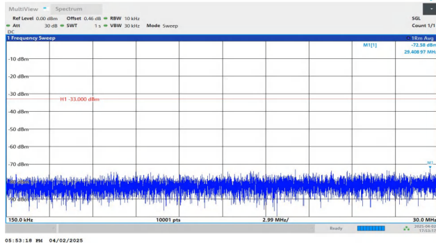
Band4-3MHz-QPSK-19965-1RB#14-0.15~30-PASS
