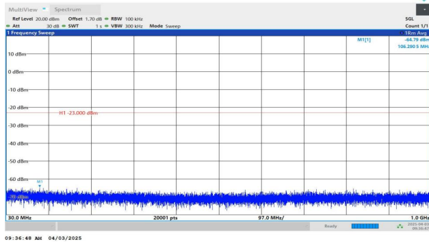
Band4-5MHz-QPSK-20375-1RB#0-30~1000-PASS
