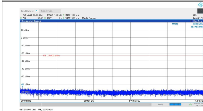
Band4-3MHz-QPSK-20385-1RB#0-30~1000-PASS
