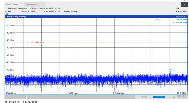
Band4-5MHz-QPSK-19975-1RB#0-0.15~30-PASS
