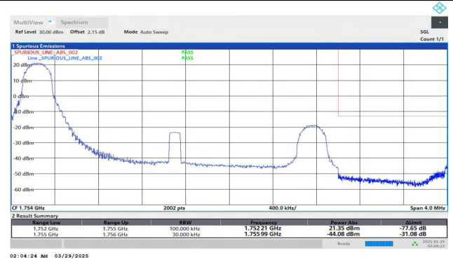
Band4-3MHz-QPSK-20385-1RB#0-PASS
