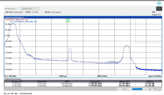
Band4-5MHz-QPSK-20375-1RB#0-PASS
