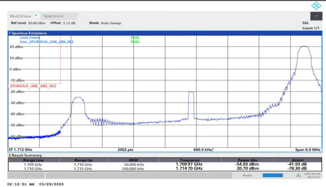
Band4-5MHz-QPSK-19975-1RB#24-PASS
