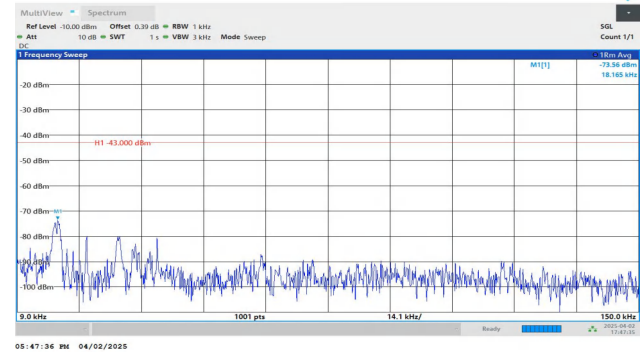
Band2-10MHz-QPSK-19150-1RB#49-0.009~0.15-PASS
