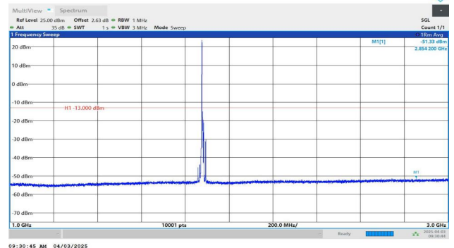
Band2-10MHz-QPSK-18900-1RB#0-1000~3000-PASS
