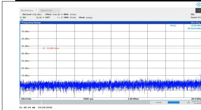
Band2-20MHz-QPSK-19100-1RB#99-0.15~30-PASS
