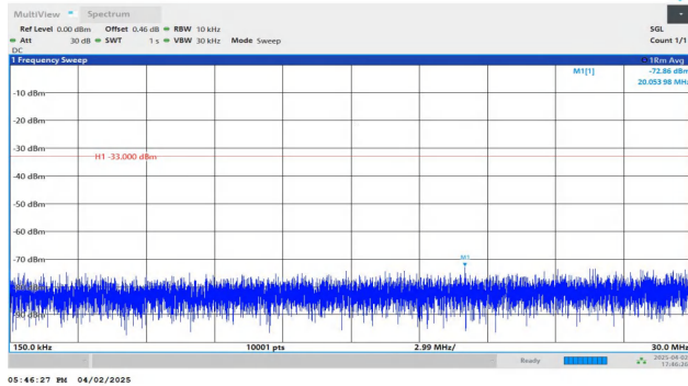
Band2-10MHz-QPSK-18900-1RB#49-0.15~30-PASS
