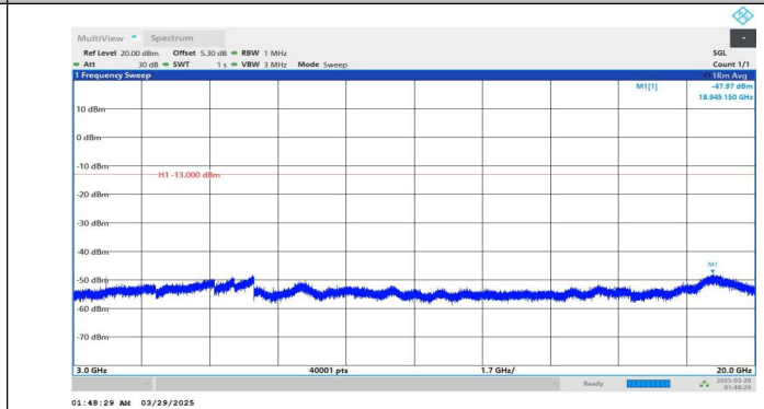
Band2-20MHz-QPSK-19100-1RB#99-3000~20000-PASS
