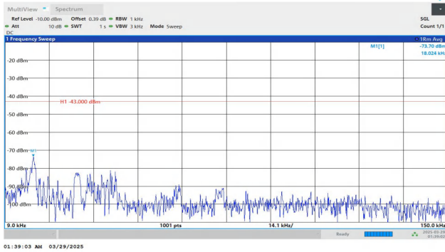
Band2-15MHz-QPSK-18900-1RB#0-0.009~0.15-PASS
