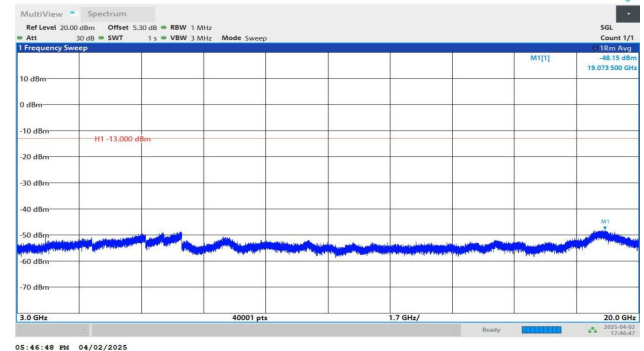
Band2-10MHz-QPSK-18900-1RB#49-3000~20000-PASS
