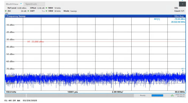
Band2-20MHz-QPSK-18900-1RB#0-0.15~30-PASS
