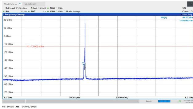
Band2-10MHz-QPSK-18650-1RB#49-1000~3000-PASS
