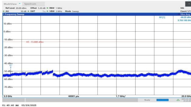
Band2-20MHz-QPSK-18700-1RB#0-3000~20000-PASS
