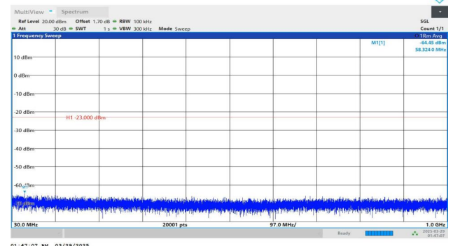
Band2-20MHz-QPSK-18900-1RB#99-30~1000-PASS
