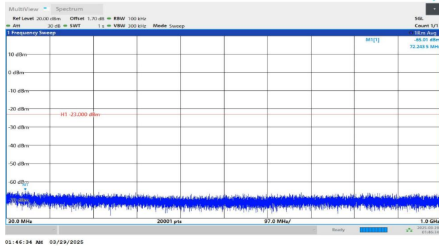
Band2-20MHz-QPSK-18900-1RB#0-30~1000-PASS
