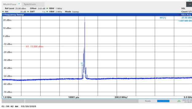
Band2-15MHz-QPSK-18675-1RB#74-1000~3000-PASS
