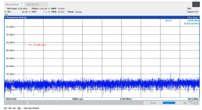
Band2-10MHz-QPSK-18900-1RB#0-0.15~30-PASS
