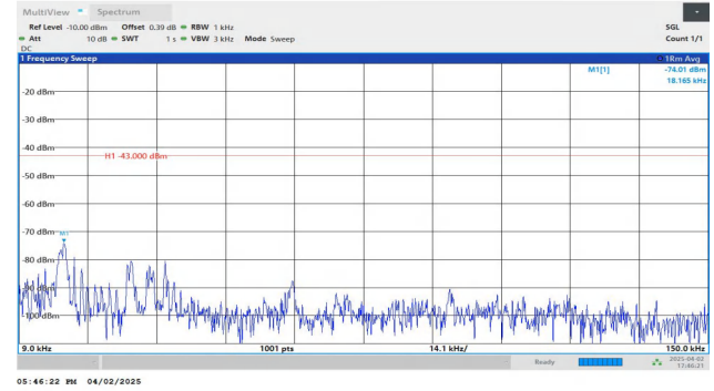
Band2-10MHz-QPSK-18900-1RB#49-0.009~0.15-PASS
