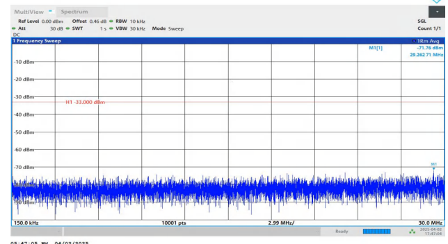
Band2-10MHz-QPSK-19150-1RB#0-0.15~30-PASS
