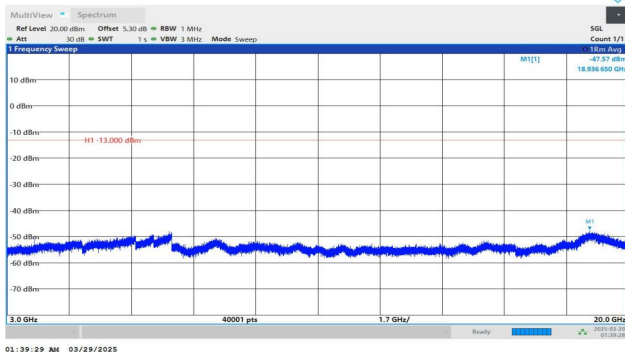
Band2-15MHz-QPSK-18900-1RB#0-3000~20000-PASS
