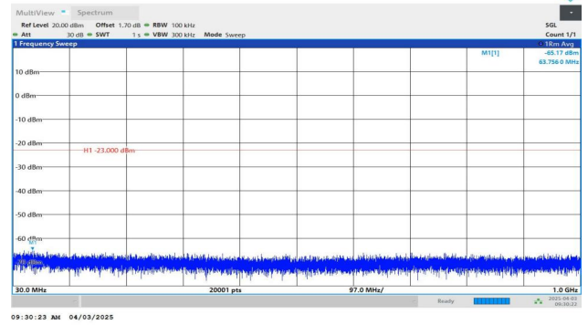
Band2-10MHz-QPSK-18650-1RB#49-30~1000-PASS
