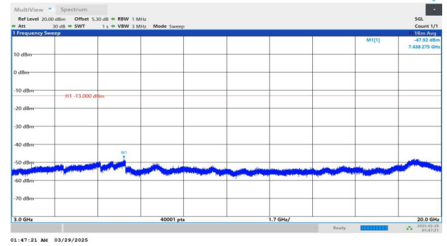
Band2-20MHz-QPSK-18900-1RB#99-3000~20000-PASS
