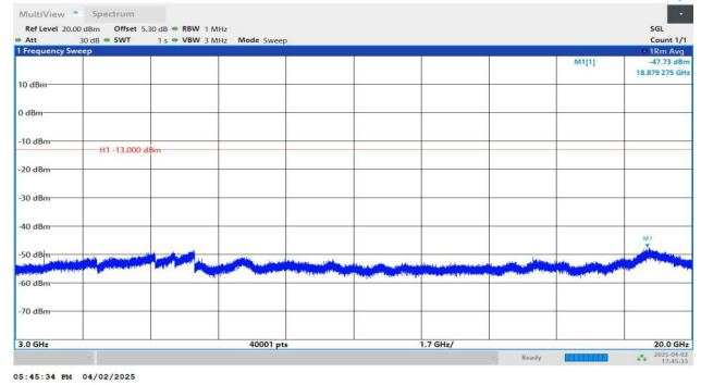
Band2-10MHz-QPSK-18650-1RB#49-3000~20000-PASS
