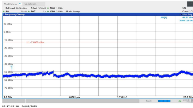
Band2-10MHz-QPSK-19150-1RB#0-3000~20000-PASS
