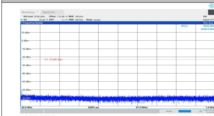
Band2-15MHz-QPSK-19125-1RB#0-30~1000-PASS
