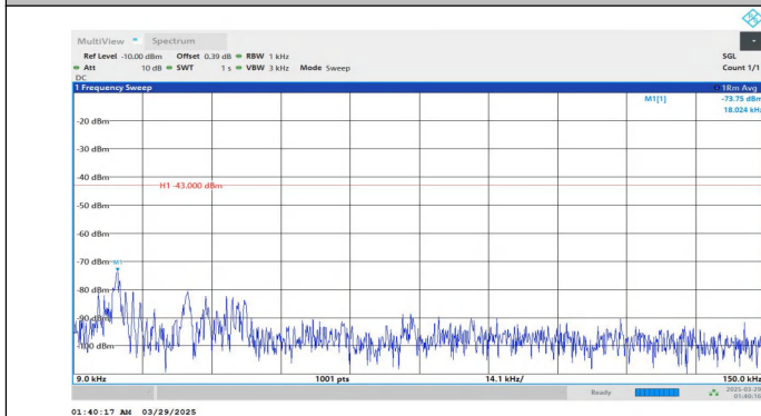
Band2-15MHz-QPSK-19125-1RB#0-0.009~0.15-PASS
