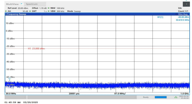
Band2-20MHz-QPSK-18700-1RB#99-30~1000-PASS
