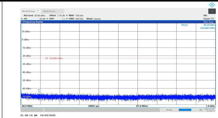
Band2-20MHz-QPSK-19100-1RB#99-30~1000-PASS
