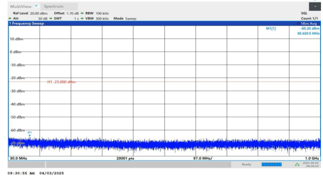
Band2-10MHz-QPSK-18900-1RB#49-30~1000-PASS
