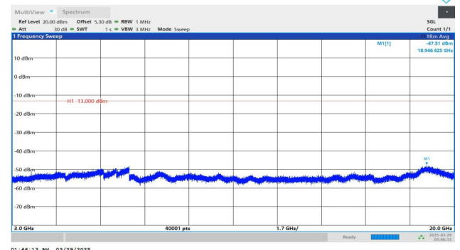
Band2-20MHz-QPSK-18700-1RB#99-3000~20000-PASS
