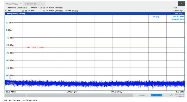
Band2-15MHz-QPSK-19125-1RB#74-30~1000-PASS
