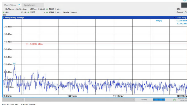
Band2-10MHz-QPSK-19150-1RB#0-0.009~0.15-PASS
