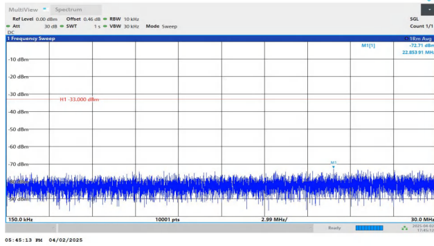
Band2-10MHz-QPSK-18650-1RB#49-0.15~30-PASS
