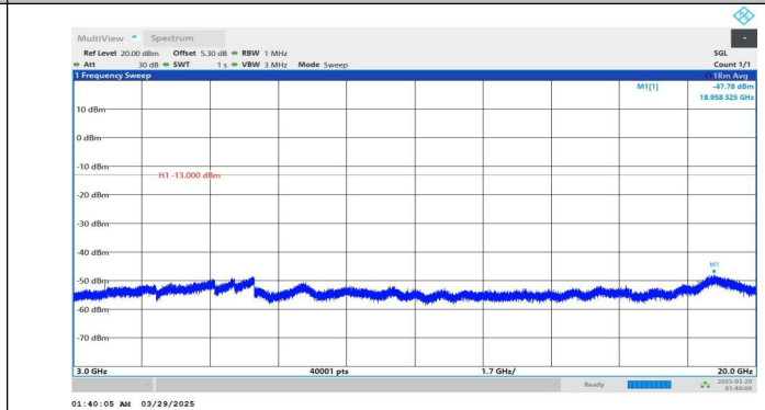
Band2-15MHz-QPSK-18900-1RB#74-3000~20000-PASS
