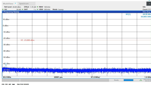
Band2-10MHz-QPSK-18900-1RB#0-30~1000-PASS
