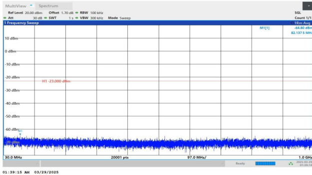
Band2-15MHz-QPSK-18900-1RB#0-30~1000-PASS
