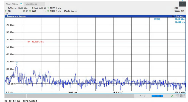
Band2-20MHz-QPSK-18900-1RB#99-0.009~0.15-PASS
