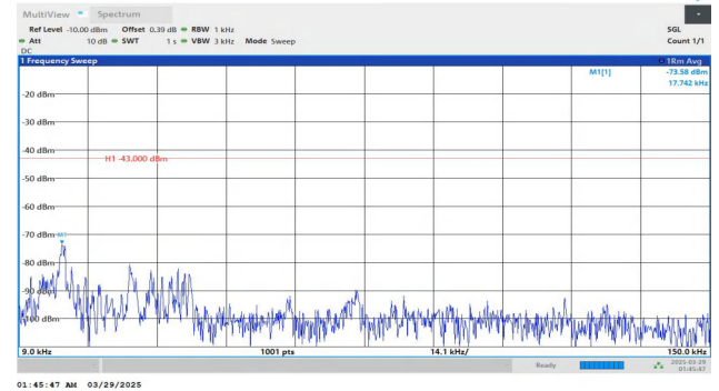
Band2-20MHz-QPSK-18700-1RB#99-0.009~0.15-PASS
