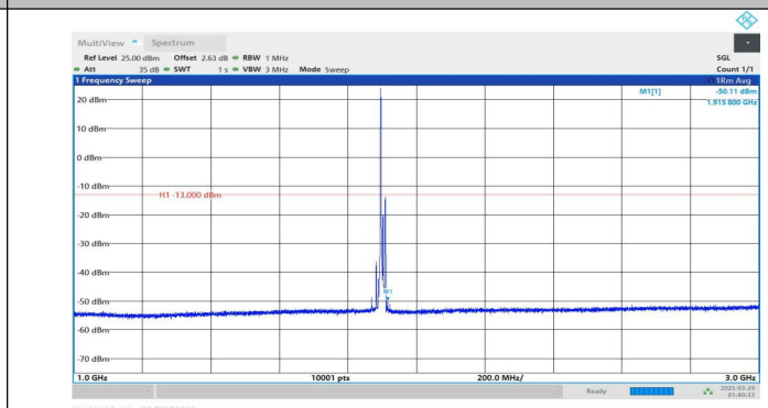
Band2-15MHz-QPSK-19125-1RB#0-1000~3000-PASS
