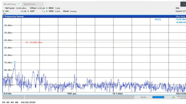
Band2-10MHz-QPSK-18900-1RB#0-0.009~0.15-PASS
