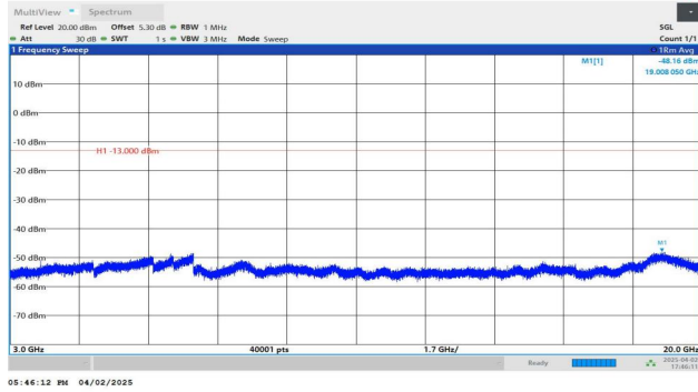
Band2-10MHz-QPSK-18900-1RB#0-3000~20000-PASS
