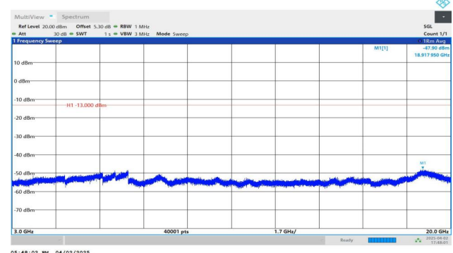
Band2-10MHz-QPSK-19150-1RB#49-3000~20000-PASS
