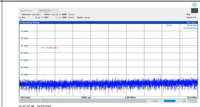
Band2-15MHz-QPSK-19125-1RB#0-0.15~30-PASS
