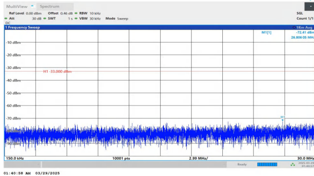
Band2-15MHz-QPSK-19125-1RB#74-0.15~30-PASS
