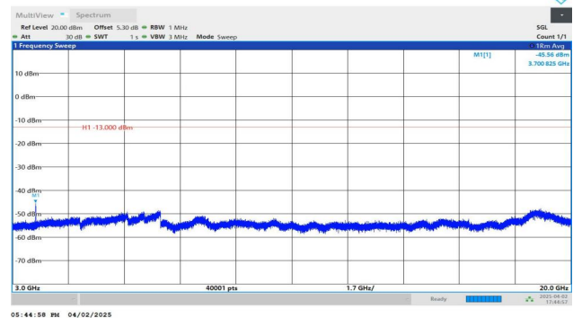
Band2-10MHz-QPSK-18650-1RB#0-3000~20000-PASS
