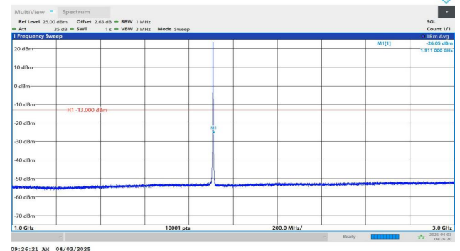
Band2-1.4MHz-QPSK-19193-1RB#0-1000~3000-PASS
