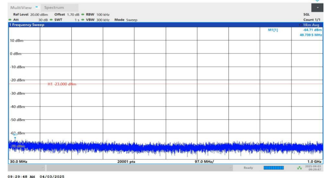
Band2-5MHz-QPSK-19175-1RB#24-30~1000-PASS
