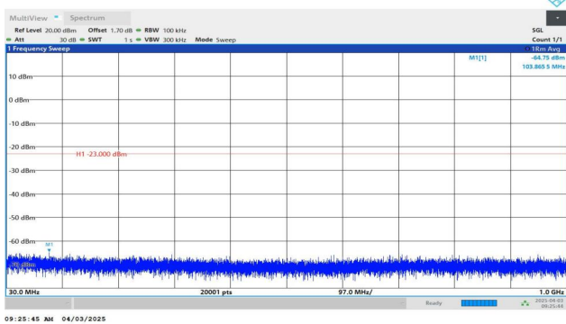
Band2-1.4MHz-QPSK-18900-1RB#0-30~1000-PASS
