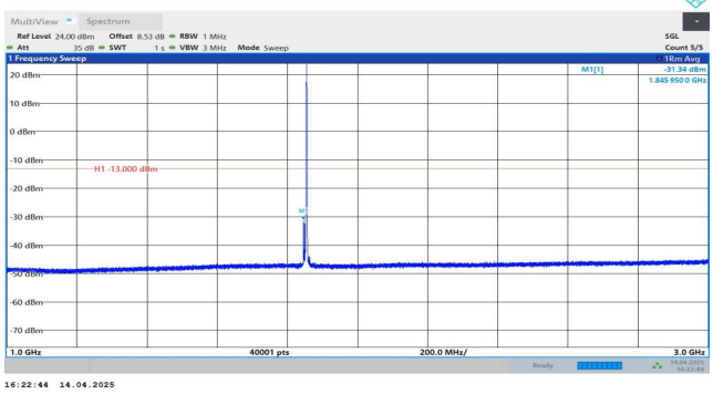
Band2-10MHz-QPSK-18650-1RB#0-1000~3000-PASS
