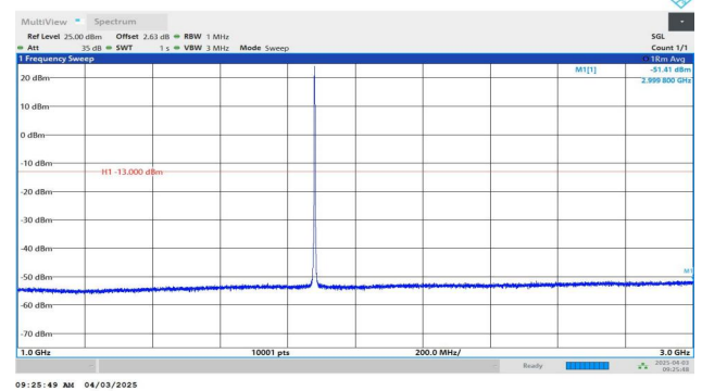
Band2-1.4MHz-QPSK-18900-1RB#0-1000~3000-PASS
