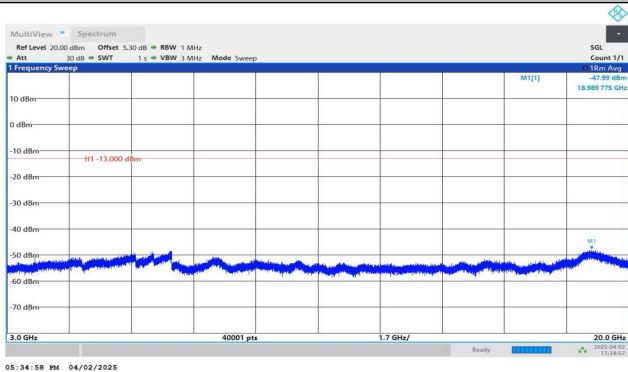
Band2-1.4MHz-QPSK-18900-1RB#0-3000~20000-PASS
