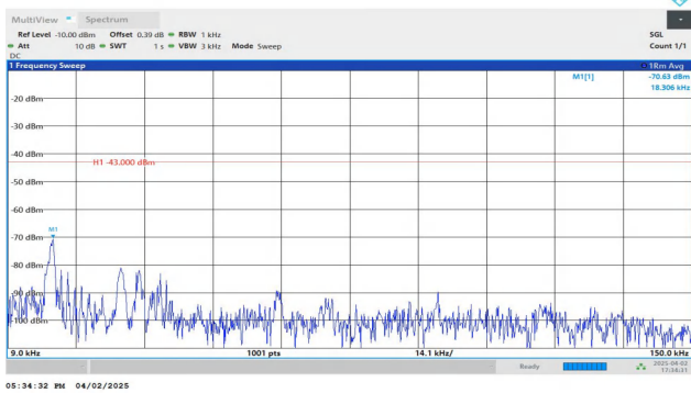
Band2-1.4MHz-QPSK-18900-1RB#0-0.009~0.15-PASS
