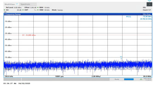
Band2-1.4MHz-QPSK-18900-1RB#0-0.15~30-PASS
