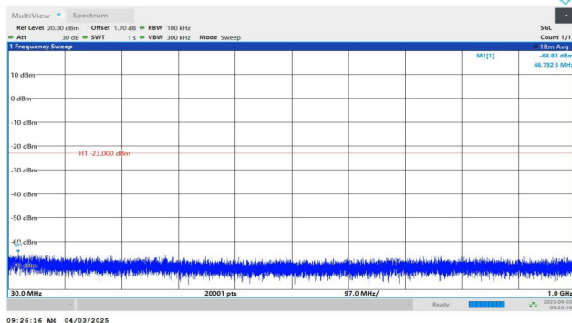
Band2-1.4MHz-QPSK-19193-1RB#0-30~1000-PASS
