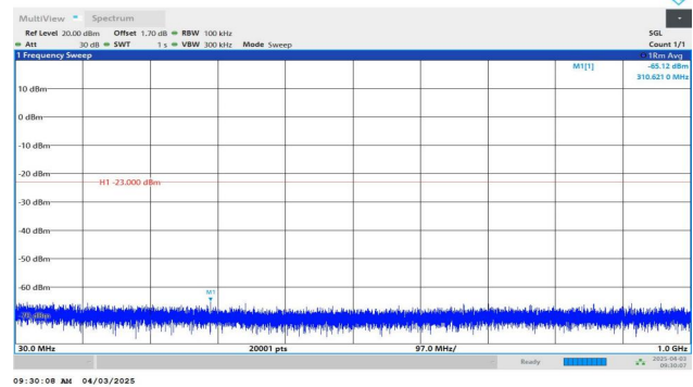
Band2-10MHz-QPSK-18650-1RB#0-30~1000-PASS
