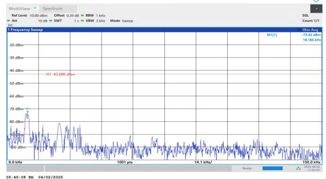
Band2-10MHz-QPSK-18650-1RB#49-0.009~0.15-PASS
