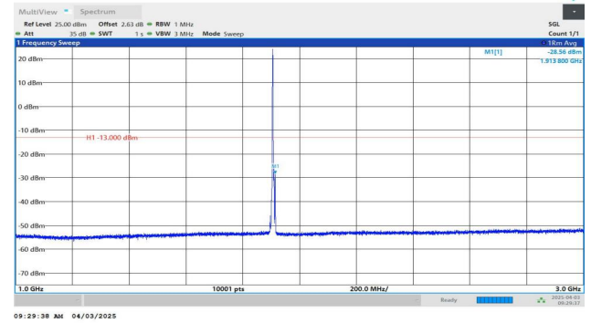
Band2-5MHz-QPSK-19175-1RB#0-1000~3000-PASS
