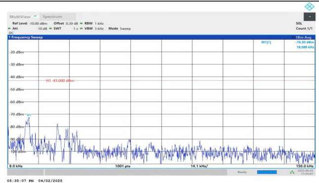
Band2-1.4MHz-QPSK-18900-1RB#5-0.009~0.15-PASS
