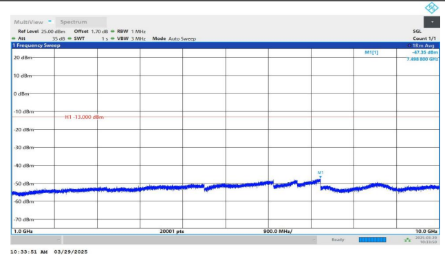
Band5-4233-2-1000~10000MHz-PASS
