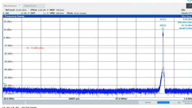
Band5-4233-4-30~1000MHz-PASS
