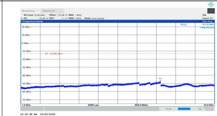
Band5-4132-3-1000~10000MHz-PASS
