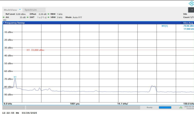
Band5-4233-4-0.009~0.15MHz-PASS
