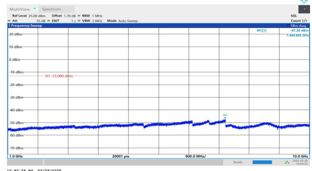
Band5-4233-4-1000~10000MHz-PASS
