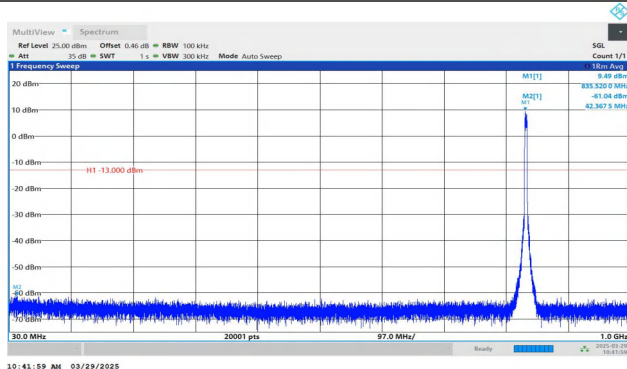
Band5-4182-5-30~1000MHz-PASS
