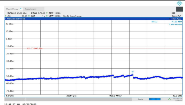
Band5-4182-5-1000~10000MHz-PASS
