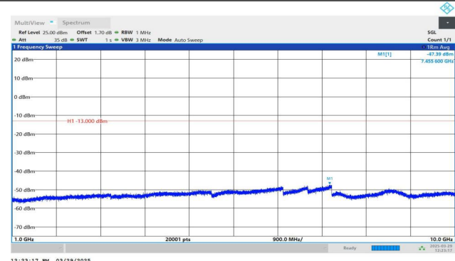
Band5-4233-4-1000~10000MHz-PASS
