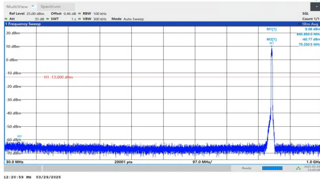
Band5-4233-3-30~1000MHz-PASS
