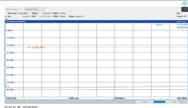
Band5-4233-4-0.15~30MHz-PASS
