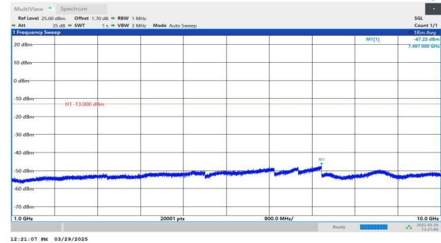
Band5-4233-3-1000~10000MHz-PASS
