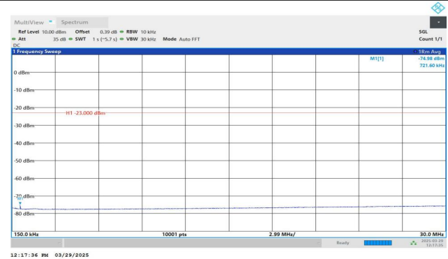
Band5-4132-2-0.15~30MHz-PASS
