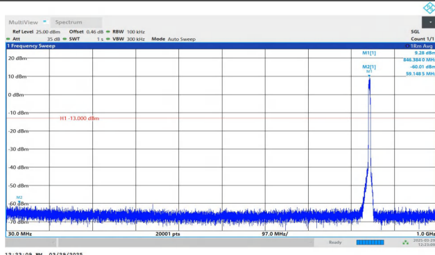
Band5-4233-4-30~1000MHz-PASS
