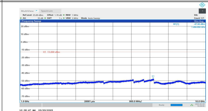
Band5-4132-4-1000~10000MHz-PASS
