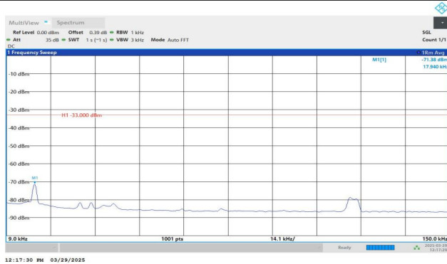
Band5-4132-2-0.009~0.15MHz-PASS
