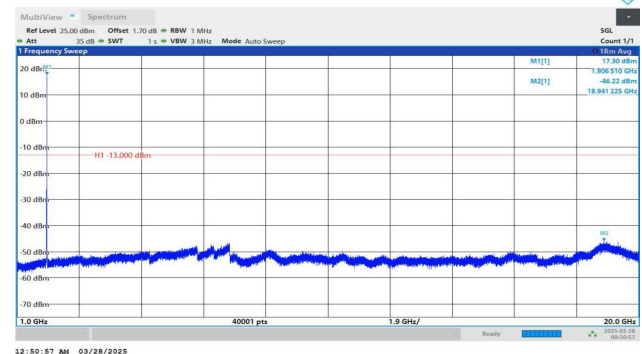
Band2-9538-2-1000~20000MHz-PASS
