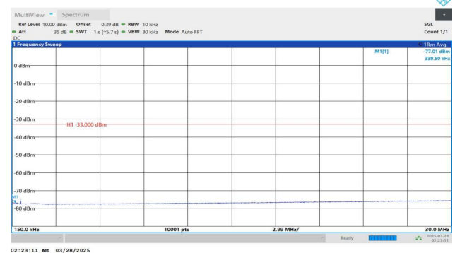
Band2-9538-4-0.15~30MHz-PASS
