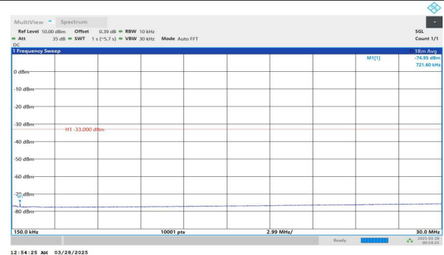
Band2-9400-4-0.15~30MHz-PASS
