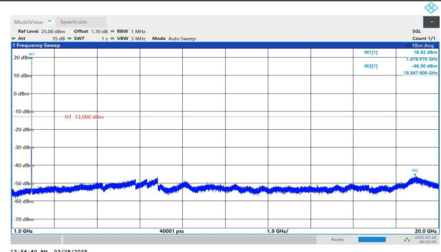
Band2-9400-4-1000~20000MHz-PASS
