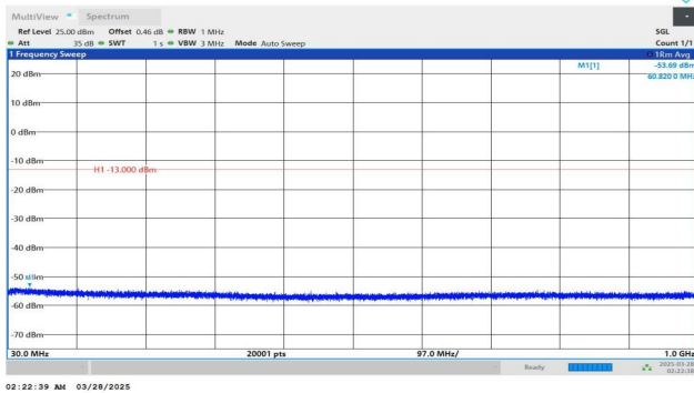
Band2-9400-4-30~1000MHz-PASS
