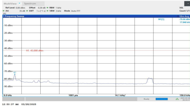
Band2-9538-2-0.009~0.15MHz-PASS
