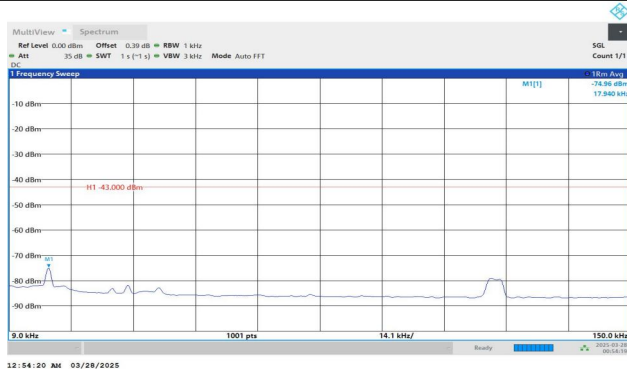
Band2-9400-4-0.009~0.15MHz-PASS
