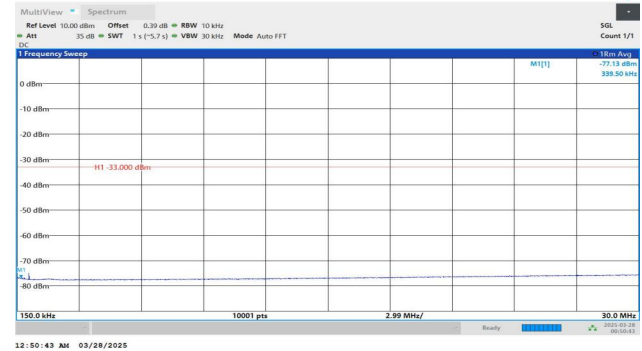
Band2-9538-2-0.15~30MHz-PASS
