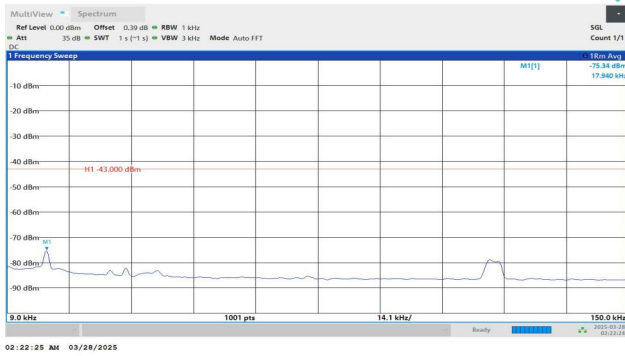
Band2-9400-4-0.009~0.15MHz-PASS
