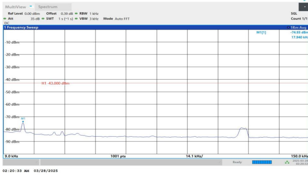
Band2-9538-3-0.009~0.15MHz-PASS
