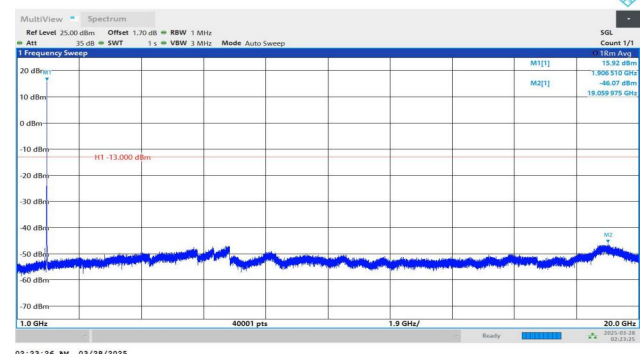
Band2-9538-4-1000~20000MHz-PASS
