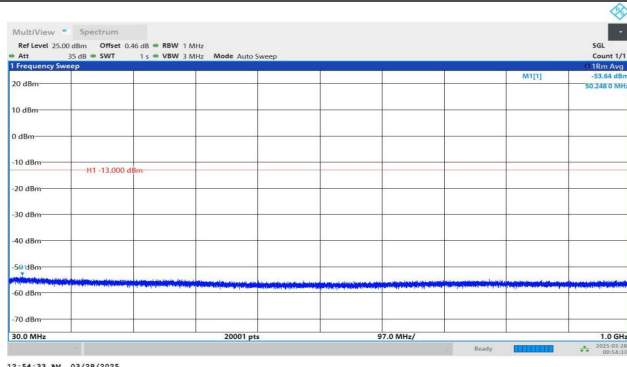
Band2-9400-4-30~1000MHz-PASS
