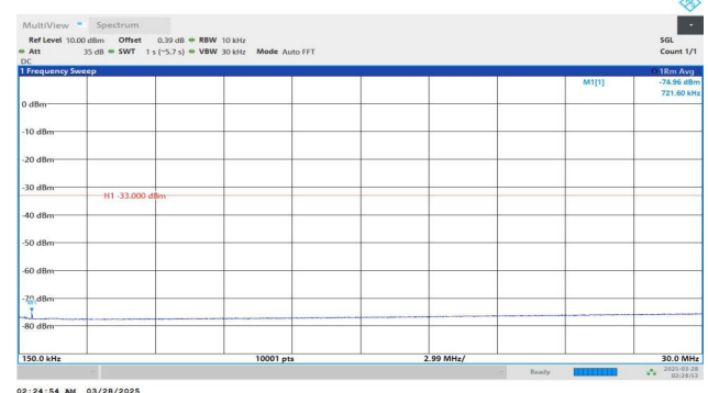
Band2-9400-5-0.15~30MHz-PASS
