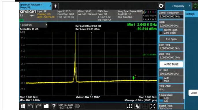
Band66-20MHz-QPSK-132322-1RB#99-1000~3000-PASS
