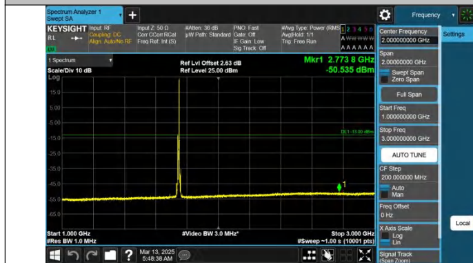
Band66-10MHz-QPSK-132322-1RB#49-1000~3000-PASS
