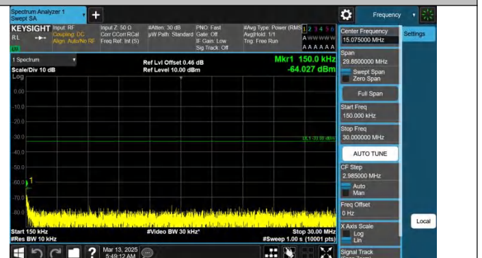
Band66-10MHz-QPSK-132622-1RB#0-0.15~30-PASS
