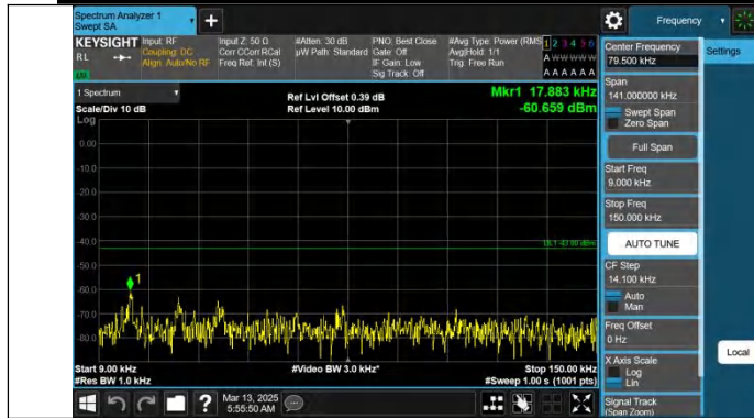
Band66-15MHz-QPSK-132047-1RB#0-0.009~0.15-PASS
