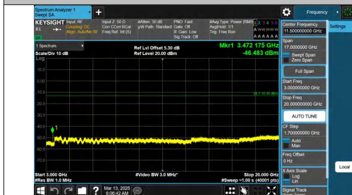
Band66-20MHz-QPSK-132322-1RB#0-3000~20000-PASS
