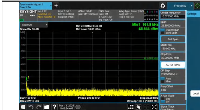
Band66-10MHz-QPSK-132322-1RB#49-0.15~30-PASS
