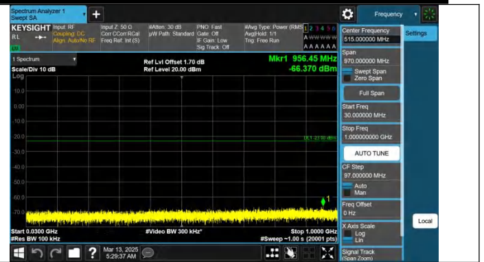
Band66-3MHz-QPSK-132657-1RB#14-30~1000-PASS
