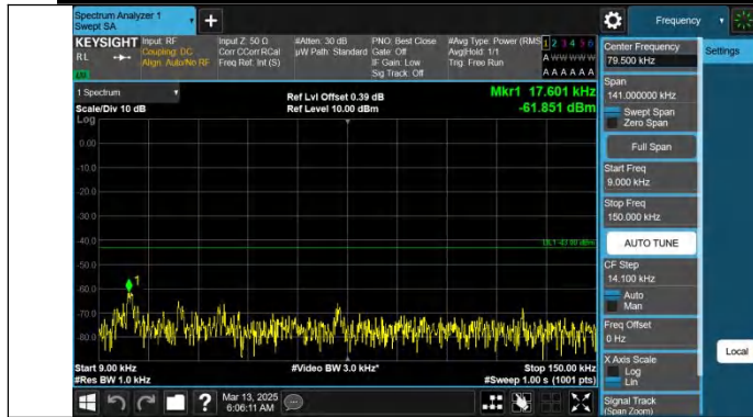
Band66-20MHz-QPSK-132322-1RB#0-0.009~0.15-PASS
