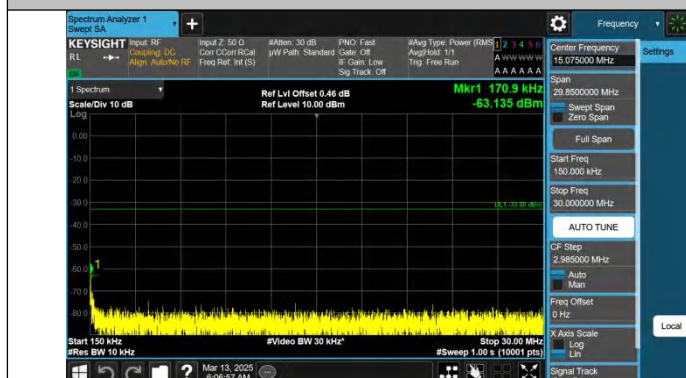
Band66-20MHz-QPSK-132322-1RB#99-0.15~30-PASS
