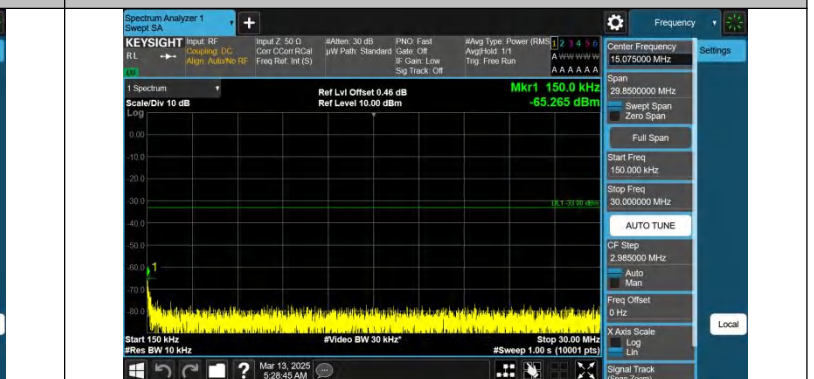
Band66-3MHz-QPSK-132657-1RB#0-0.15~30-PASS
