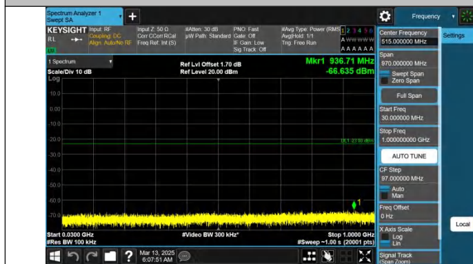
Band66-20MHz-QPSK-132572-1RB#0-30~1000-PASS
