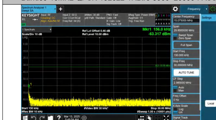
Band66-10MHz-QPSK-132622-1RB#49-0.15~30-PASS
