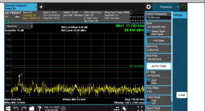
Band66-20MHz-QPSK-132322-1RB#99-0.009~0.15-PASS
