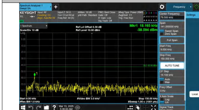
Band66-5MHz-QPSK-131997-1RB#0-0.009~0.15-PASS
