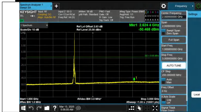
Band66-15MHz-QPSK-132047-1RB#74-1000~3000-PASS
