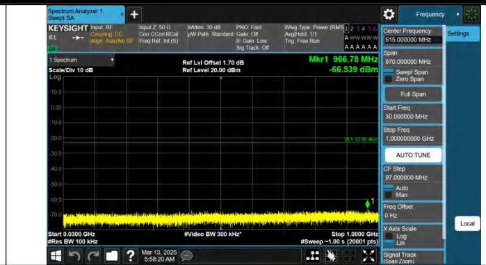
Band66-15MHz-QPSK-132322-1RB#74-30~1000-PASS
