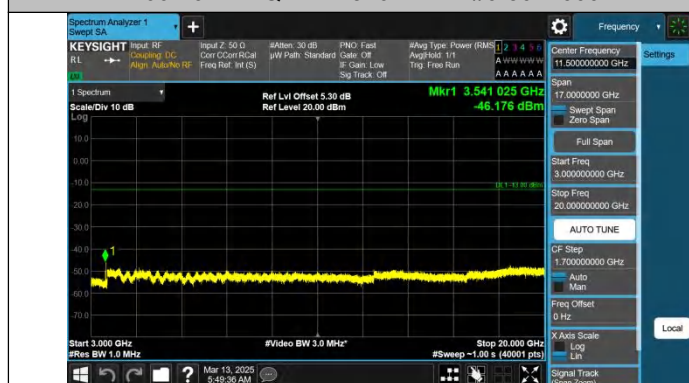
Band66-10MHz-QPSK-132622-1RB#0-3000~20000-PASS
