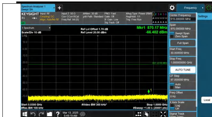
Band66-10MHz-QPSK-132622-1RB#0-30~1000-PASS
