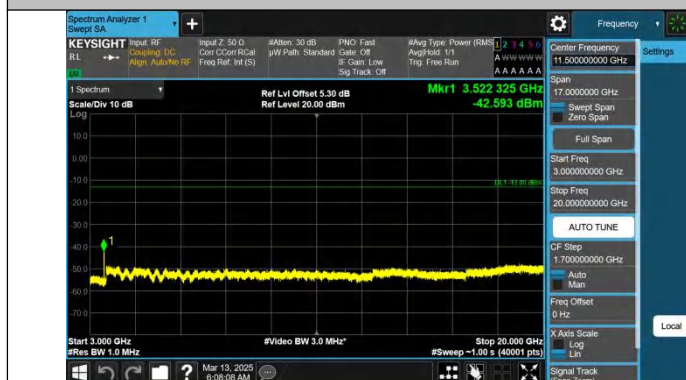
Band66-20MHz-QPSK-132572-1RB#0-3000~20000-PASS
