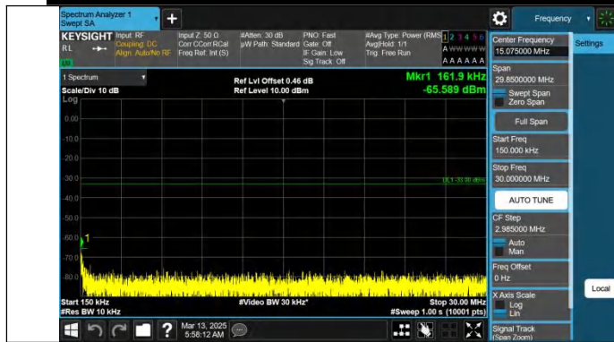
Band66-15MHz-QPSK-132322-1RB#74-0.15~30-PASS
