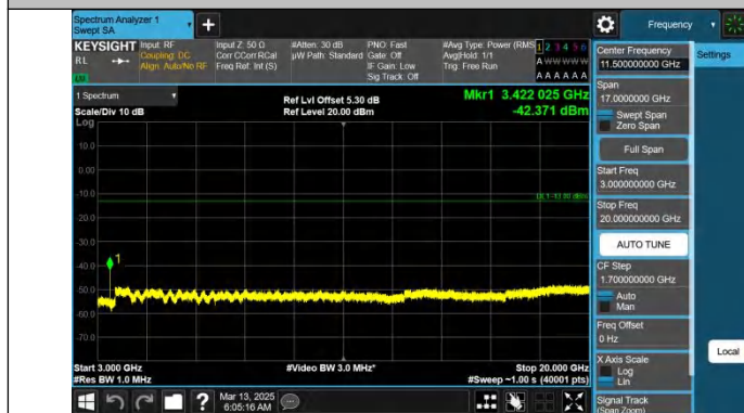
Band66-20MHz-QPSK-132072-1RB#0-3000~20000-PASS
