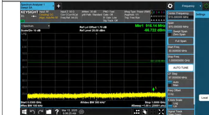
Band66-20MHz-QPSK-132322-1RB#0-30~1000-PASS
