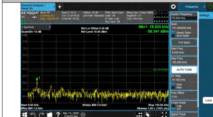
Band66-10MHz-QPSK-132622-1RB#0-0.009~0.15-PASS
