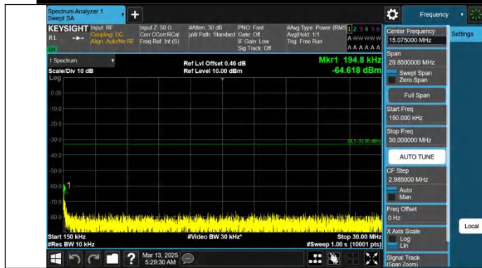
Band66-3MHz-QPSK-132657-1RB#14-0.15~30-PASS
