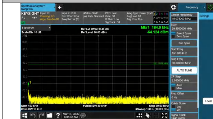
Band66-20MHz-QPSK-132072-1RB#99-0.15~30-PASS
