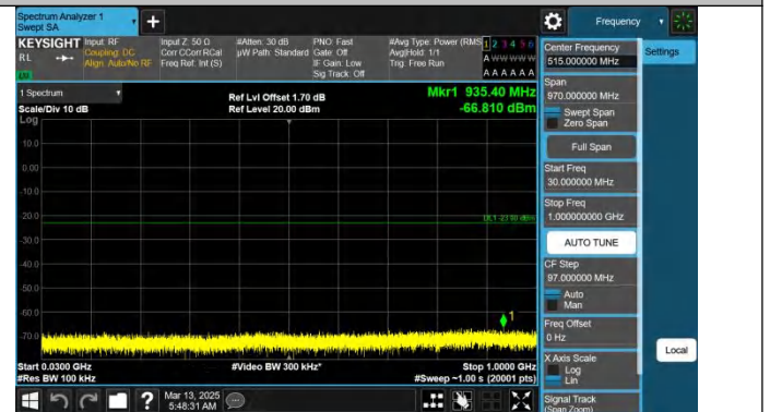
Band66-10MHz-QPSK-132322-1RB#49-30~1000-PASS
