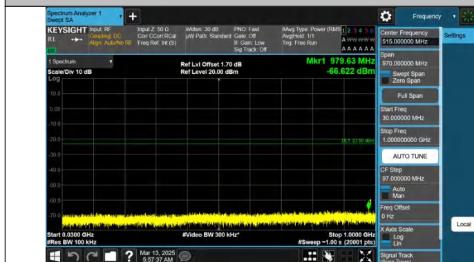
Band66-15MHz-QPSK-132322-1RB#0-30~1000-PASS
