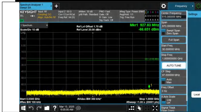
Band66-20MHz-QPSK-132072-1RB#0-30~1000-PASS
