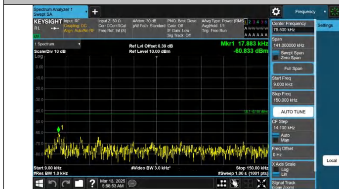
Band66-15MHz-QPSK-132597-1RB#0-0.009~0.15-PASS
