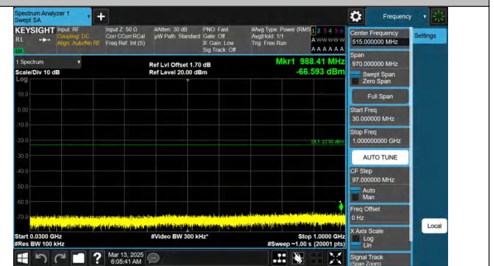
Band66-20MHz-QPSK-132072-1RB#99-30~1000-PASS
