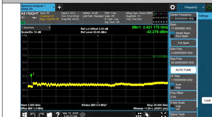
Band66-10MHz-QPSK-132022-1RB#0-3000~20000-PASS
