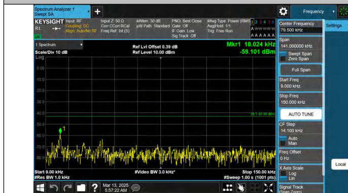
Band66-15MHz-QPSK-132322-1RB#0-0.009~0.15-PASS
