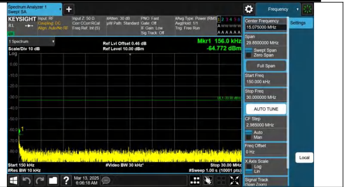
Band66-20MHz-QPSK-132322-1RB#0-0.15~30-PASS
