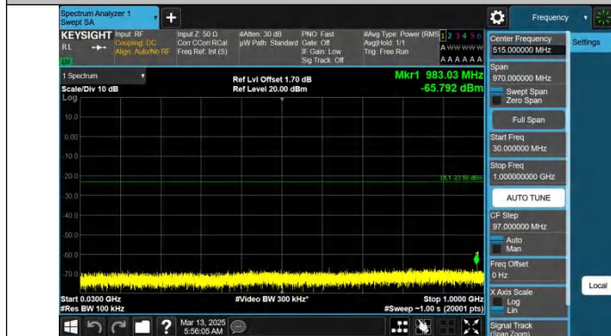
Band66-15MHz-QPSK-132047-1RB#0-30~1000-PASS
