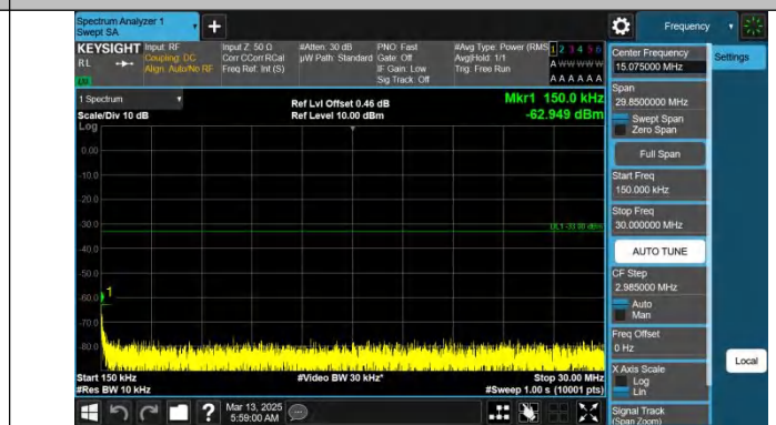
Band66-15MHz-QPSK-132597-1RB#0-0.15~30-PASS
