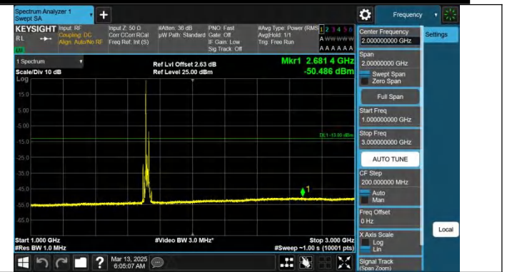
Band66-20MHz-QPSK-132072-1RB#0-1000~3000-PASS
