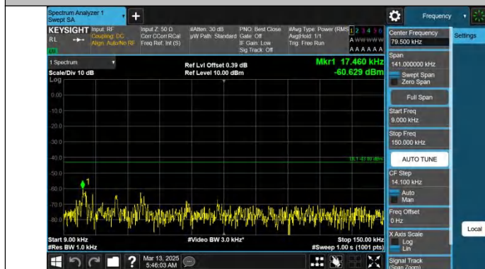
Band66-10MHz-QPSK-132022-1RB#0-0.009~0.15-PASS
