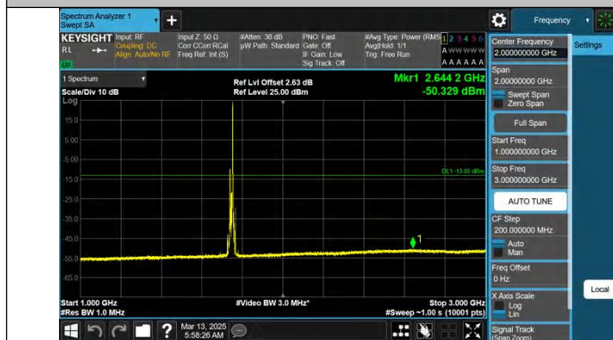
Band66-15MHz-QPSK-132322-1RB#74-1000~3000-PASS
