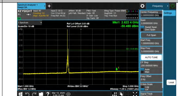
Band66-15MHz-QPSK-132597-1RB#0-1000~3000-PASS
