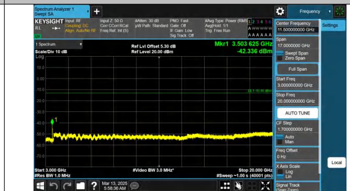
Band66-15MHz-QPSK-132322-1RB#74-3000~20000-PASS
