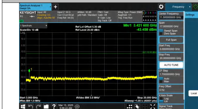
Band66-15MHz-QPSK-132047-1RB#0-3000~20000-PASS
