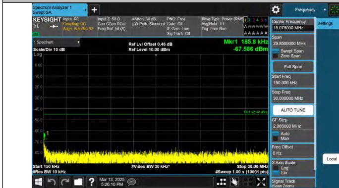
Band41-15MHz-QPSK-39725-1RB#74-0.15~30-PASS
