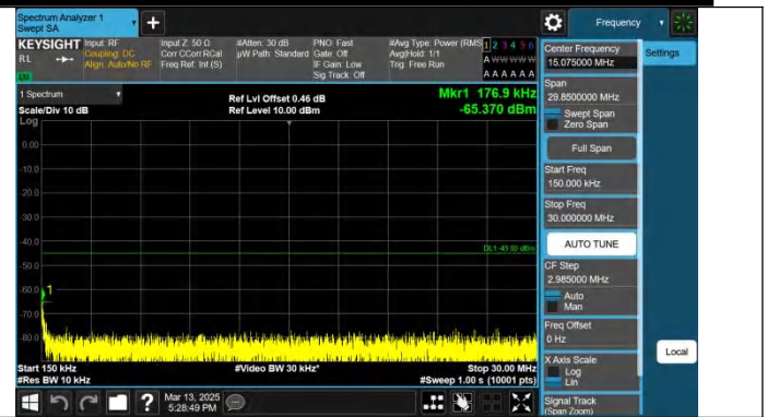
Band41-15MHz-QPSK-41515-1RB#0-0.15~30-PASS
