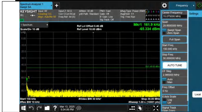
Band41-20MHz-QPSK-39750-1RB#99-0.15~30-PASS
