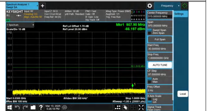
Band41-15MHz-QPSK-39725-1RB#74-30~1000-PASS
