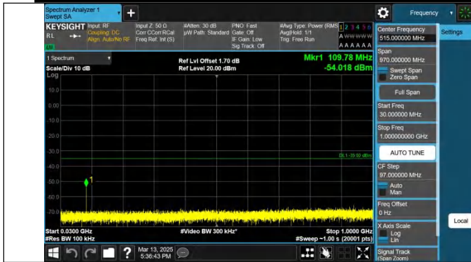
Band41-20MHz-QPSK-41490-1RB#0-30~1000-PASS
