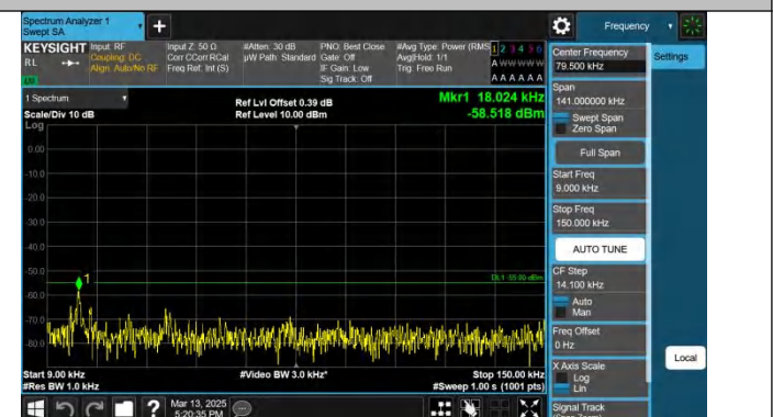
Band41-10MHz-QPSK-41540-1RB#49-0.009~0.15-PASS
