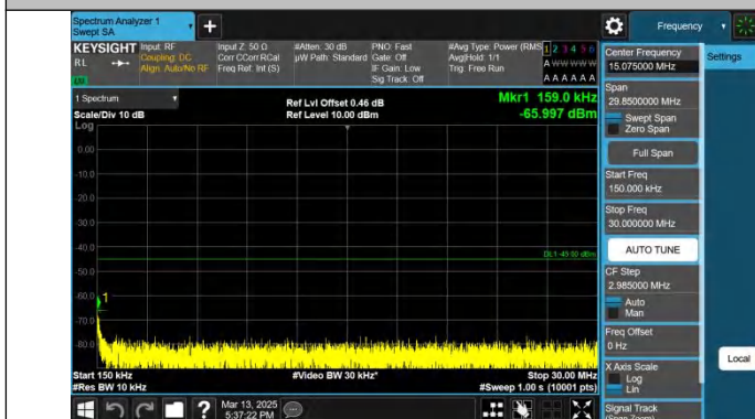
Band41-20MHz-QPSK-41490-1RB#99-0.15~30-PASS
