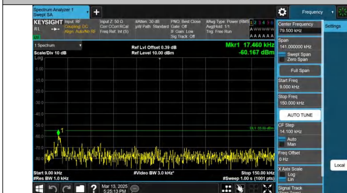
Band41-15MHz-QPSK-39725-1RB#0-0.009~0.15-PASS
