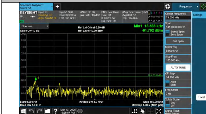
Band41-15MHz-QPSK-40620-1RB#0-0.009~0.15-PASS
