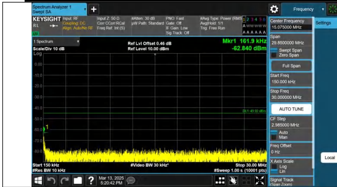
Band41-10MHz-QPSK-41540-1RB#49-0.15~30-PASS
