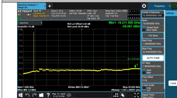
Band41-5MHz-QPSK-41565-1RB#24-1000~20000-PASS
