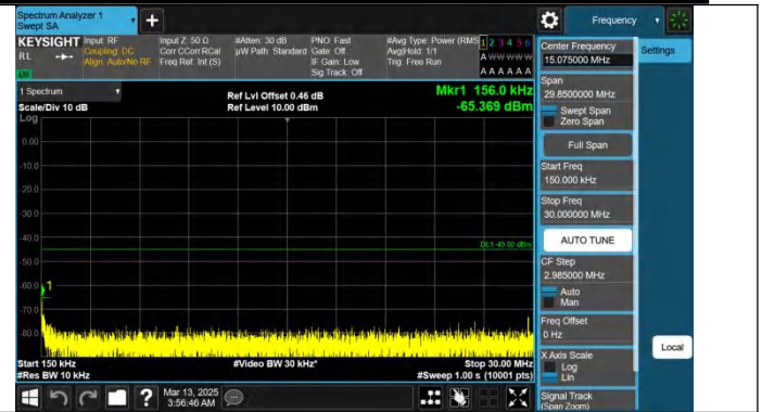
Band38-15MHz-QPSK-38175-1RB#0-0.15~30-PASS
