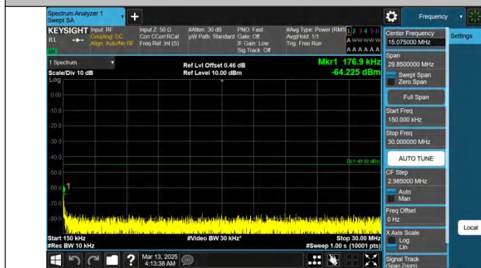
Band38-20MHz-QPSK-38150-1RB#99-0.15~30-PASS
