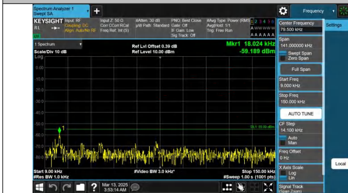
Band38-15MHz-QPSK-37825-1RB#0-0.009~0.15-PASS
