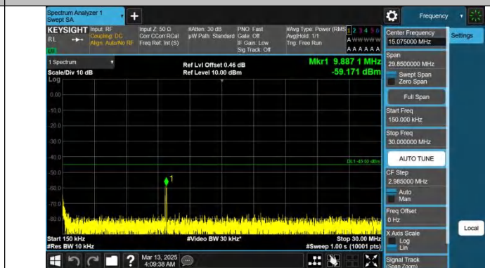
Band38-20MHz-QPSK-37850-1RB#0-0.15~30-PASS
