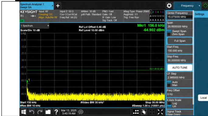
Band38-10MHz-QPSK-38200-1RB#49-0.15~30-PASS
