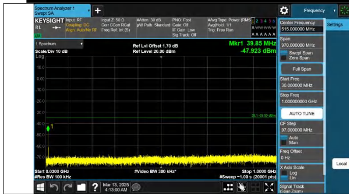
Band38-20MHz-QPSK-38150-1RB#0-30~1000-PASS
