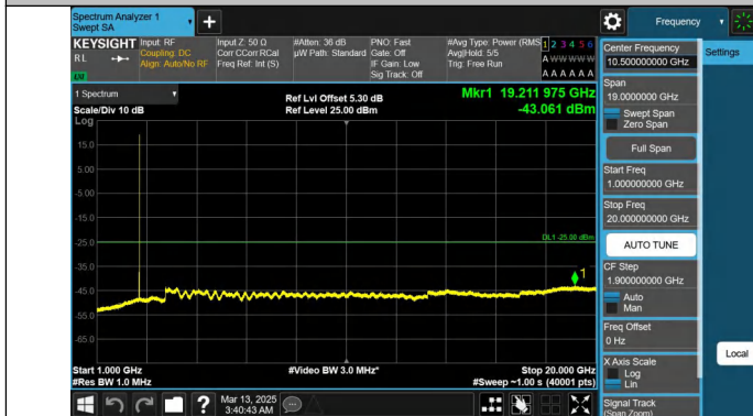
Band38-10MHz-QPSK-38200-1RB#49-1000~20000-PASS
