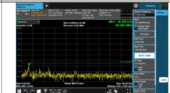
Band38-20MHz-QPSK-37850-1RB#99-0.009~0.15-PASS
