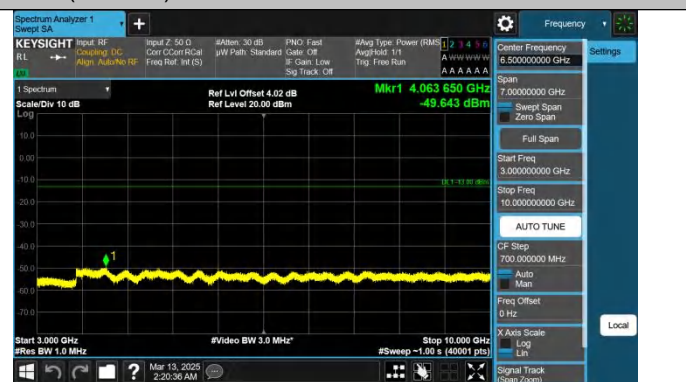
Band26(824-849)-1.4MHz-QPSK-27033-1RB#5-3000~10000-PAS
