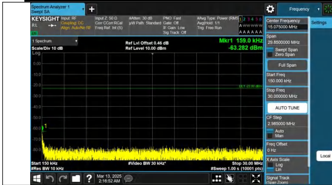
Band26(824-849)-1.4MHz-QPSK-26797-1RB#5-0.15~30-PASS
