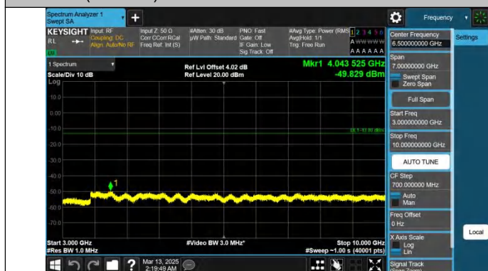
Band26(824-849)-1.4MHz-QPSK-27033-1RB#0-3000~10000-PAS
