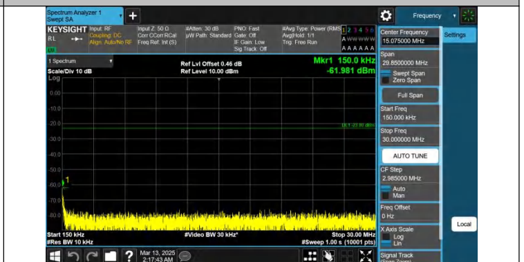
Band26(824-849)-1.4MHz-QPSK-26915-1RB#0-0.15~30-PASS
