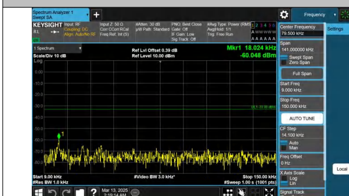
Band26(824-849)-1.4MHz-QPSK-27033-1RB#0-0.009~0.15-PASS
