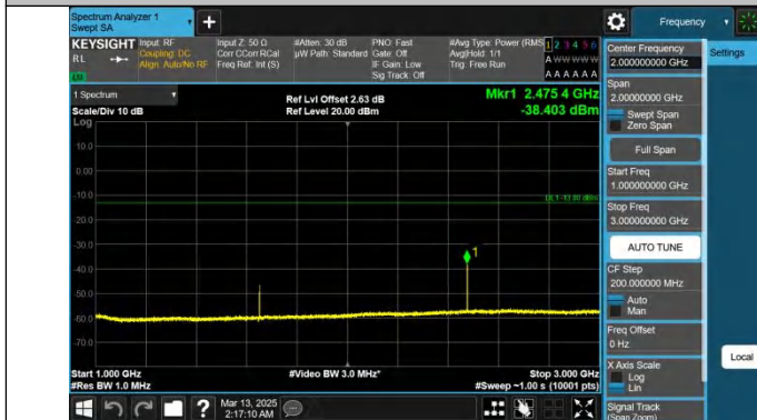
Band26(824-849)-1.4MHz-QPSK-26797-1RB#5-1000~3000-PASS
