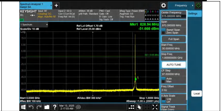
Band26(824-849)-1.4MHz-QPSK-26797-1RB#5-30~1000-PASS
