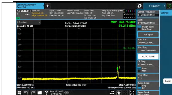
Band26(824-849)-1.4MHz-QPSK-27033-1RB#0-30~1000-PASS
