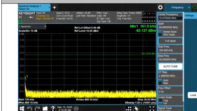
Band26(824-849)-1.4MHz-QPSK-26915-1RB#5-0.15~30-PASS
