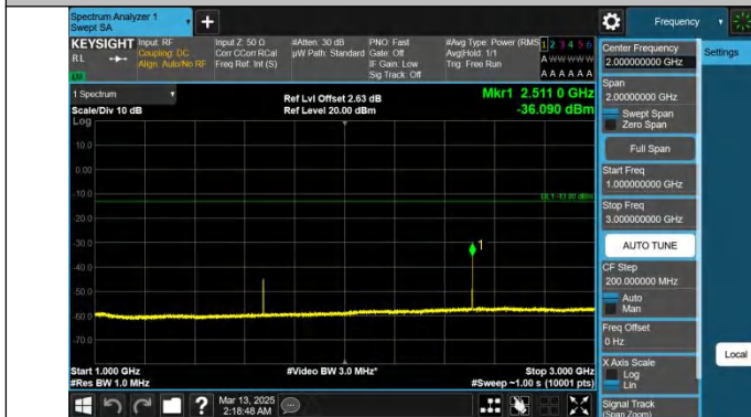
Band26(824-849)-1.4MHz-QPSK-26915-1RB#5-1000~3000-PASS
