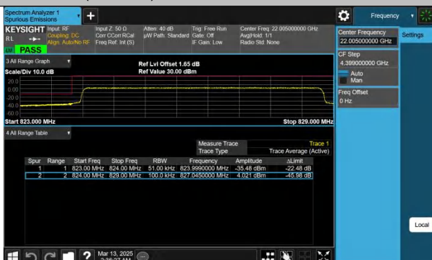
Band26(824-849)-5MHz-QPSK-26815-25RB#0-PASS
