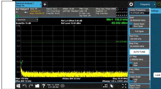
Band26(824-849)-5MHz-QPSK-27015-1RB#24-0.15~30-PASS
