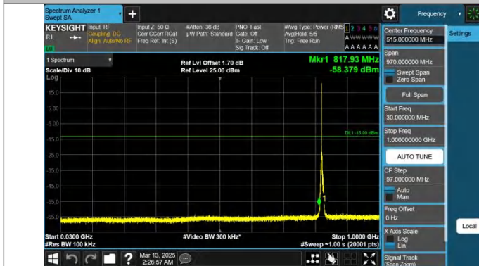
Band26(824-849)-3MHz-QPSK-26805-1RB#0-30~1000-PASS
