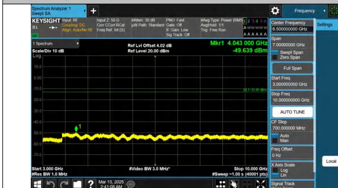
Band26(824-849)-5MHz-QPSK-27015-1RB#0-3000~10000-PASS
