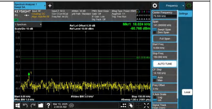
Band26(824-849)-5MHz-QPSK-26815-1RB#24-0.009~0.15-PASS
