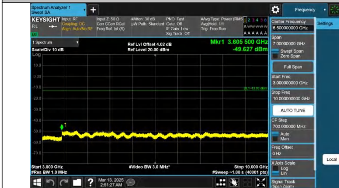
Band26(824-849)-10MHz-QPSK-26990-1RB#0-3000~10000-PASS
