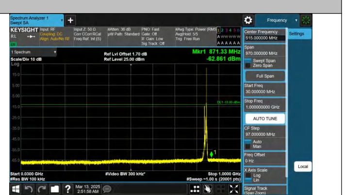
Band26(824-849)-10MHz-QPSK-26990-1RB#49-30~1000-PASS
