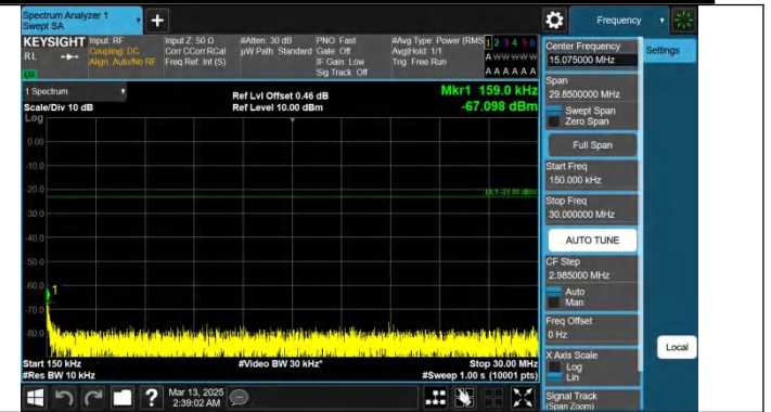
Band26(824-849)-5MHz-QPSK-26915-1RB#0-0.15~30-PASS
