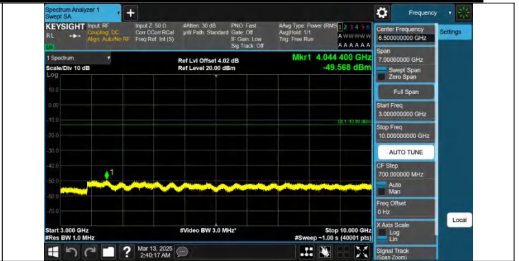
Band26(824-849)-5MHz-QPSK-26915-1RB#24-3000~10000-PASS
