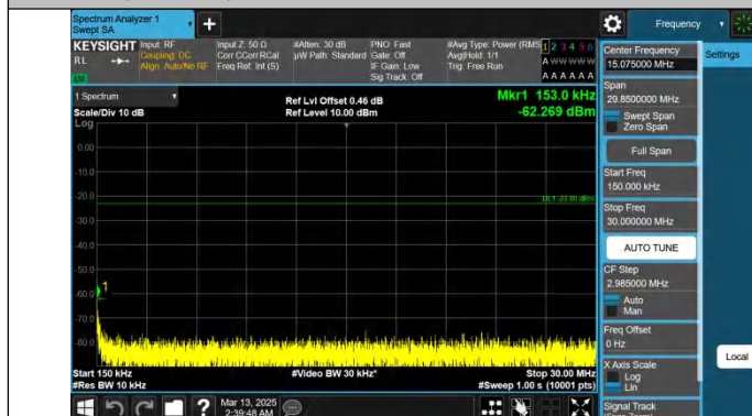
Band26(824-849)-5MHz-QPSK-26915-1RB#24-0.15~30-PASS
