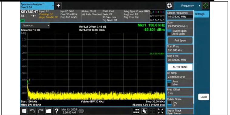
Band26(824-849)-3MHz-QPSK-26805-1RB#0-0.15~30-PASS
