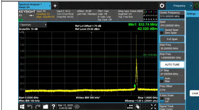
Band26(824-849)-5MHz-QPSK-27015-1RB#0-30~1000-PASS
