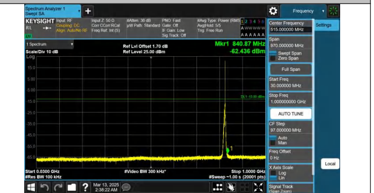
Band26(824-849)-5MHz-QPSK-26815-1RB#24-30~1000-PASS
