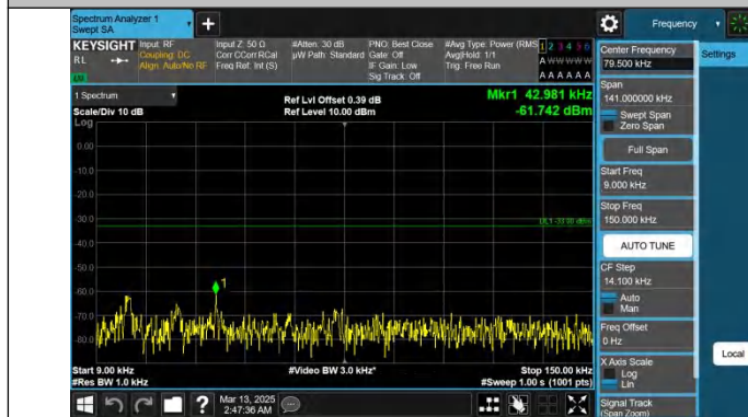
Band26(824-849)-10MHz-QPSK-26840-1RB#0-0.009~0.15-PASS
