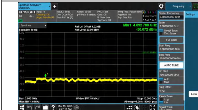
Band26(824-849)-3MHz-QPSK-26805-1RB#0-3000~10000-PASS
