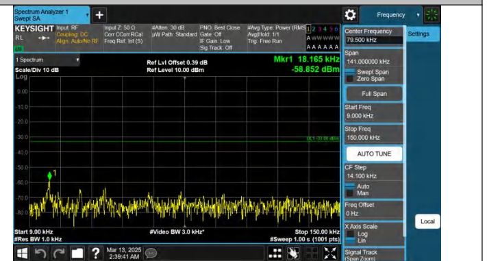
Band26(824-849)-5MHz-QPSK-26915-1RB#24-0.009~0.15-PASS
