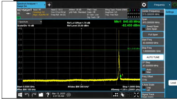
Band26(824-849)-5MHz-QPSK-26815-1RB#0-30~1000-PASS
