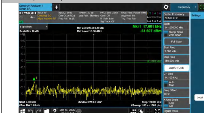
Band26(824-849)-5MHz-QPSK-26815-1RB#0-0.009~0.15-PASS
