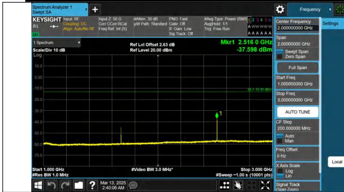
Band26(824-849)-5MHz-QPSK-26915-1RB#24-1000~3000-PASS
