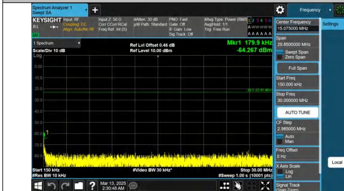
Band26(824-849)-3MHz-QPSK-27025-1RB#14-0.15~30-PASS
