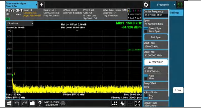
Band26(824-849)-10MHz-QPSK-26990-1RB#0-0.15~30-PASS
