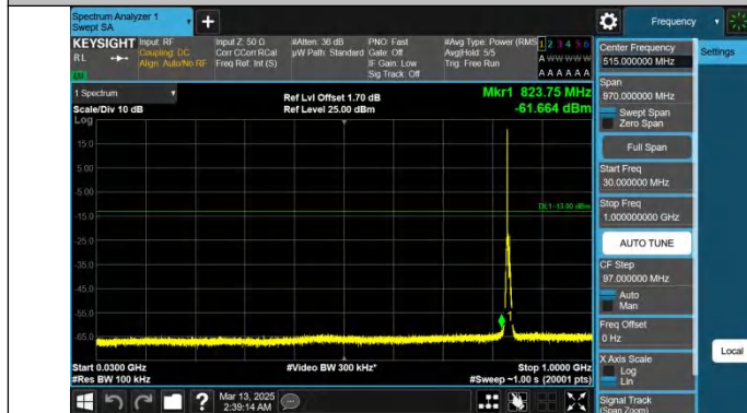
Band26(824-849)-5MHz-QPSK-26915-1RB#0-30~1000-PASS
