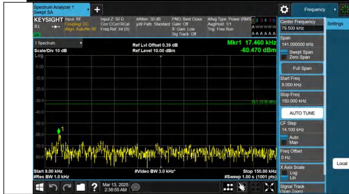
Band26(824-849)-5MHz-QPSK-26915-1RB#0-0.009~0.15-PASS
