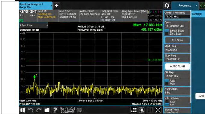
Band26(824-849)-3MHz-QPSK-26805-1RB#0-0.009~0.15-PASS
