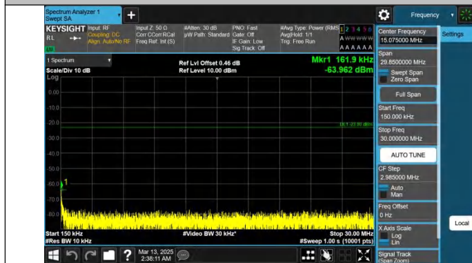
Band26(824-849)-5MHz-QPSK-26815-1RB#24-0.15~30-PASS
