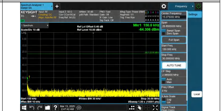
Band26(824-849)-10MHz-QPSK-26840-1RB#0-0.15~30-PASS
