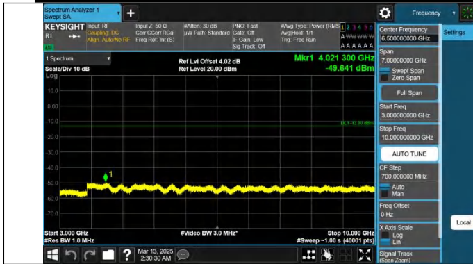
Band26(824-849)-3MHz-QPSK-27025-1RB#0-3000~10000-PASS
