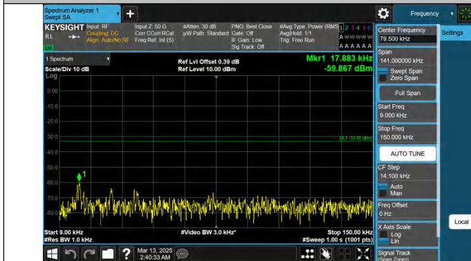
Band26(824-849)-5MHz-QPSK-27015-1RB#0-0.009~0.15-PASS
