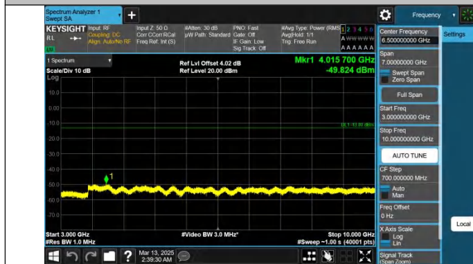
Band26(824-849)-5MHz-QPSK-26915-1RB#0-3000~10000-PASS
