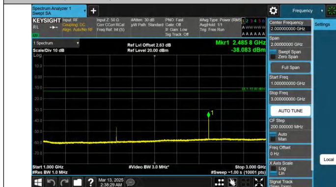
Band26(824-849)-5MHz-QPSK-26815-1RB#24-1000~3000-PASS
