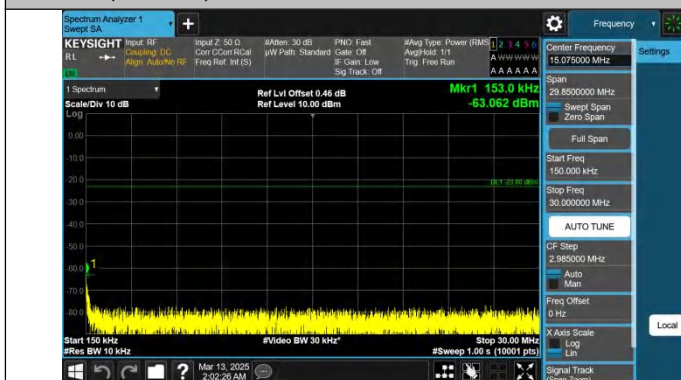
Band26(814-824)-5MHz-QPSK-26715-1RB#24-0.15~30-PASS
