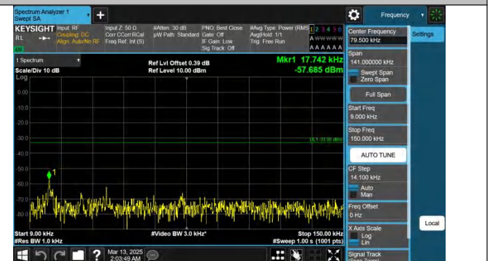
Band26(814-824)-5MHz-QPSK-26740-1RB#24-0.009~0.15-PASS
