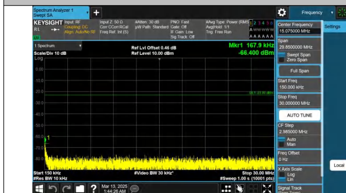
Band26(814-824)-1.4MHz-QPSK-26783-1RB#5-0.15~30-PASS
