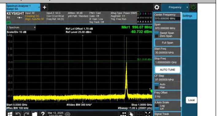
Band26(814-824)-5MHz-QPSK-26740-1RB#24-30~1000-PASS
