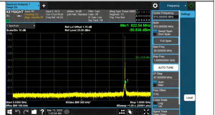
Band26(814-824)-1.4MHz-QPSK-26740-1RB#5-30~1000-PASS
