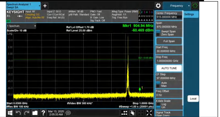
Band26(814-824)-5MHz-QPSK-26765-1RB#24-30~1000-PASS
