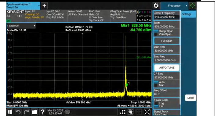
Band26(814-824)-3MHz-QPSK-26740-1RB#14-30~1000-PASS
