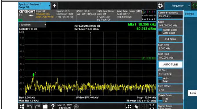
Band26(814-824)-1.4MHz-QPSK-26740-1RB#0-0.009~0.15-PASS
