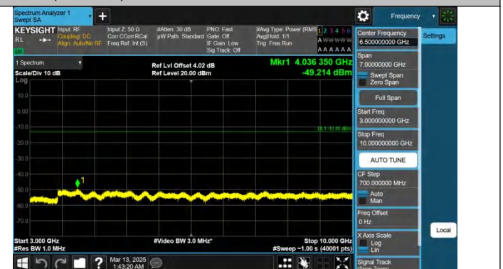
Band26(814-824)-1.4MHz-QPSK-26740-1RB#5-3000~10000-PASS S
