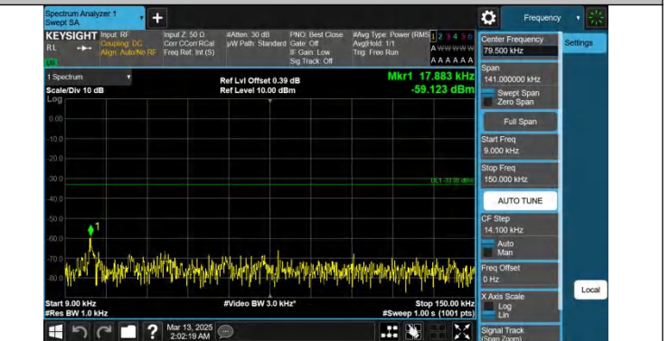
Band26(814-824)-5MHz-QPSK-26715-1RB#24-0.009~0.15-PASS
