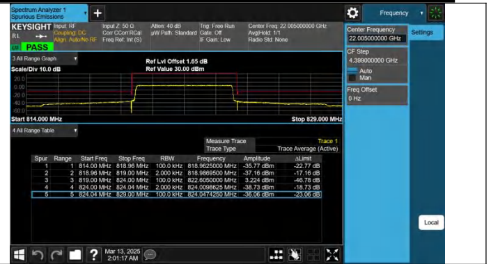
Band26(814-824)-5MHz-QPSK-26765-25RB#0-PASS
