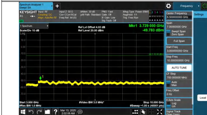
Band26(814-824)-5MHz-QPSK-26715-1RB#0-3000~10000-PASS
