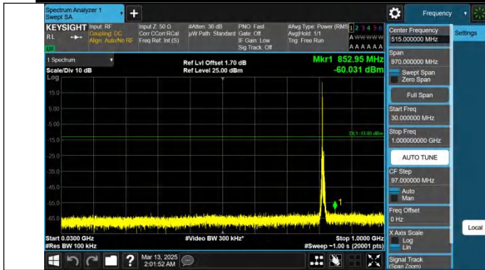
Band26(814-824)-5MHz-QPSK-26715-1RB#0-30~1000-PASS
