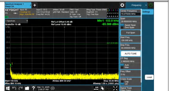
Band26(814-824)-10MHz-QPSK-26740-1RB#0-0.15~30-PASS
