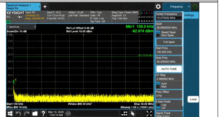
Band26(814-824)-3MHz-QPSK-26775-1RB#0-0.15~30-PASS
