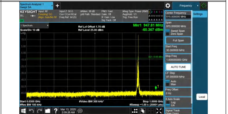
Band26(814-824)-10MHz-QPSK-26740-1RB#49-30~1000-PASS
