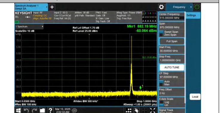
Band26(814-824)-5MHz-QPSK-26715-1RB#24-30~1000-PASS
