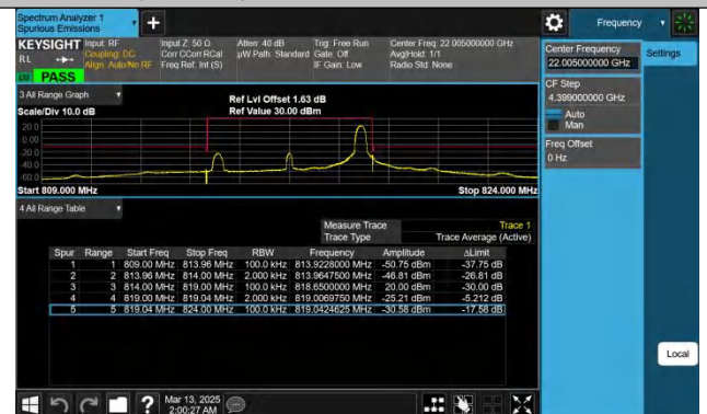
Band26(814-824)-5MHz-QPSK-26715-1RB#24-PASS
