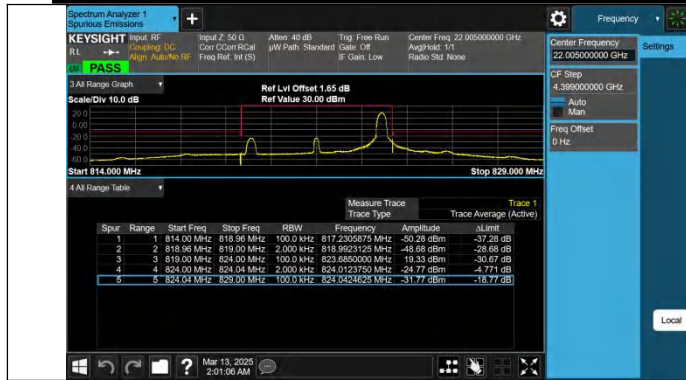
Band26(814-824)-5MHz-QPSK-26765-1RB#24-PASS
