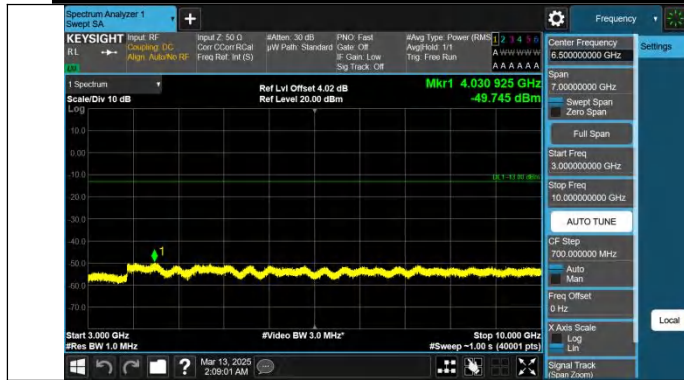
Band26(814-824)-10MHz-QPSK-26740-1RB#0-3000~10000-PAS
