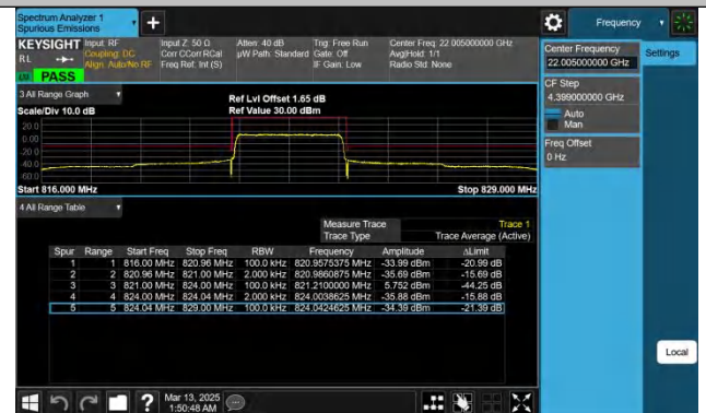
Band26(814-824)-3MHz-QPSK-26775-15RB#0-PASS
