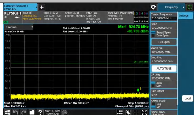
Band25-20MHz-QPSK-26140-1RB#99-30~1000-PASS
