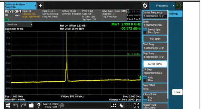
Band25-15MHz-QPSK-26115-1RB#0-1000~3000-PASS
