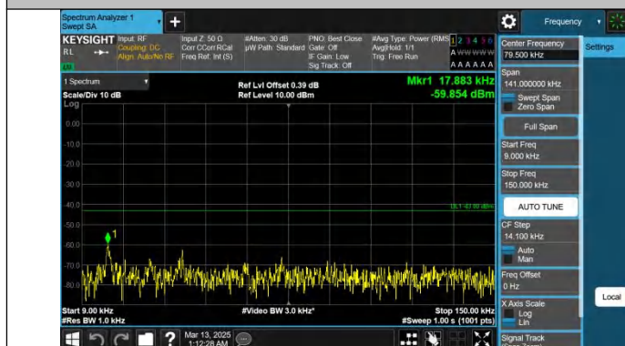
Band25-10MHz-QPSK-26640-1RB#0-0.009~0.15-PASS
