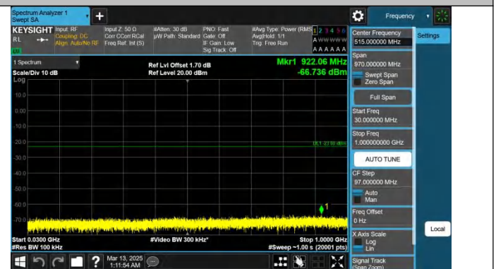
Band25-10MHz-QPSK-26365-1RB#49-30~1000-PASS
