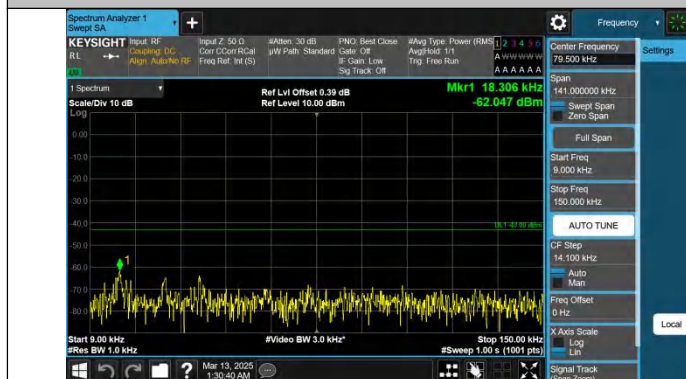
Band25-20MHz-QPSK-26590-1RB#0-0.009~0.15-PASS
