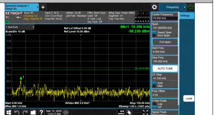
Band25-5MHz-QPSK-26665-1RB#24-0.009~0.15-PASS
