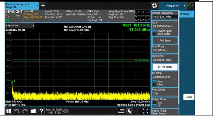
Band25-15MHz-QPSK-26115-1RB#0-0.15~30-PASS
