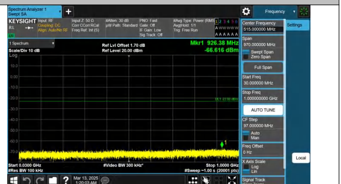
Band25-15MHz-QPSK-26115-1RB#74-30~1000-PASS
