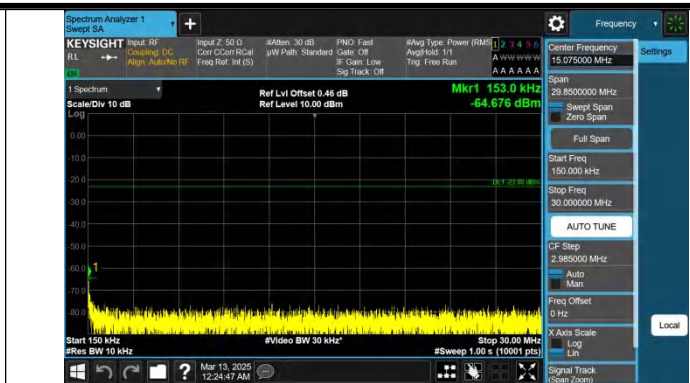
Band13-5MHz-QPSK-23255-1RB#0-0.15~30-PASS
