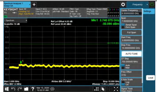
Band13-5MHz-QPSK-23205-1RB#24-3000~10000-PASS
