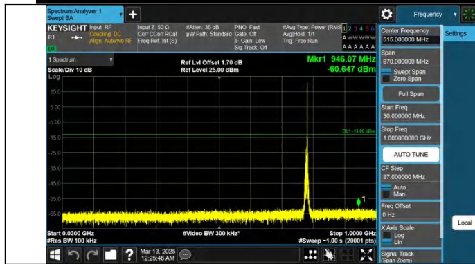
Band13-5MHz-QPSK-23255-1RB#24-30~1000-PASS
