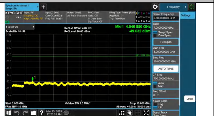
Band13-5MHz-QPSK-23255-1RB#24-3000~10000-PASS
