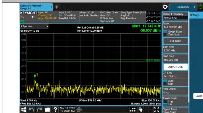
Band13-10MHz-QPSK-23230-1RB#0-0.009~0.15-PASS
