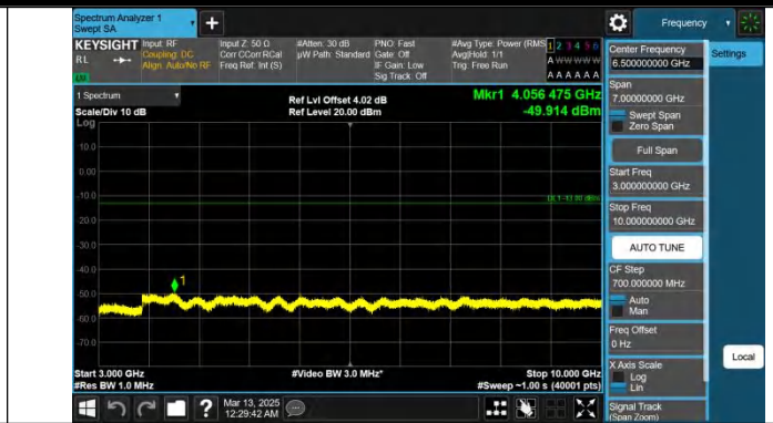
Band13-10MHz-QPSK-23230-1RB#0-3000~10000-PASS
