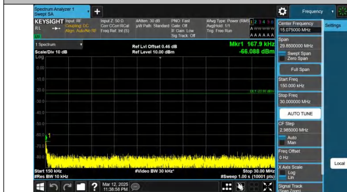
Band12-1.4MHz-QPSK-23173-1RB#5-0.15~30-PASS
