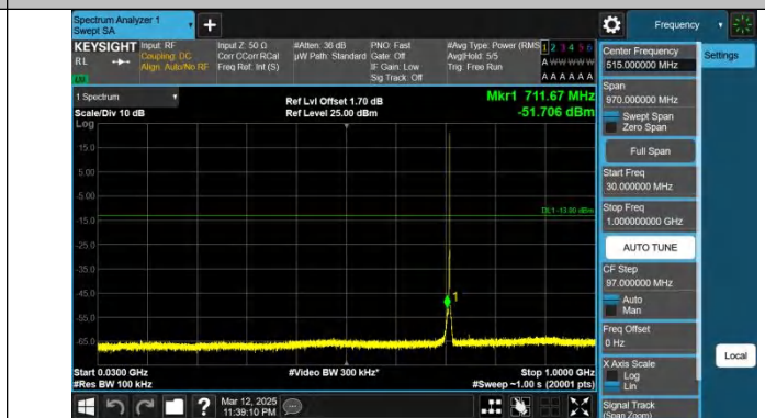
Band12-1.4MHz-QPSK-23173-1RB#5-30~1000-PASS
