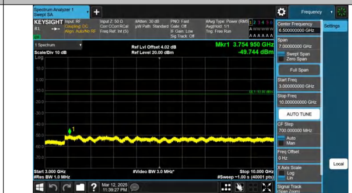
Band12-1.4MHz-QPSK-23173-1RB#5-3000~10000-PASS
