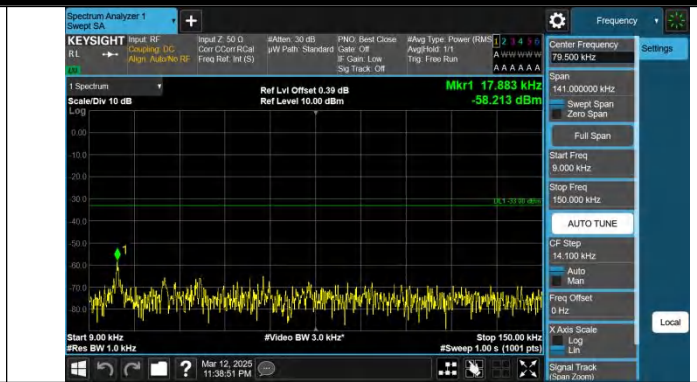
Band12-1.4MHz-QPSK-23173-1RB#5-0.009~0.15-PASS
