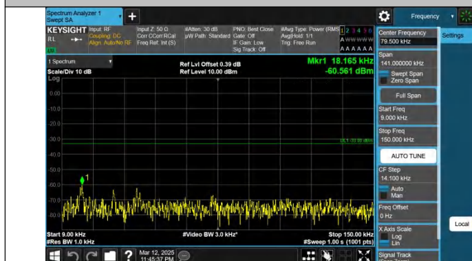
Band12-3MHz-QPSK-23025-1RB#0-0.009~0.15-PASS
