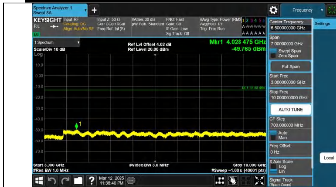
Band12-1.4MHz-QPSK-23173-1RB#0-3000~10000-PASS
