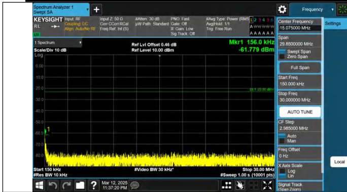
Band12-1.4MHz-QPSK-23095-1RB#5-0.15~30-PASS
