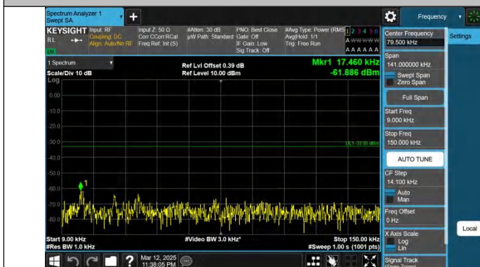
Band12-1.4MHz-QPSK-23173-1RB#0-0.009~0.15-PASS
