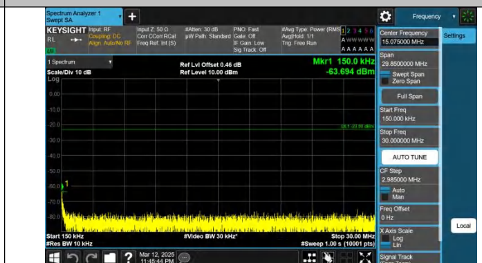
Band12-3MHz-QPSK-23025-1RB#0-0.15~30-PASS
