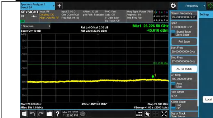
Band7-20MHz-QPSK-21100-1RB#0-20000~27000-PASS
