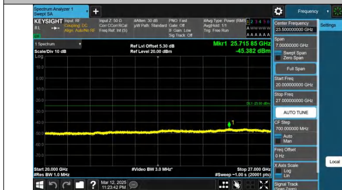
Band7-20MHz-QPSK-21350-1RB#0-20000~27000-PASS
