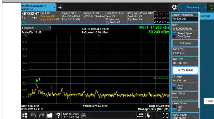
Band7-15MHz-QPSK-20825-1RB#0-0.009~0.15-PASS
