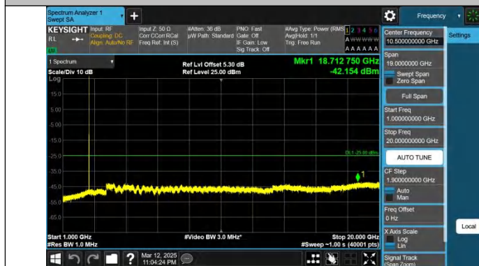
Band7-10MHz-QPSK-21400-1RB#49-1000~20000-PASS
