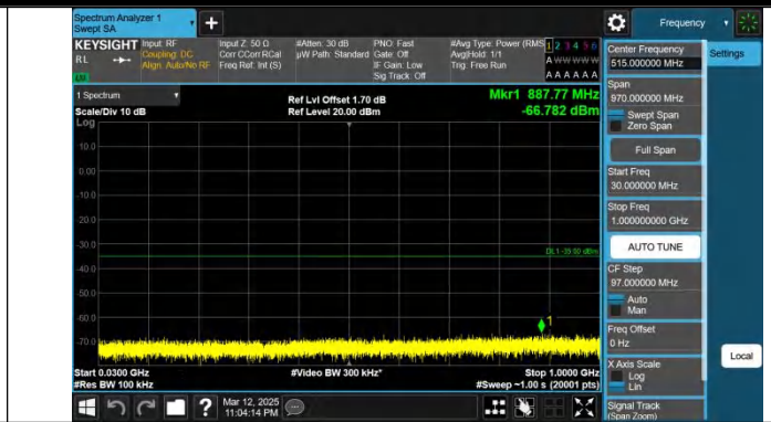
Band7-10MHz-QPSK-21400-1RB#49-30~1000-PASS
