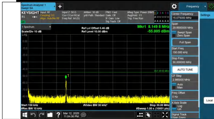
Band7-10MHz-QPSK-21400-1RB#49-0.15~30-PASS
