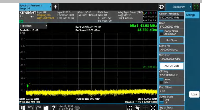
Band7-10MHz-QPSK-21100-1RB#49-30~1000-PASS
