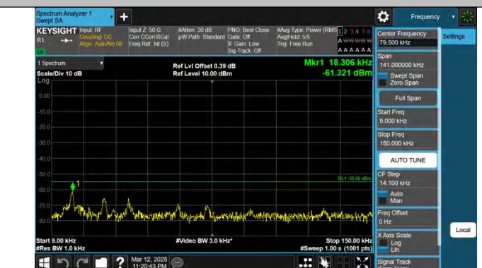
Band7-20MHz-QPSK-20850-1RB#99-0.009~0.15-PASS
