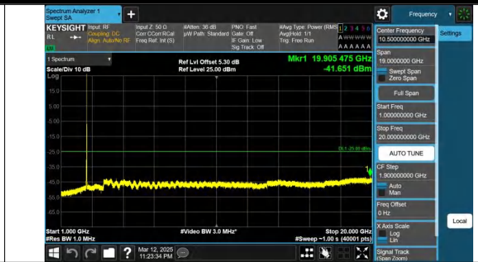
Band7-20MHz-QPSK-21350-1RB#0-1000~20000-PASS
