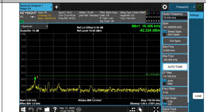
Band7-10MHz-QPSK-21100-1RB#49-0.009~0.15-PASS
