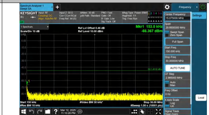
Band7-15MHz-QPSK-20825-1RB#0-0.15~30-PASS
