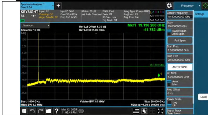
Band7-10MHz-QPSK-21100-1RB#49-1000~20000-PASS
