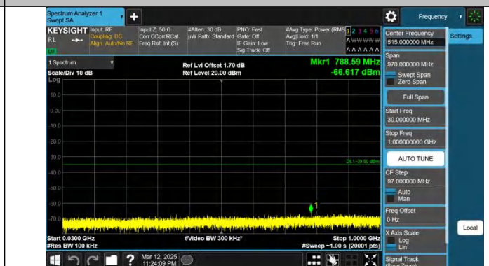
Band7-20MHz-QPSK-21350-1RB#99-30~1000-PASS
