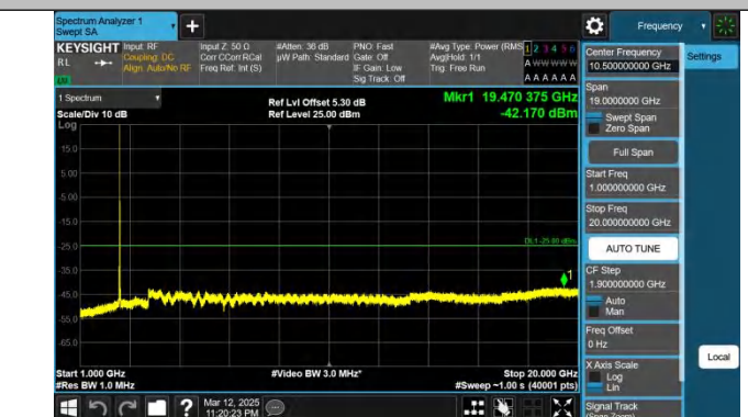
Band7-20MHz-QPSK-20850-1RB#0-1000~20000-PASS
