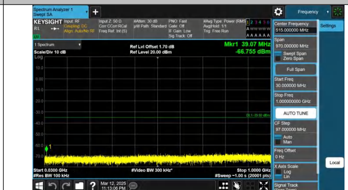
Band7-15MHz-QPSK-21100-1RB#74-30~1000-PASS
