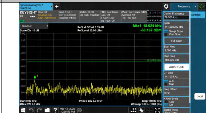
Band5-10MHz-QPSK-20450-1RB#49-0.009~0.15-PASS
