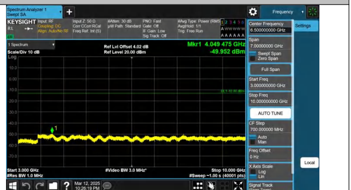
Band5-5MHz-QPSK-20425-1RB#24-3000~10000-PASS
