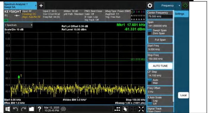
Band5-5MHz-QPSK-20425-1RB#24-0.009~0.15-PASS
