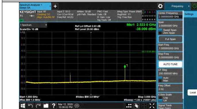
Band5-10MHz-QPSK-20525-1RB#49.1000~3000-PASS
