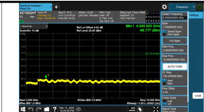
Band5-5MHz-QPSK-20625-1RB#24-3000~10000-PASS
