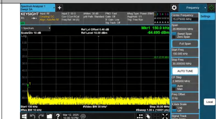
Band5-10MHz-QPSK-20450-1RB#0-0.15~30-PASS
