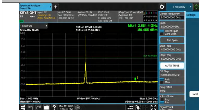
Band2-15MHz-QPSK-19125-1RB#74-1000~3000-PASS
