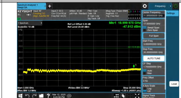
Band2-15MHz-QPSK-19125-1RB#74-3000~20000-PASS
