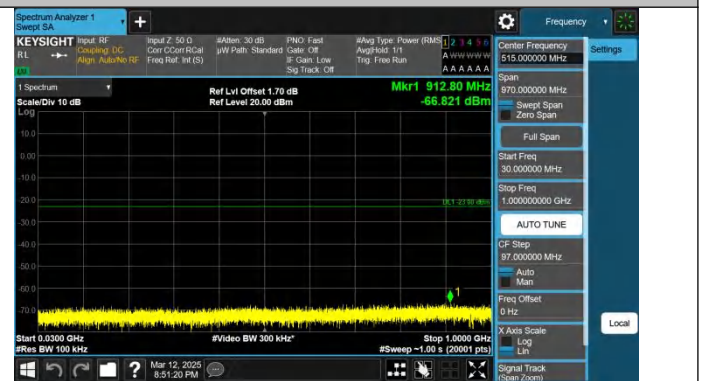
Band2-20MHz-QPSK-18700-1RB#99-30~1000-PASS
