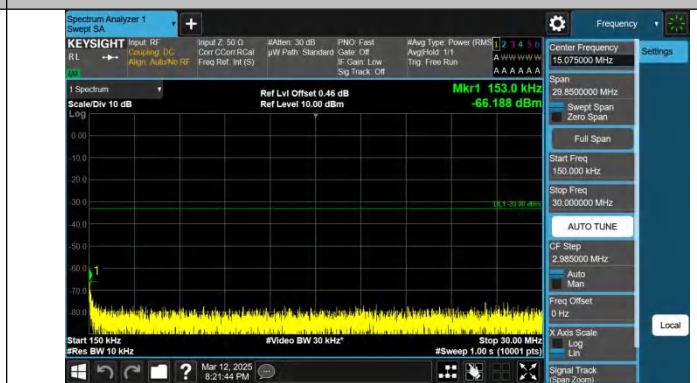
Band2-5MHz-QPSK-18625-1RB#0-0.15~30-PASS
