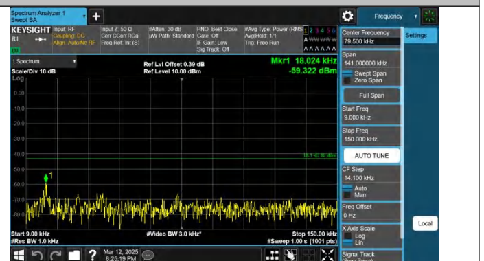
Band2-5MHz-QPSK-19175-1RB#24-0.009~0.15-PASS
