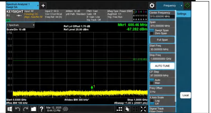
Band2-15MHz-QPSK-18900-1RB#74-30~1000-PASS
