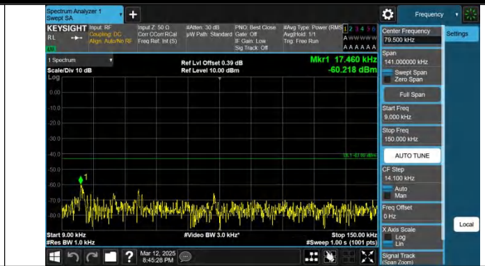
Band2-15MHz-QPSK-19125-1RB#74-0.009~0.15-PASS
