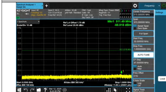
Band2-15MHz-QPSK-18900-1RB#0-30~1000-PASS
