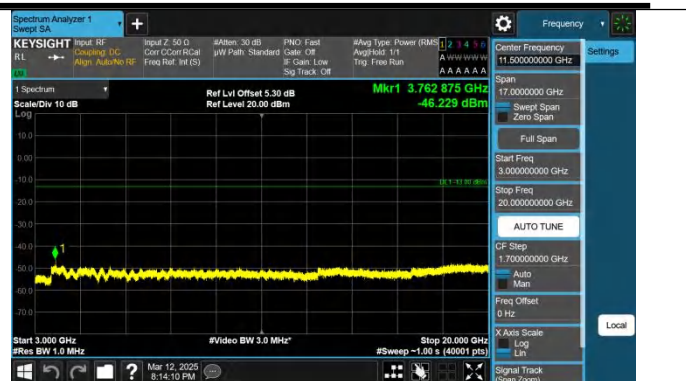
Band2-3MHz-QPSK-18900-1RB#14-3000~20000-PASS
