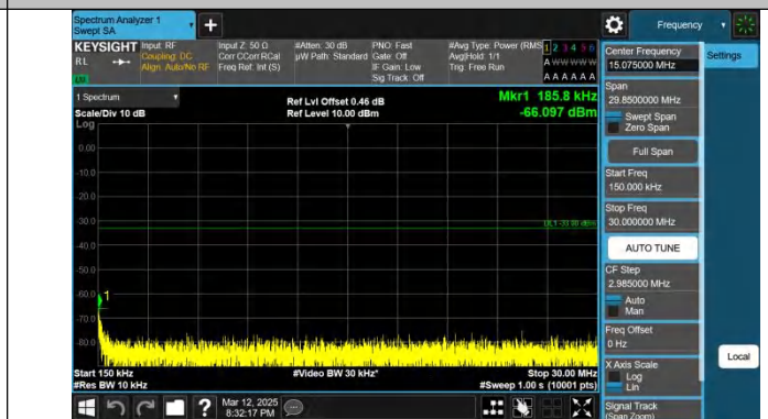
Band2-10MHz-QPSK-18650-1RB#0-0.15~30-PASS
