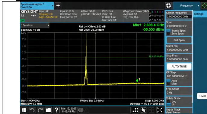
Band2-15MHz-QPSK-18675-1RB#74-1000~3000-PASS
