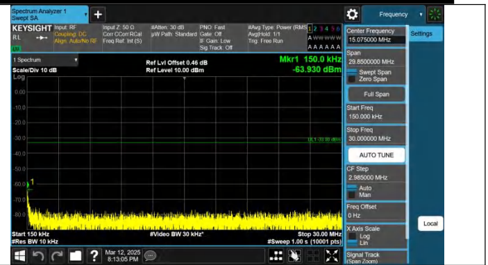
Band2-3MHz-QPSK-18900-1RB#0-0.15~30-PASS
