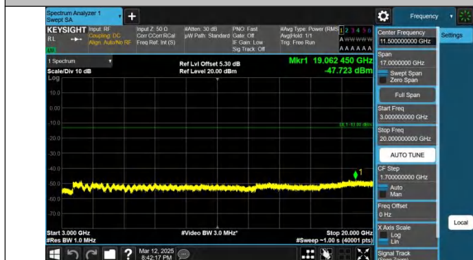
Band2-15MHz-QPSK-18675-1RB#0-3000~20000-PASS
