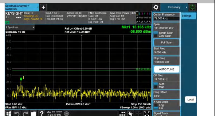
Band2-15MHz-QPSK-18900-1RB#74-0.009~0.15-PASS
