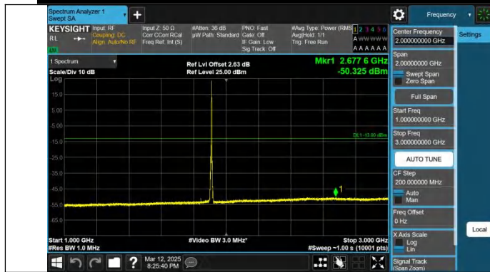
Band2-5MHz-QPSK-19175-1RB#24-1000~3000-PASS
