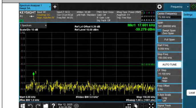
Band2-20MHz-QPSK-18700-1RB#0-0.009~0.15-PASS
