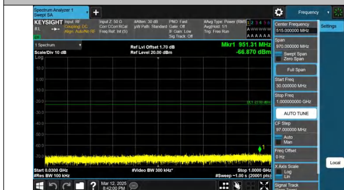
Band2-15MHz-QPSK-18675-1RB#0-30~1000-PASS
