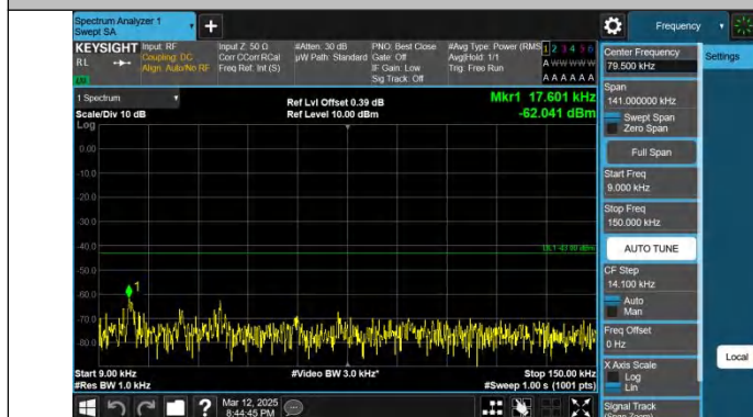
Band2-15MHz-QPSK-19125-1RB#0-0.009~0.15-PASS
