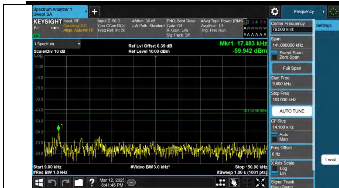
Band2-15MHz-QPSK-18675-1RB#0-0.009~0.15-PASS
