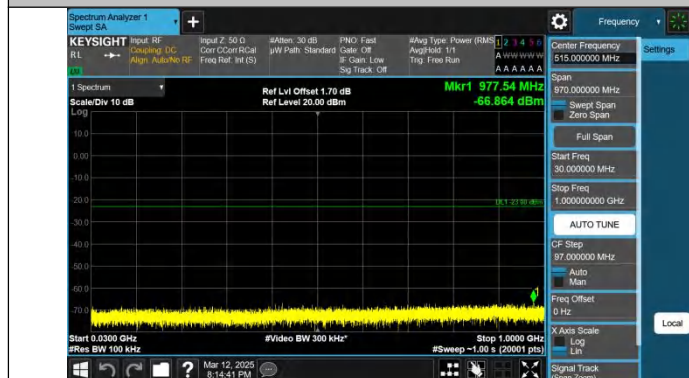
Band2-3MHz-QPSK-19185-1RB#0-30~1000-PASS
