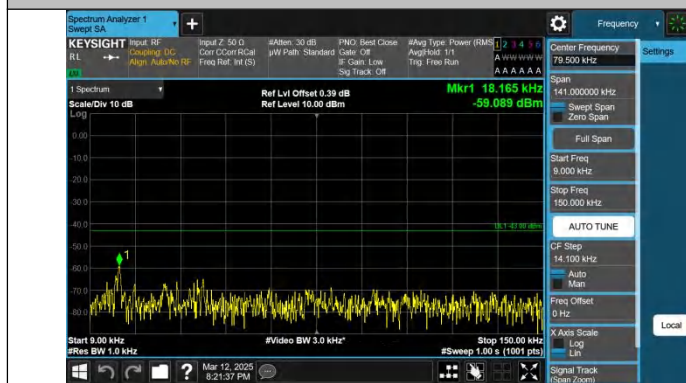
Band2-5MHz-QPSK-18625-1RB#0-0.009~0.15-PASS
