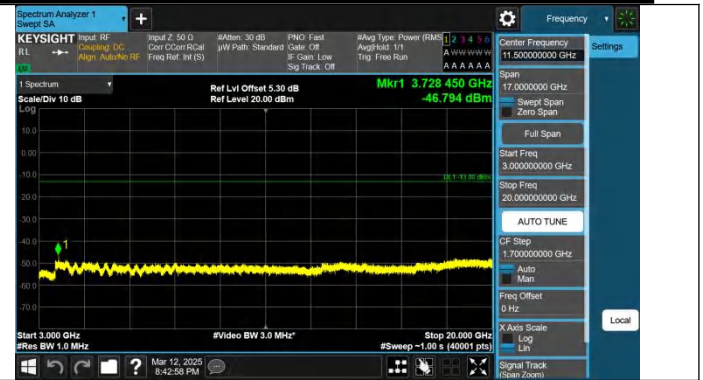
Band2-15MHz-QPSK-18675-1RB#74-3000~20000-PASS
