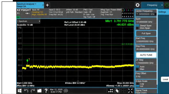
Band2-15MHz-QPSK-19125-1RB#0-3000~20000-PASS
