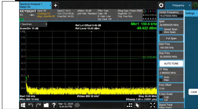
Band2-15MHz-QPSK-18900-1RB#74-0.15~30-PASS
