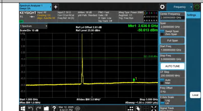
Band2-10MHz-QPSK-18650-1RB#0-1000~3000-PASS
