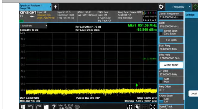
Band2-15MHz-QPSK-19125-1RB#0-30~1000-PASS
