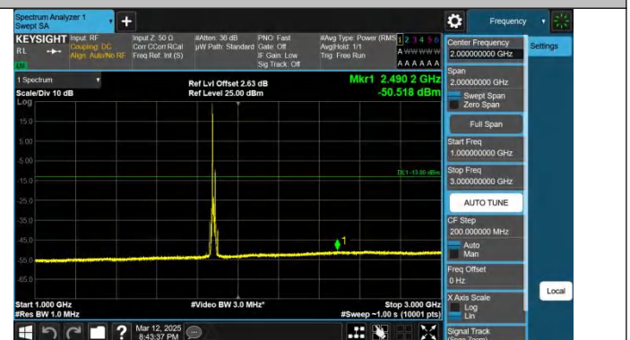
Band2-15MHz-QPSK-18900-1RB#0-1000~3000-PASS
