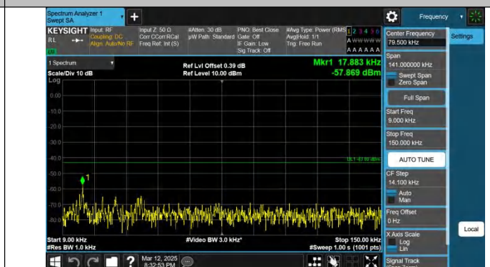
Band2-10MHz-QPSK-18650-1RB#49-0.009~0.15-PASS
