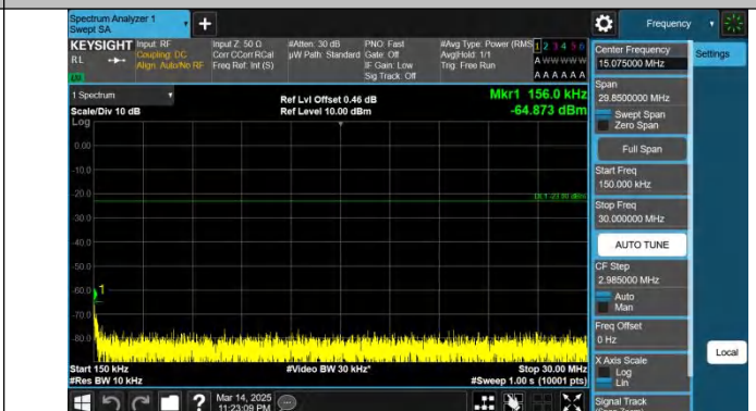
Band71-15MHz-QPSK-133297-1RB#0-0.15~30-PASS
