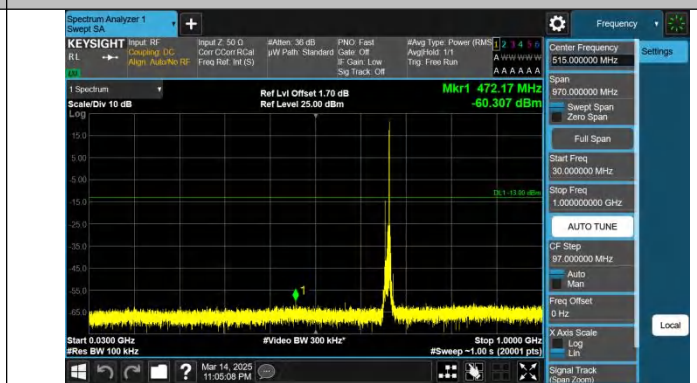
Band71-10MHz-QPSK-133172-1RB#49-30~1000-PASS
