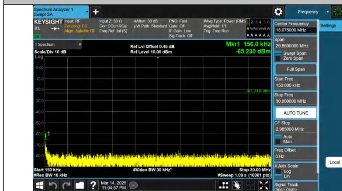
Band71-10MHz-QPSK-133172-1RB#49-0.15~30-PASS
