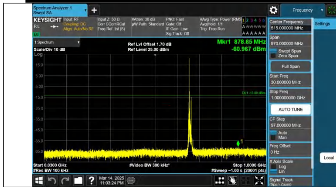
Band71-10MHz-QPSK-133172-1RB#0-30~1000-PASS
