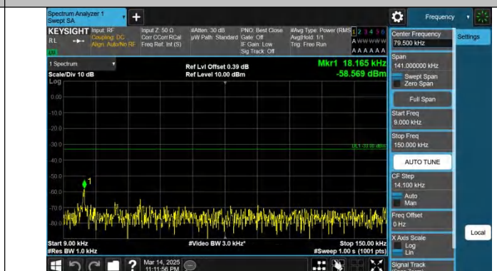
Band71-10MHz-QPSK-133422-1RB#49-0.009~0.15-PASS
