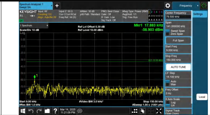
Band71-15MHz-QPSK-133197-1RB#74-0.009~0.15-PASS
