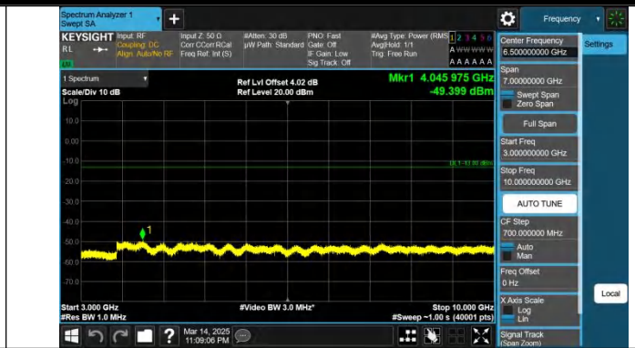
Band71-10MHz-QPSK-133297-1RB#49-3000~10000-PASS
