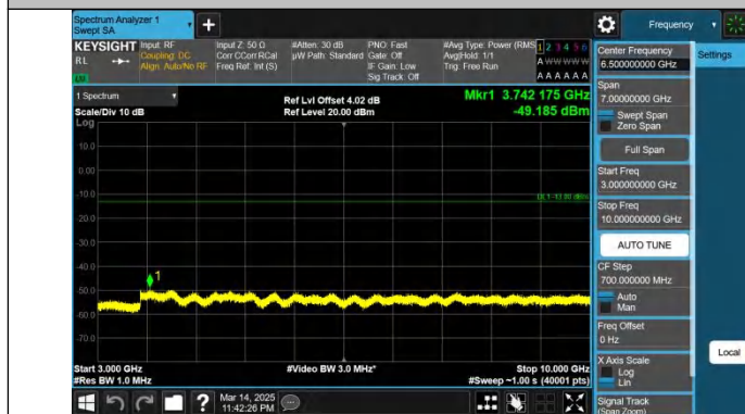
Band71-20MHz-QPSK-133372-1RB#0-3000~10000-PASS
