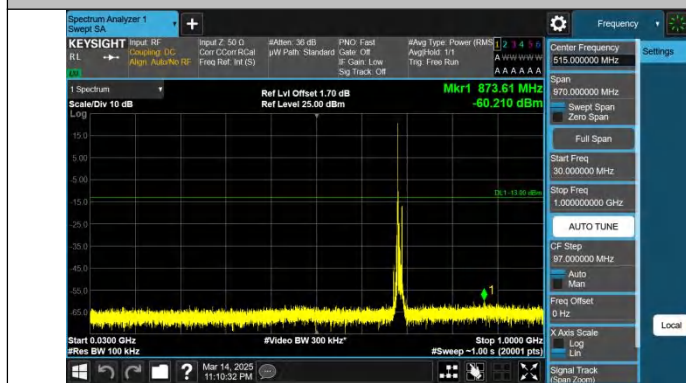
Band71-10MHz-QPSK-133422-1RB#0-30~1000-PASS
