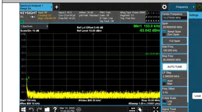
Band71-20MHz-QPSK-133372-1RB#99-0.15~30-PASS
