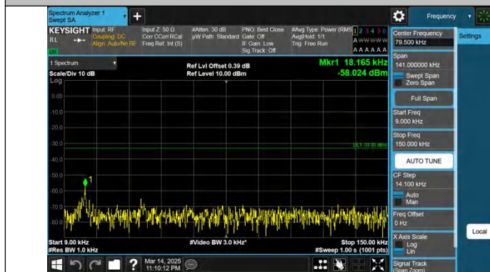
Band71-10MHz-QPSK-133422-1RB#0-0.009~0.15-PASS
