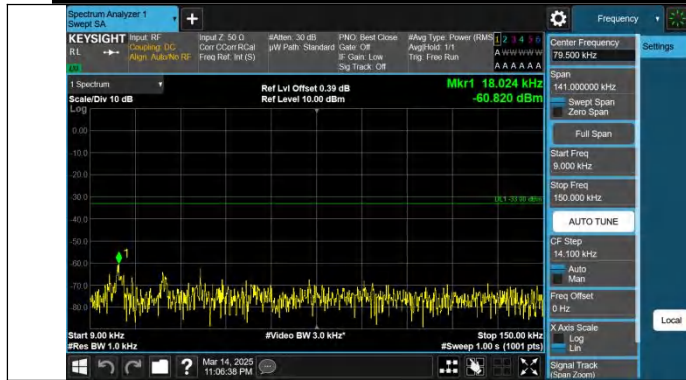
Band71-10MHz-QPSK-133297-1RB#0-0.009~0.15-PASS
