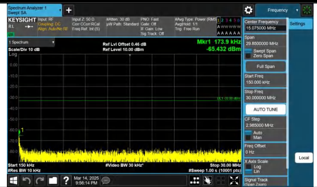
Band66-3MHz-QPSK-132322-1RB#0-0.15~30-PASS
