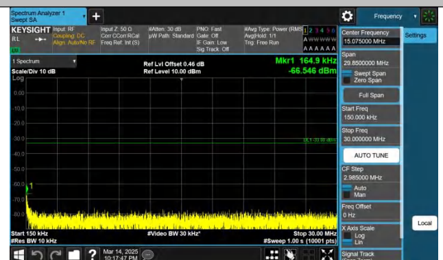
Band66-10MHz-QPSK-132622-1RB#0-0.15~30-PASS
