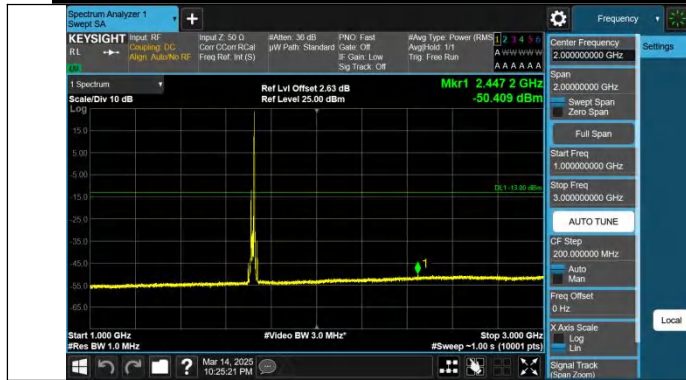
Band66-15MHz-QPSK-132047-1RB#74-1000~3000-PASS
