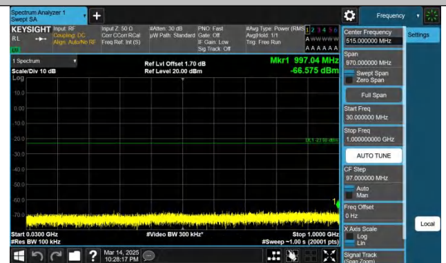
Band66-15MHz-QPSK-132597-1RB#74-30~1000-PASS
