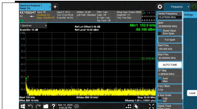
Band66-3MHz-QPSK-132657-1RB#14-0.15~30-PASS
