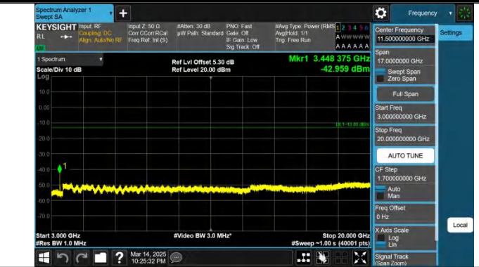
Band66-15MHz-QPSK-132047-1RB#74-3000~20000-PASS
