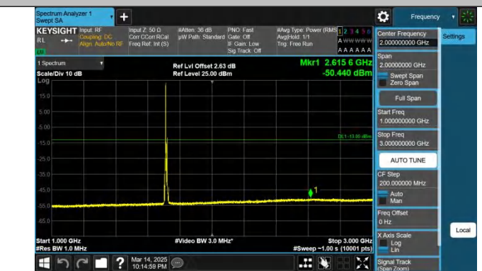
Band66-10MHz-QPSK-132022-1RB#0-1000~3000-PASS
