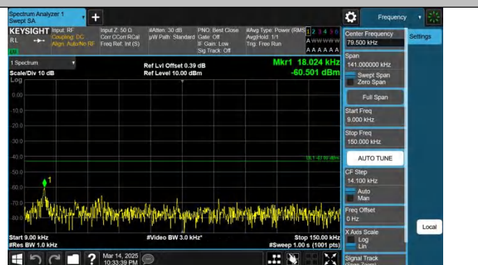
Band66-20MHz-QPSK-132072-1RB#99-0.009~0.15-PASS
