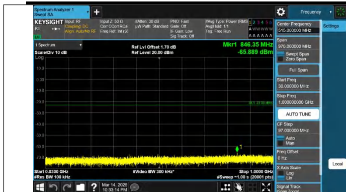
Band66-20MHz-QPSK-132072-1RB#0-30~1000-PASS
