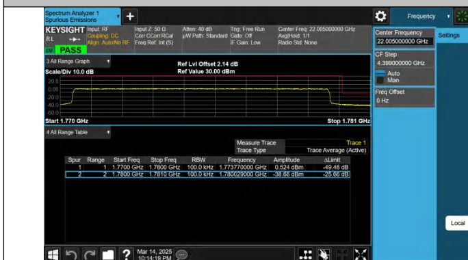
Band66-10MHz-QPSK-132622-50RB#0-PASS
