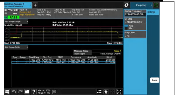
Band66-15MHz-QPSK-132047-75RB#0-PASS
