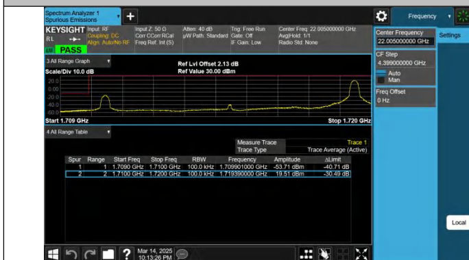
Band66-10MHz-QPSK-132022-1RB#49-PASS
