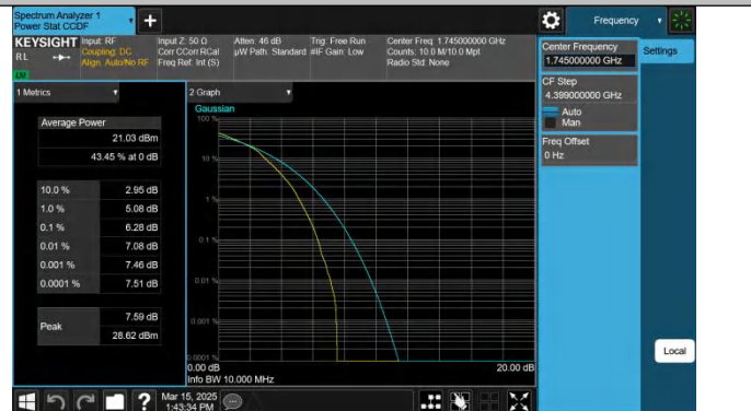
Band66-10MHz-16QAM@QPSK-132322-27RB#0-PASS
