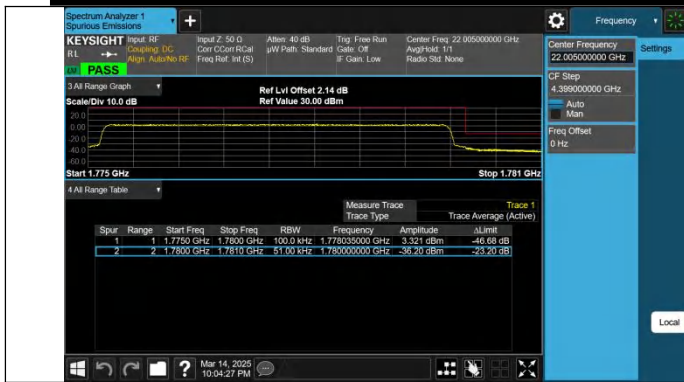
Band66-5MHz-QPSK-132647-25RB#0-PASS
