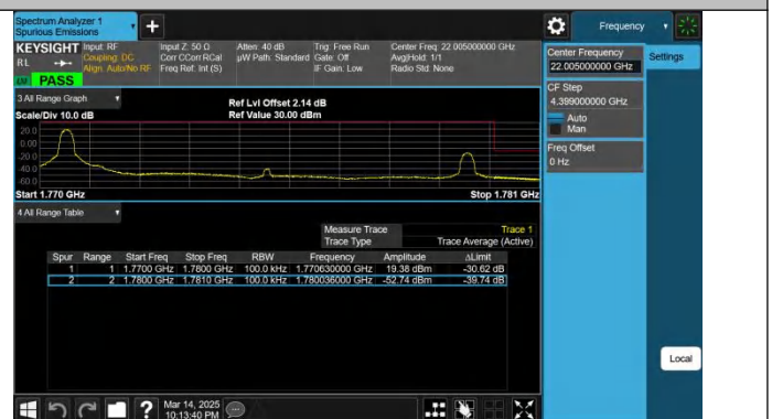
Band66-10MHz-QPSK-132622-1RB#0-PASS
