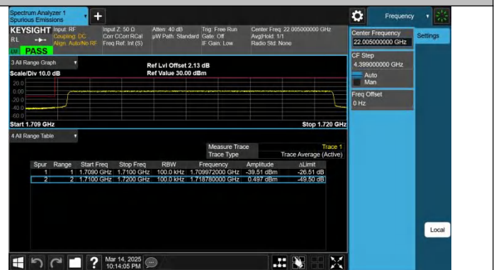
Band66-10MHz-QPSK-132022-50RB#0-PASS
