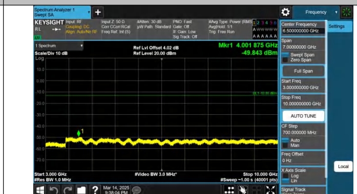
Band14-10MHz-QPSK-23330-1RB#49-3000~10000-PASS
