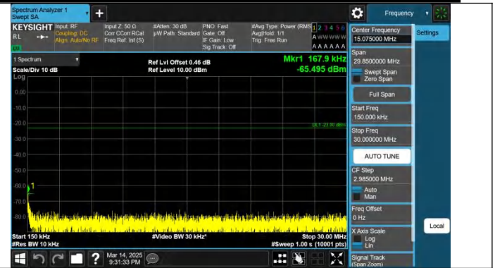
Band14-5MHz-QPSK-23355-1RB#0-0.15~30-PASS
