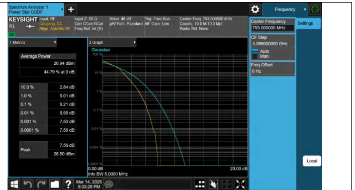
Band14-5MHz-16QAM-23330-25RB#0-PASS
