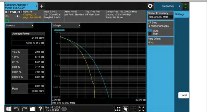
Band14-10MHz-16QAM-23330-27RB#0-PASS
