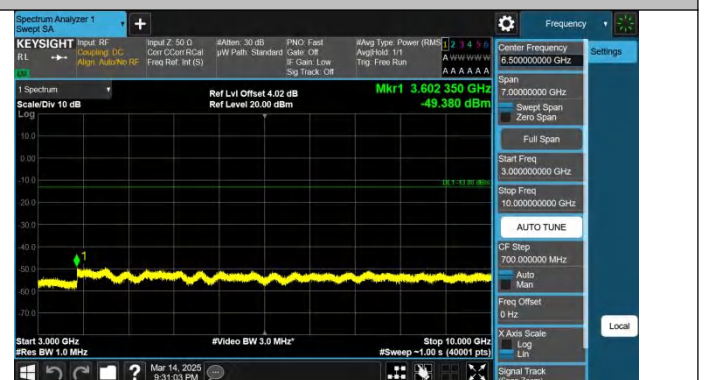
Band14-5MHz-QPSK-23330-1RB#24-3000~10000-PASS
