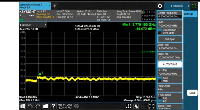
Band13-5MHz-QPSK-23230-1RB#0-3000~10000-PASS
