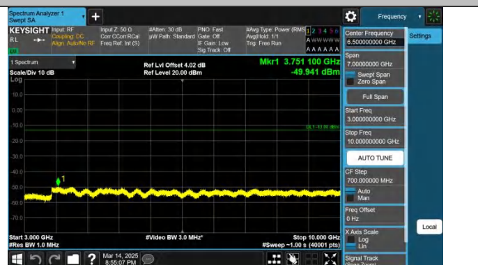
Band12-10MHz-QPSK-23095-1RB#49-3000~10000-PASS
