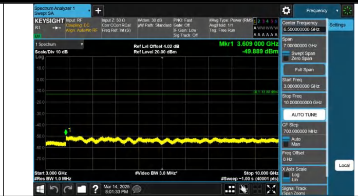
Band5-5MHz-QPSK-20625-1RB#24-3000~10000-PASS
