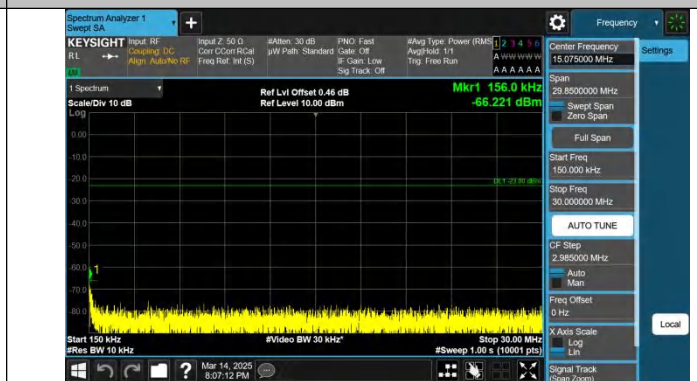
Band5-10MHz-QPSK-20450-1RB#0-0.15~30-PASS
