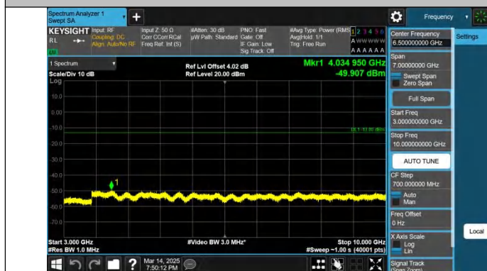
Band5-3MHz-QPSK-20635-1RB#0-3000~10000-PASS
