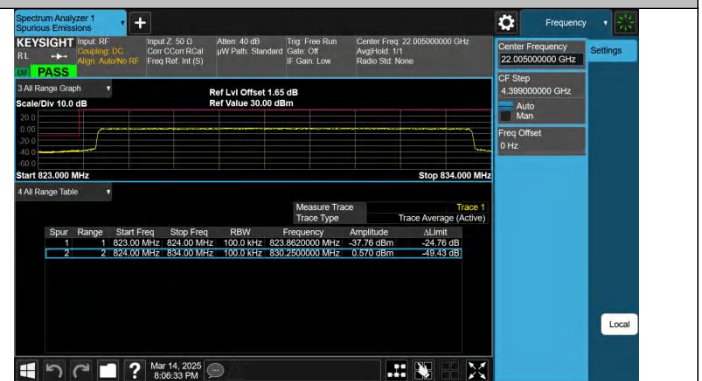
Band5-10MHz-QPSK-20450-50RB#0-PASS
