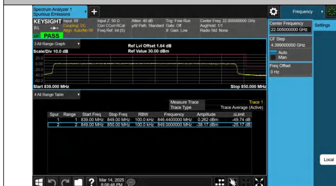
Band5-10MHz-QPSK-20600-50RB#0-PASS
