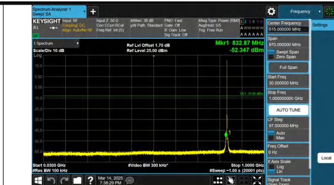
Band5-1.4MHz-QPSK-20525-1RB#5-30~1000-PASS
