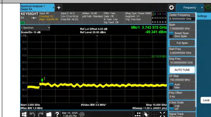
Band5-1.4MHz-QPSK-20525-1RB#5-3000~10000-PASS
