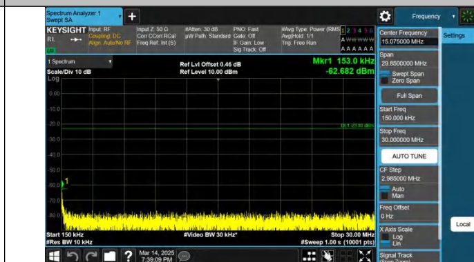
Band5-1.4MHz-QPSK-20643-1RB#0-0.15~30-PASS
