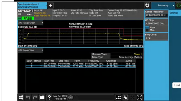
Band5-5MHz-QPSK-20625-25RB#0-PASS
