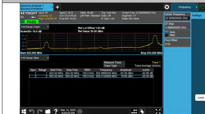
Band5-10MHz-QPSK-20450-1RB#49-PASS
