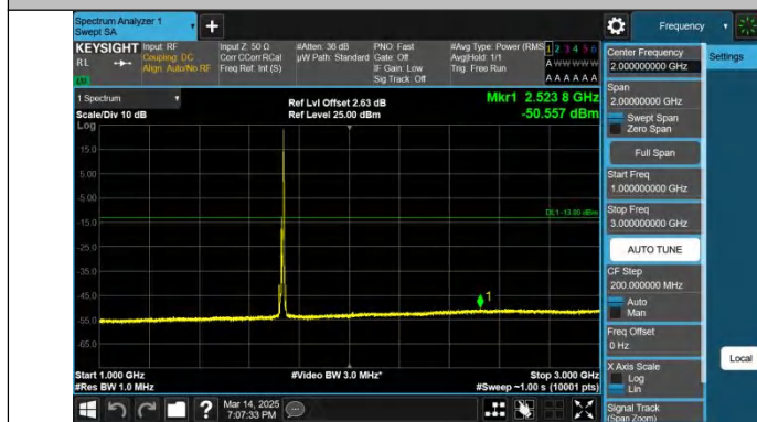
Band4-10MHz-QPSK-20175-1RB#49.1000~3000-PASS
