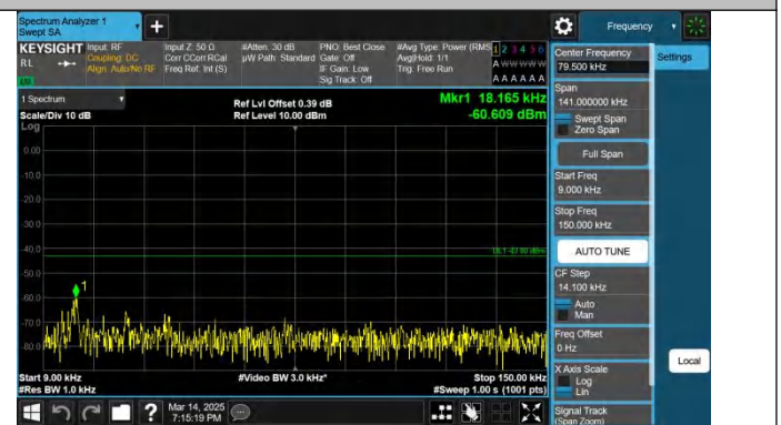
Band4-15MHz-QPSK-20025-1RB#74-0.009~0.15-PASS
