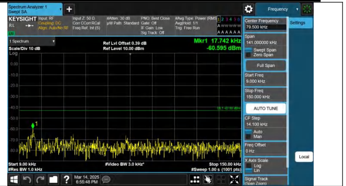
Band4-5MHz-QPSK-19975-1RB#24-0.009~0.15-PASS
