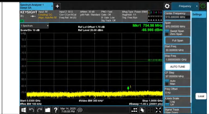
Band4-10MHz-QPSK-20000-1RB#49-30~1000-PASS
