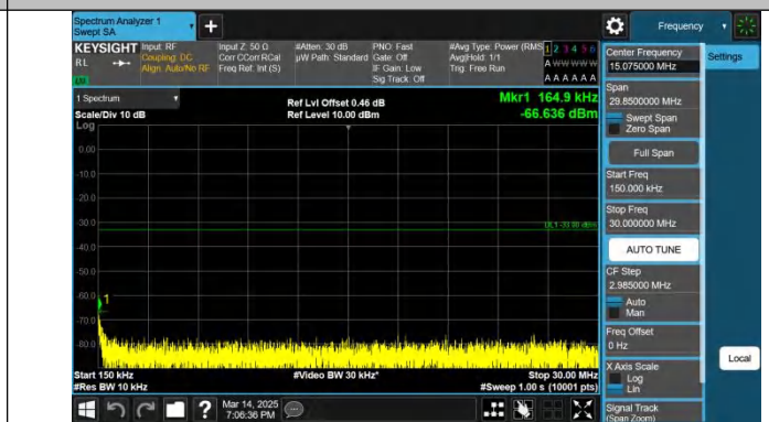
Band4-10MHz-QPSK-20175-1RB#0-0.15~30-PASS
