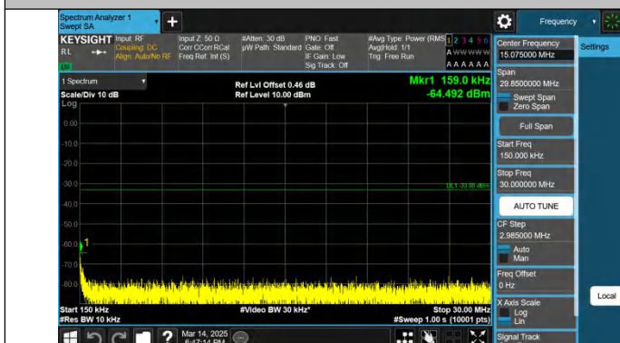
Band4-3MHz-QPSK-20175-1RB#14-0.15~30-PASS
