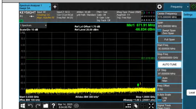
Band2-10MHz-QPSK-18650-1RB#0-30~1000-PASS
