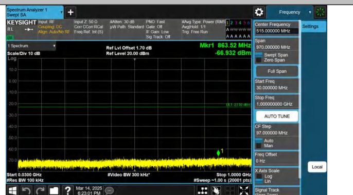
Band2-20MHz-QPSK-18700-1RB#99-30~1000-PASS
