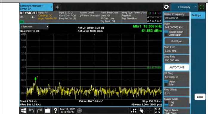
Band2-15MHz-QPSK-18675-1RB#74-0.009~0.15-PASS
