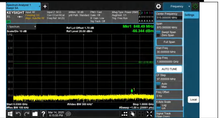
Band2-15MHz-QPSK-18900-1RB#74-30~1000-PASS
