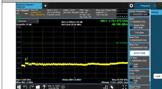
Band2-20MHz-QPSK-18700-1RB#0-3000~20000-PASS
