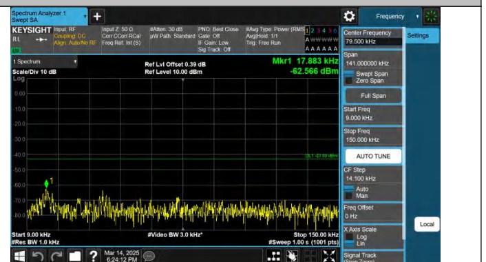
Band2-20MHz-QPSK-18900-1RB#99-0.009~0.15-PASS
