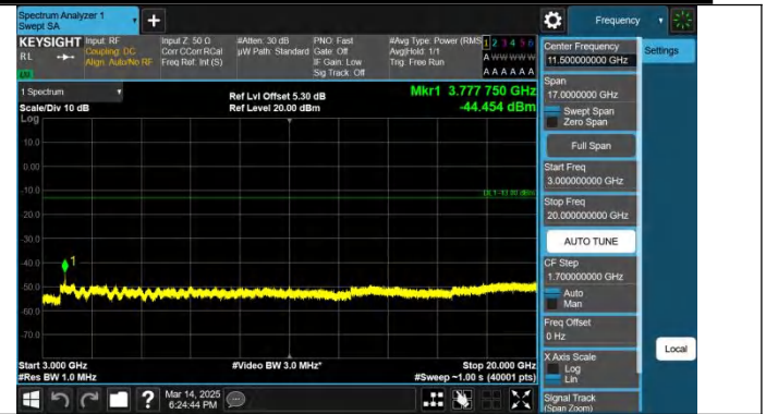
Band2-20MHz-QPSK-18900-1RB#99-3000~20000-PASS
