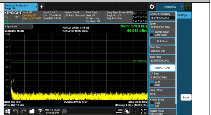
Band2-3MHz-QPSK-19185-1RB#0-0.15~30-PASS
