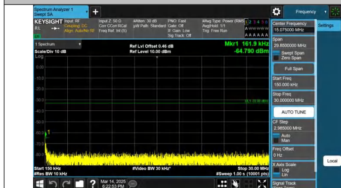
Band2-20MHz-QPSK-18700-1RB#99-0.15~30-PASS
