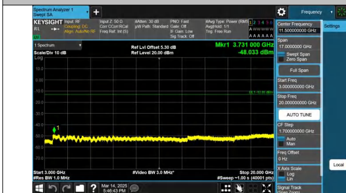
Band2-3MHz-QPSK-19185-1RB#0-3000~20000-PASS
