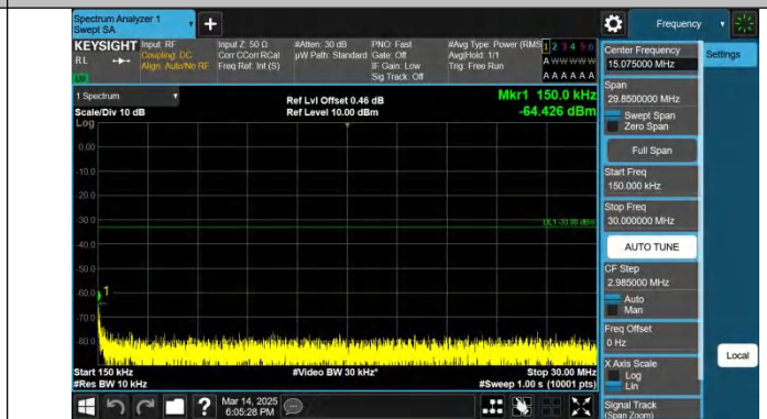
Band2-10MHz-QPSK-18900-1RB#0-0.15~30-PASS
