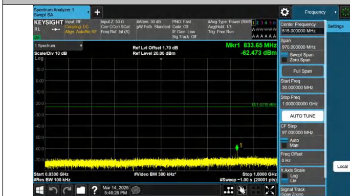
Band2-3MHz-QPSK-19185-1RB#0-30~1000-PASS
