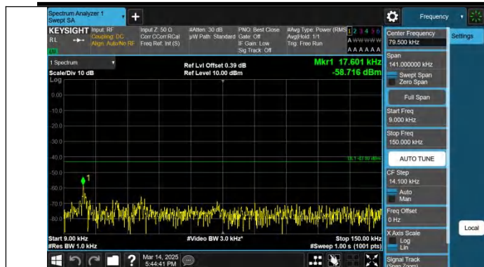
Band2-3MHz-QPSK-18900-1RB#0-0.009~0.15-PASS
