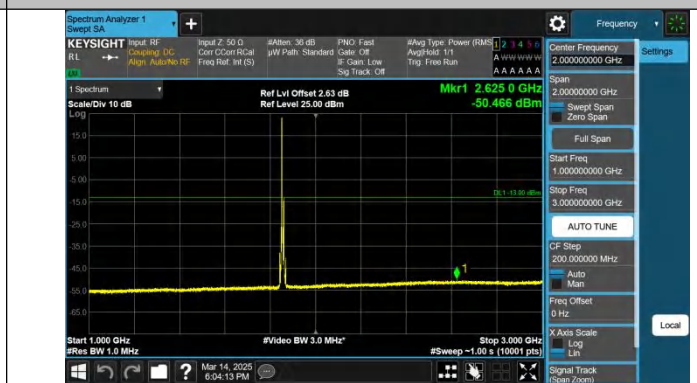
Band2-10MHz-QPSK-18650-1RB#0-1000~3000-PASS
