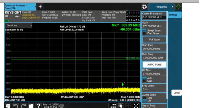
Band2-20MHz-QPSK-18900-1RB#99-30~1000-PASS
