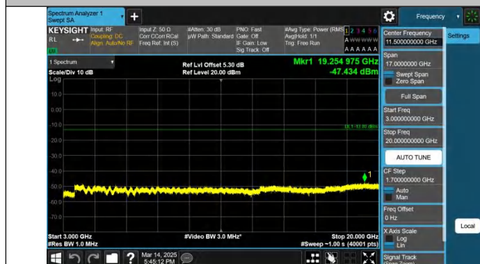
Band2-3MHz-QPSK-18900-1RB#0-3000~20000-PASS
