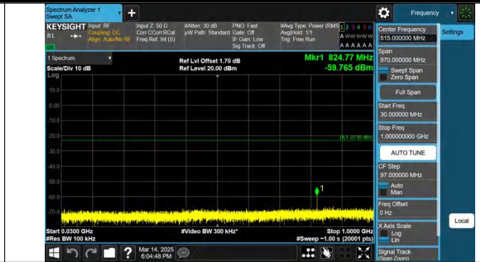
Band2-10MHz-QPSK-18650-1RB#49-30~1000-PASS
