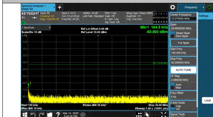
Band2-3MHz-QPSK-18900-1RB#14-0.15~30-PASS
