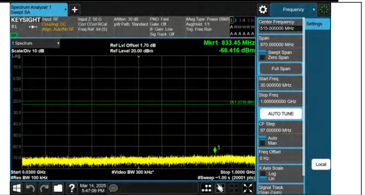
Band2-3MHz-QPSK-19185-1RB#14-30~1000-PASS
