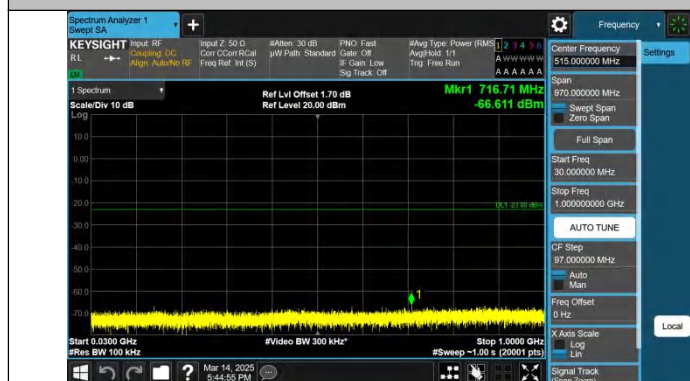
Band2-3MHz-QPSK-18900-1RB#0-30~1000-PASS
