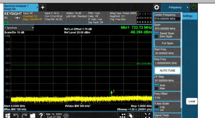
Band2-3MHz-QPSK-18900-1RB#14-30~1000-PASS
