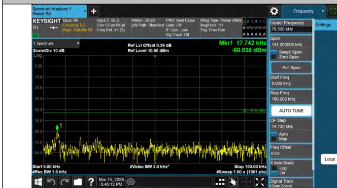
Band2-3MHz-QPSK-19185-1RB#0-0.009~0.15-PASS
