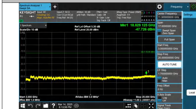
Band2-15MHz-QPSK-18675-1RB#0-3000~20000-PASS
