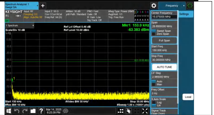
Band2-20MHz-QPSK-18900-1RB#0-0.15~30-PASS
